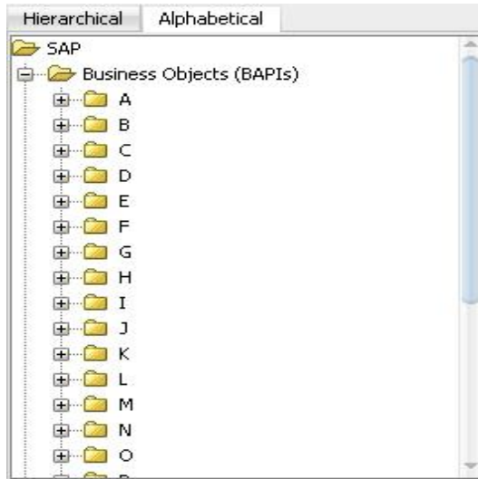
Figure 6-22 Alphabetical Tab
