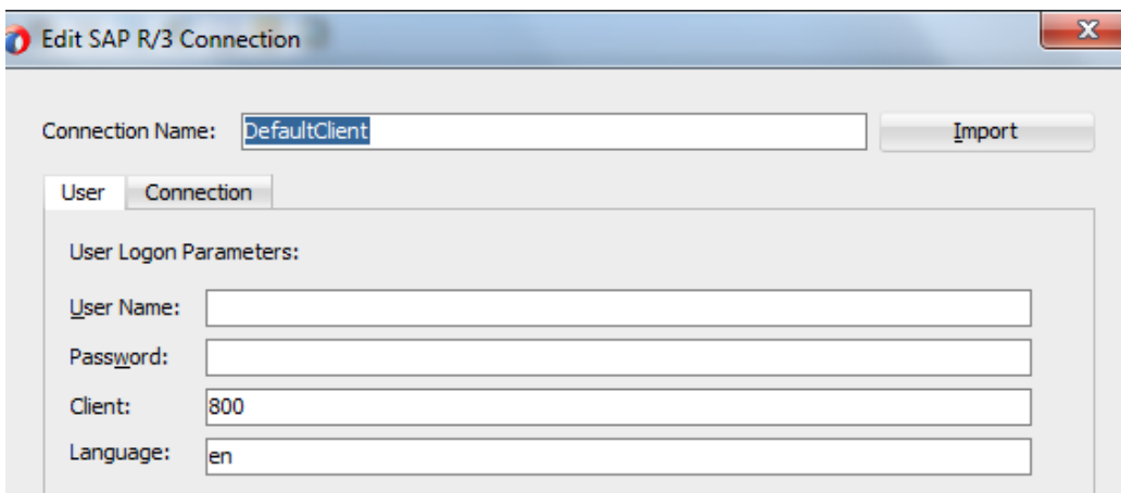
Figure 6-4 Import Button
