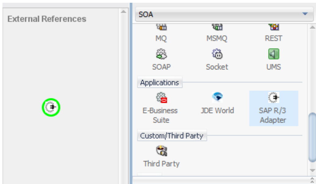
Figure 2-9 Adapter Component
