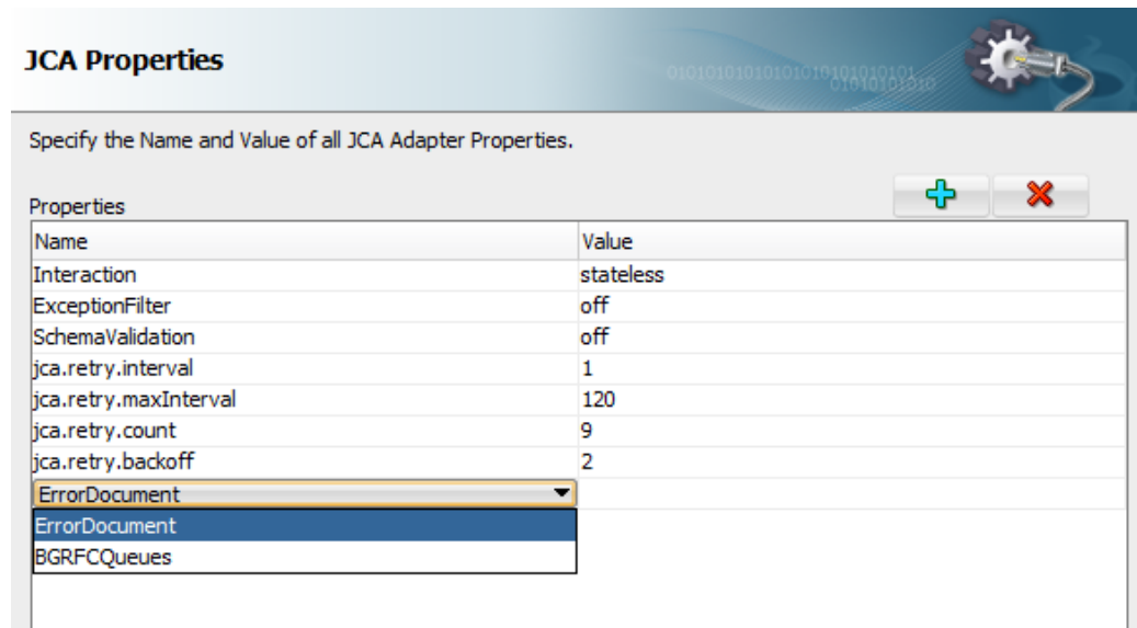
Figure 5-88 JCA Property
