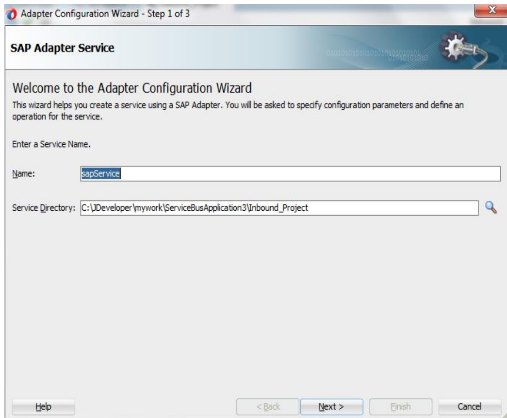
Figure 8-195 Welcome Page
