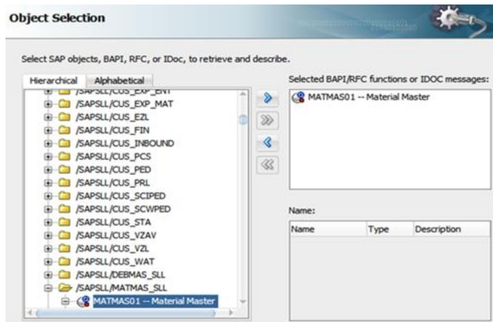
Figure 5-105 JCA Properties
