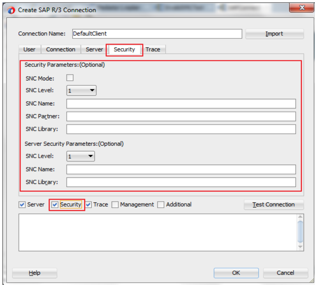
Figure 6-18 Security Tab
