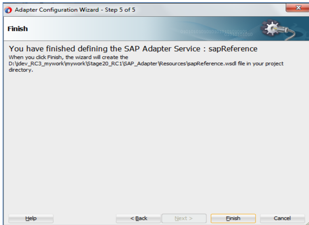
Figure 8-27 Finish Page
