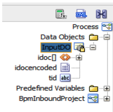
Figure 8-157 Data Object
