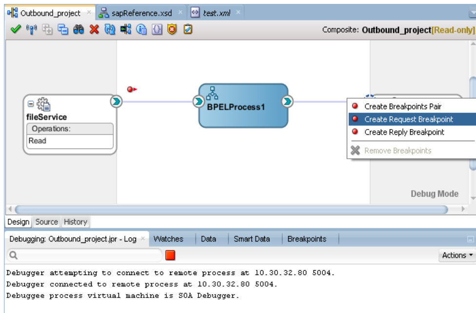
Figure 5-78 Breakpoint Options
