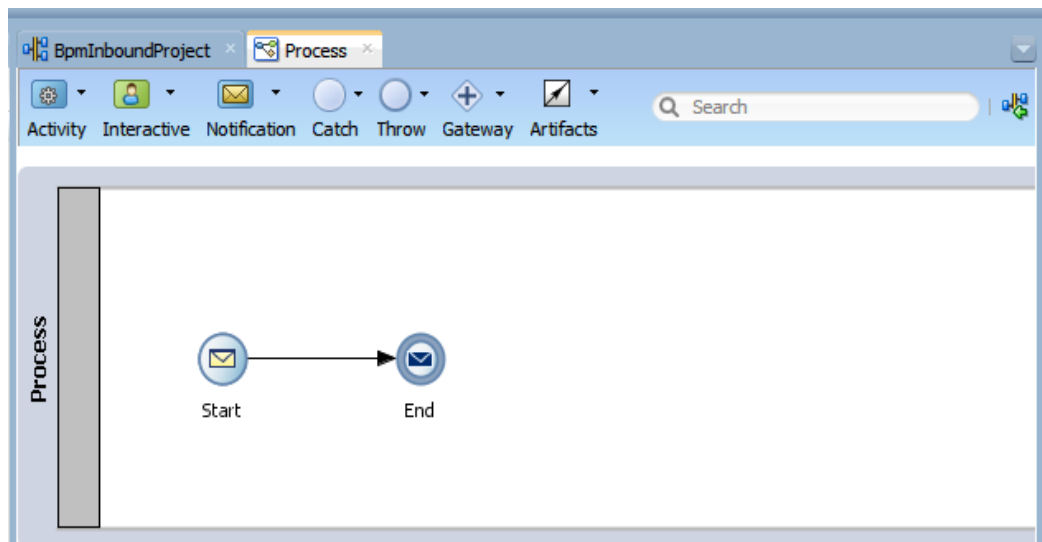
Figure 8-150 BPMN Process
