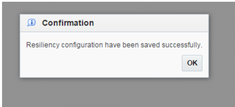
Figure 5-117 Confirmation Window
