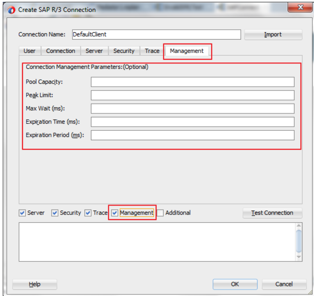
Figure 6-17 Management Tab
