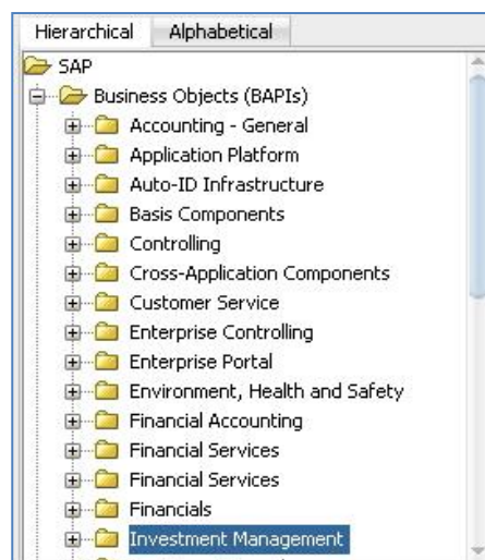
Figure 6-21 Hierarchical Tab
