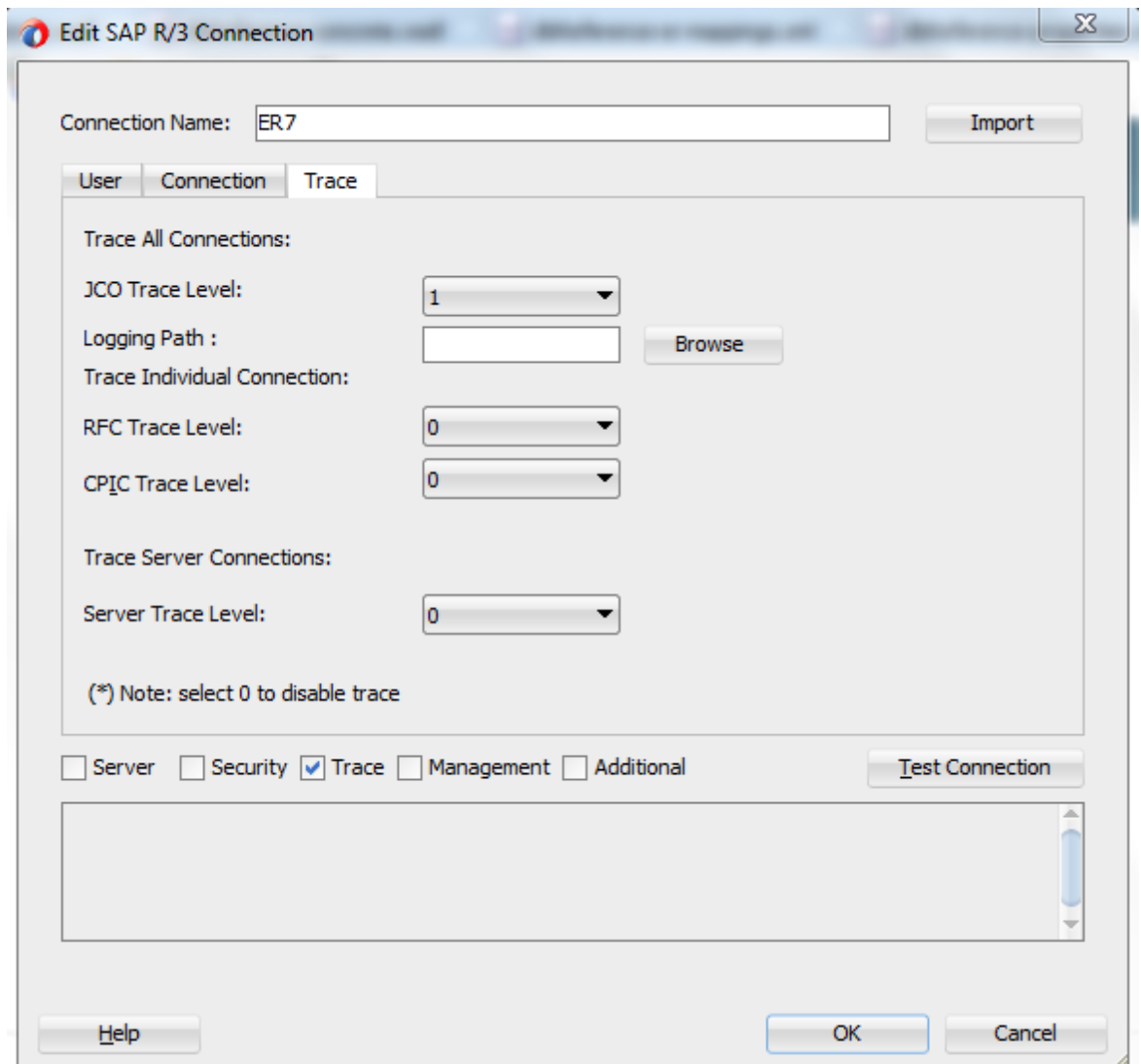
Figure 6-14 Trace Tab
