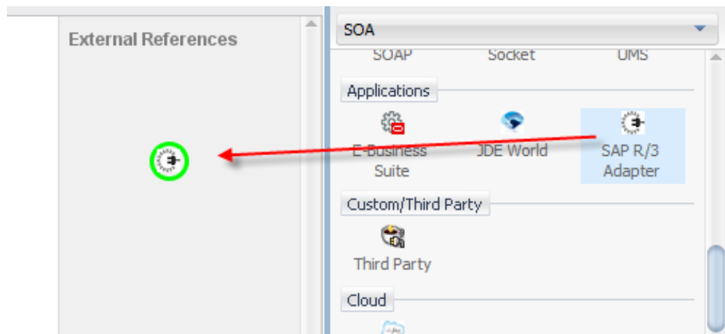
Figure 8-16 Adapter Component
