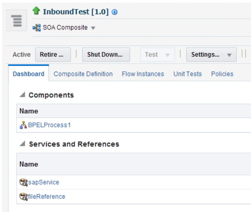
Figure 8-245 Instances Tab
