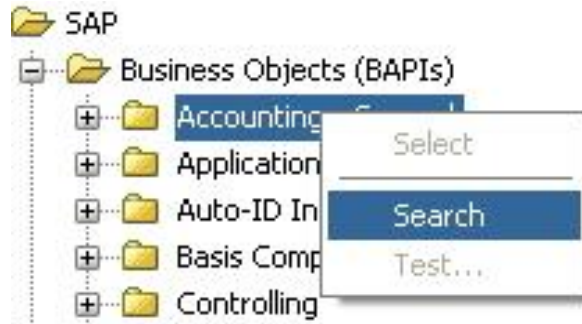
Figure 6-24 Search Option
