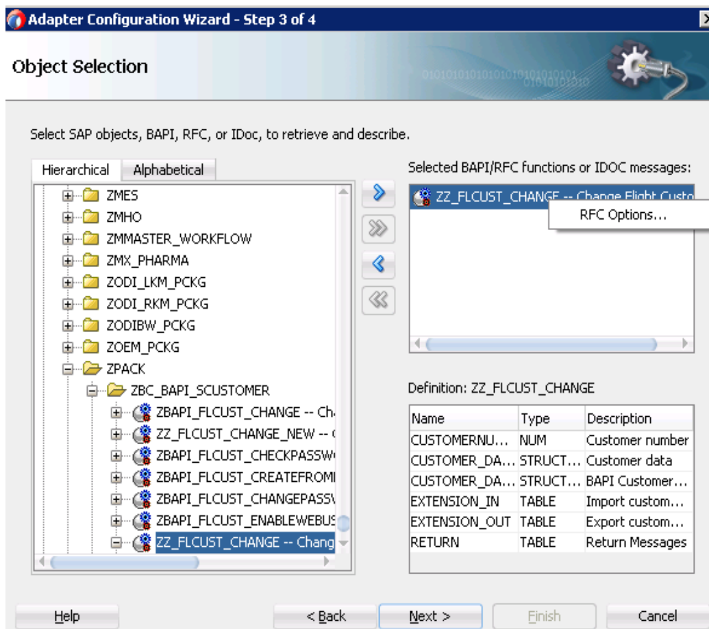
Figure 5-13 Select RFC
