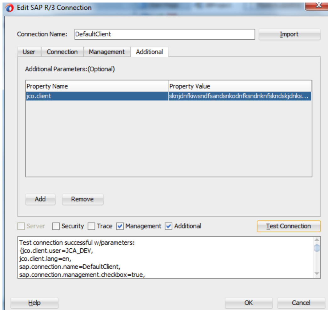
Figure 6-19 Additional Tab
