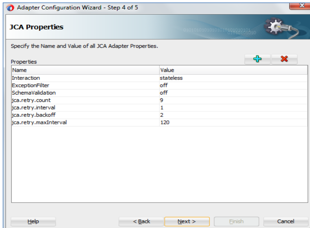
Figure 6-32 JCA Properties
