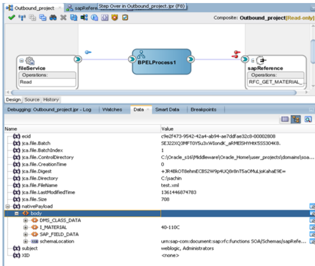
Figure 5-80 Breakpoint Options
