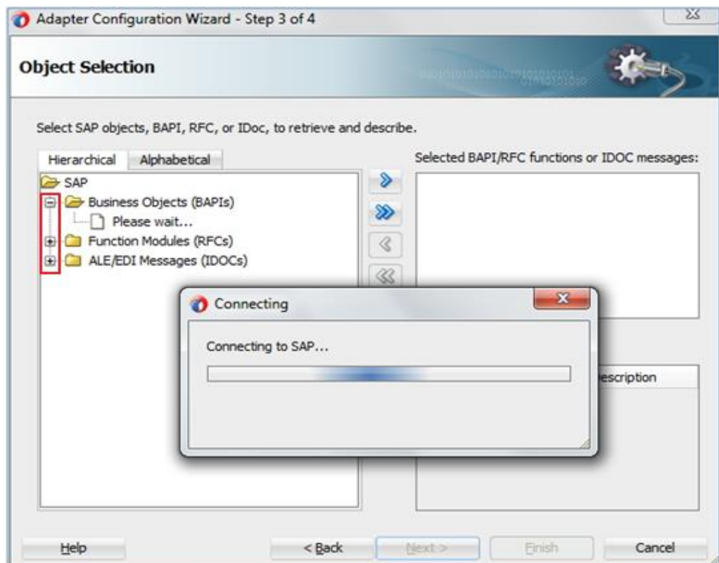
Figure 6-23 Expanded Node
