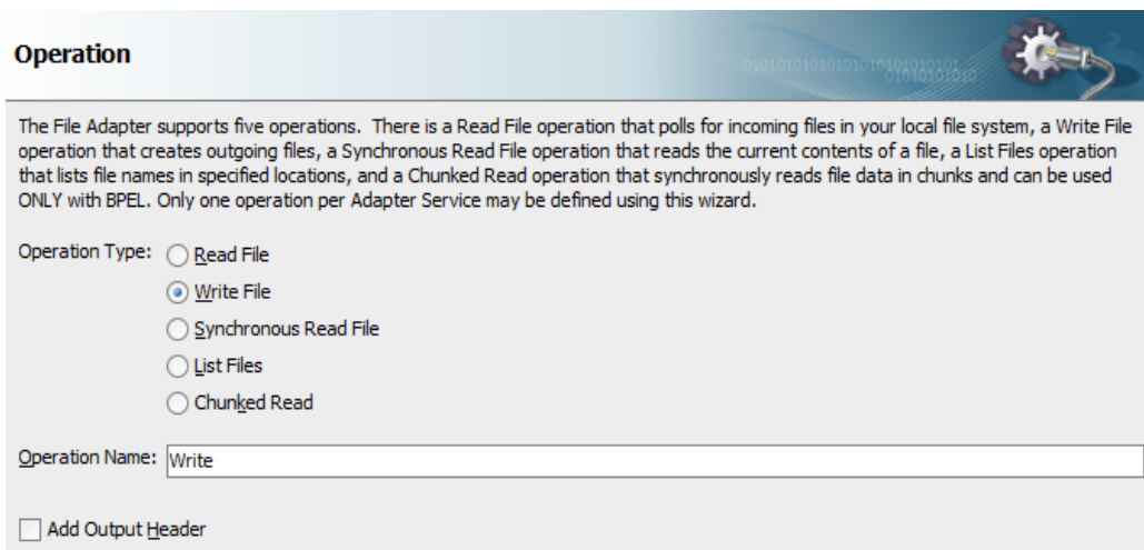
Figure 8-212 Operation Page
