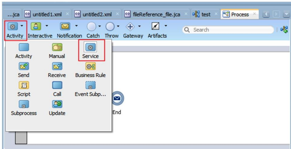
Figure 8-116 Activity Icon
