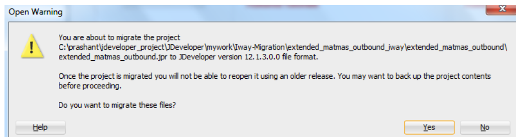
Figure 12-2 Open Warning
