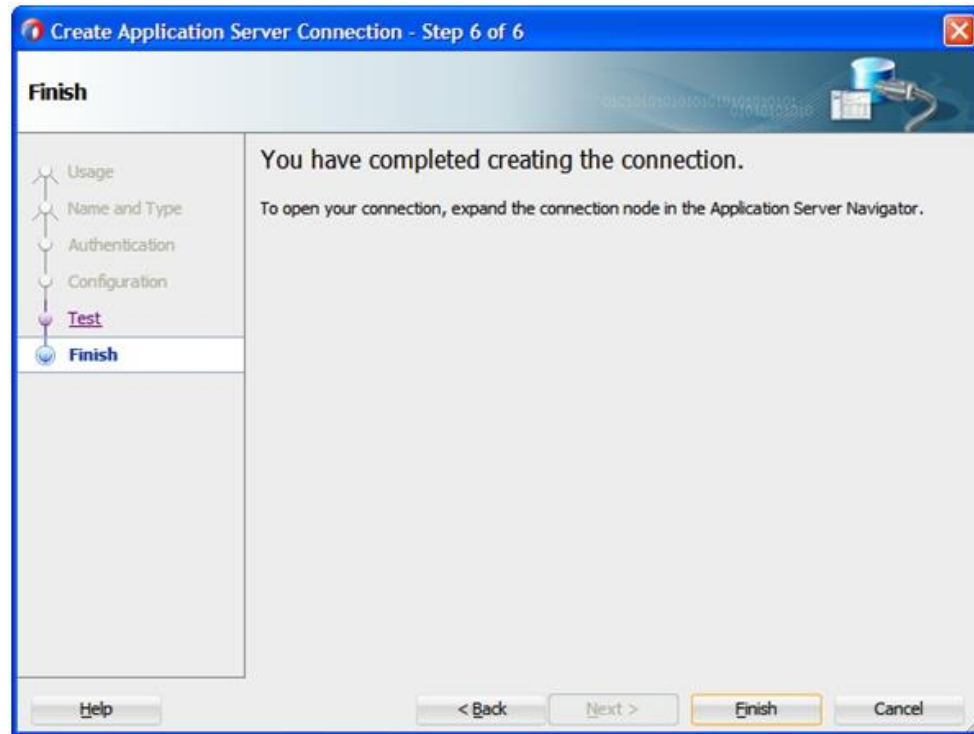
Figure 8-9 Finish Page
