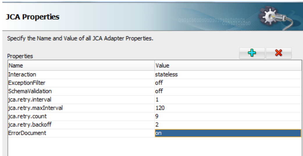
Figure 5-89 JCA Property
