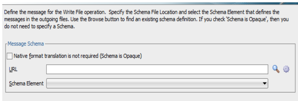
Figure 8-214 Messages Page
