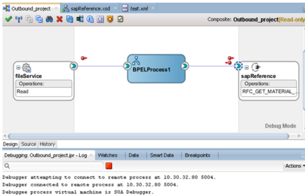
Figure 5-79 Breakpoint Options
