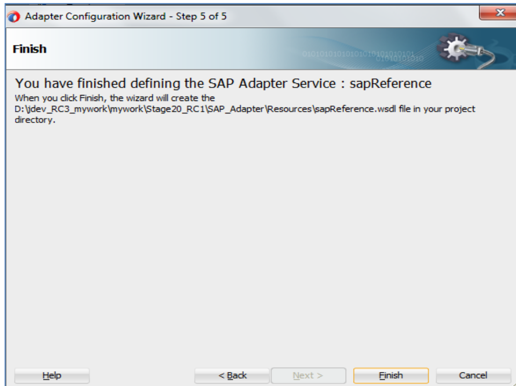
Figure 6-34 Finish Page
