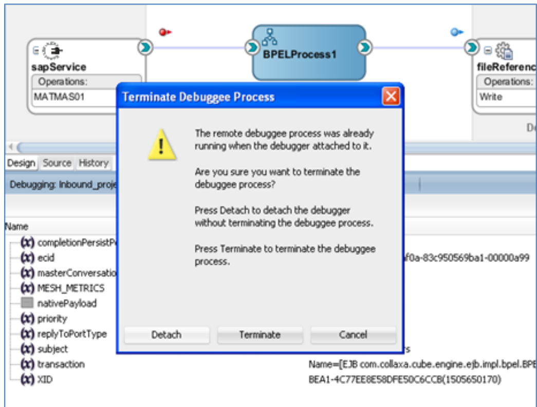
Figure 5-74 Detach Debugger
