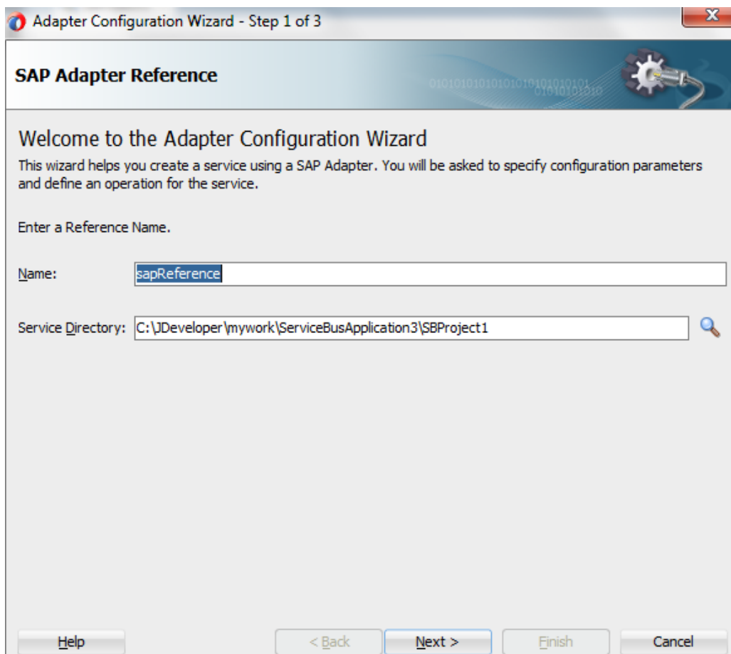
Figure 8-169 Welcome Page
