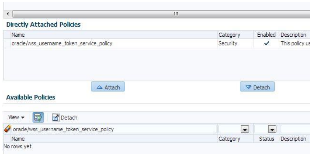
Figure 5-59 Search Policy
