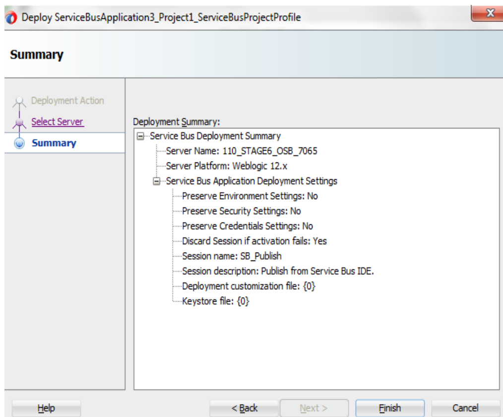
Figure 8-186 Summary Page
