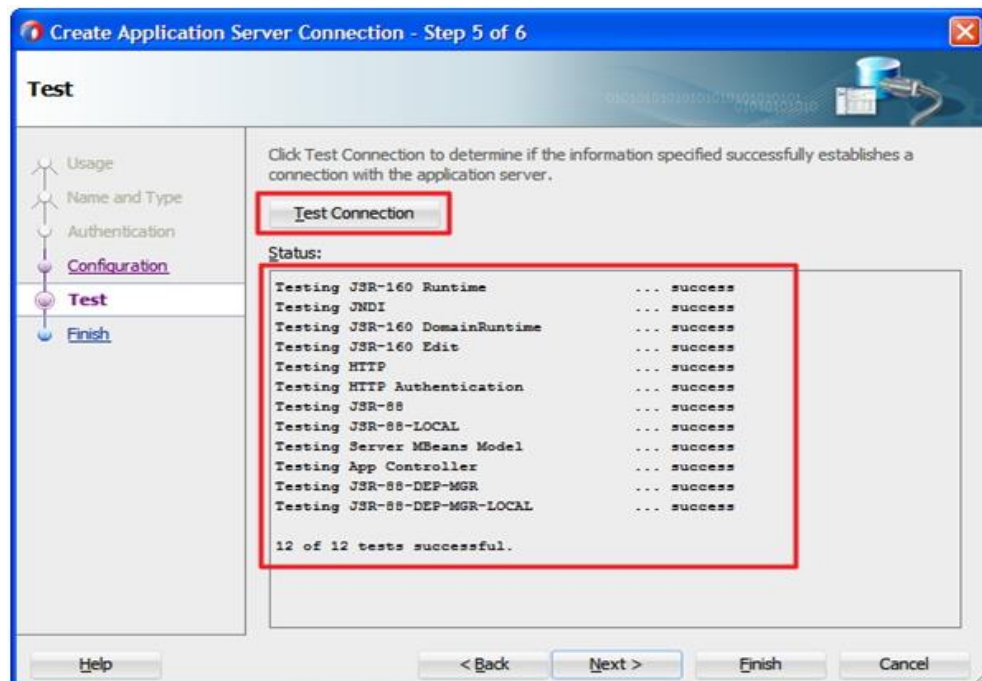
Figure 8-8 Test Page
