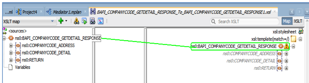
Figure 8-85 Mapping Page
