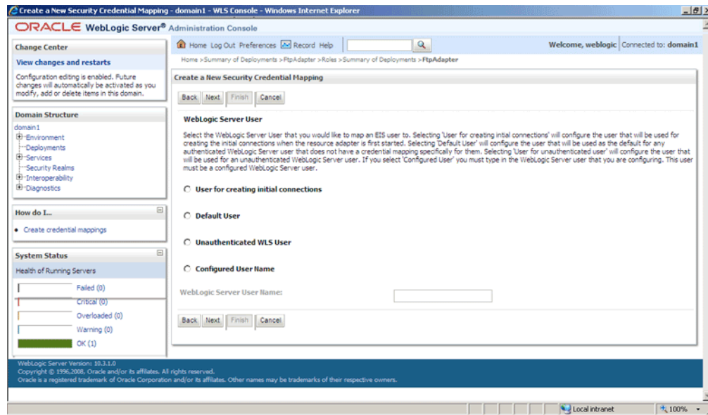
Figure 5-20 The Oracle WebLogic Server Administration Console - Create a New Security Credential Mapping Page
