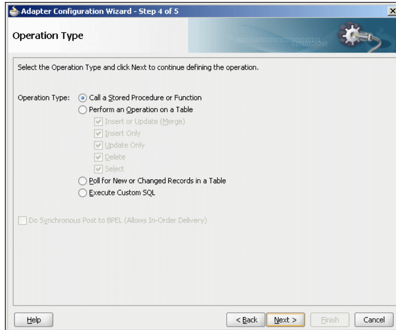
Figure 9-66 The Adapter Configuration Wizard - Operation Type Page
