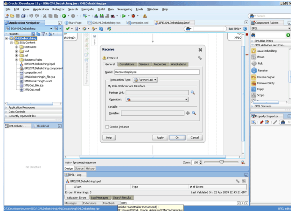
Figure 5-74 The JDeveloper - BPELXMLDebatching.bpel
