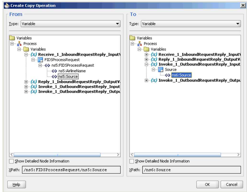
Figure 6-93 The Create Copy Operation Dialog
