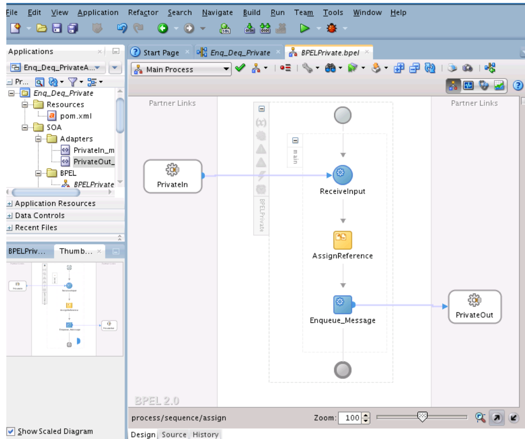
Figure 13-29 BPELPublic.bpel Page After Wiring Elements
