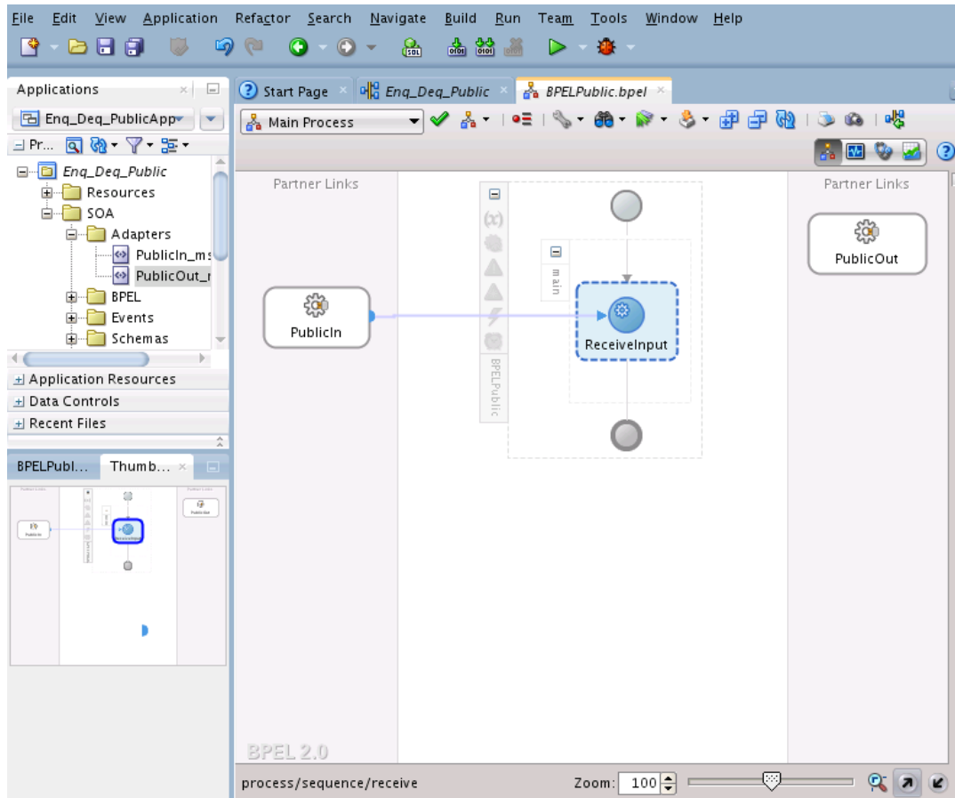
Figure 13-10 JDeveloper BPELPublic.bpel Page Showing the PublicIn Partner Link Wired to the Receive Activity
