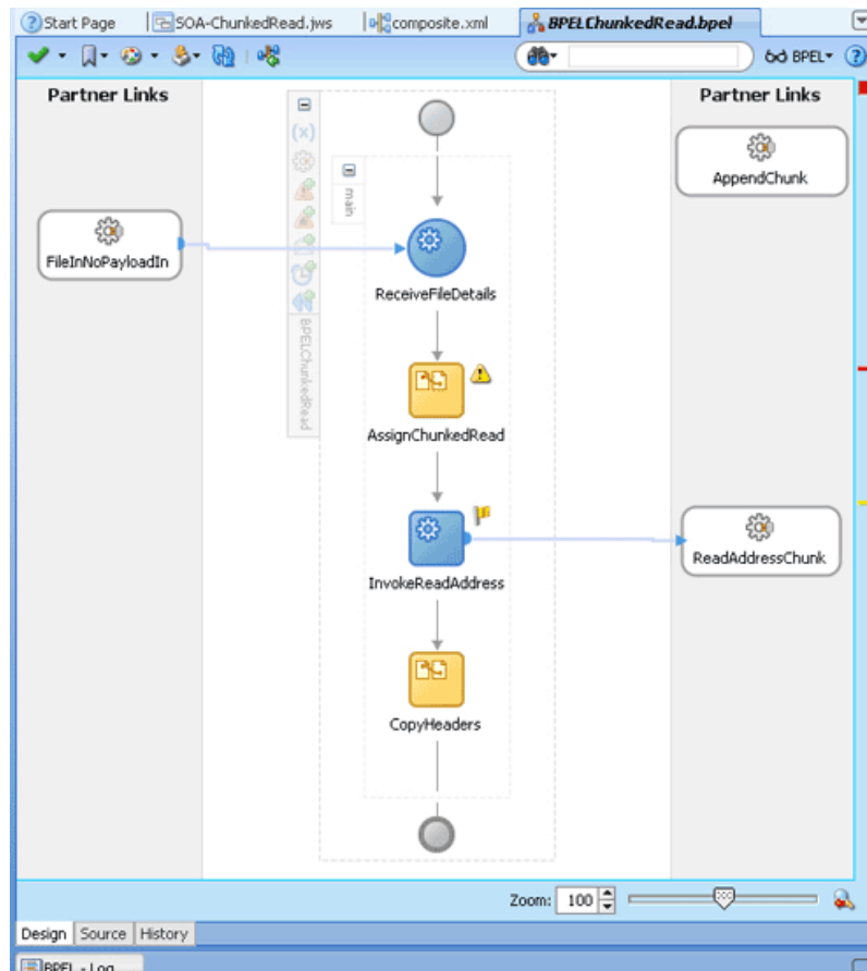
Figure 5-121 The JDeveloper - BPELChunkedRead.bpel
