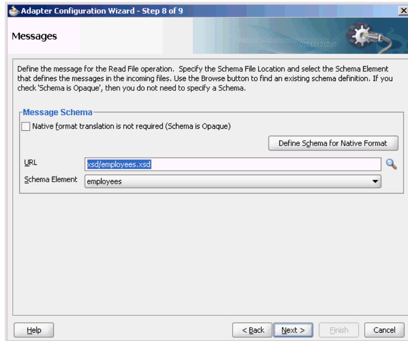
Figure 5-69 The Adapter Configuration Wizard File Messages Page
