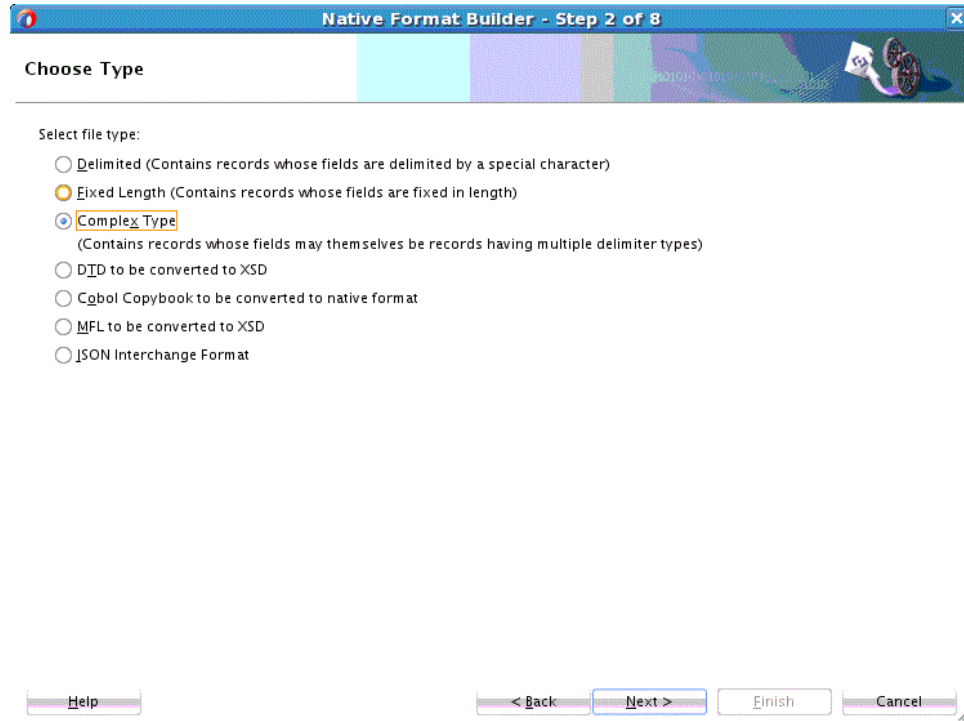
Figure 4-26 Native Format Builder Wizard Choose Type Page
