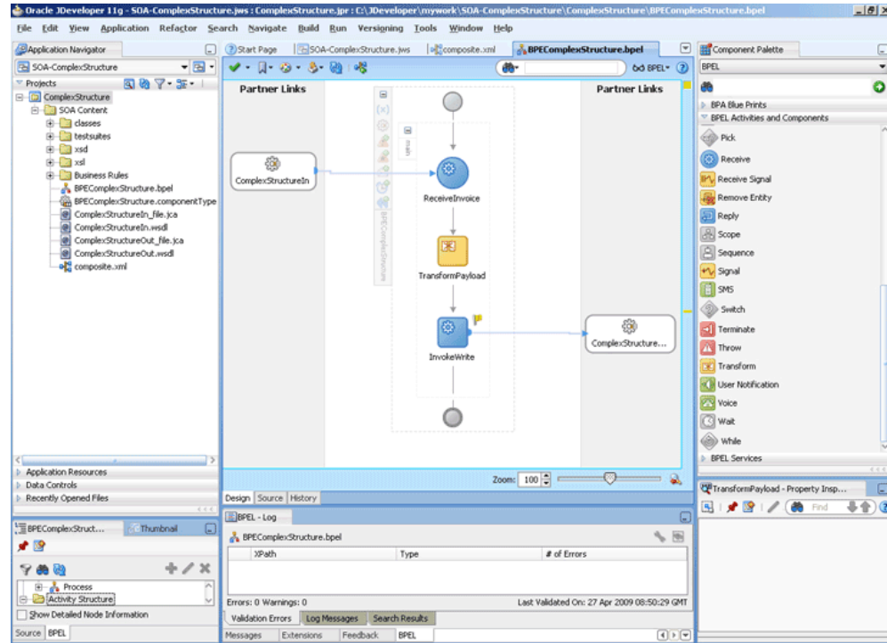
Figure 5-154 The JDeveloper - BPELComplexStructure.bpel
