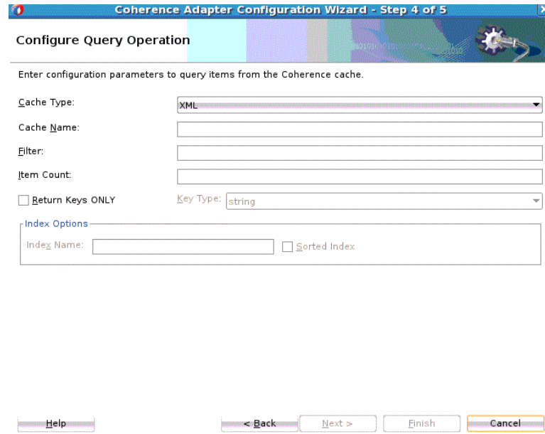
Figure 14-6 The Coherence Adapter Configure Query Operation Screen
