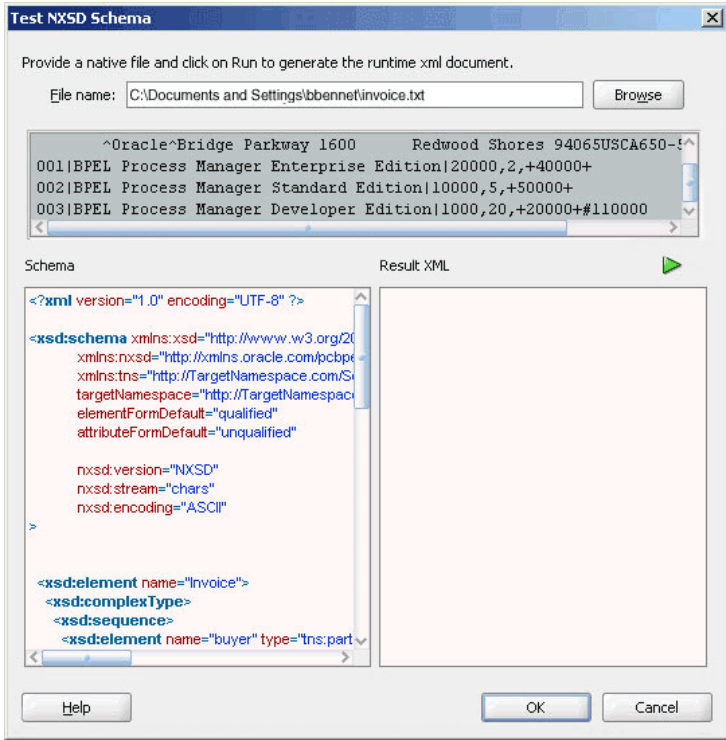
Figure 4-44 Test NXSD Schema Dialog
