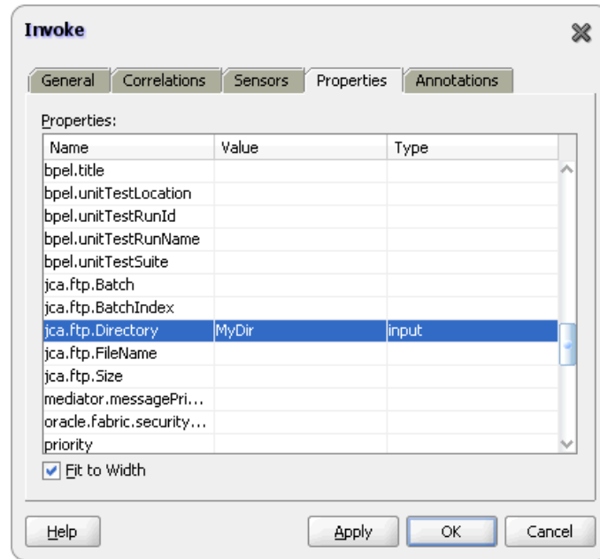
Figure 5-34 The Invoke Dialog
