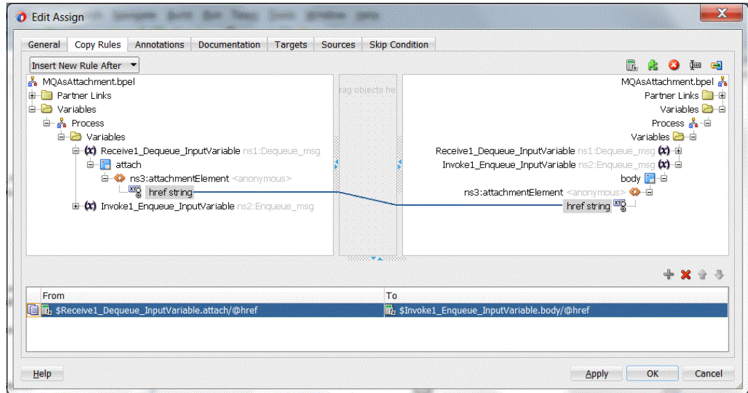
Figure 10-109 The Assign Activity Dialog
