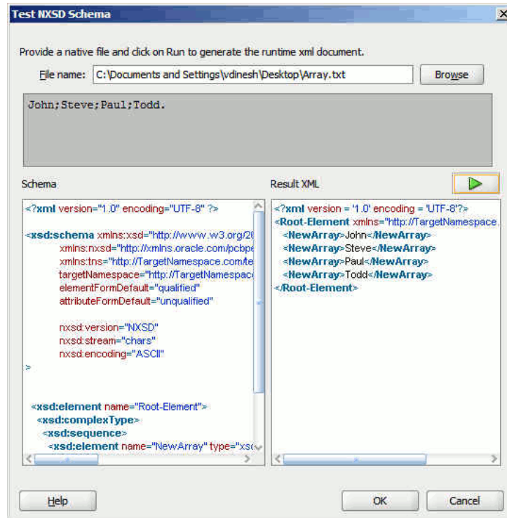
Figure 4-62 Test NXSD Schema Dialog
