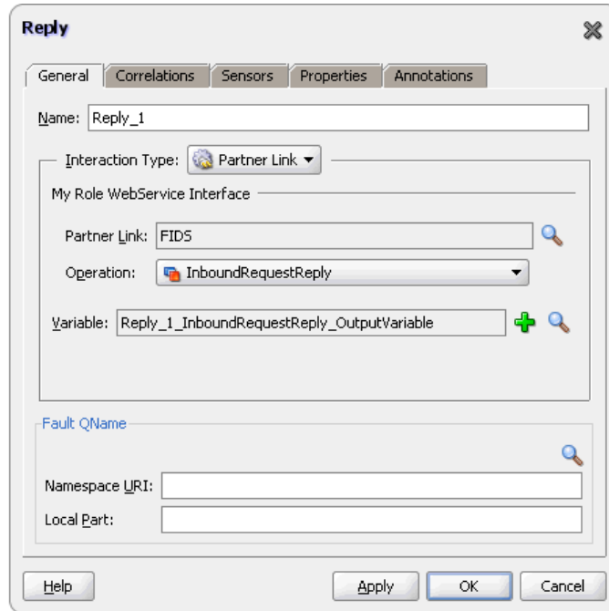
Figure 6-86 The Reply Dialog
