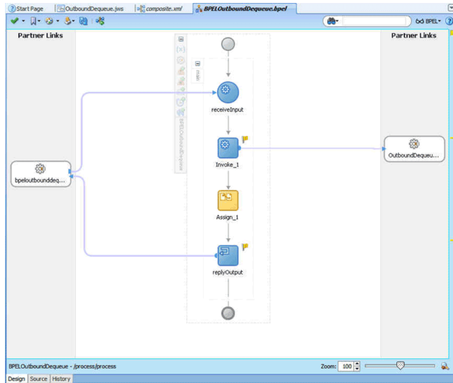
Figure 10-90 The BPELOutboundDequeue.bpel Page
