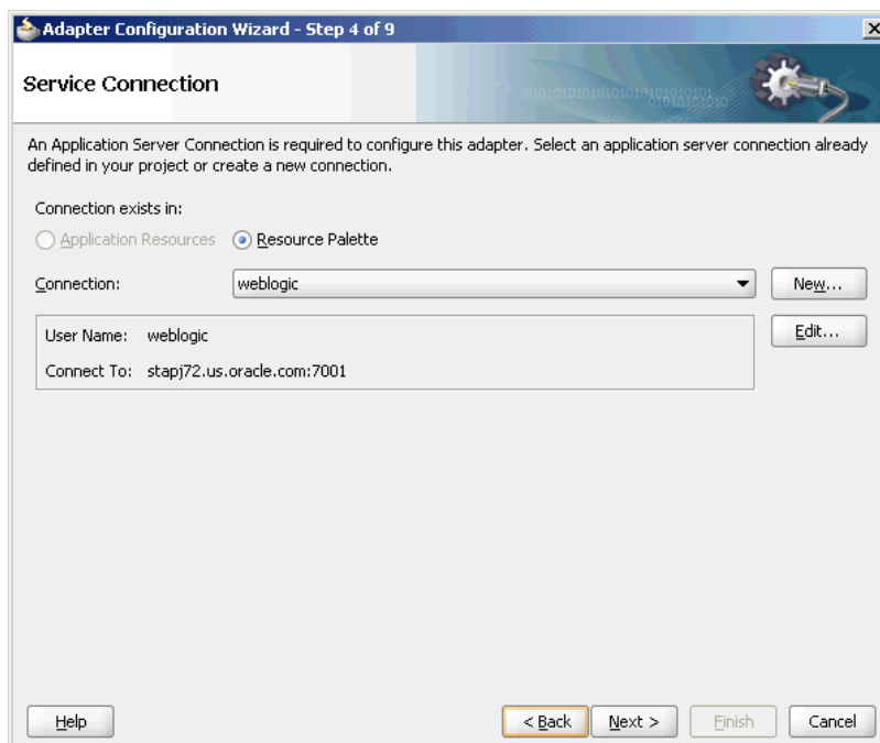
Figure 8-15 The Adapter Configuration Wizard Service Connection Page
