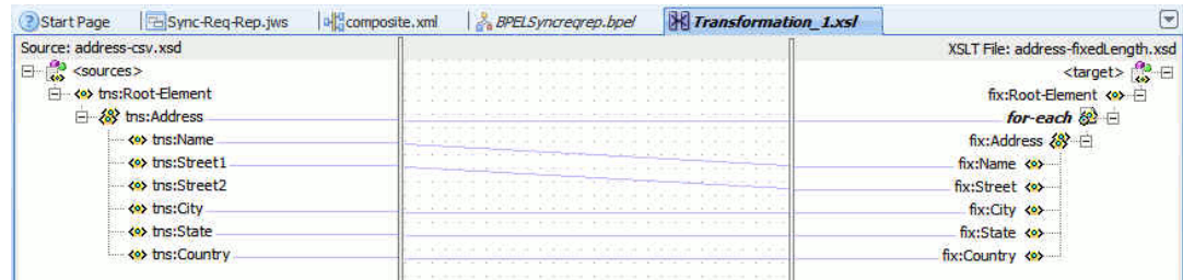
Figure 10-72 The Transformation.xsl Page with Mappings
