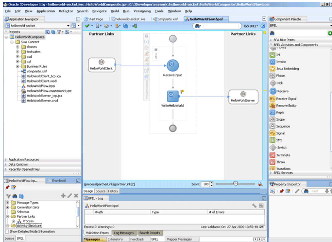
Figure 6-62 The JDeveloper - HelloWorldFlow.bpel
