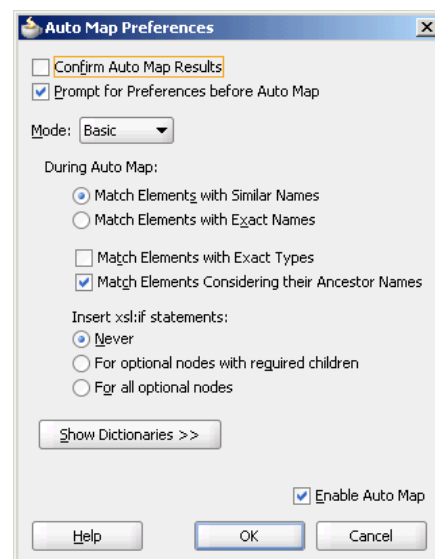
Figure 7-40 The Auto Map Preferences Dialog
