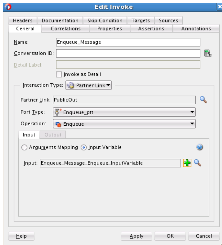
Figure 13-12 Edit Invoke Dialog
