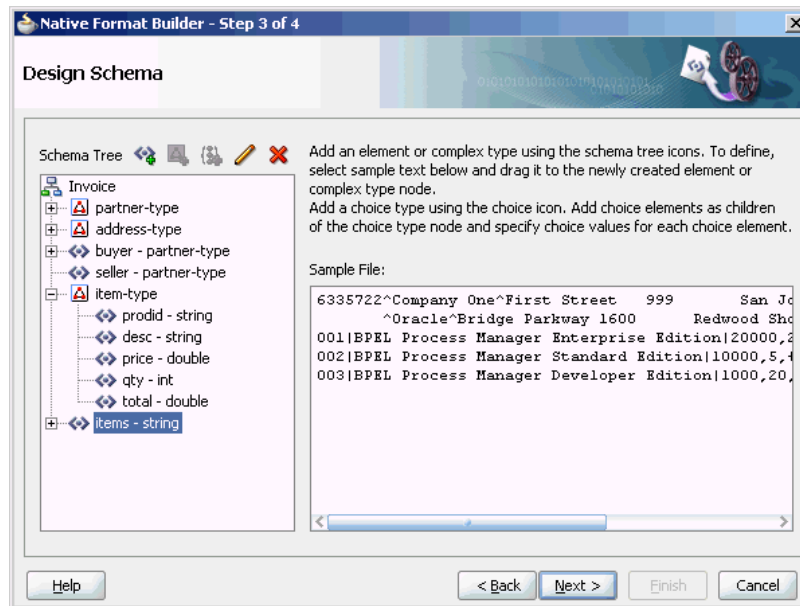
Figure 4-39 Native Format Builder Wizard Design Schema Page
