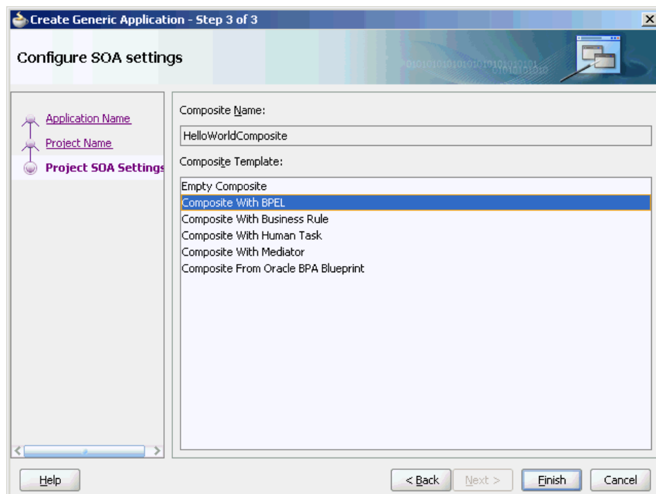
Figure 6-41 The Configure SOA Settings Dialog
