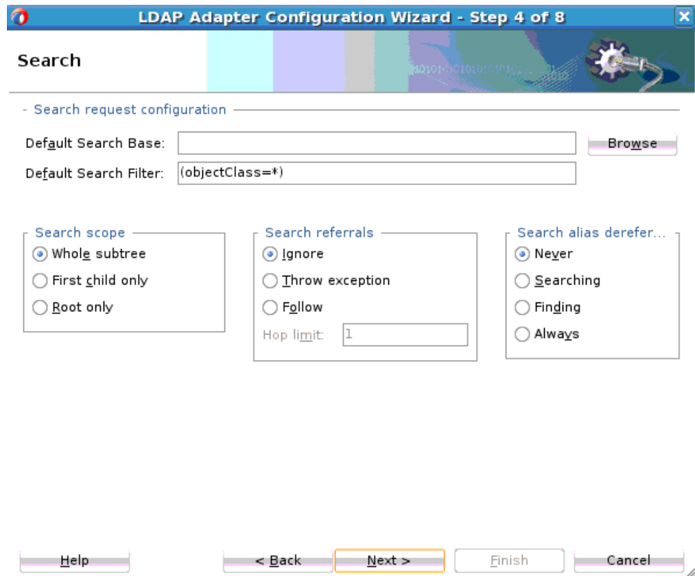
Figure 12-18 The LDAP Adapter Configuration Search Configuration Wizard Search Request Configuration Page
