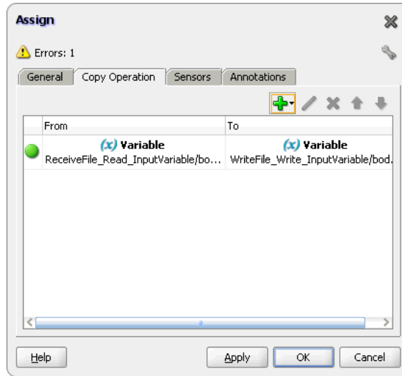
Figure 5-106 The Assign Dialog
