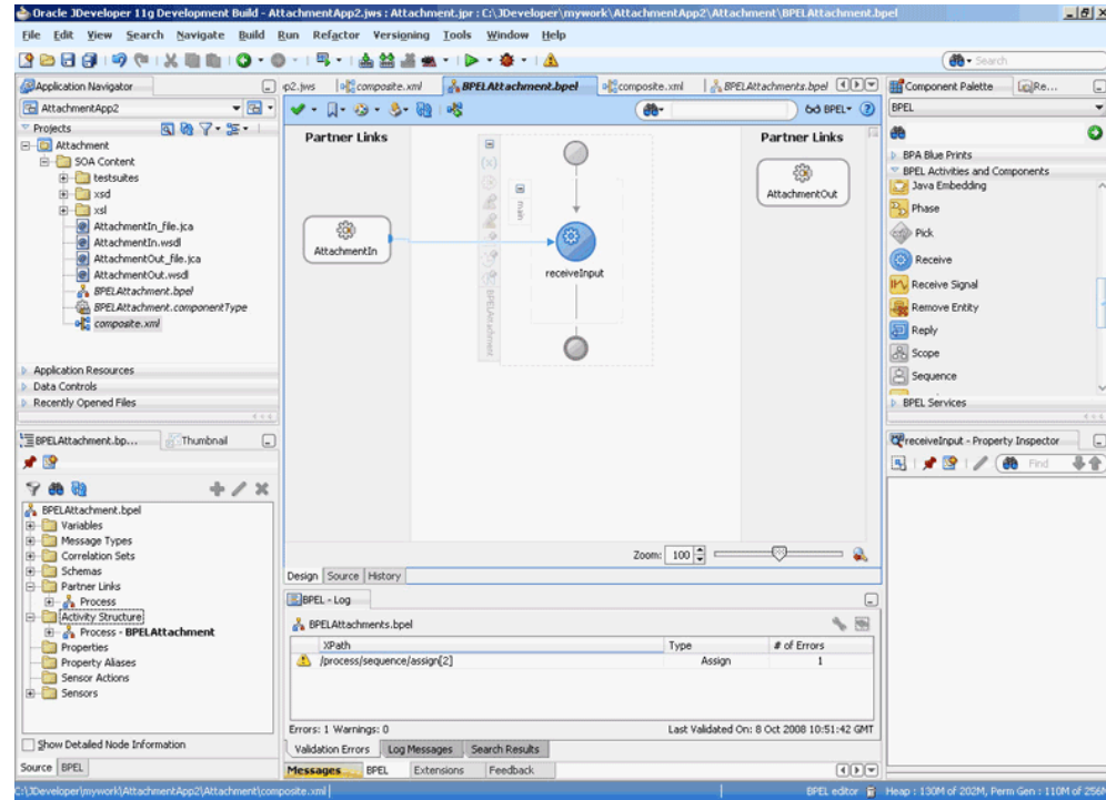
Figure 5-133 The JDeveloper - BPELXMLDebatching.bpel
