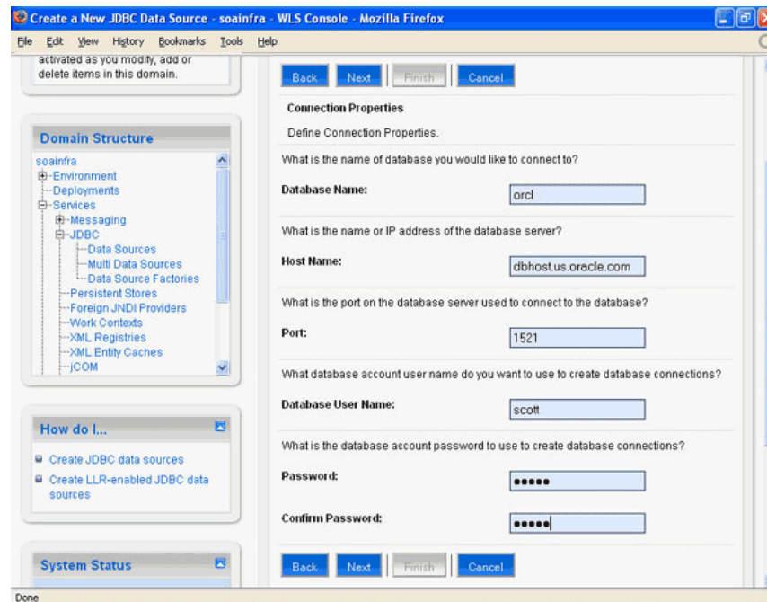
Figure 7-46 The Create a New JDBC Data Source Connection Properties Page
