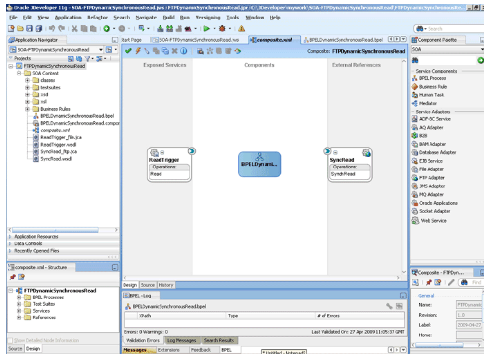
Figure 5-166 The JDeveloper - Composite.xml
