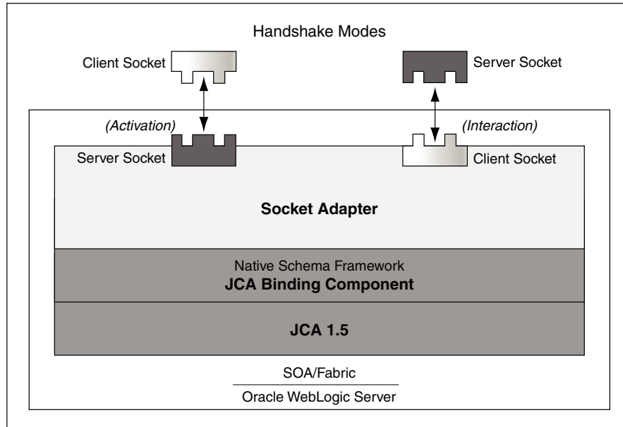
Figure 6-1 Oracle Socket Adapter Architecture
