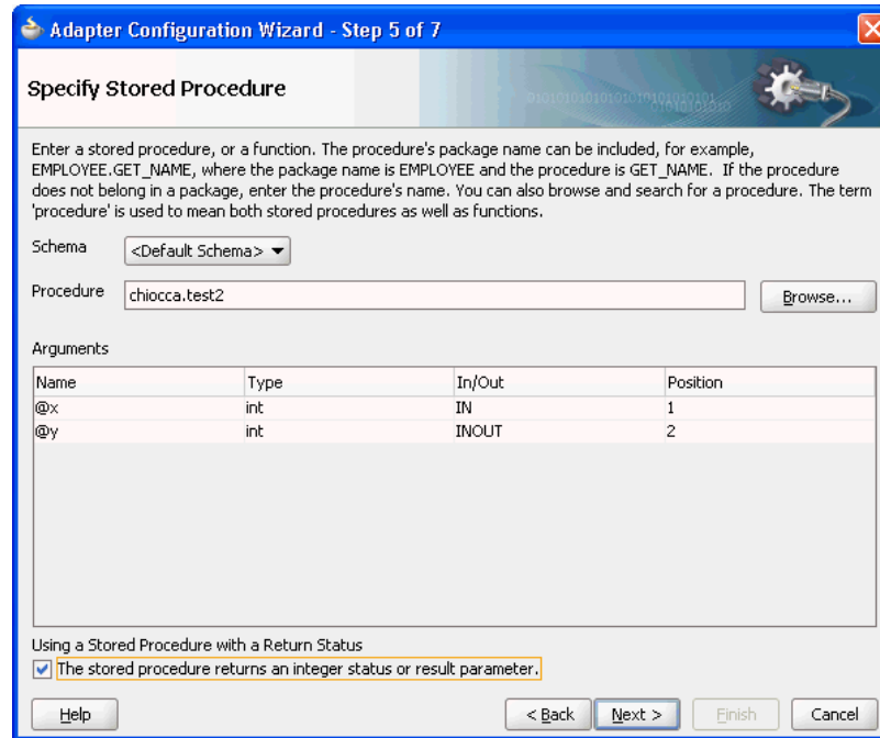
Figure 9-50 The Specify Stored Procedure Page
