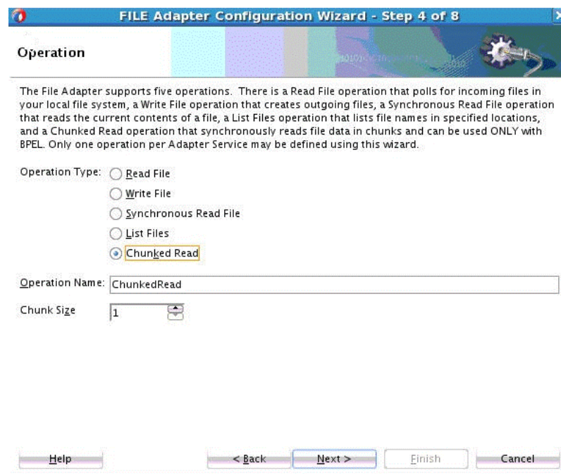
Figure 5-2 File Adapter Configuration Wizard Operation Page with Chunked Read Selected
