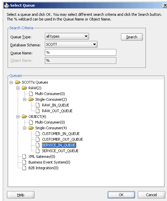
Figure 7-13 The Select Queue Dialog
