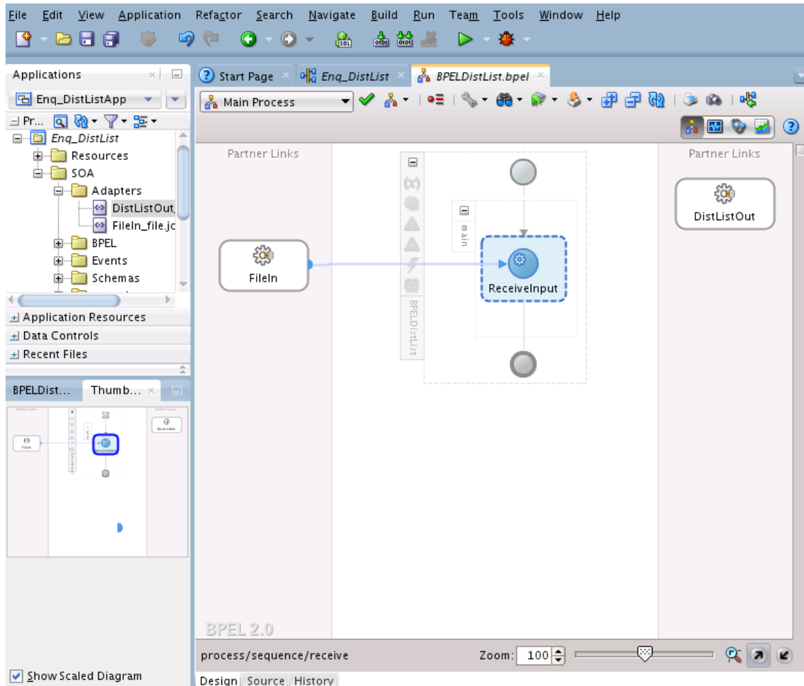
Figure 13-37 JDeveloper BPELDistList.bpel Page Showing the FileIn Partner Link Wired to the Receive Activity
