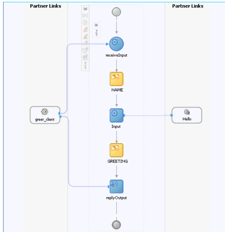
Figure 9-63 The Final BPEL Process Screen
