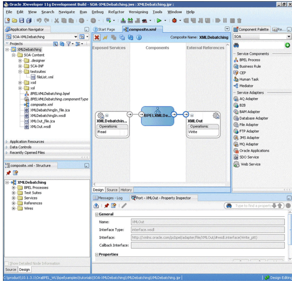
Figure 5-73 The JDeveloper - Composite.xml
