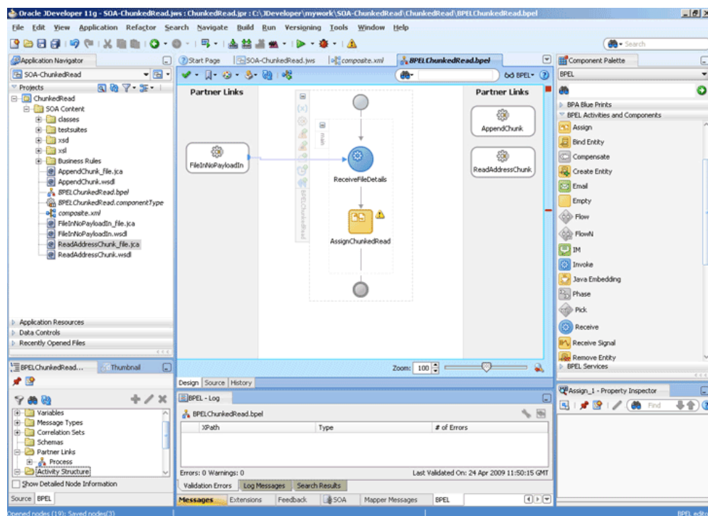
Figure 5-117 The JDeveloper - BPELChunkedRead.bpel
