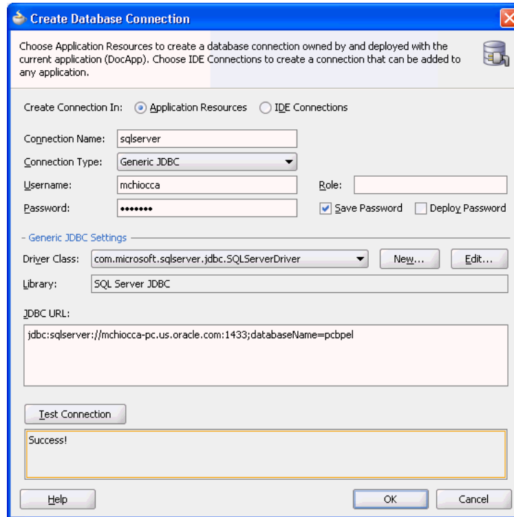
Figure 9-49 The Create Database Connection Dialog
