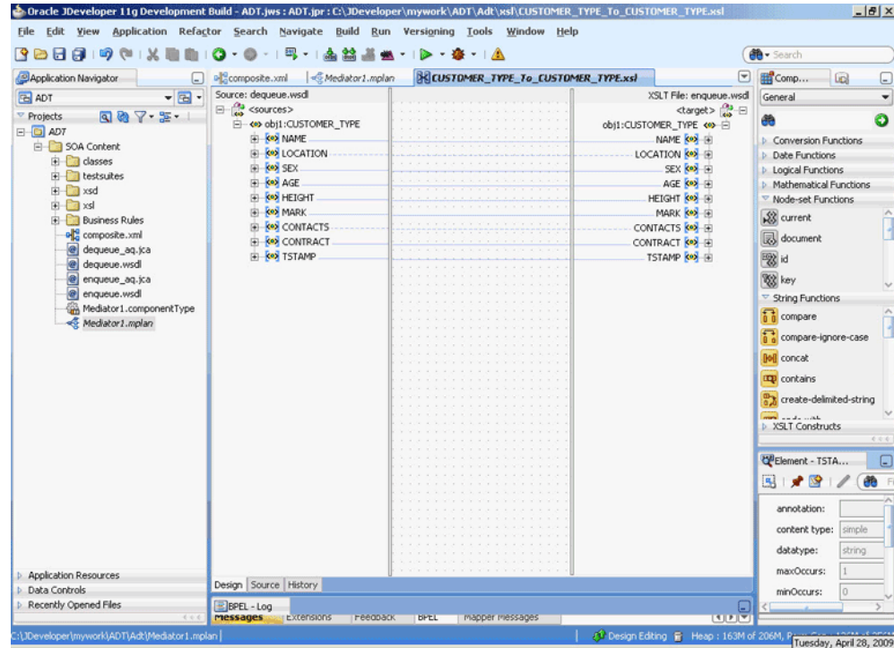
Figure 7-41 The Application Window After Setting the Map Preferences
