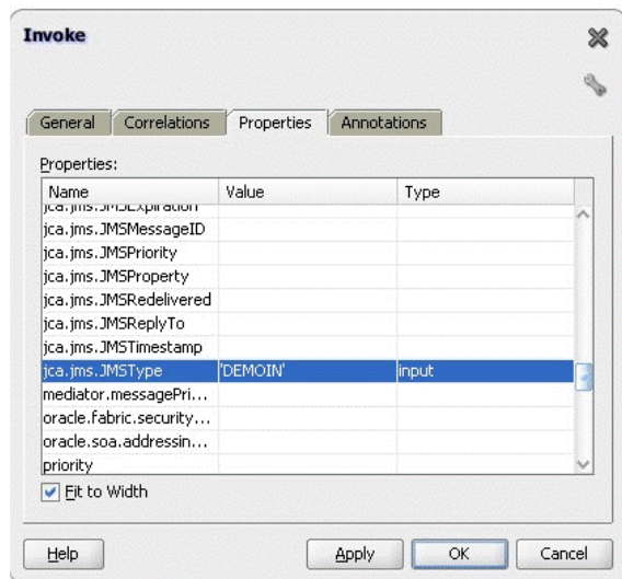
Figure 8-30 Invoke BPEL Properties Dialog Corresponding to the JMS Adapter Link
