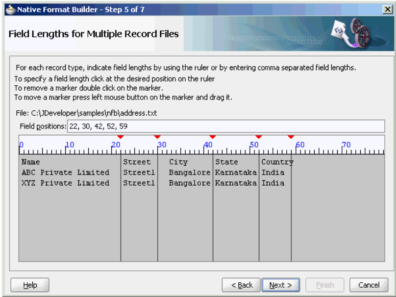
Figure 4-21 Native Format Builder Wizard Field Lengths for Multiple Record Files Page
