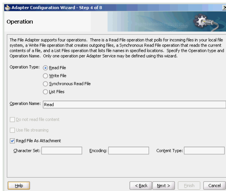
Figure 5-126 The Adapter Configuration Wizard Operation Page
