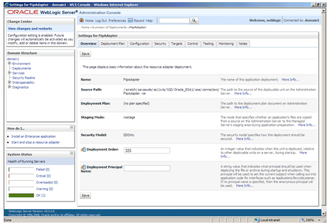
Figure 5-16 The Oracle WebLogic Server Administration Console - Settings for FTPAdapter Page
