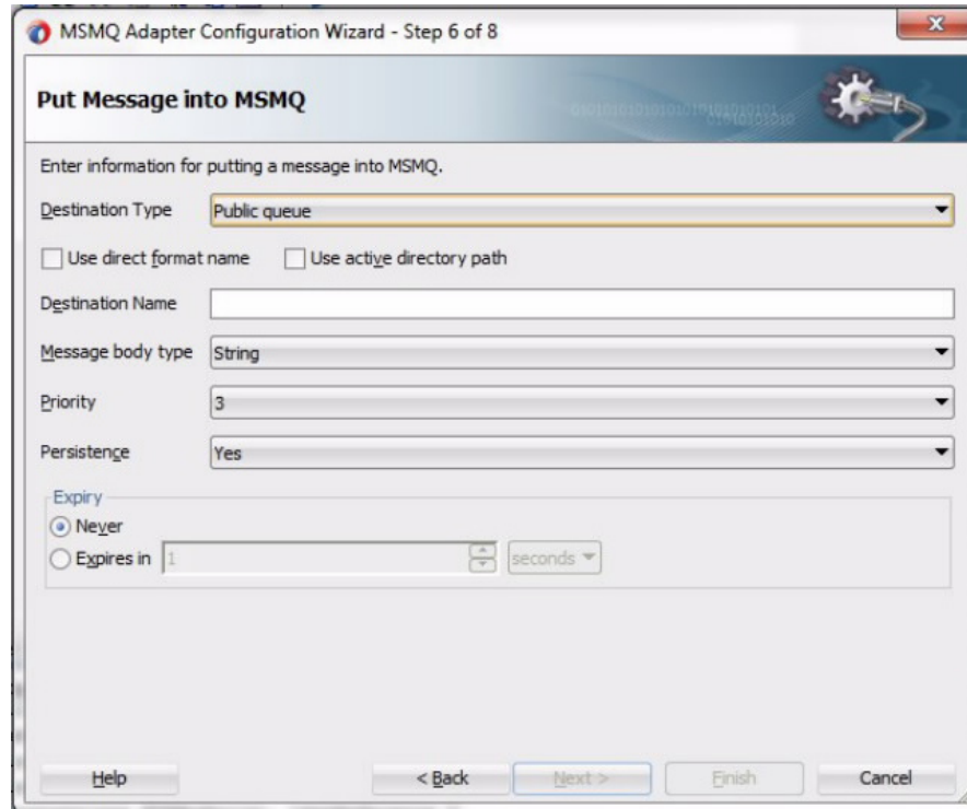
Figure 13-3 Enqueue Operation
