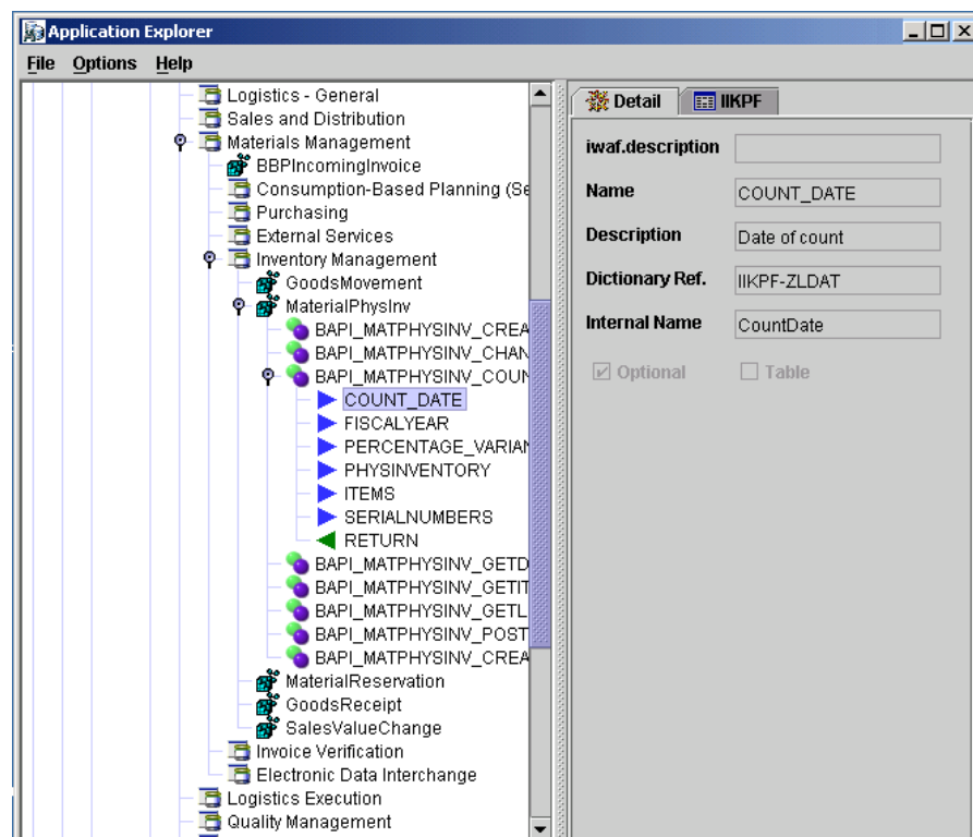
Figure 1-12 Application Explorer
