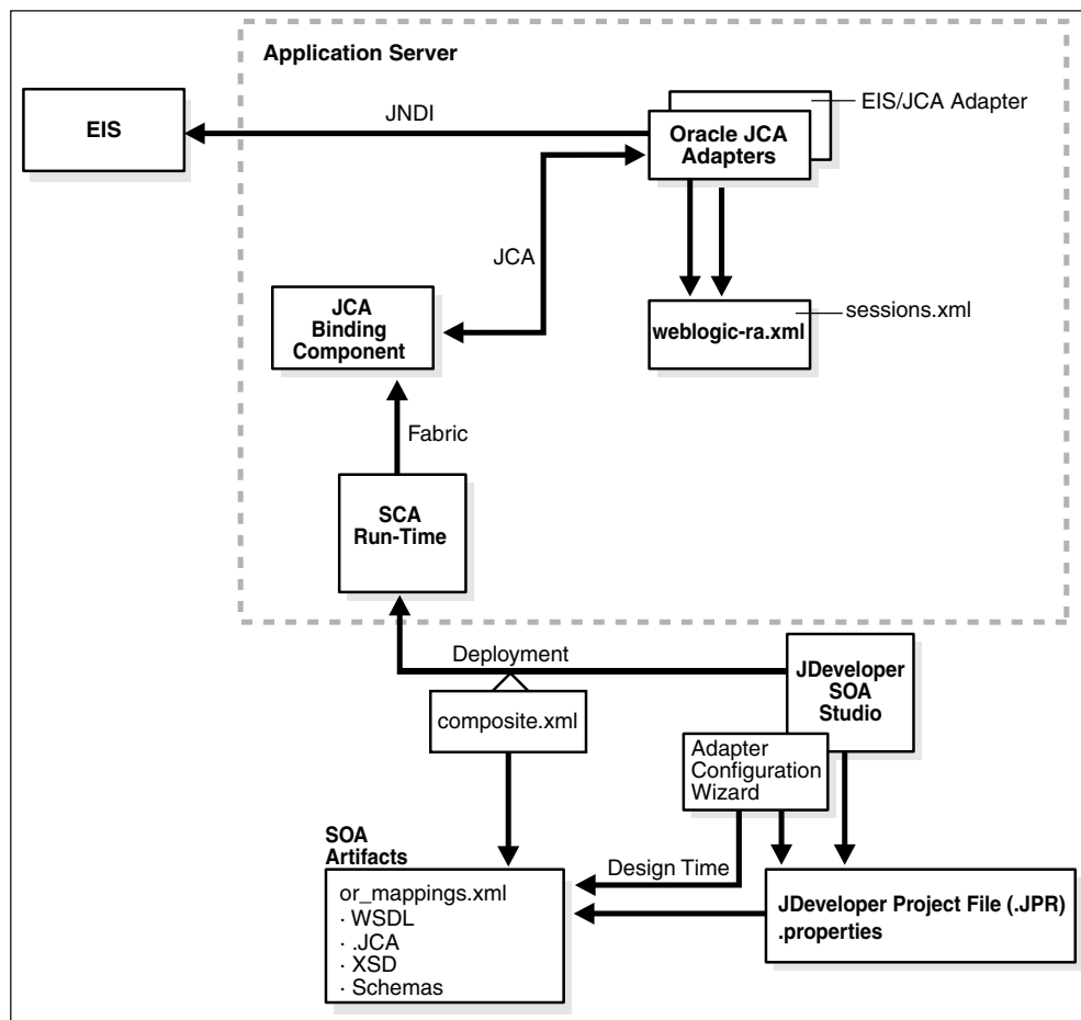
Figure 3-2 Oracle Adapter Architecture in Oracle Fusion Middleware
