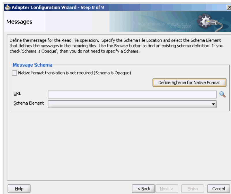
Figure 4-4 Starting the Native Format Builder Wizard
