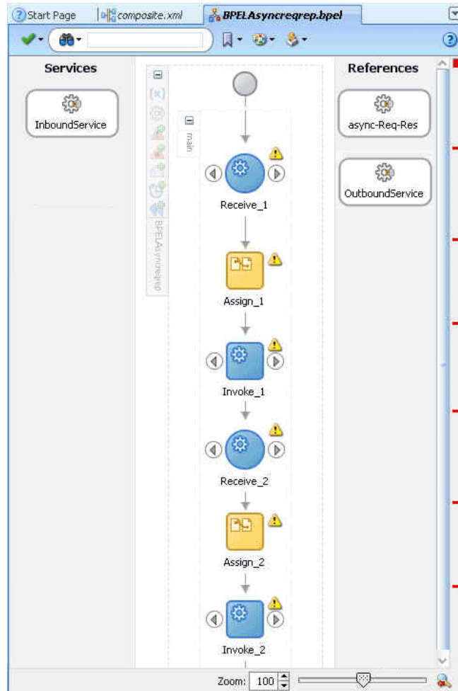
Figure 10-81 The BPELAsyncreqrep.bpel Page
