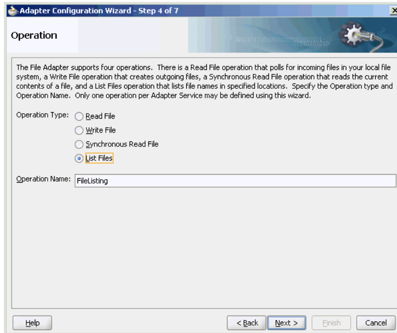
Figure 5-39 List Files Operation Page
