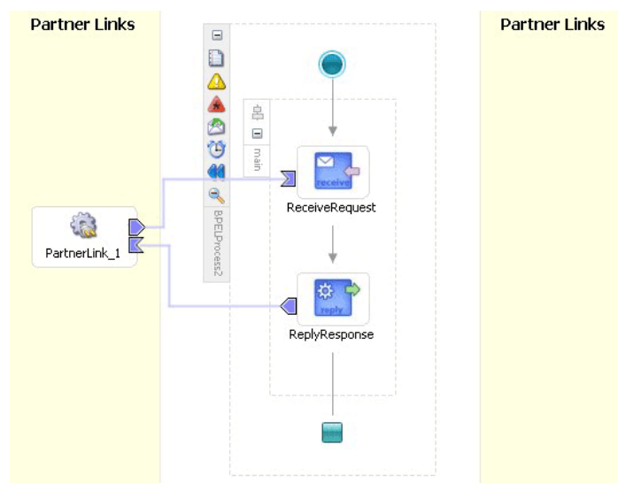
Figure 6-2 BPEL Scenario of Inbound Synchronous Request/Response
