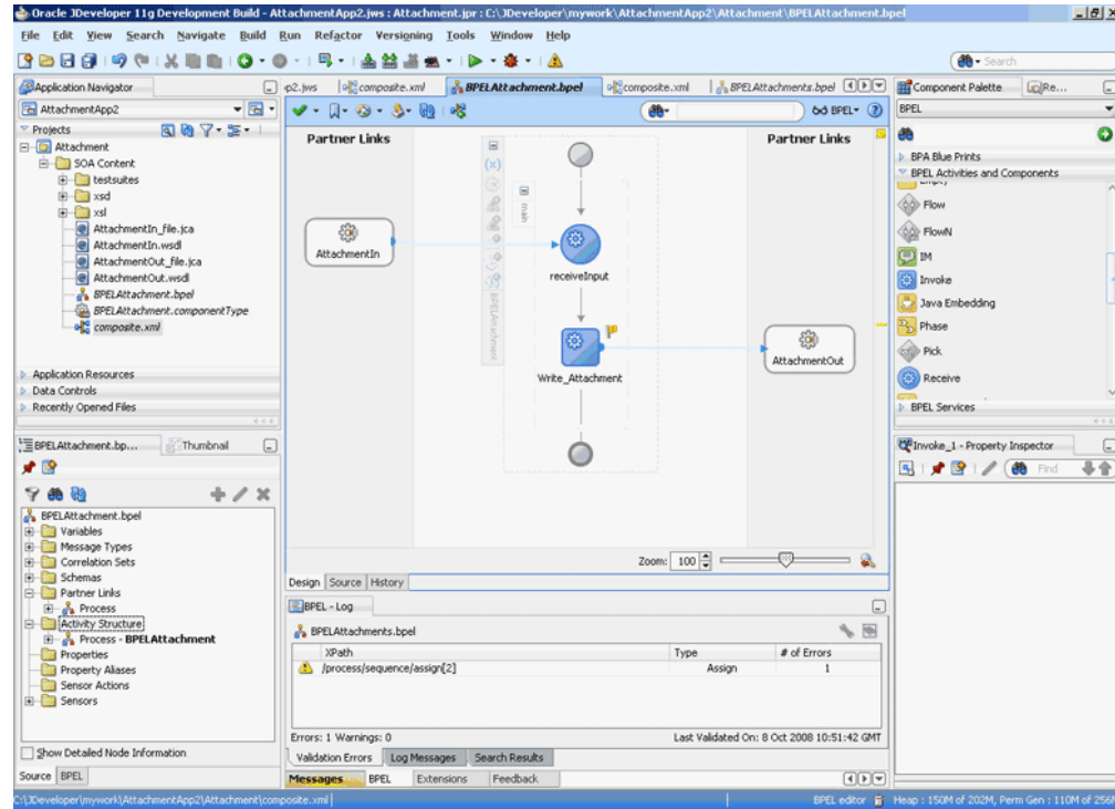
Figure 5-136 The JDeveloper - BPELXMLDebatching.bpel
