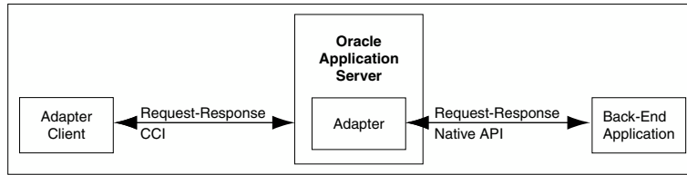
Figure 1-16 Request-Response Service
