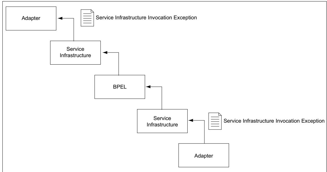
Figure 2-13 Fault Propagation
