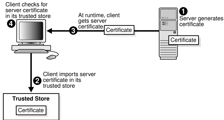
Figure 5-50 Establishing Trust
