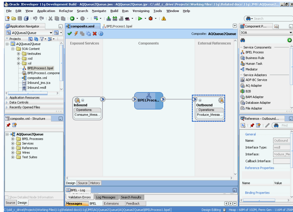
Figure 8-24 JDeveloper - Composite.xml
