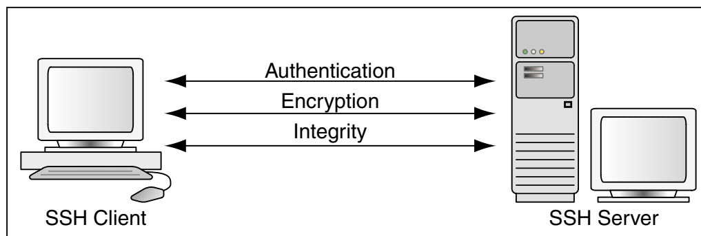
Figure 5-52 SFTP Communication
