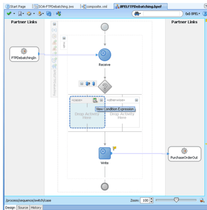
Figure 5-161 BPELFTPDebatching.bpel Page
