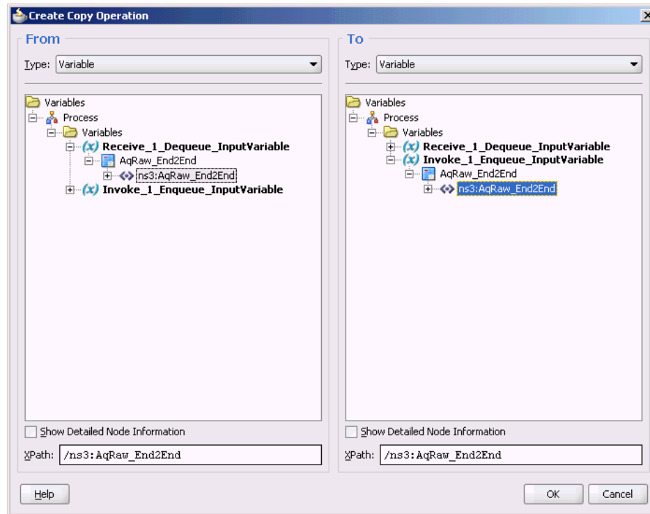
Figure 7-61 The Create Copy Operation Dialog
