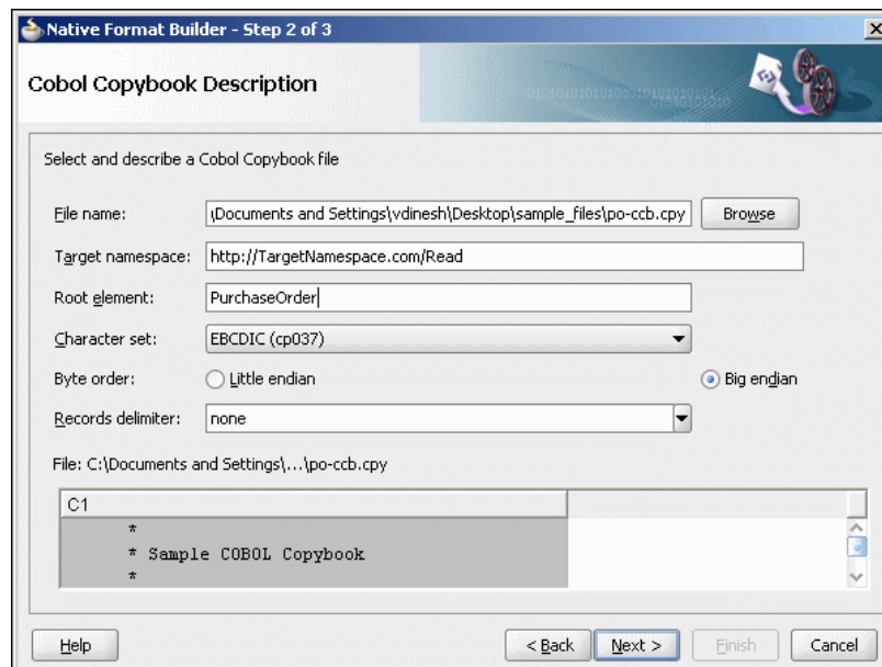
Figure 4-67 Native Format Builder Wizard File Description Page
