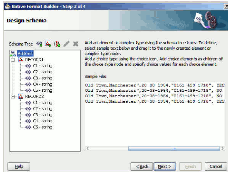
Figure 4-53 Native Format Builder Design Schema Page
