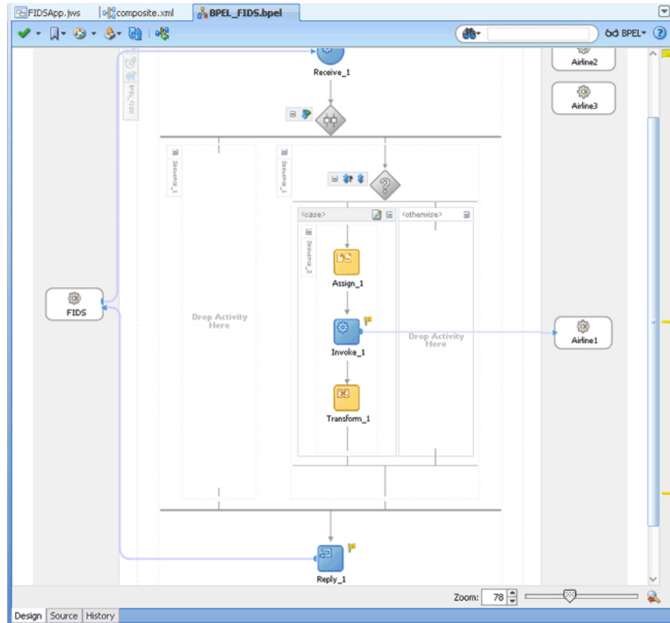
Figure 6-96 The JDeveloper - BPEL_FIDS.bpel
