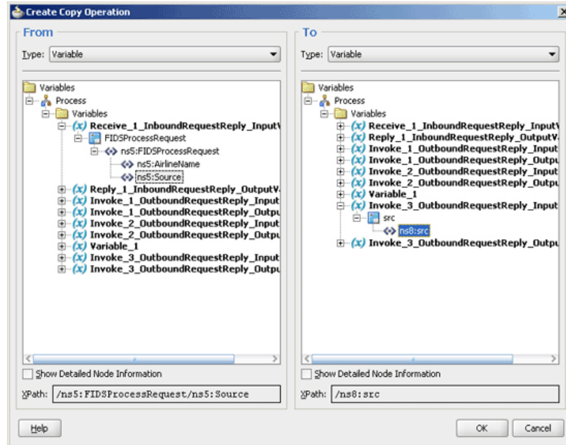
Figure 6-103 The Create Copy Operation Dialog
