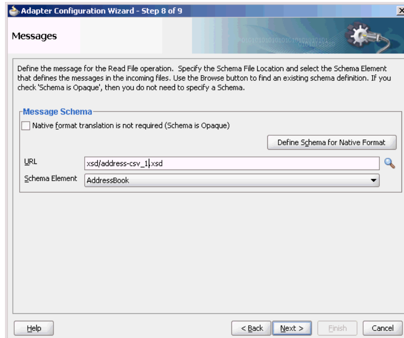
Figure 4-16 Adapter Configuration Wizard Messages Page
