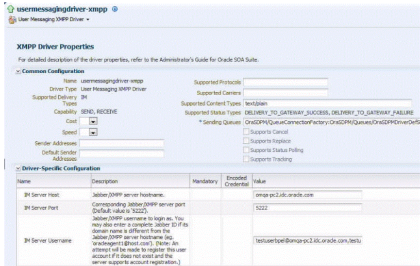
Figure 11-4 Configuring the User Messaging XMPP Driver
