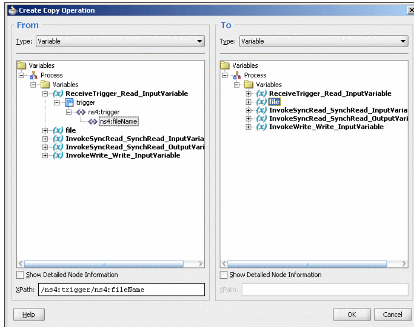
Figure 5-171 The Create Copy Operation Dialog
