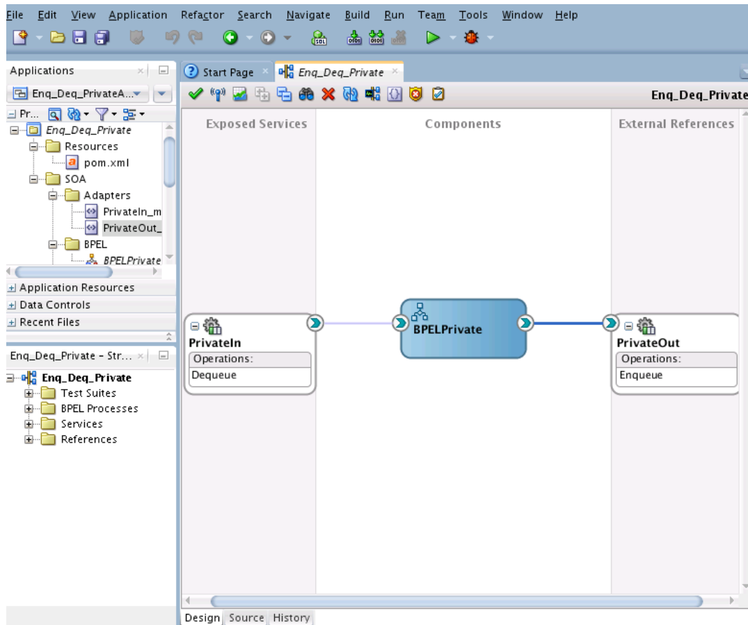
Figure 13-21 The MSMQ Adapter JDeveloper composite.xml Wired
