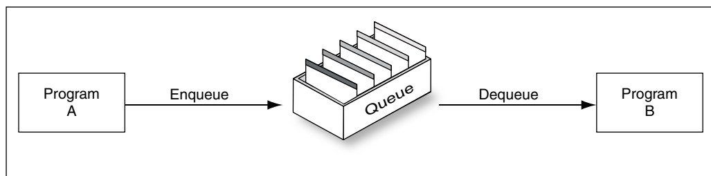
Figure 10-1 Enqueue/Dequeue
