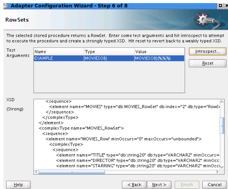
Figure 9-51 RowSets Page
