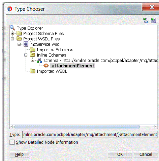
Figure 10-105 Selecting attachmentElement
