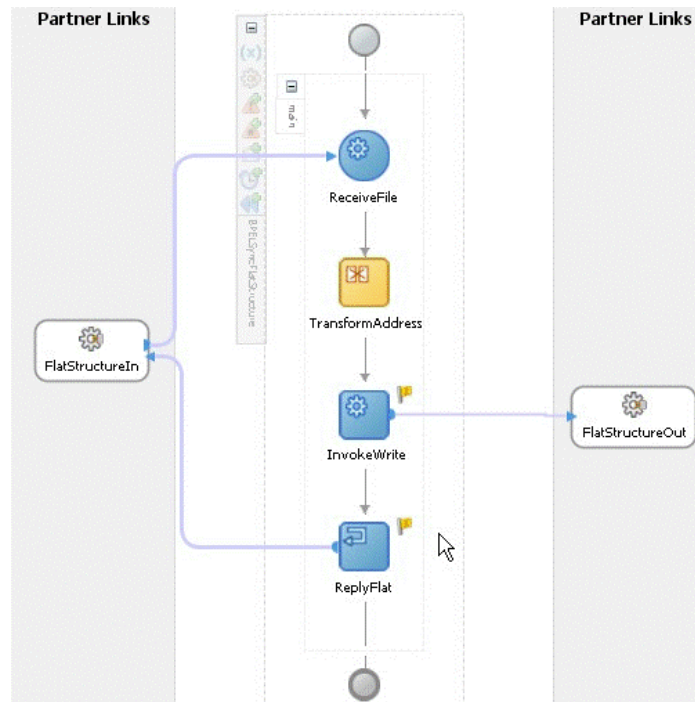
Figure 5-180 The Synchronous File Adapter Process with Receive and Reply BPEL Activities
