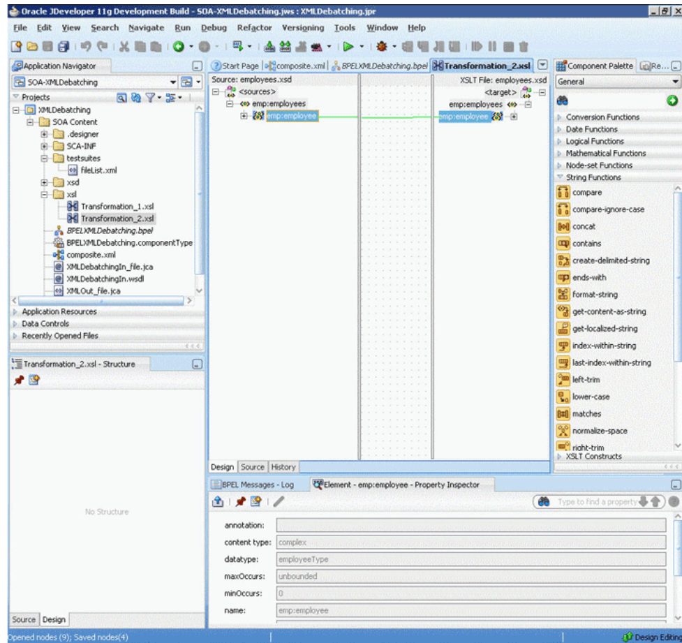
Figure 5-85 The JDeveloper - Transformation_2.xsl
