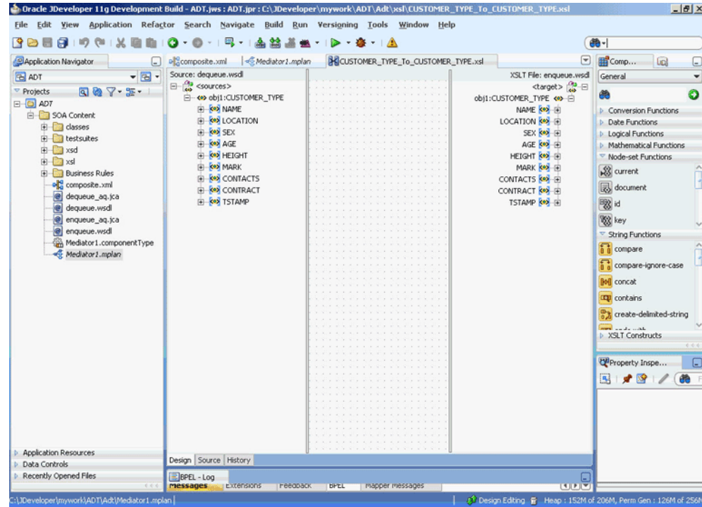
Figure 7-39 The Transformation Window
