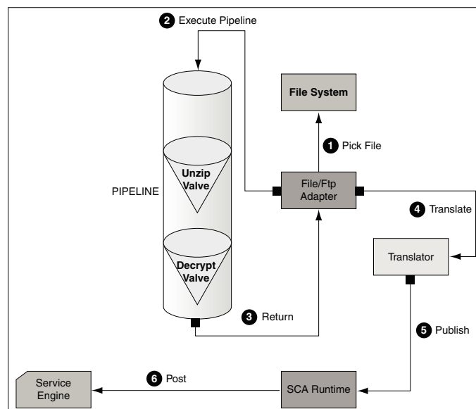
Figure 5-9 A Sample Pre-Processing Pipeline
