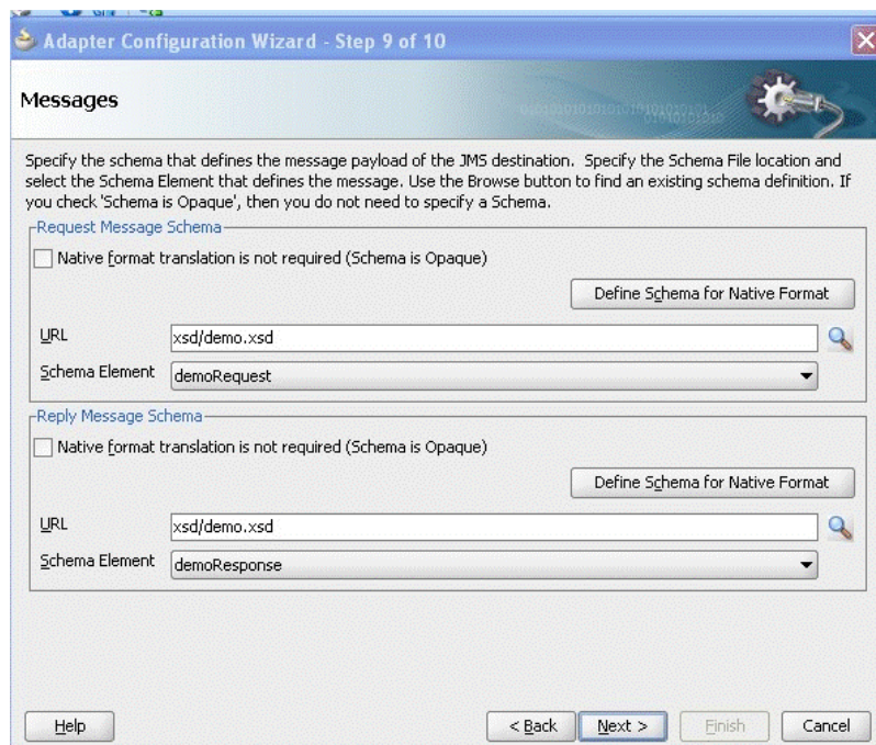
Figure 8-29 Selecting Message Schema for Request and for Response
