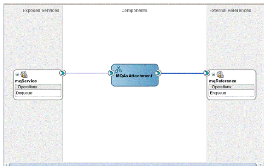
Figure 10-107 The composite.xml with Activities and Services Wired
