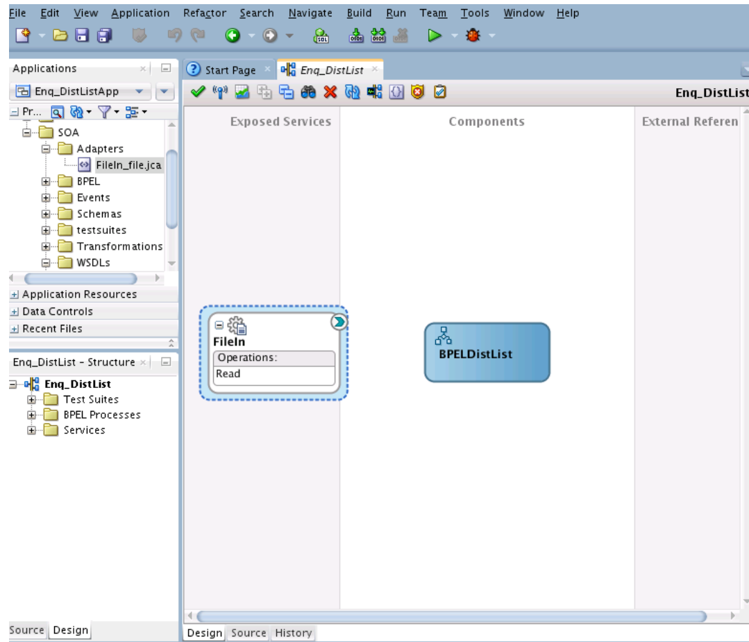
Figure 13-32 The Configured Inbound File Adapter with the composite.xml
