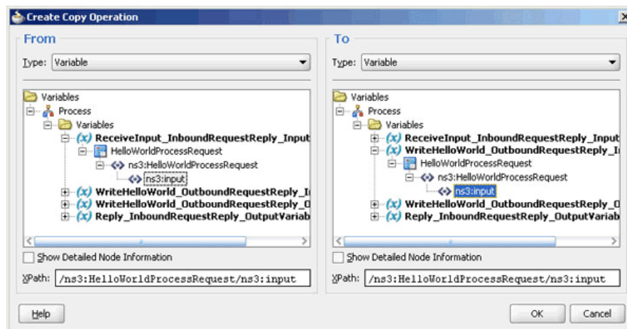
Figure 6-67 The Create Copy Operation Dialog
