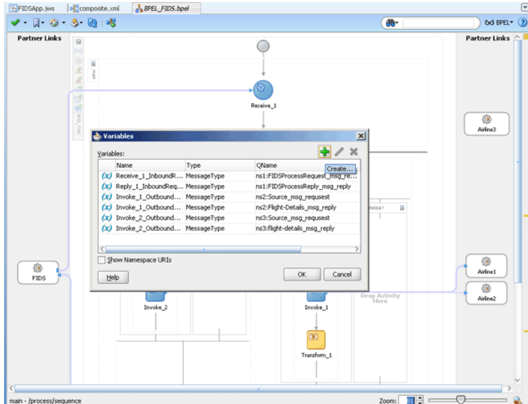
Figure 6-104 The Variables Dialog
