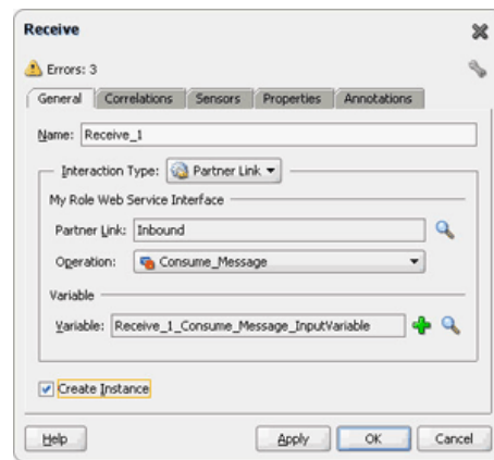
Figure 8-21 The Receive Dialog
