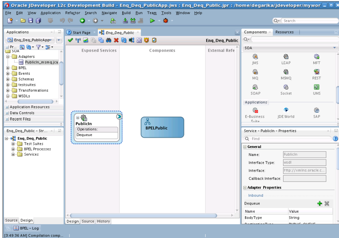
Figure 13-6 The composite.xml for the Enqueue-Dequeue from Public Queue Use Case
