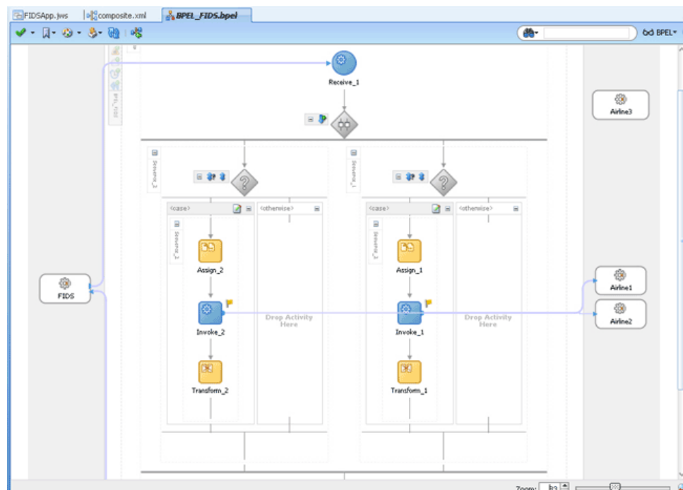
Figure 6-102 The JDeveloper - BPEL_FIDS.bpel
