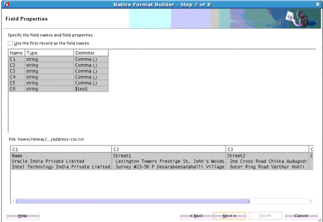
Figure 4-11 Native Format Builder Wizard Field Properties Page
