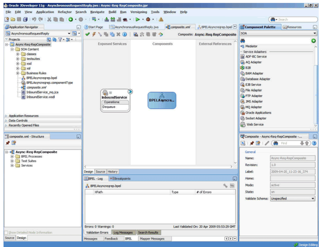
Figure 10-76 The JDeveloper Page - Composite.xml Page
