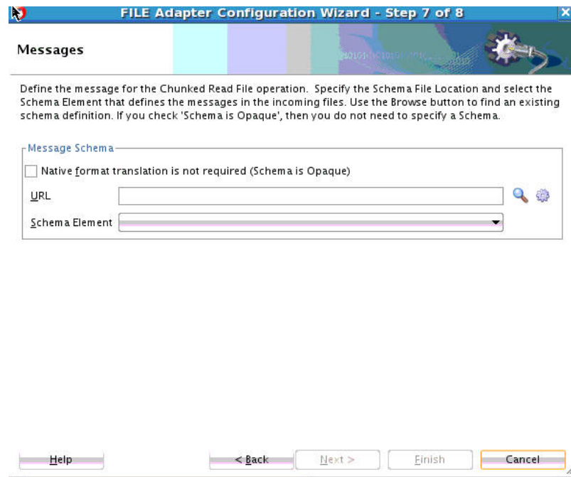
Figure 5-5 File Adapter Configuration Wizard Messages Screen
