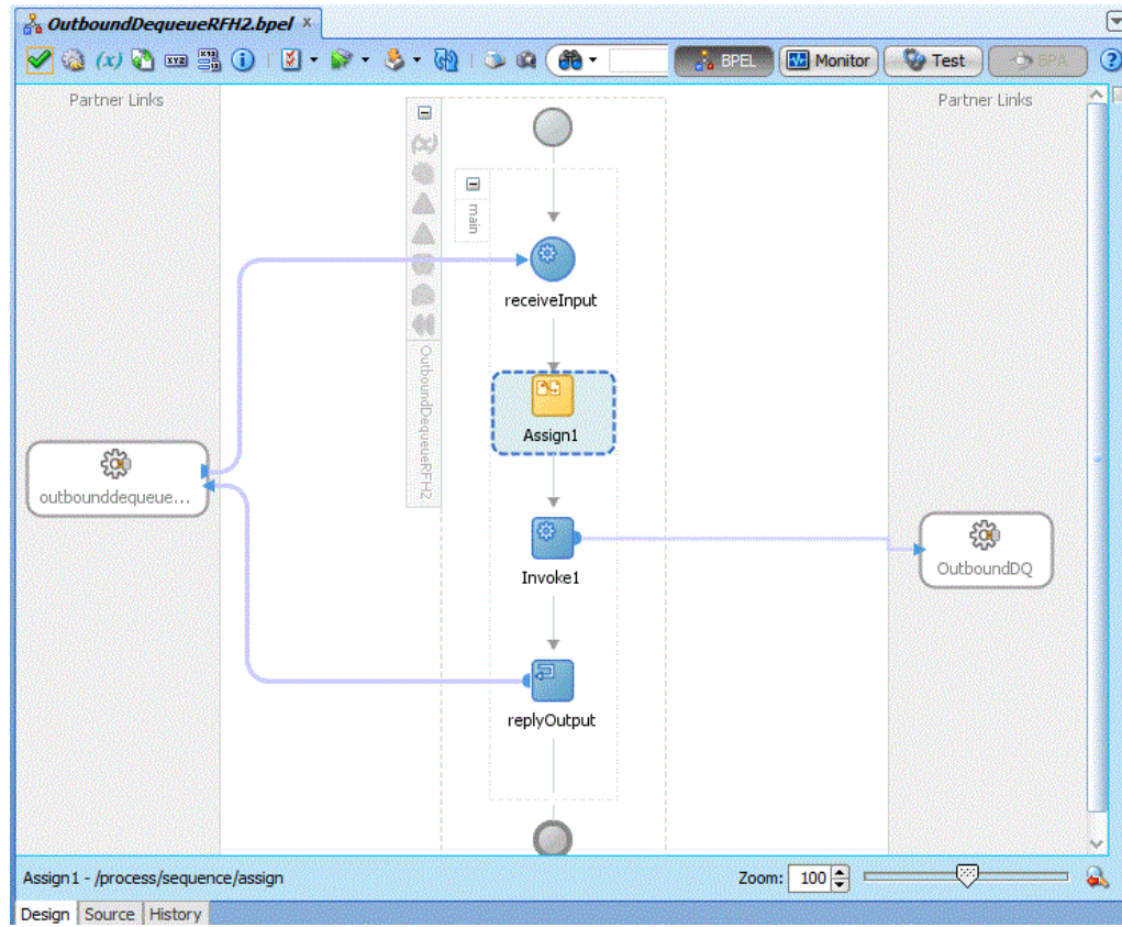
Figure 10-103 The JDeveloper BPELOutboundDequeue.bpel page
