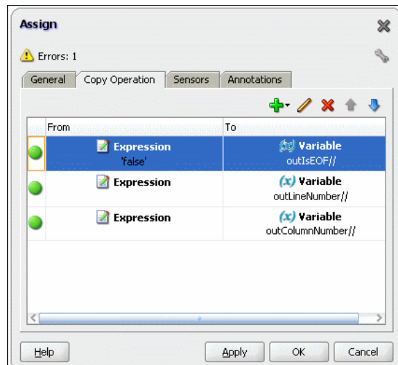
Figure 5-116 The Assign Dialog
