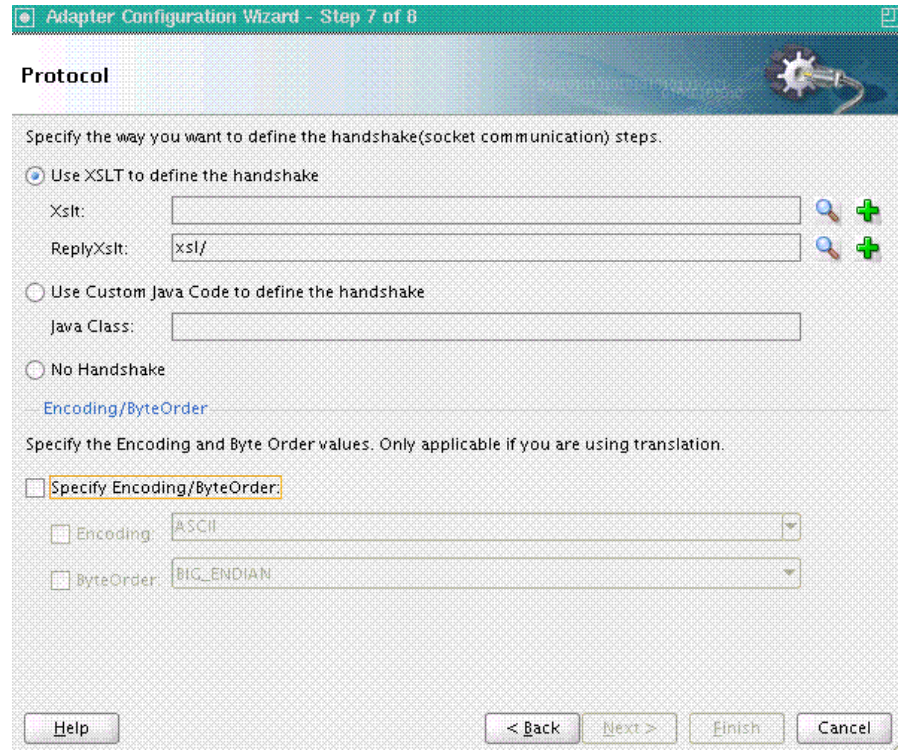
Figure 6-17 The Adapter Configuration Wizard - Protocol Page
