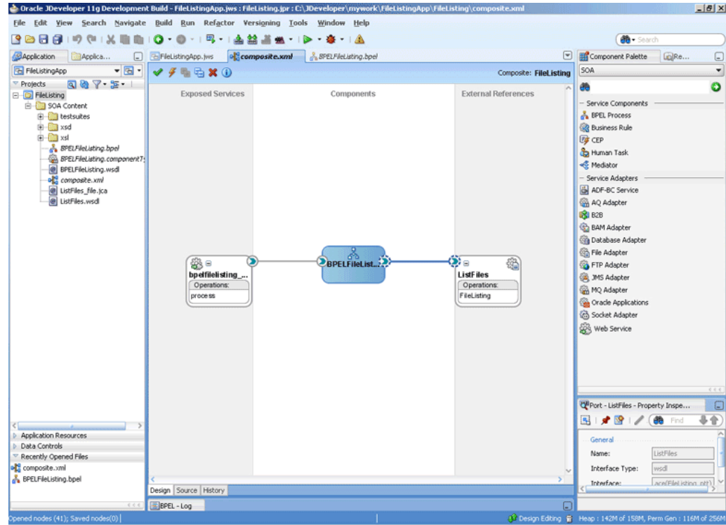
Figure 5-143 The JDeveloper - Composite.xml
