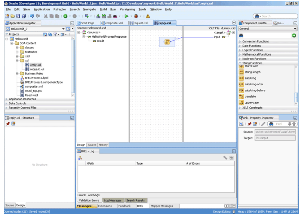
Figure 6-25 The JDeveloper - reply.xsl Page
