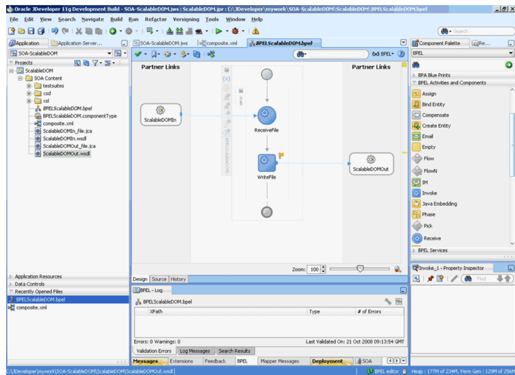
Figure 5-103 The JDeveloper - BPELScalableDOM.bpel Page
