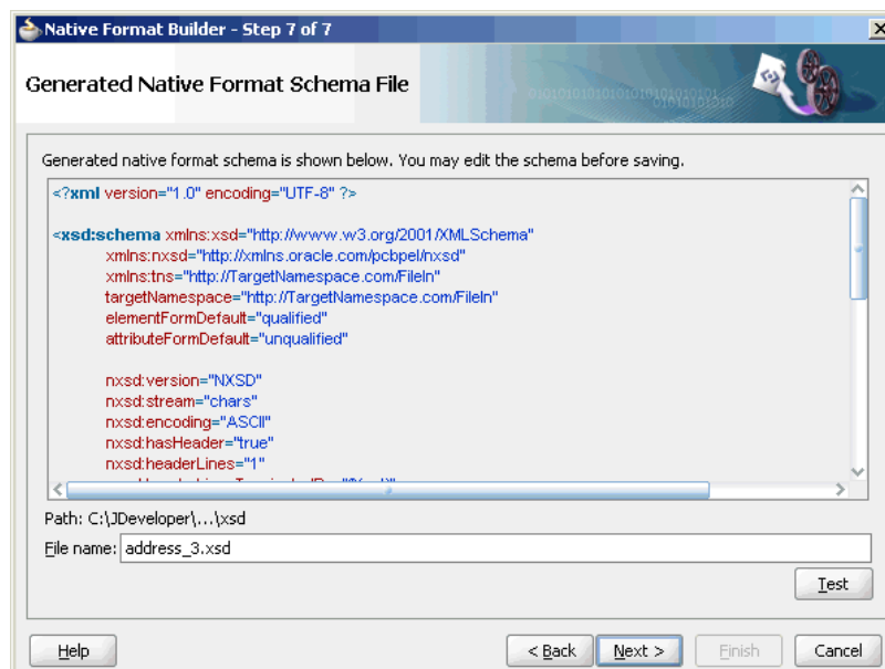
Figure 4-23 Native Format Builder Wizard Native Format Schema File Page
