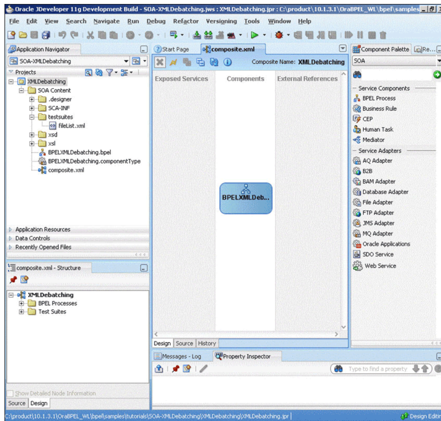
Figure 5-63 The JDeveloper - composite.xml Page
