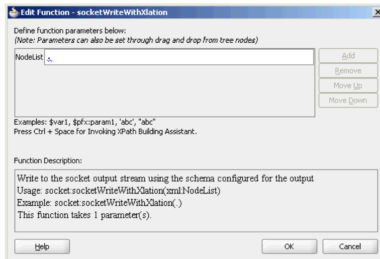
Figure 6-31 The Edit Function - socketWriteWithXlation Dialog
