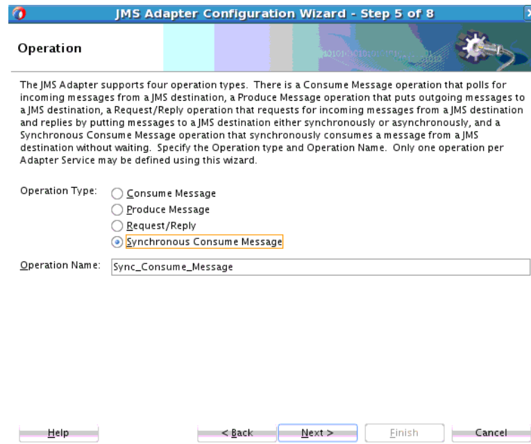
Figure 8-32 JMS Adapter Configuration Wizard Operation Screen, with Synchronous Consume Message Selected
