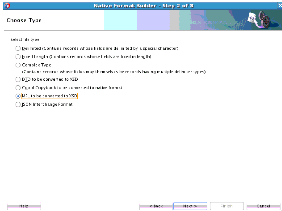
Figure 4-75 Native Format Builder Choose Type Screen with MFL to be Converted to XSD Selected
