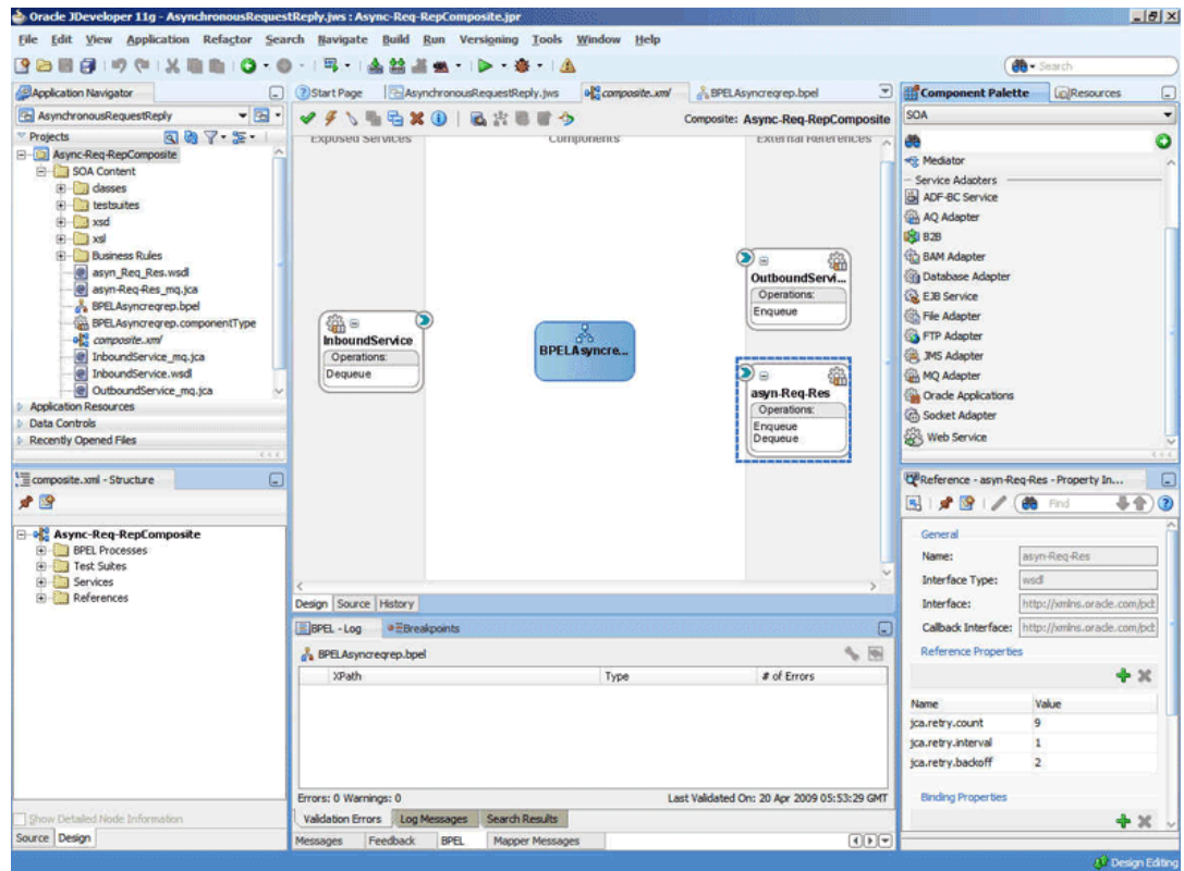
Figure 10-79 The JDeveloper Page - Composite.xml Page
