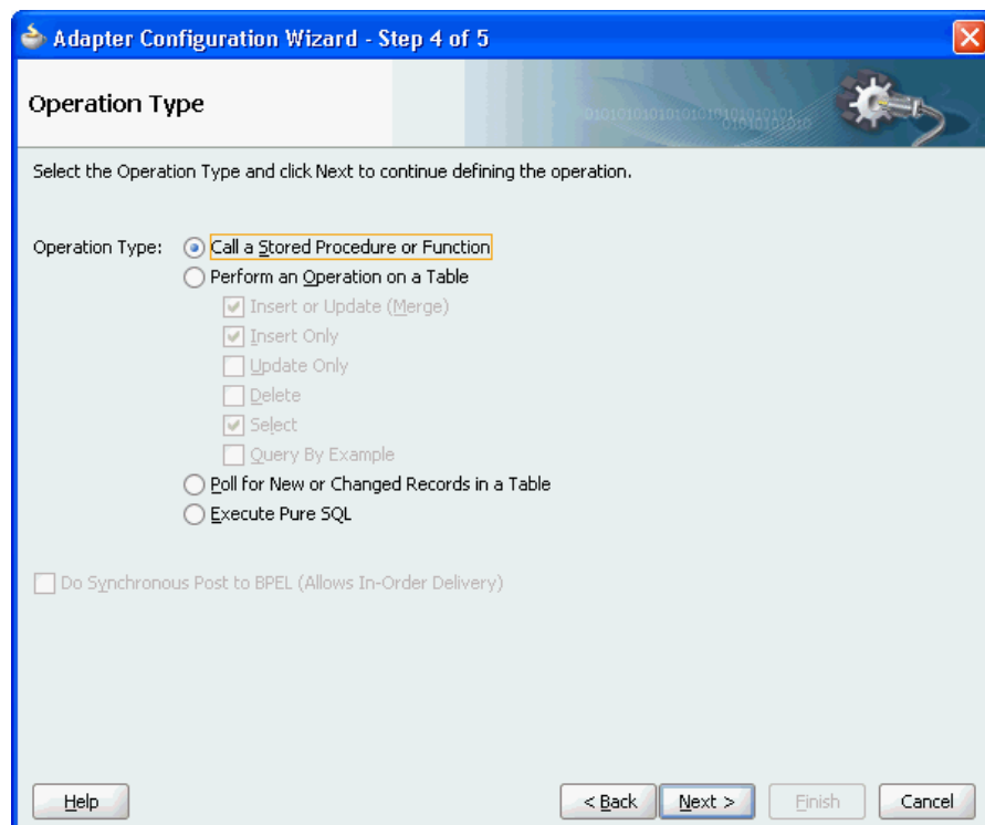
Figure 9-33 Calling a Stored Procedure or Function in the Adapter Configuration Wizard
