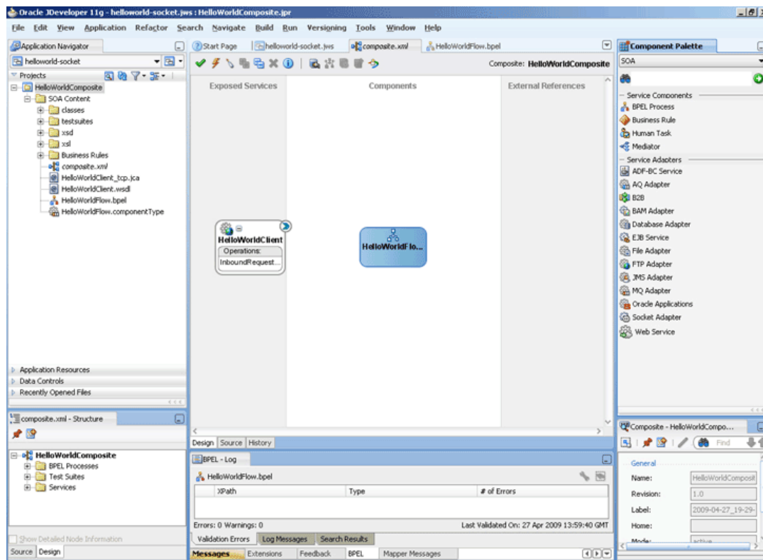
Figure 6-48 The JDeveloper - composite.xml Page
