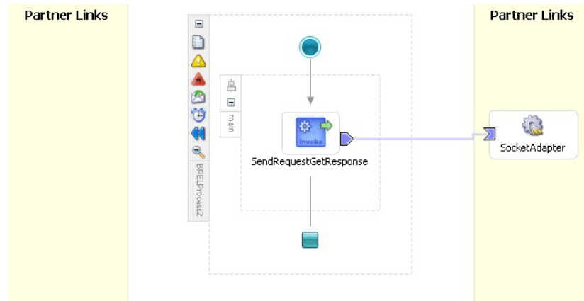
Figure 6-3 BPEL Scenario of Outbound Synchronous Request/Response
