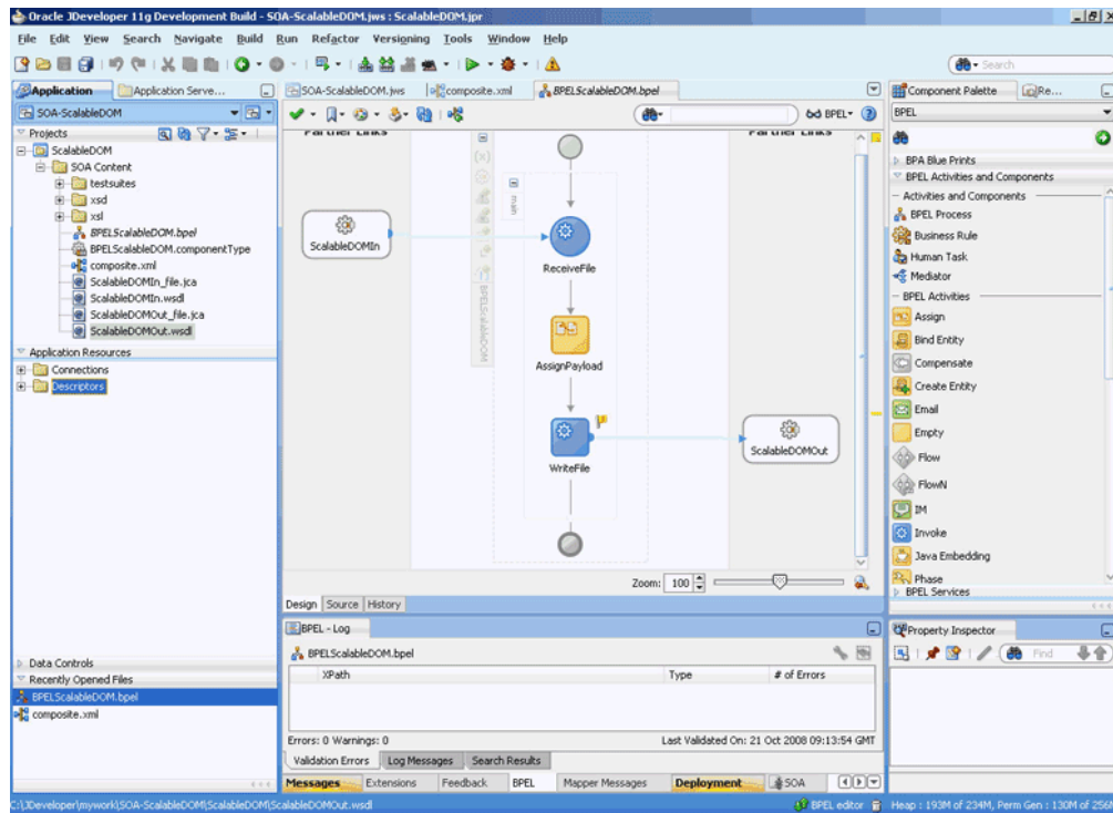
Figure 5-107 The JDeveloper - BPELScalableDOM.bpel
