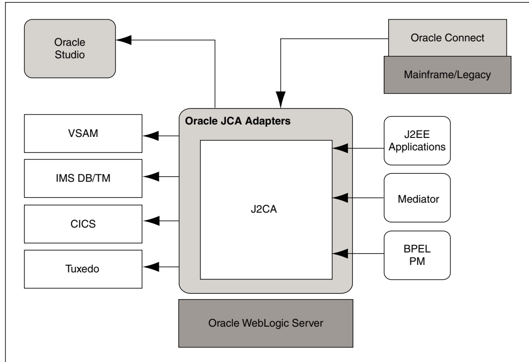
Figure 1-7 Legacy Adapter Architecture
