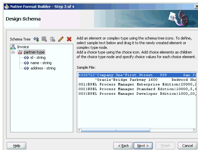
Figure 4-33 Native Format Builder Wizard Design Schema Page - partner-type Complex Type
