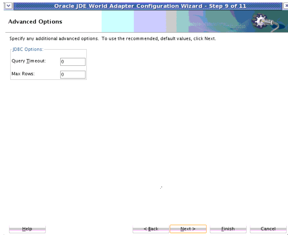
Figure 15-28 The Oracle JDE World Adapter Configuration Wizard Adapter Advanced Options Screen
