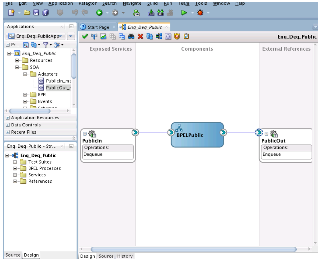
Figure 13-7 Wiring the composite.xml
