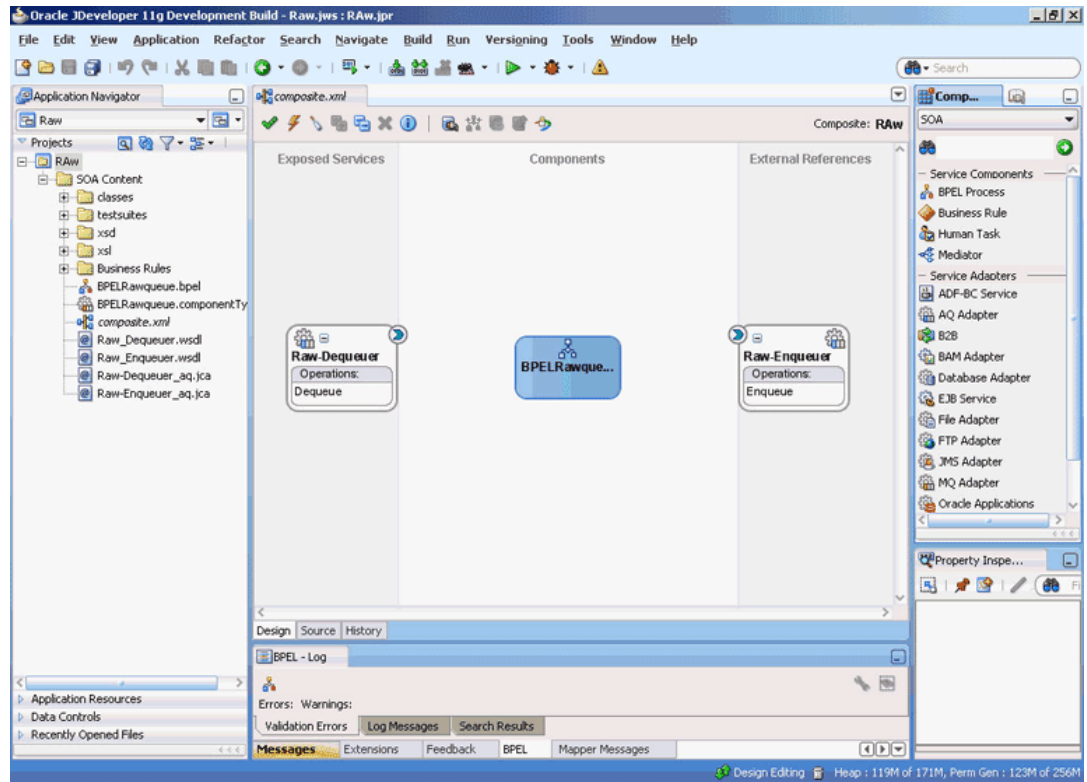
Figure 7-56 The JDeveloper Window Composite.xml Page
