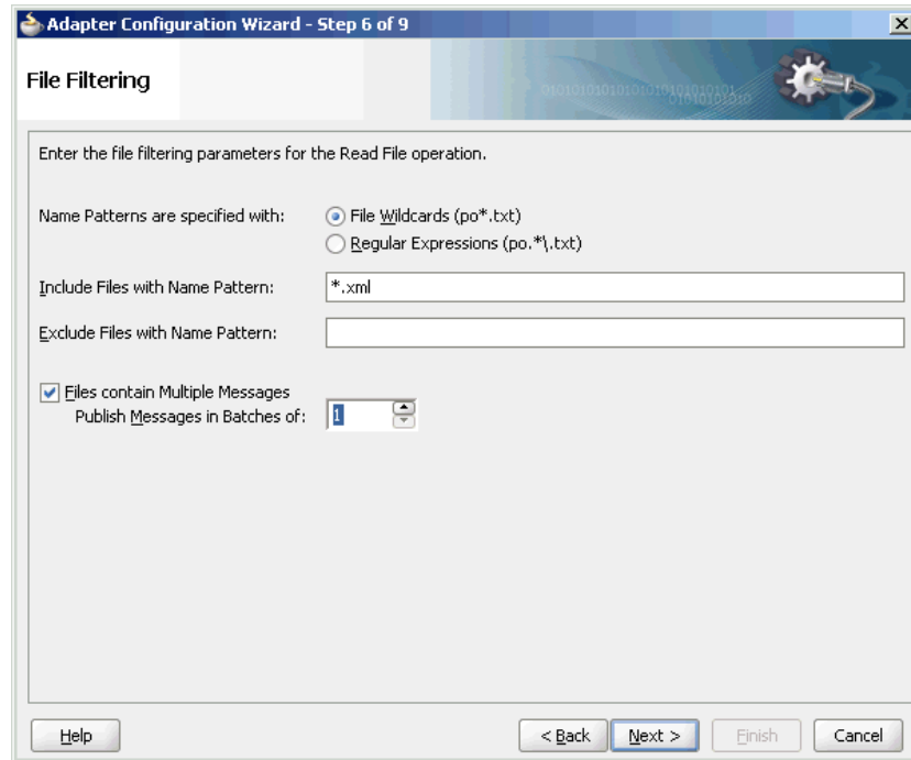
Figure 5-67 The Adapter Configuration Wizard File Filtering Page
