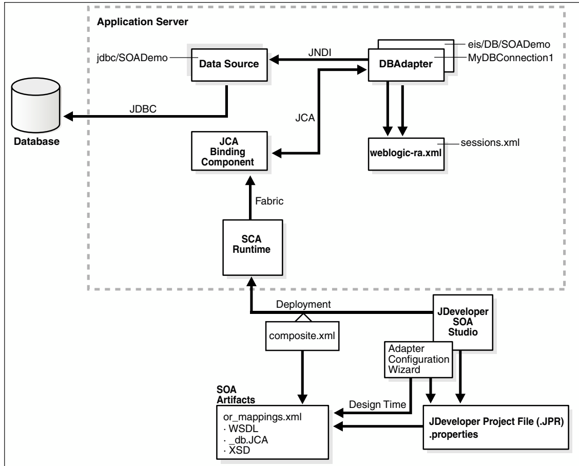
Figure 9-1 How the Oracle Database Adapter Works
