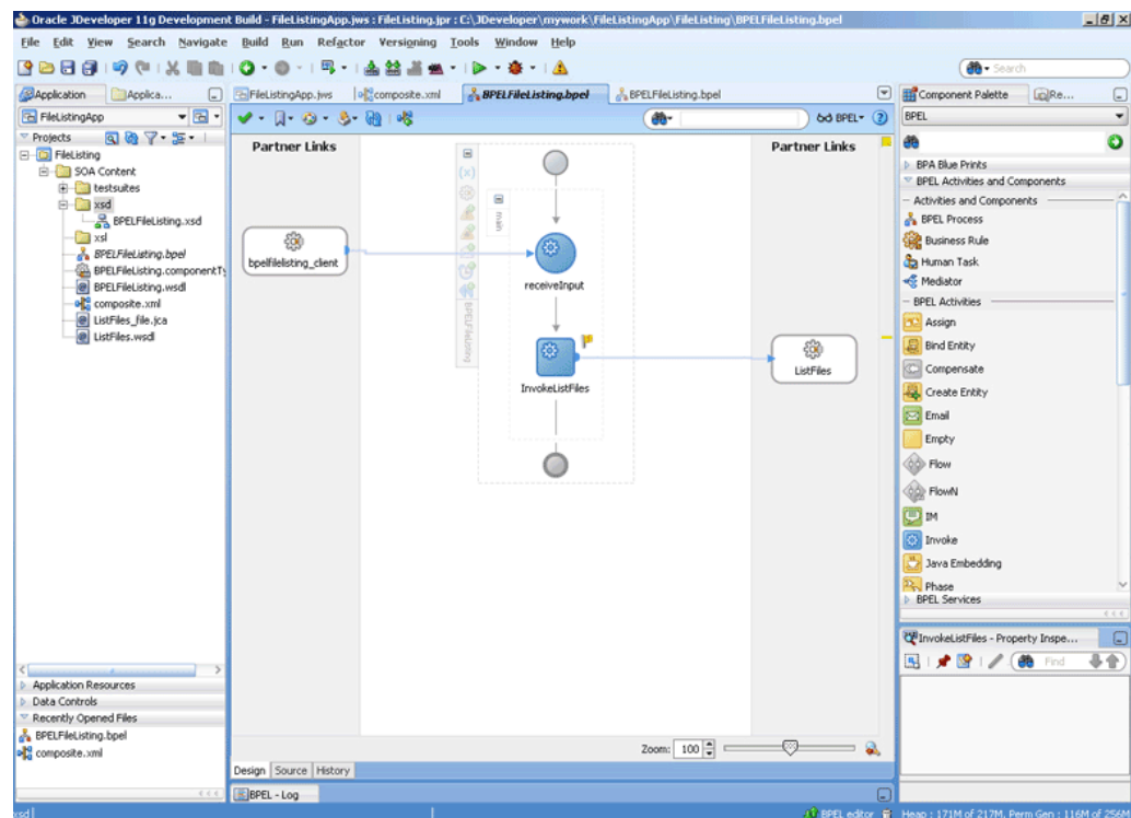
Figure 5-147 The JDeveloper - BPELFileListing.bpel
