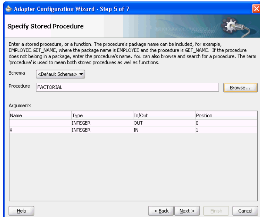
Figure 9-38 Viewing Procedure or Function Details in the Adapter Configuration Wizard
