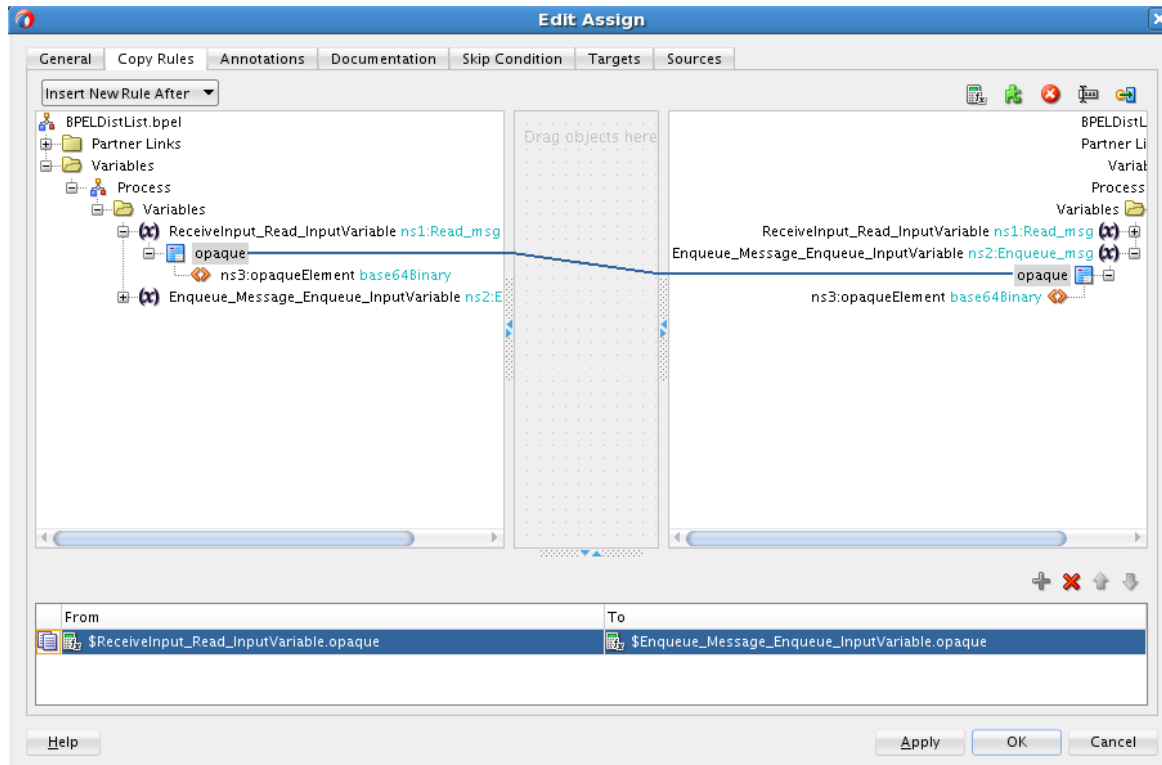
Figure 13-41 Wiring Elements in the Edit Assign Dialog
