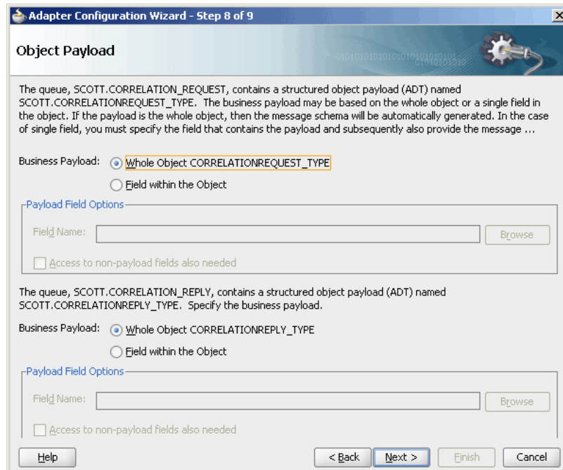
Figure 7-23 The Adapter Configuration Wizard Object Payload Page
