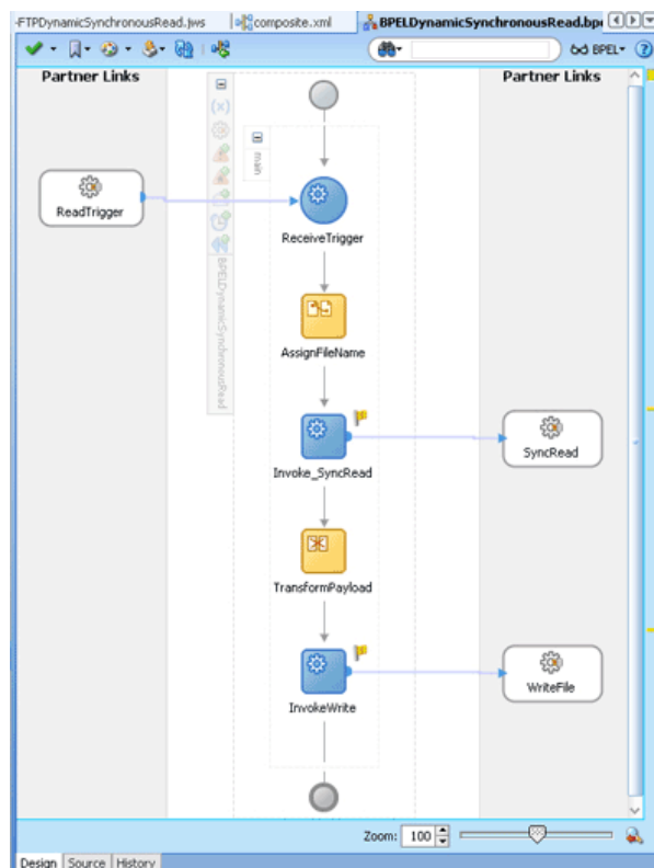
Figure 5-173 The JDeveloper - BPELDynamicSynchronousRead.bpel
