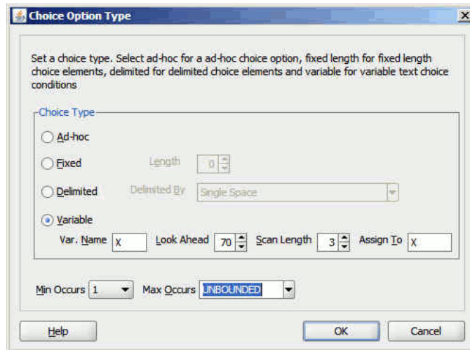
Figure 4-54 The Choice Option Type Dialog
