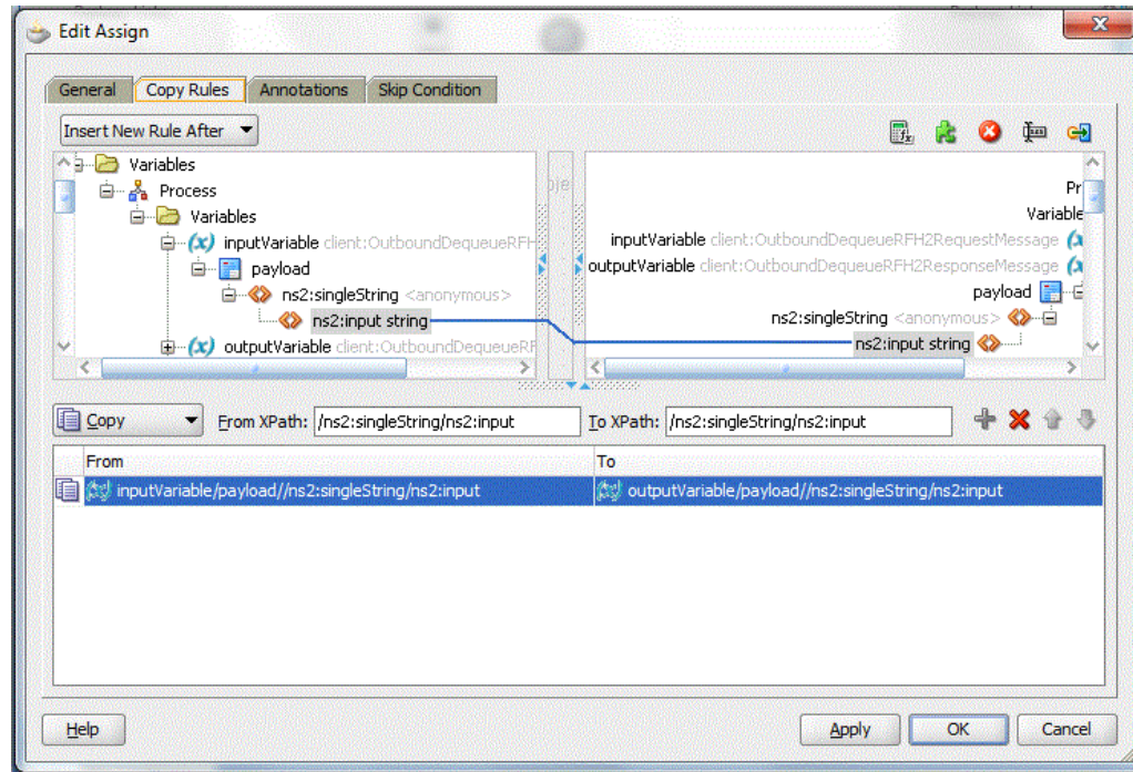
Figure 10-102 The Assign Activity Dialog
