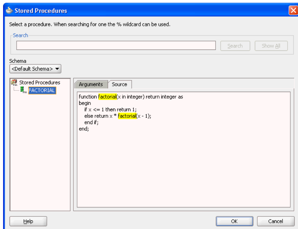
Figure 9-37 Viewing the Source Code of a Selected Procedure
