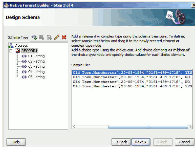
Figure 4-52 Native Format Builder Design Schema Page
