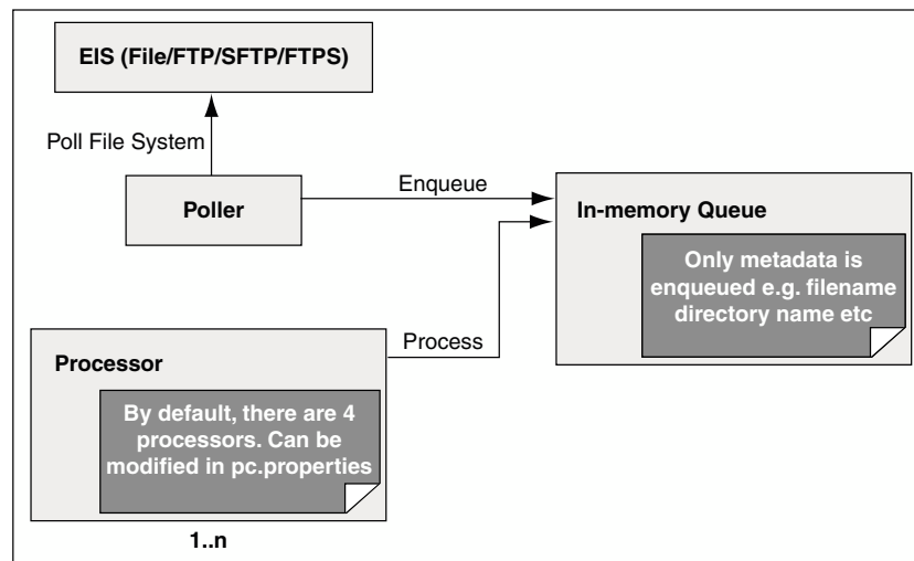
Figure 5-12 Default Threading Model
