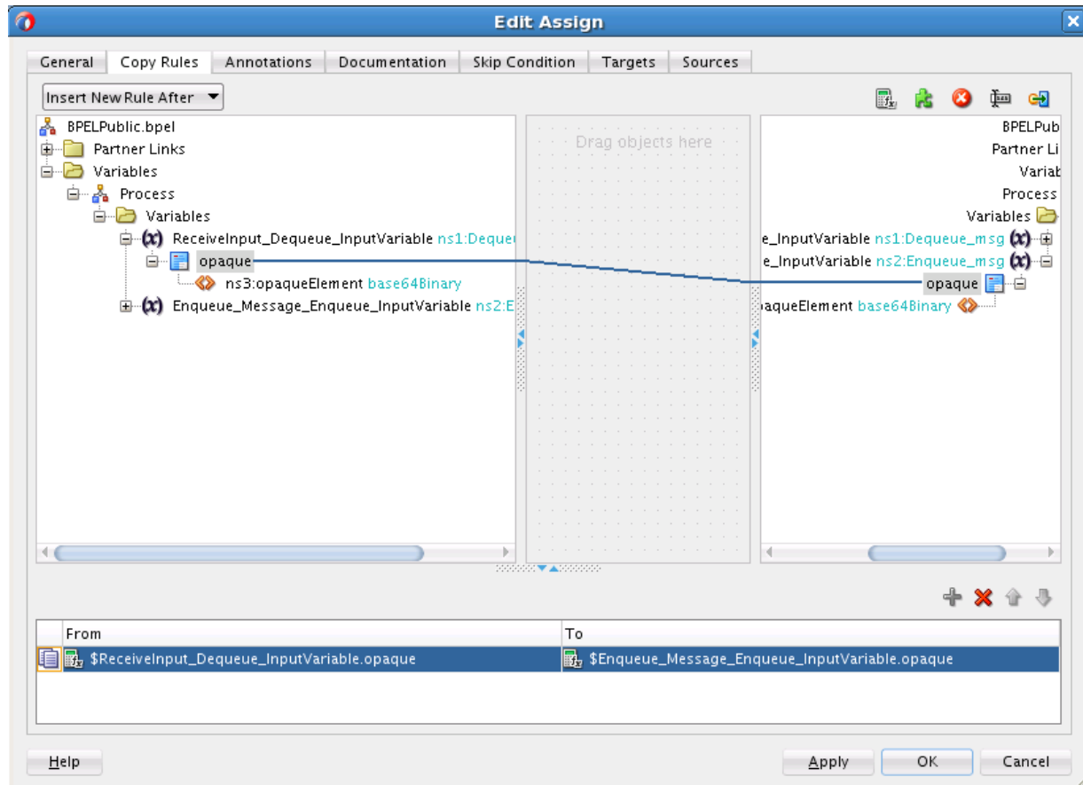
Figure 13-14 Wiring Elements in the Edit Assign Dialog
