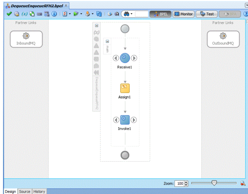
Figure 10-97 The DequeueEnqueueRFH2.bpel Page"
