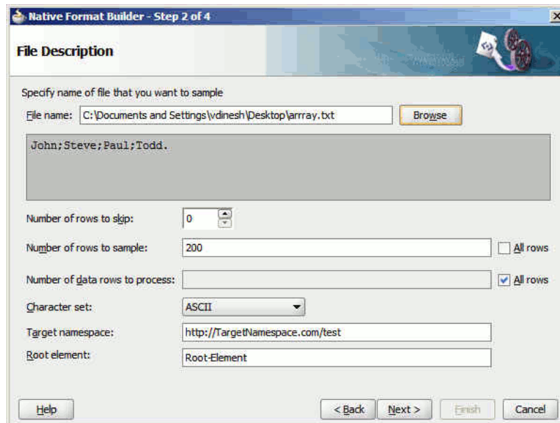
Figure 4-58 Native Format Builder File Description Page
