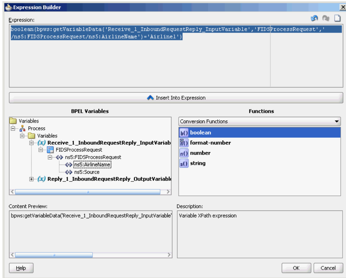
Figure 6-91 The Expression Builder Dialog
