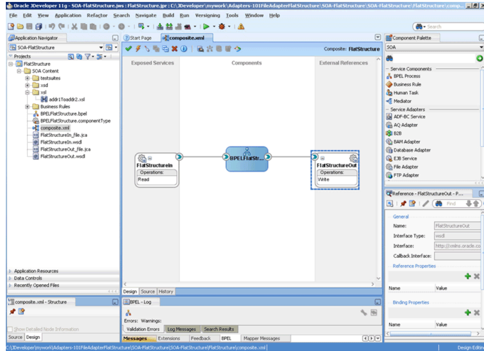
Figure 5-90 The JDeveloper - composite.xml
