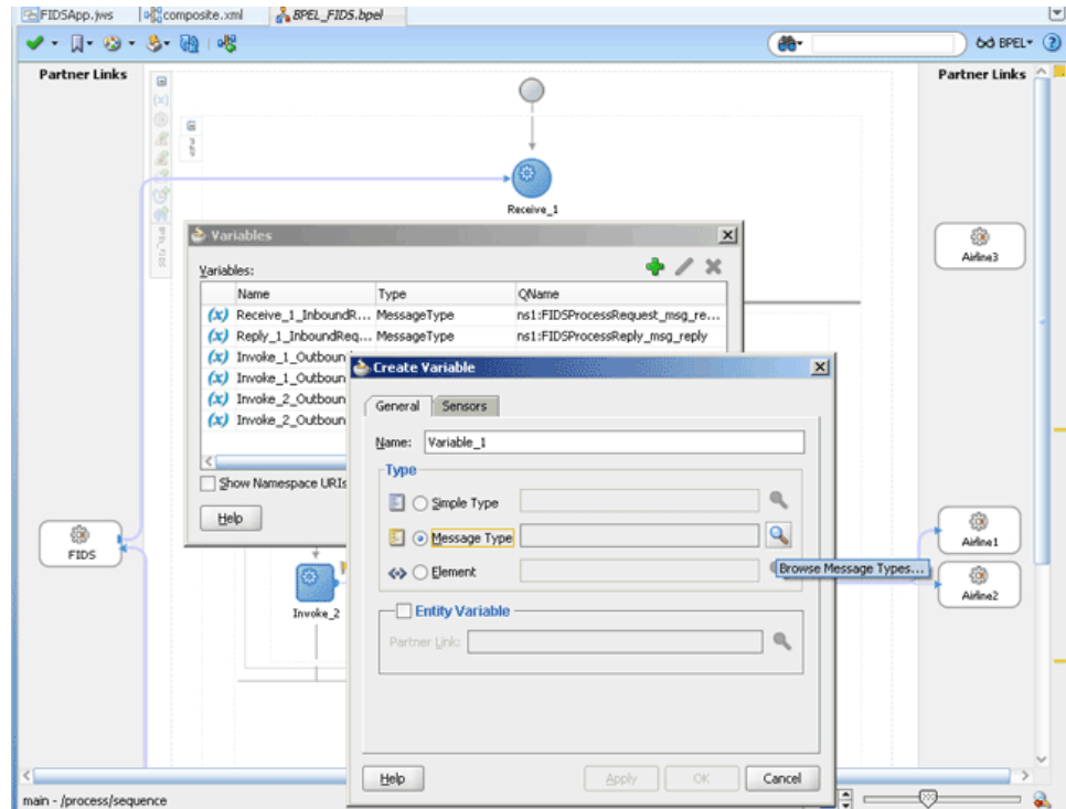
Figure 6-99 The Create Variable Dialog
