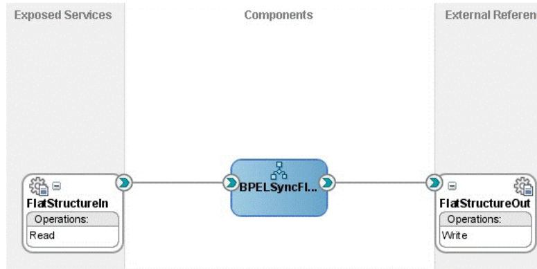
Figure 5-175 Cresting the Inbound Service and Outbound References
