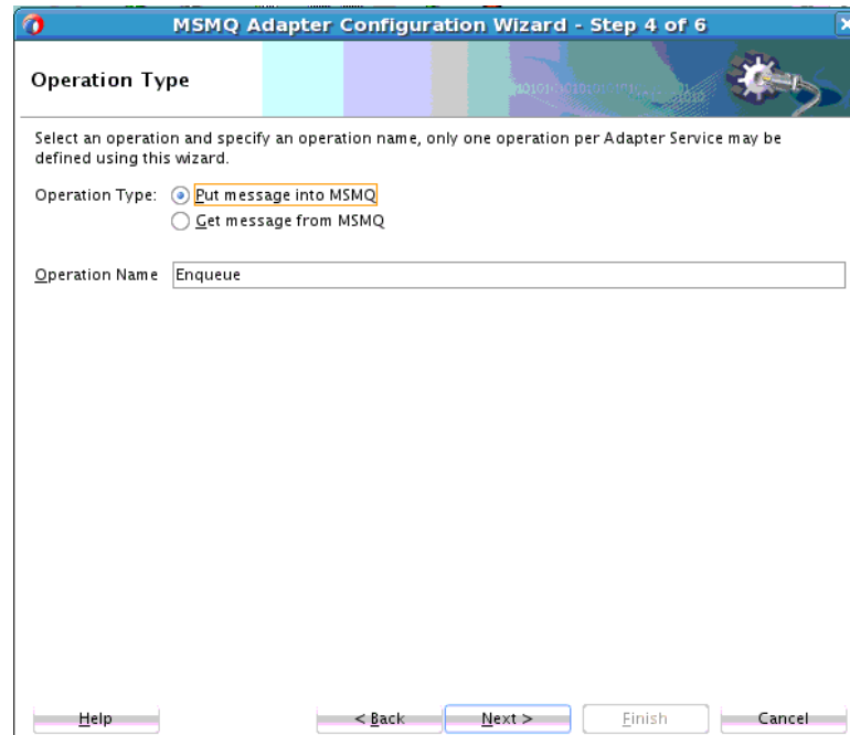
Figure 13-2 MSMQ Adapter Operation Type Screen
