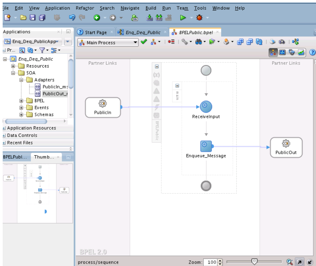
Figure 13-13 BPELPublic.bpel Page After Invoke Activity Has Been Added
