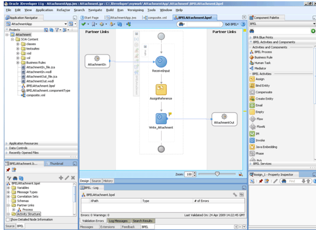
Figure 5-140 The JDeveloper - BPELScalableDOM.bpel
