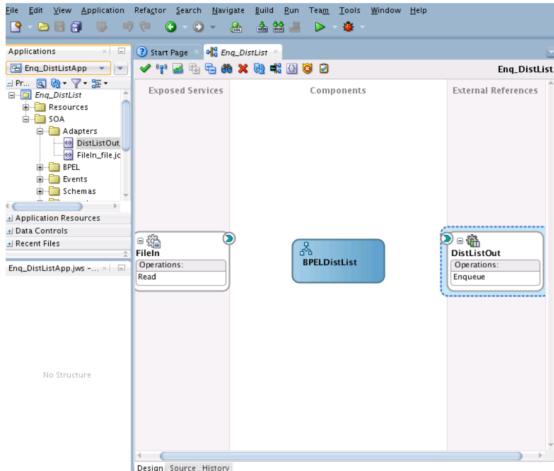
Figure 13-33 The Configured Outbound File Adapter with the composite.xml
