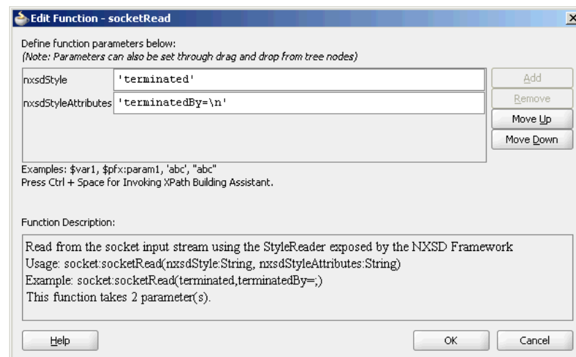
Figure 6-22 The Edit Function - socketRead Dialog
