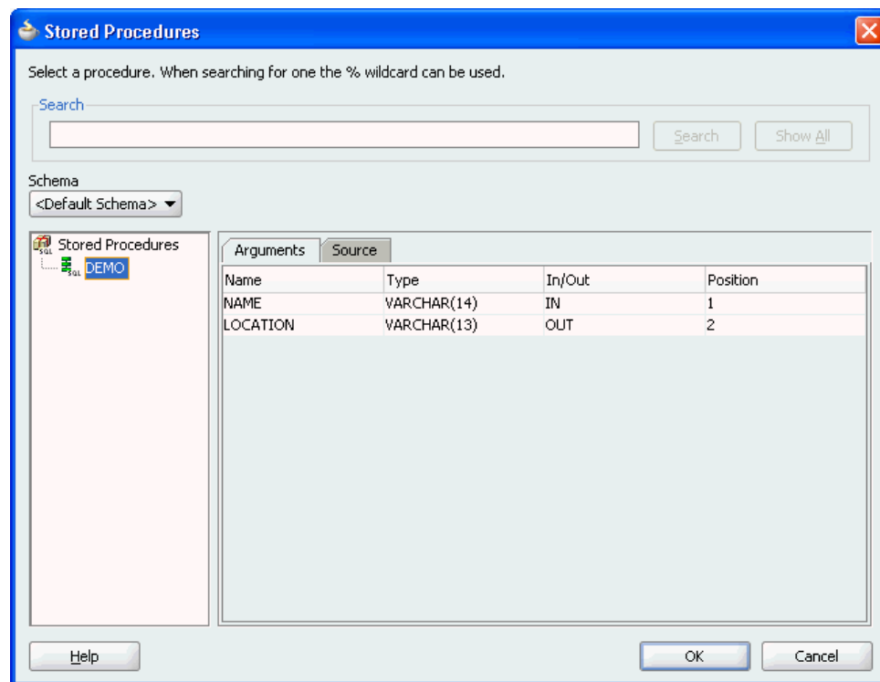
Figure 9-44 The Stored Procedures Dialog
