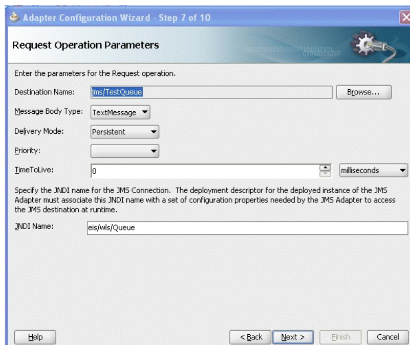
Figure 8-27 The Request Operation Parameters Screen
