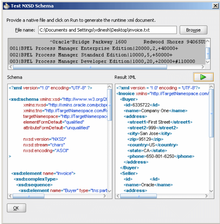
Figure 4-45 Test NXSD Schema Dialog - Result XML
