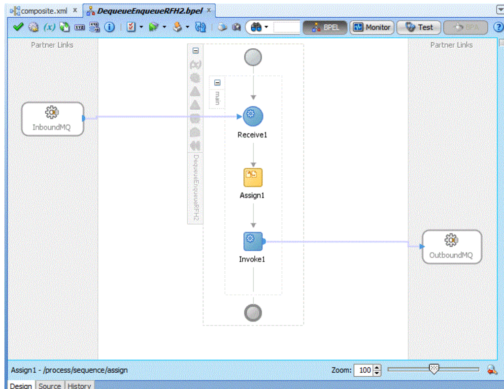
Figure 10-99 The DequeueEnqueueRFH2.bpel page
