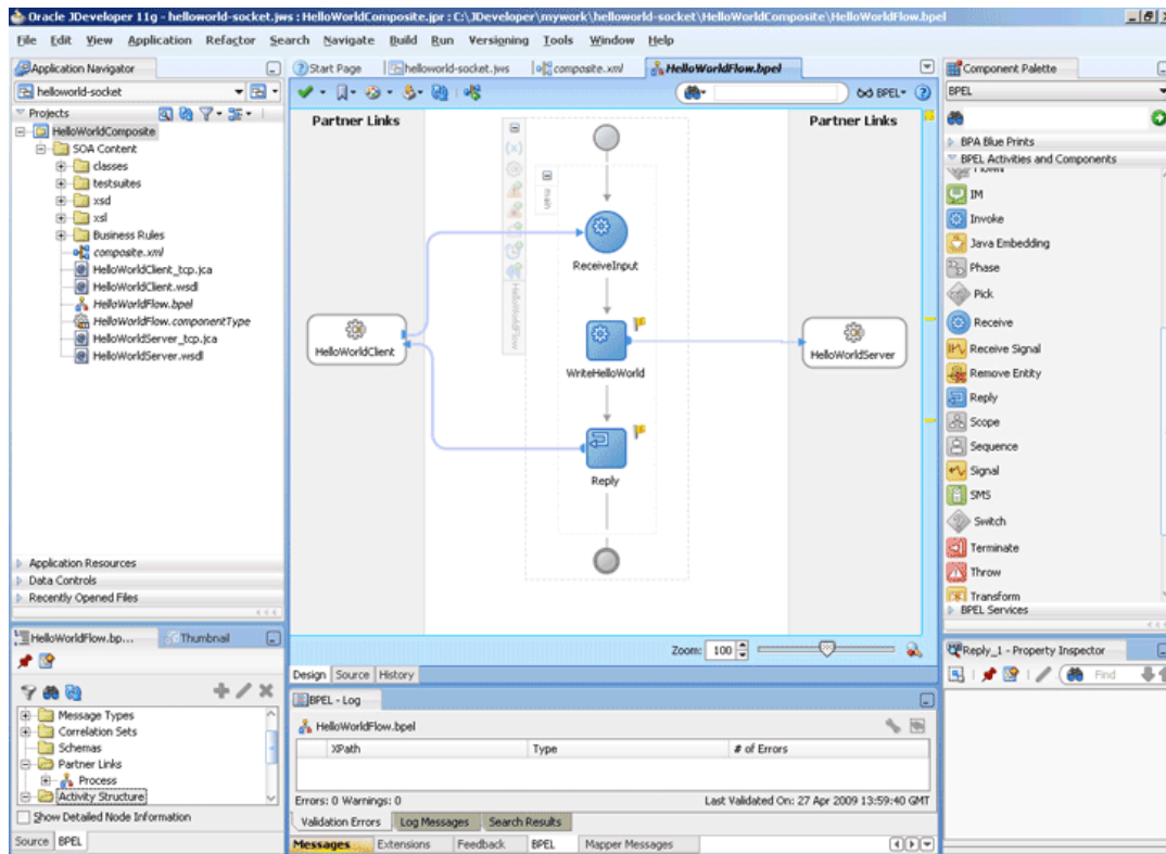
Figure 6-65 The JDeveloper - HelloWorldFlow.bpel
