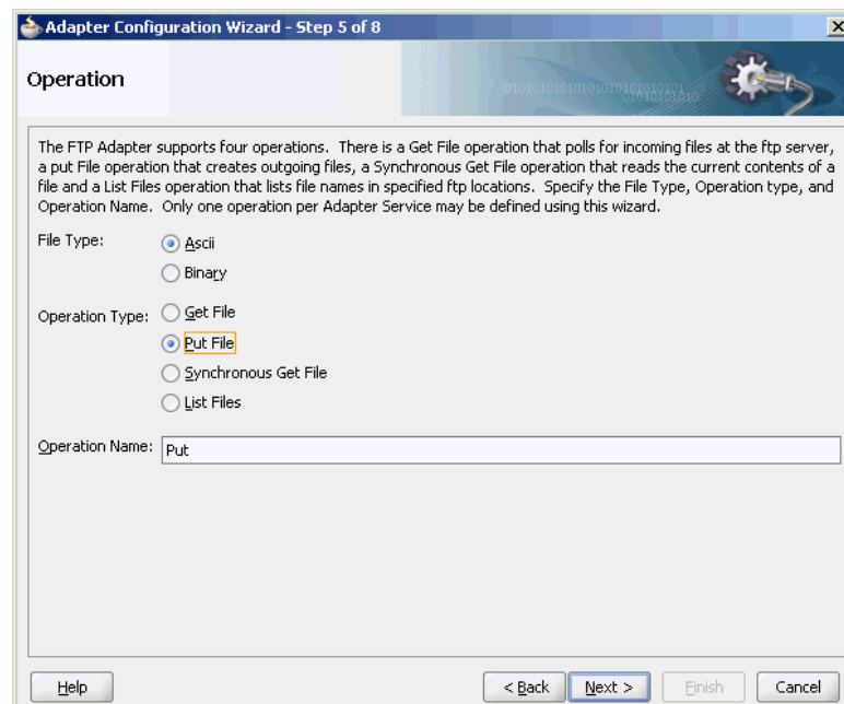
Figure 5-45 Selecting the Put File Operation
