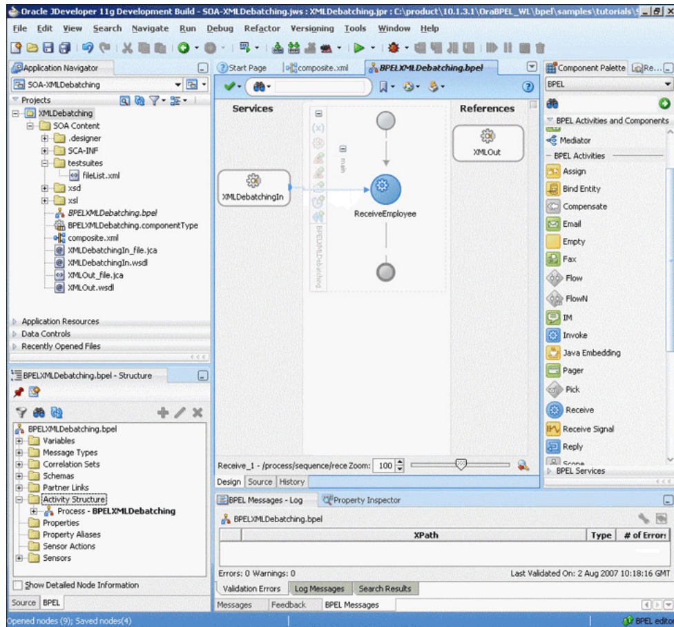
Figure 5-77 The JDeveloper - BPELXMLDebatching.bpel
