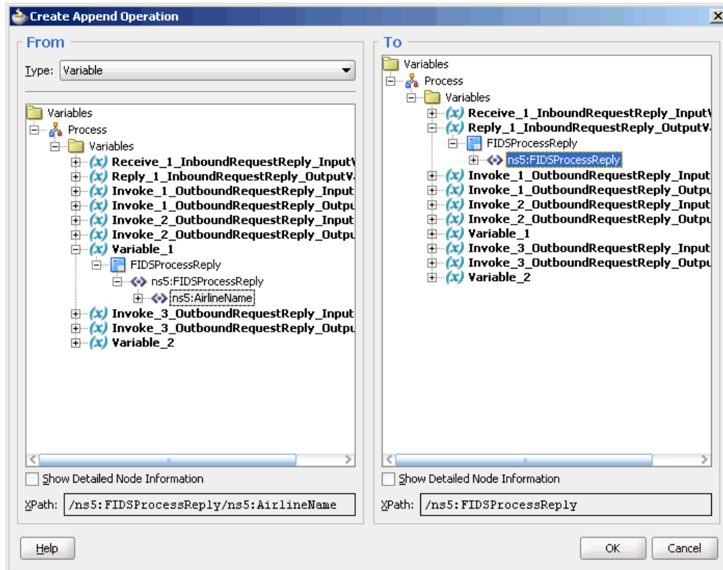
Figure 6-108 The Create Append Operation Dialog
