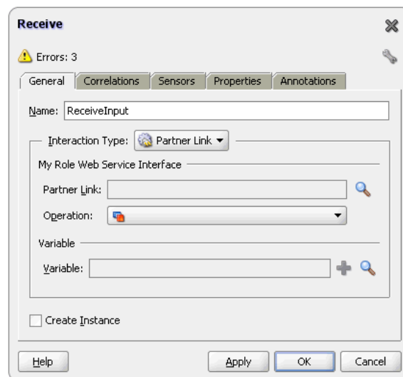
Figure 6-54 The Receive Dialog
