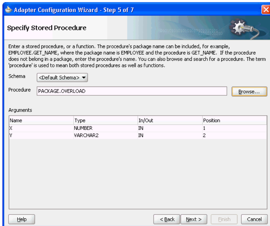
Figure 9-43 Viewing Procedure or Function Details in the Adapter Configuration Wizard
