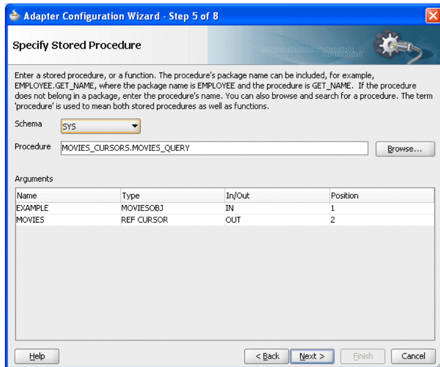
Figure 9-39 Viewing Procedure or Function Details in the Adapter Configuration Wizard: Row Set Type
