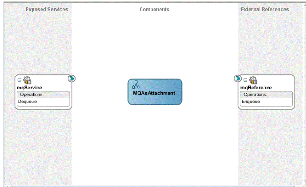
Figure 10-106 Composite.xml after Outbound Adapter Service Configured
