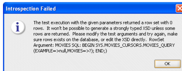
Figure 9-53 Introspection Failed Dialog
