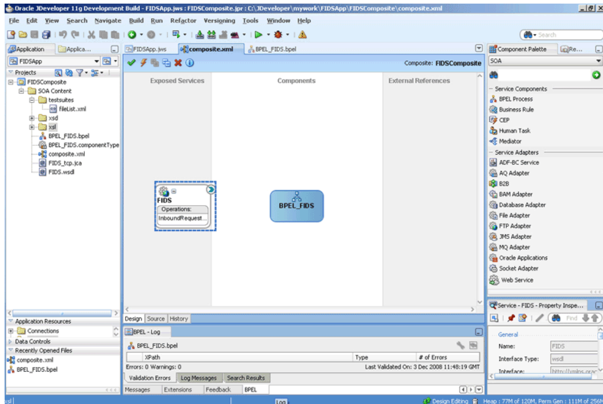
Figure 6-74 The JDeveloper - composite.xml Page
