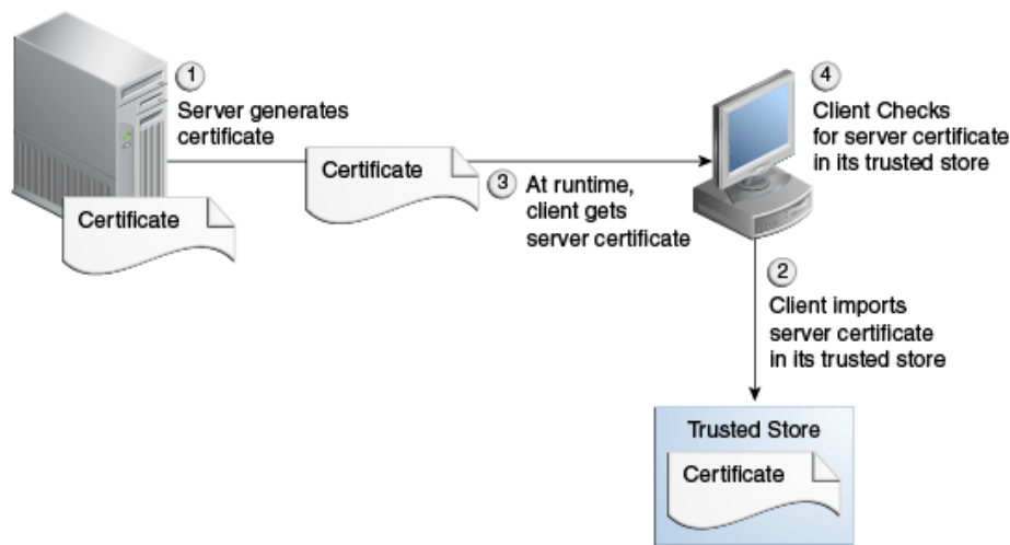
Figure 12-27 Using Certificates and Trusted Store with SSL
