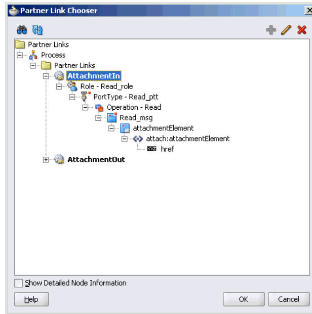
Figure 5-131 The Partner Link Chooser Dialog
