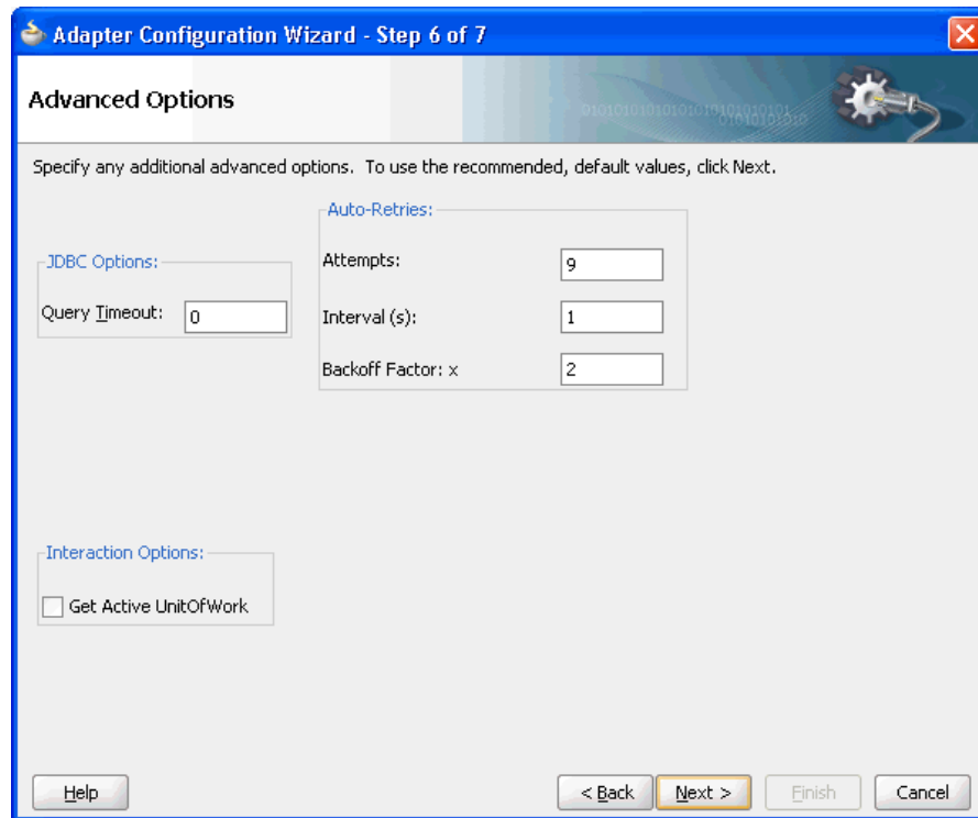
Figure 9-40 The Advanced Options Page
