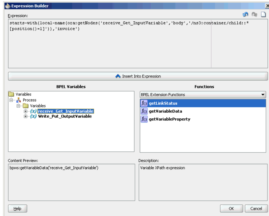
Figure 5-162 The Expression Builder Dialog
