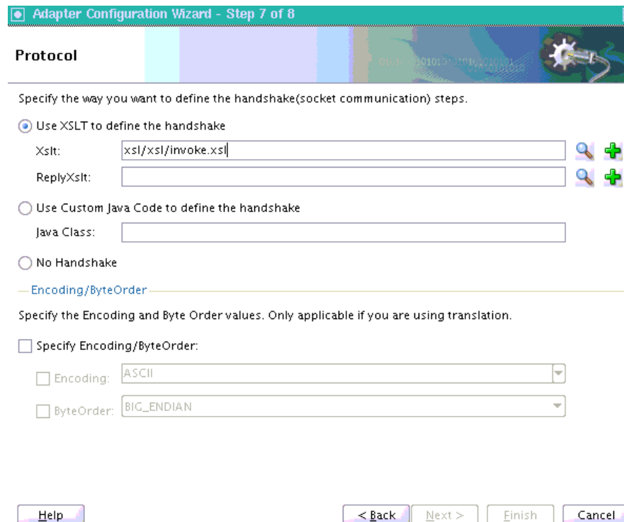
Figure 6-6 Defining a Protocol with the Handshake Mechanism By Using a Style Sheet
