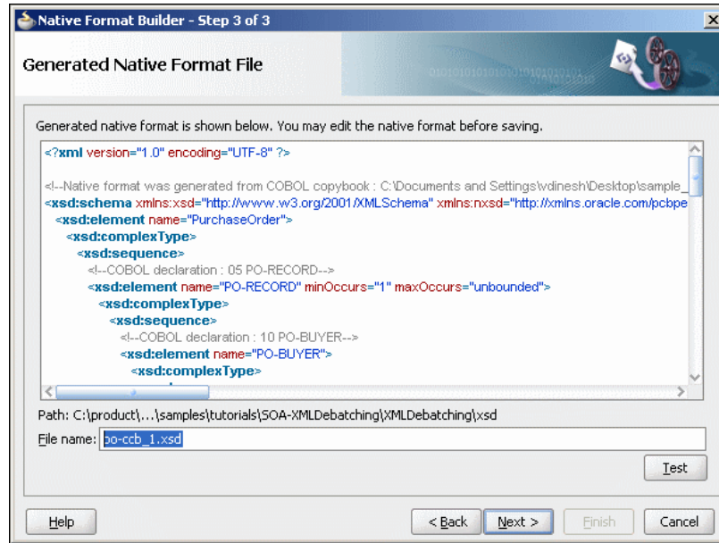
Figure 4-68 Native Format Builder Wizard Generated Native Format File Page
