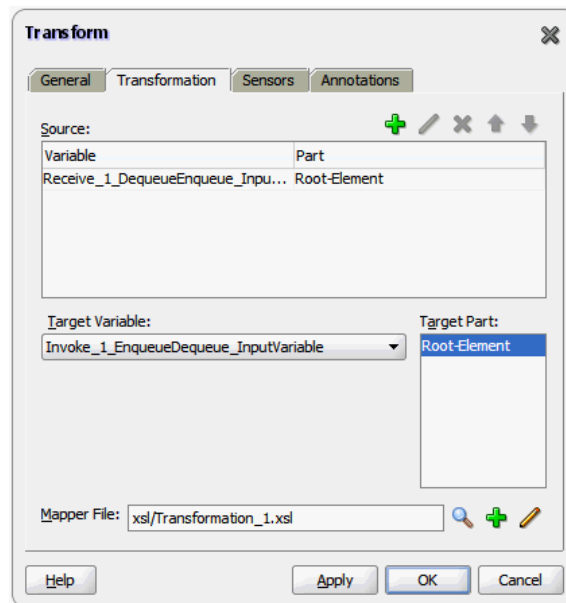
Figure 10-71 The Transform Dialog
