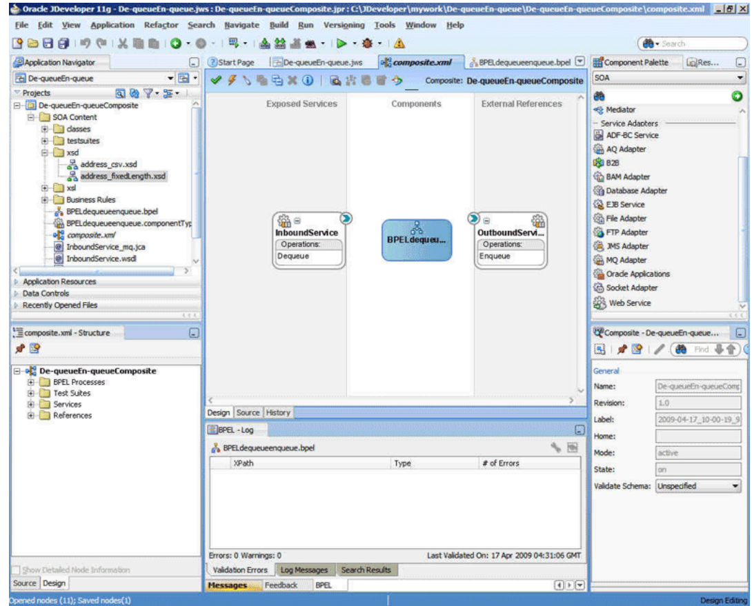
Figure 10-54 The JDeveloper Page - composite.xml Page
