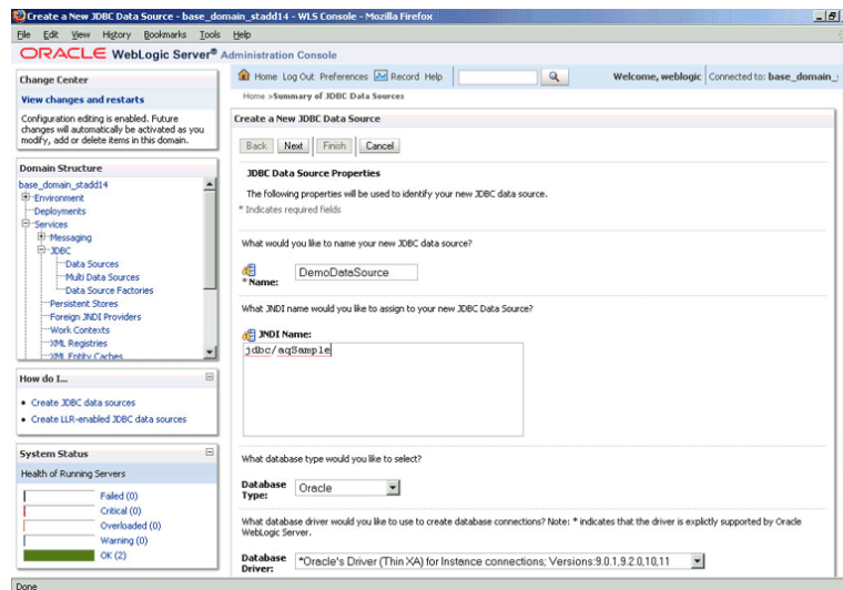
Figure 7-44 The Create a New JDBC Data Source Page
