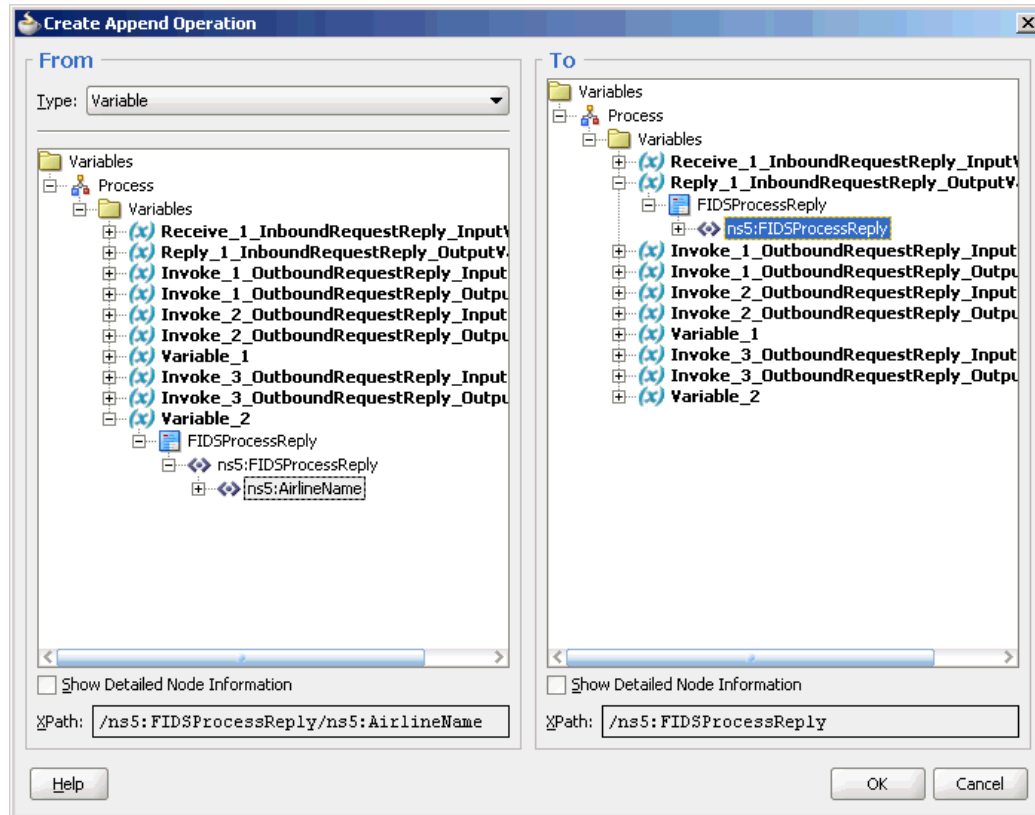
Figure 6-109 The Create Append Operation Dialog
