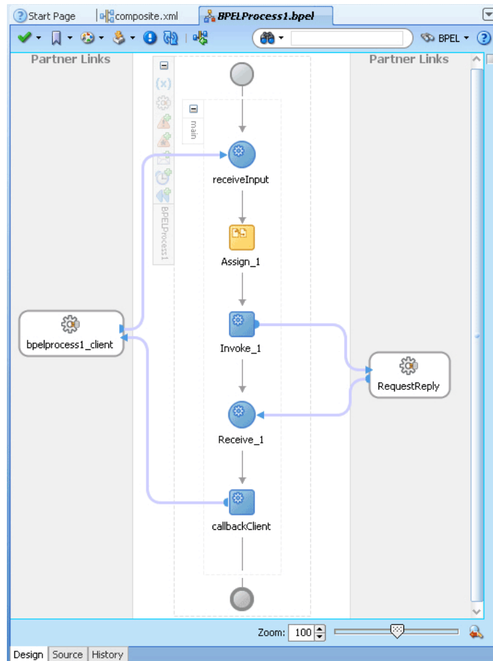
Figure 7-31 The JDeveloper - BPELProcess1.bpel
