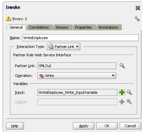
Figure 5-80 The Invoke Dialog
