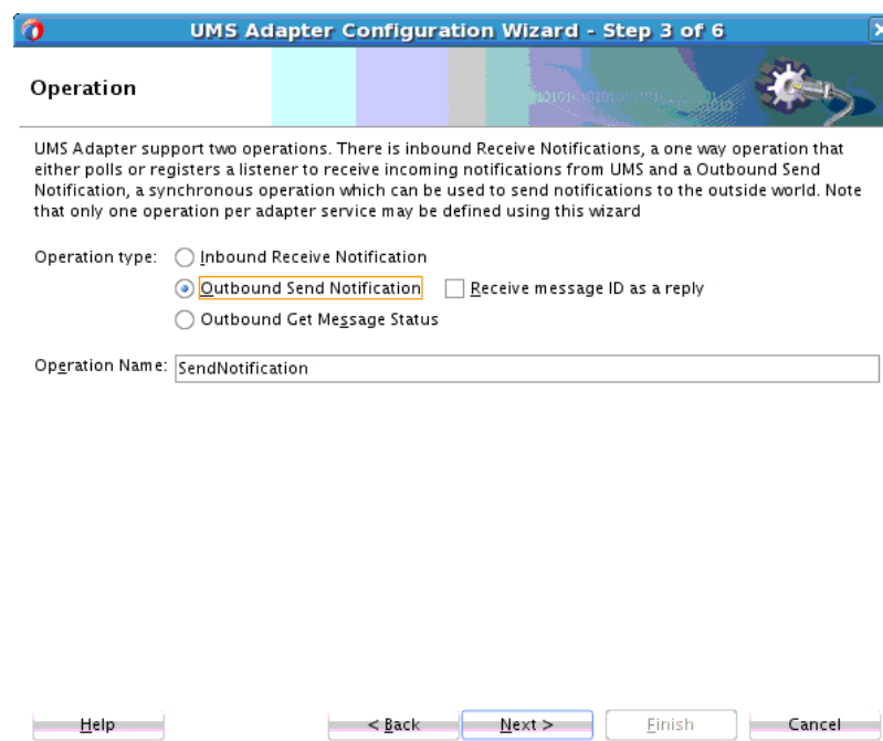
Figure 11-13 UMS Adapter Configuration Wizard Operation Screen with Outbound Send Operation Selected
