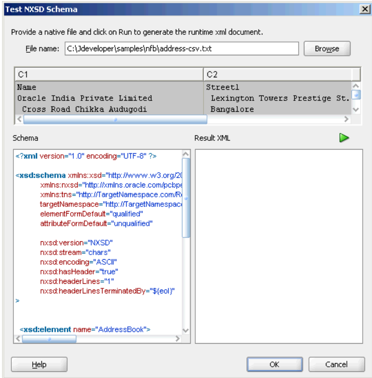
Figure 4-13 Test NXSD Schema Dialog
