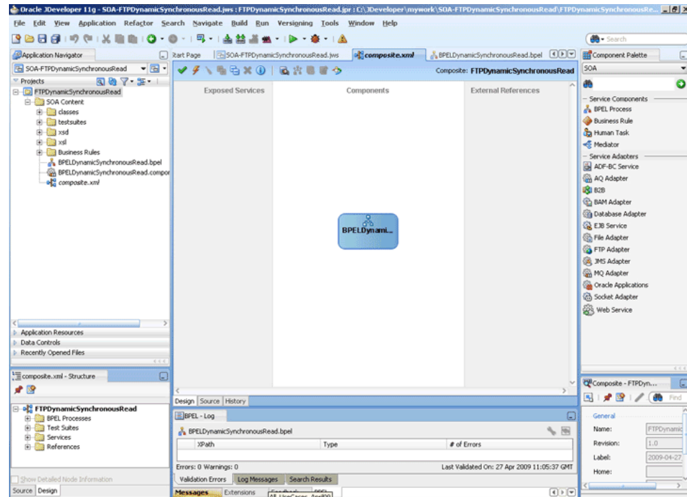
Figure 5-164 The JDeveloper - Composite.xml
