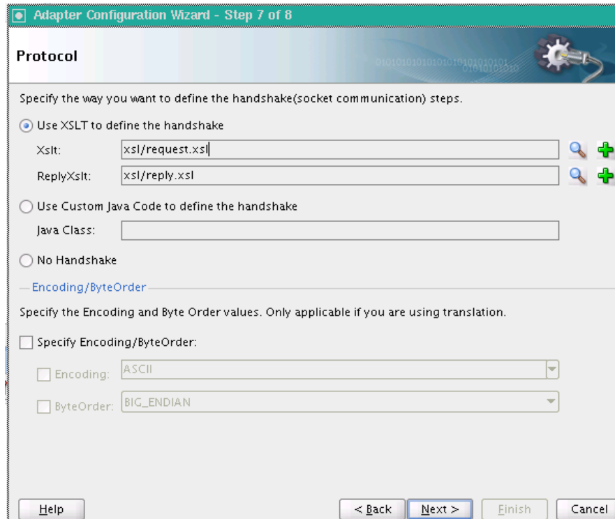
Figure 6-73 The Adapter Configuration Wizard - Protocol Page
