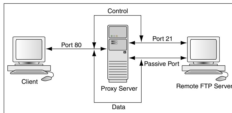
Figure 5-8 Remote FTP Server Communication Through a Proxy Server
