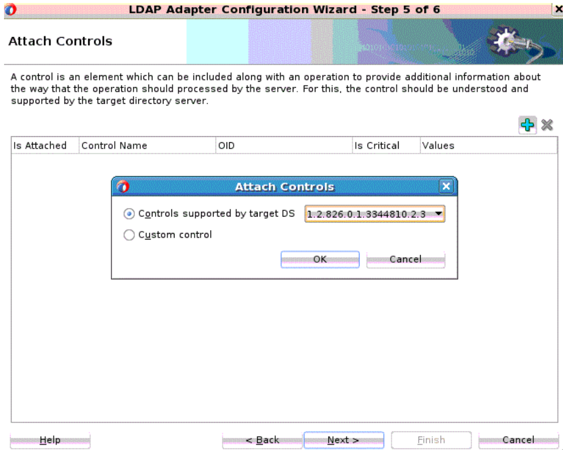
Figure 12-14 LDAP Adapter Configuration Wizard Attach Controls Chooser Screen
