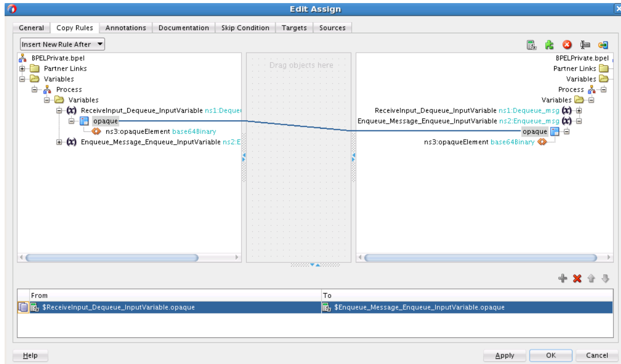
Figure 13-28 Wiring Elements in the Edit Assign Dialog
