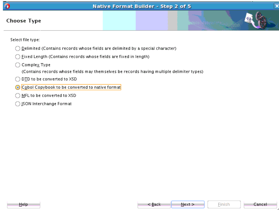
Figure 4-66 Native Format Builder Wizard Choose Type Page
