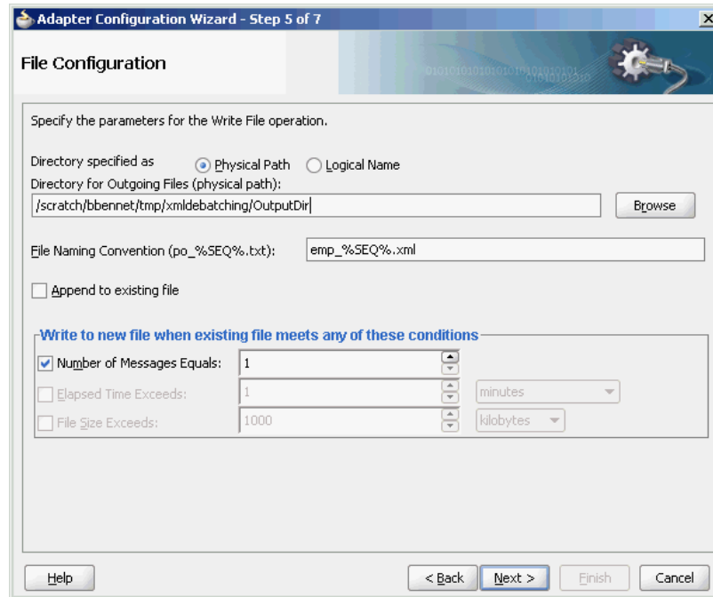
Figure 5-71 The Adapter Configuration Wizard - File Configuration Page
