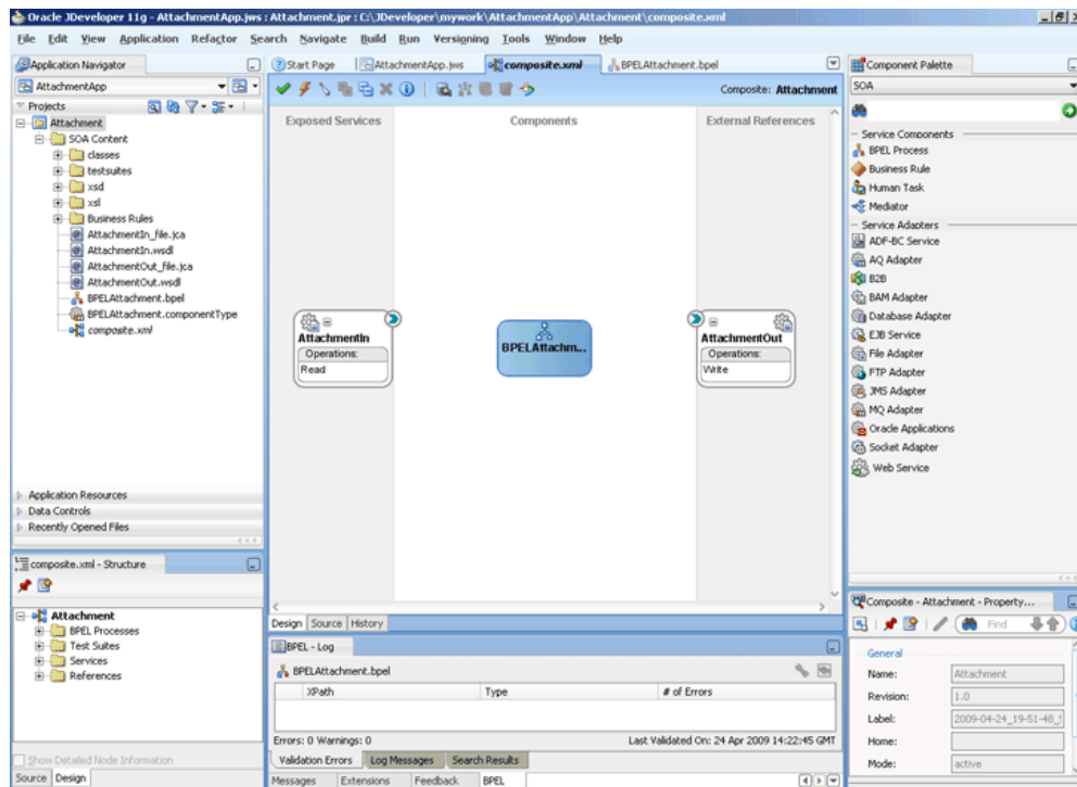
Figure 5-129 The JDeveloper - Composite.xml
