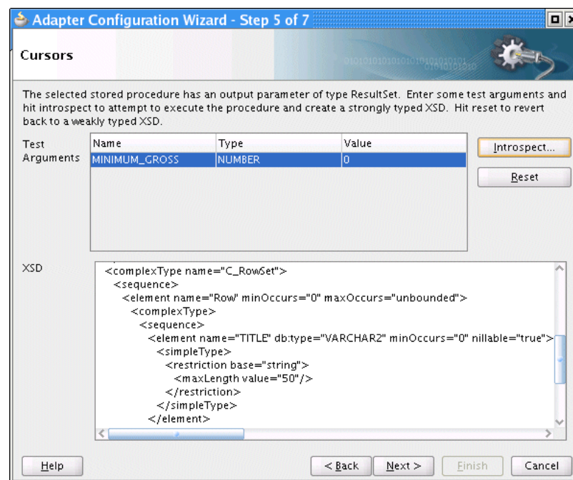
Figure 9-52 RowSets Page: Successful Introspection
