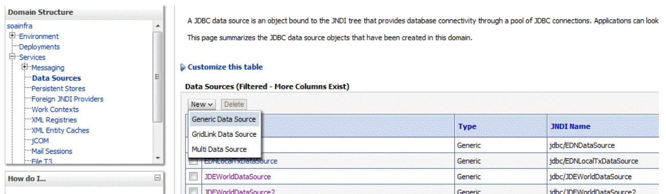
Figure 15-4 Choosing a Generic Data Source
