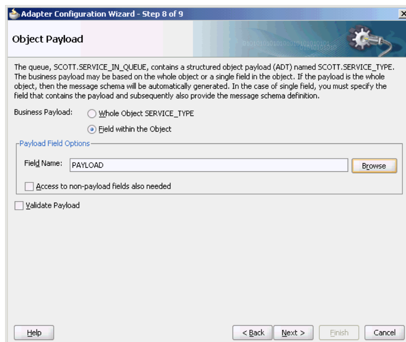
Figure 7-14 The Adapter Configuration Wizard Object payload Page
