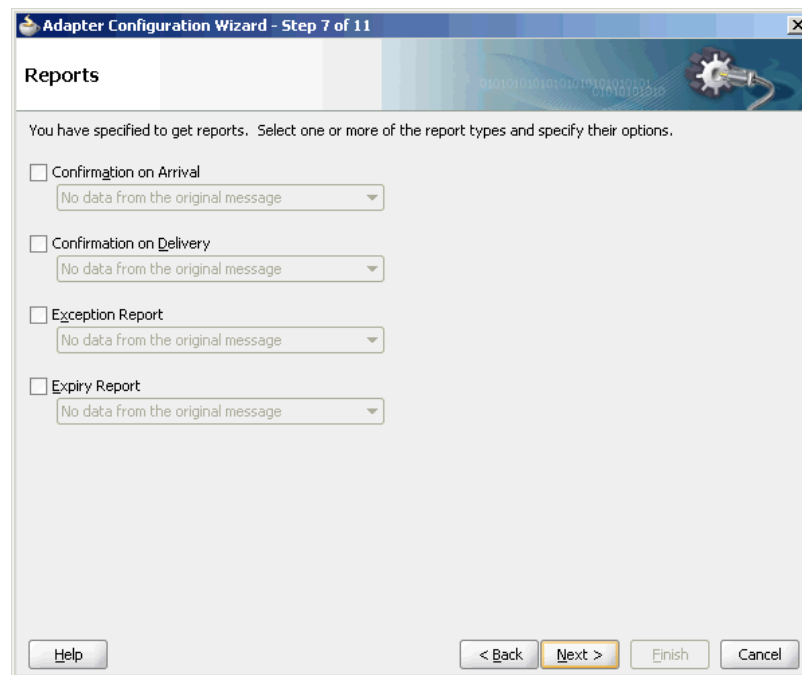
Figure 10-14 Reports Page
