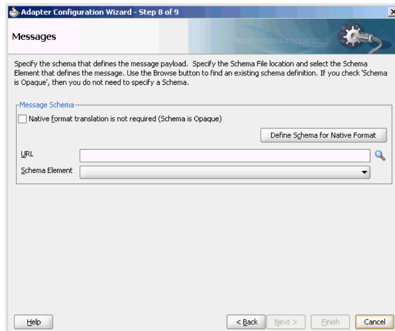
Figure 10-9 Messages Page
