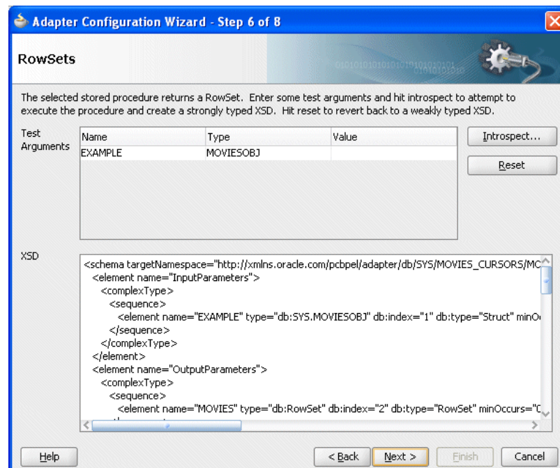
Figure 9-56 RowSets Page
