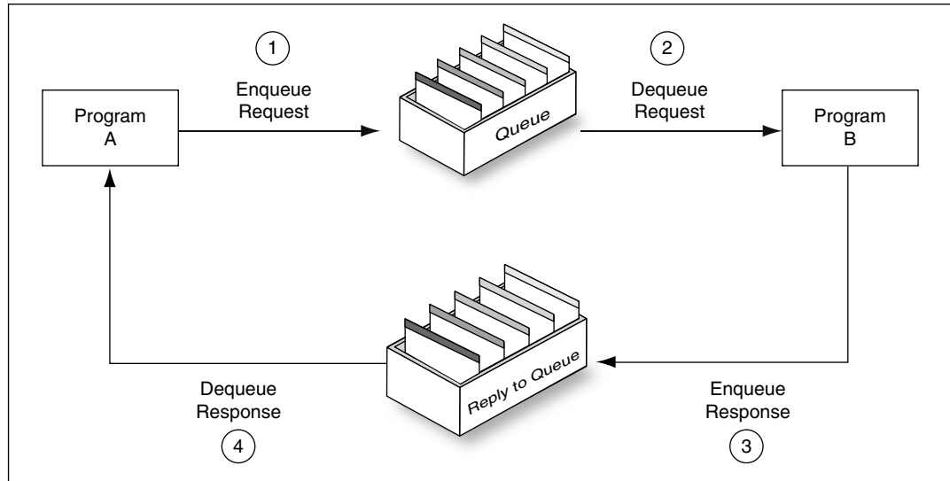
Figure 10-2 Request/Response Interaction
