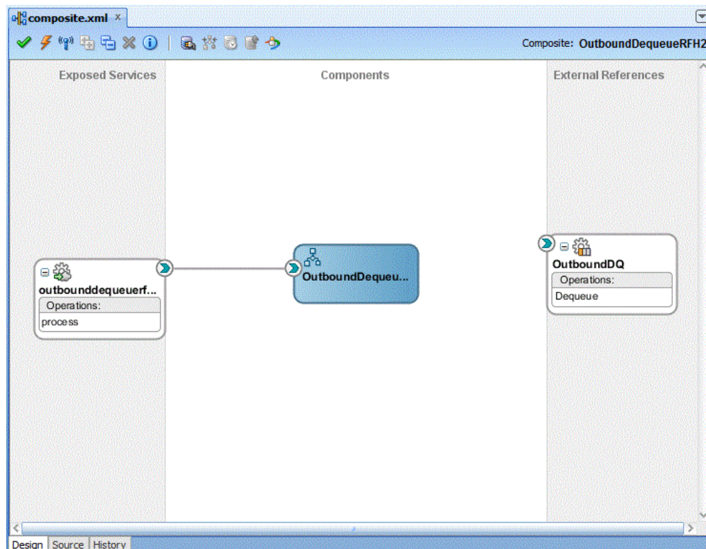
Figure 10-100 The JDeveloper-composite.xml
