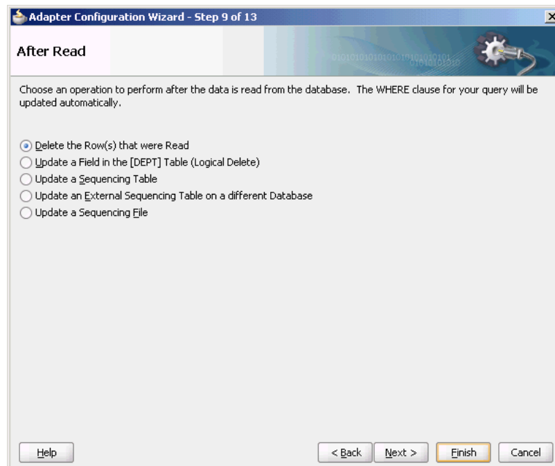
Figure 9-9 Polling Operations
