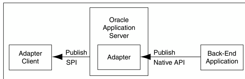
Figure 1-17 Event-Notification Service
