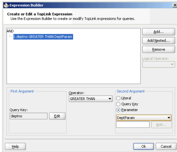
Figure 9-19 Expression Builder
