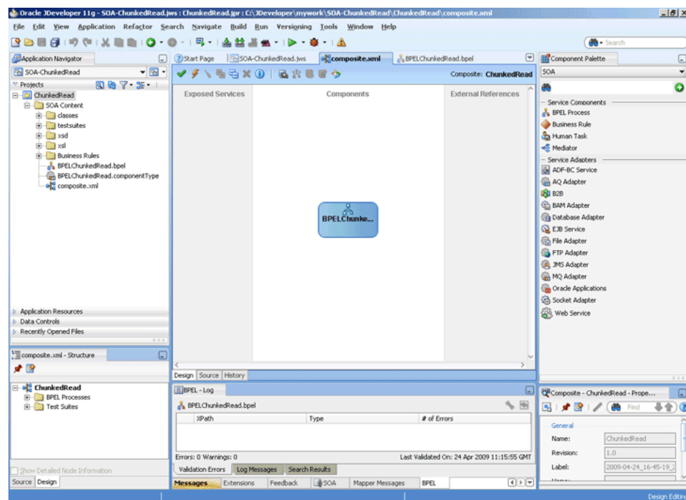
Figure 5-108 The JDeveloper - Composite.xml
