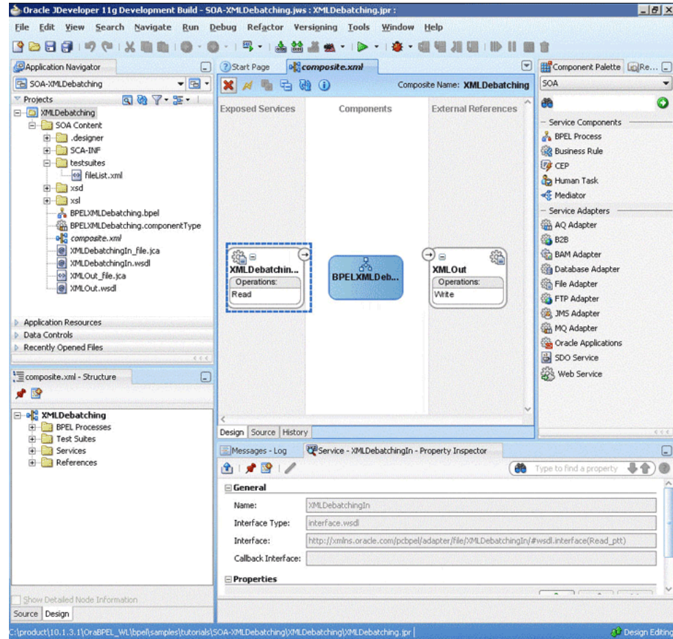
Figure 5-72 The JDeveloper - Composite.xml
