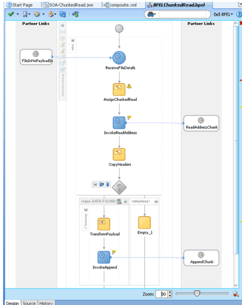
Figure 5-124 The JDeveloper - BPELChunkedRead.bpel
