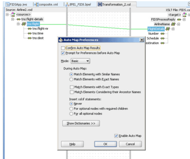
Figure 6-101 The Transformation_2.XSL Page With Auto Map Preference Dialog
