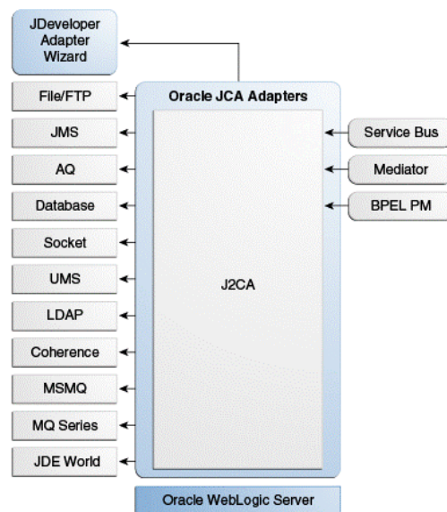
Figure 1-2 Oracle Technology Adapters Architecture
