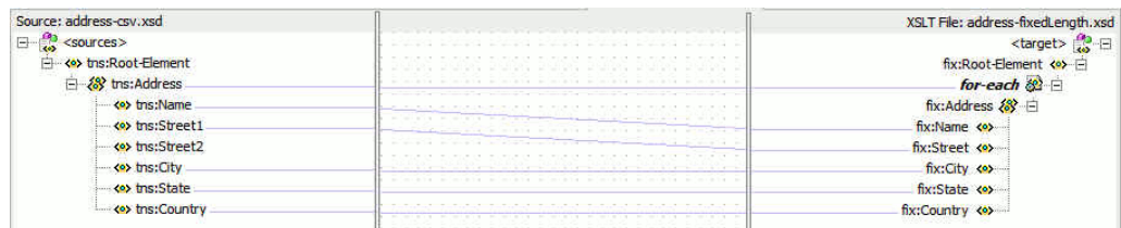
Figure 10-61 The Transformation.xsl Page
