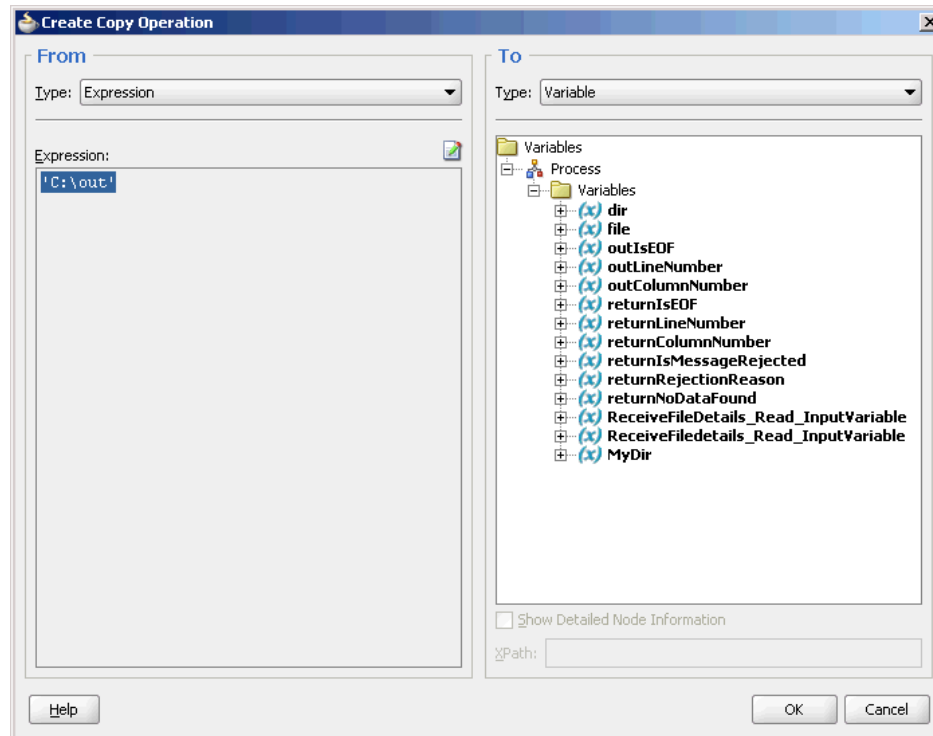
Figure 5-33 Create Copy Operation Dialog
