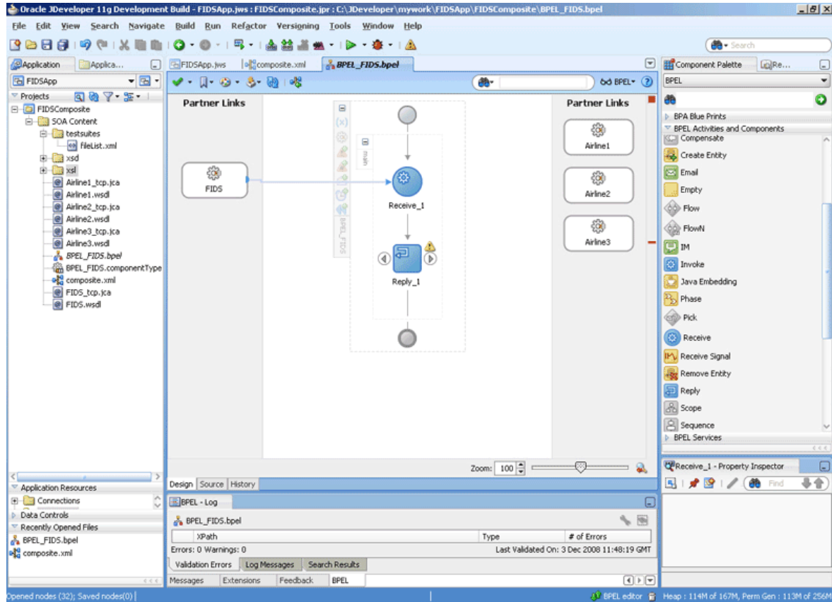
Figure 6-85 The JDeveloper - BPEL_FIDS.bpel
