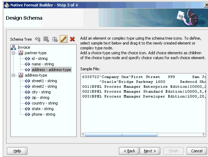
Figure 4-37 Native Format Builder Wizard Design Schema Page
