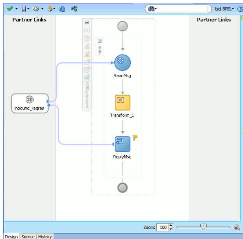
Figure 10-62 The BPELsyncreqres.bpel Page
