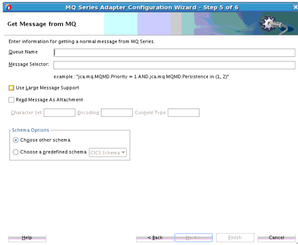
Figure 10-42 Message Selector Field on the Get Message from MQ Screen in the MQ Adapter Configuration Wizard
