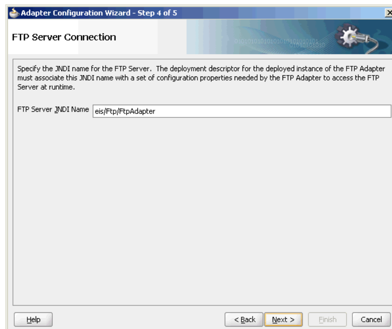
Figure 5-42 Specifying FTP Server Connection Information
