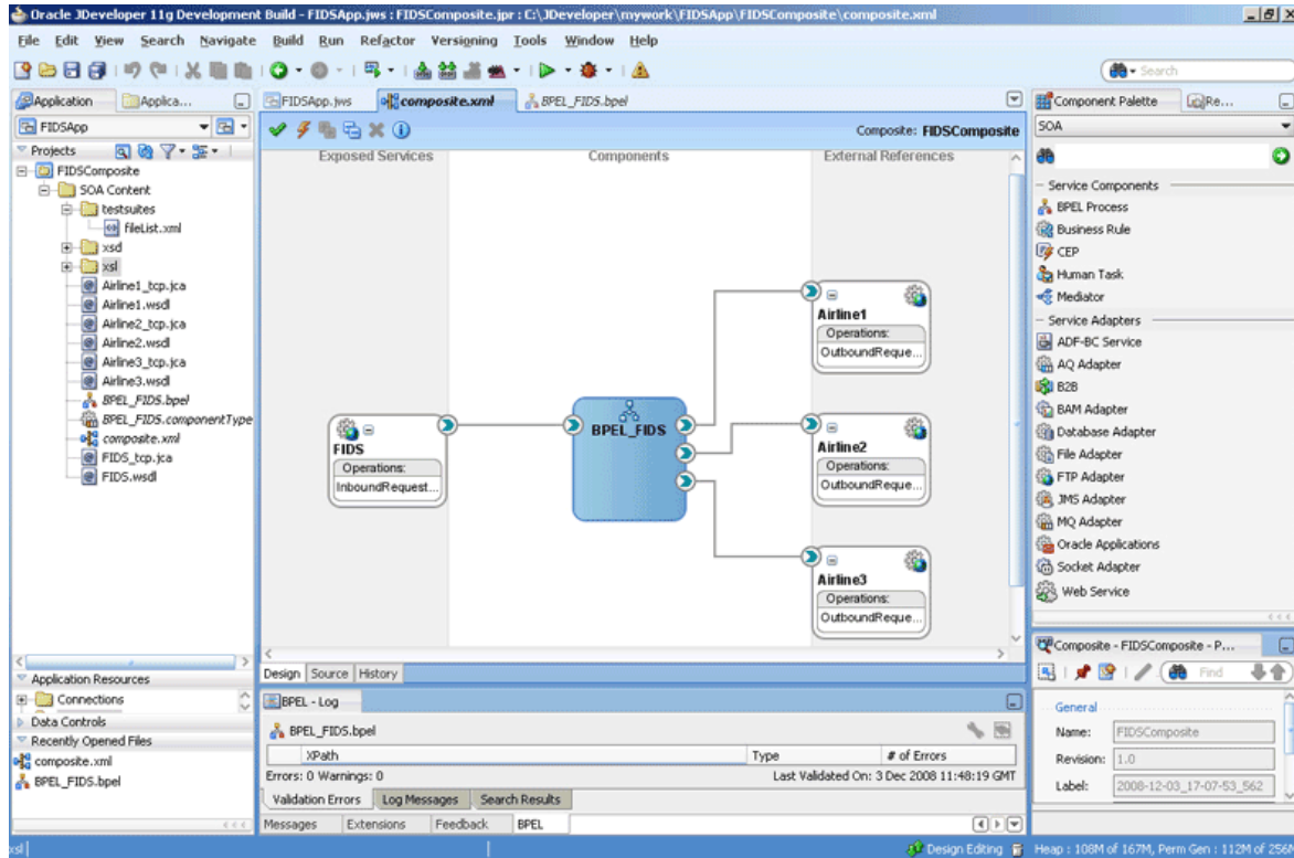
Figure 6-81 The JDeveloper - composite.xml
