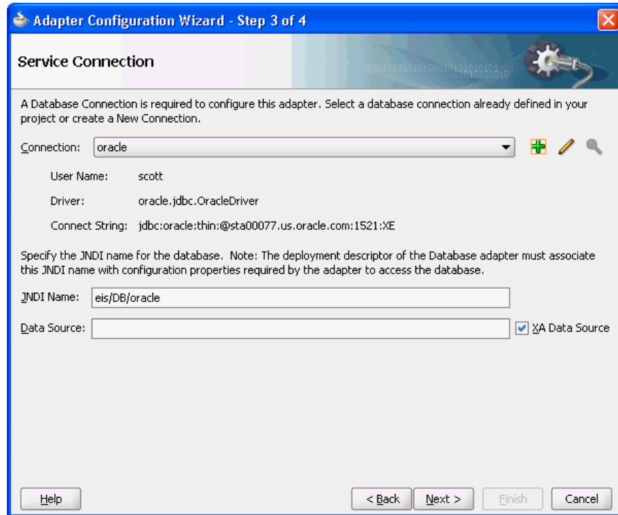
Figure 9-32 Setting the Database Connection in the Adapter Configuration Wizard
