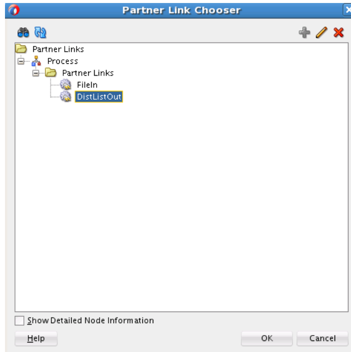
Figure 13-38 Partner Link Chooser with DistListOut Selected
