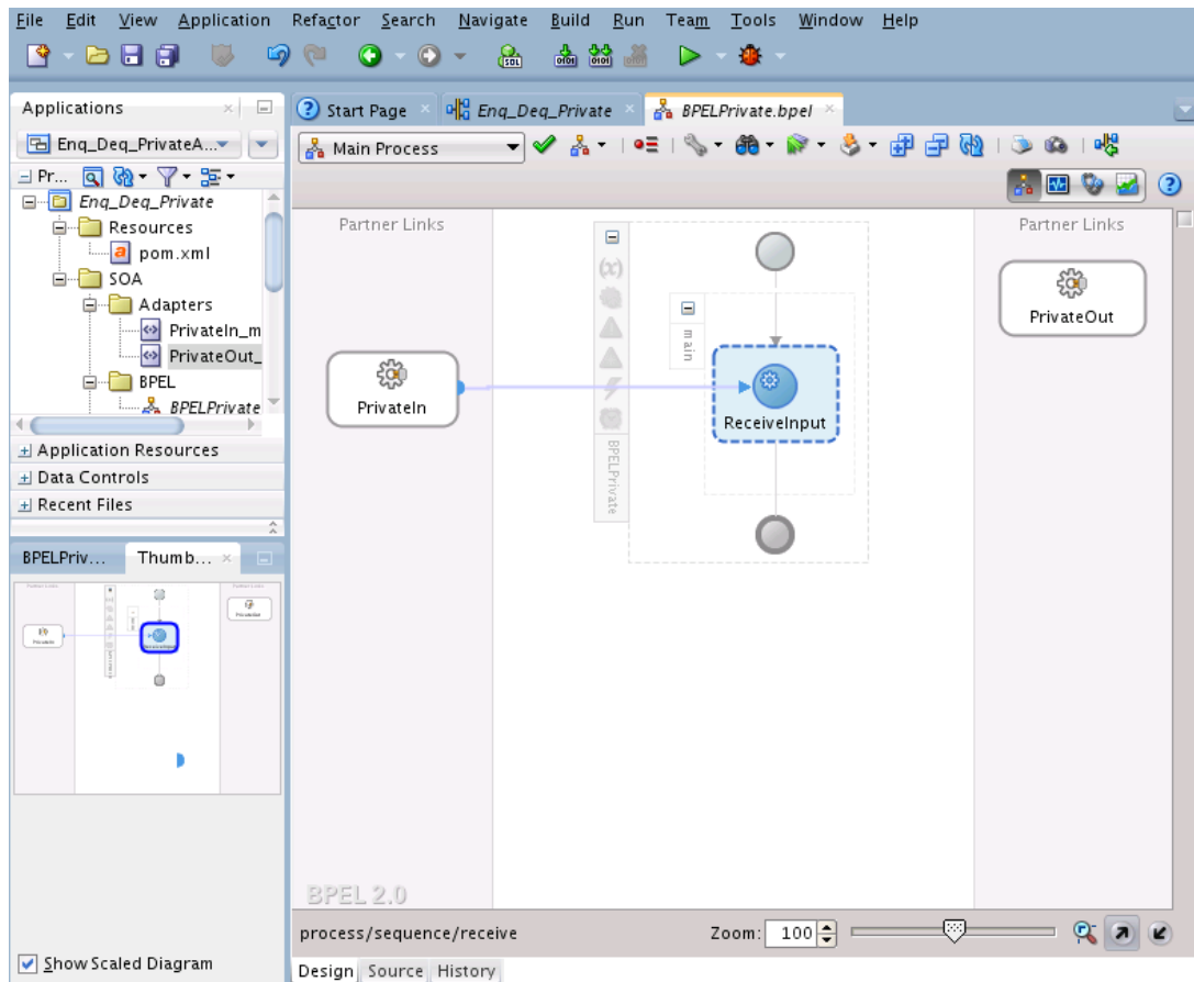
Figure 13-24 JDeveloper BPELPrivate.bpel Page Showing the PrivateIn Partner Link Wired to the Receive Activity
