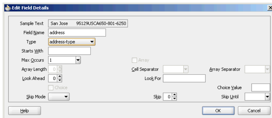
Figure 4-36 Edit Field Details Dialog
