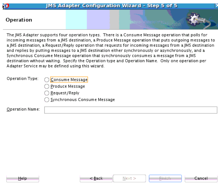
Figure 8-7 The Adapter Configuration Wizard - Operation Page
