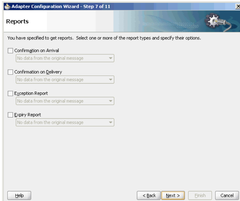
Figure 10-14 Reports Page
