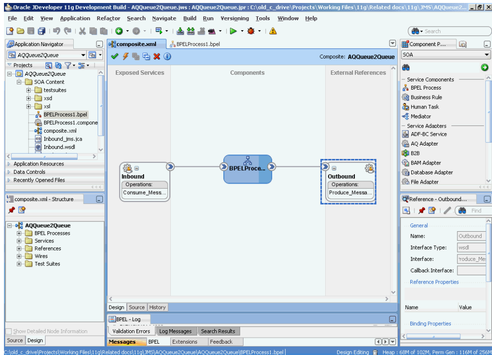
Figure 8-24 JDeveloper - Composite.xml
