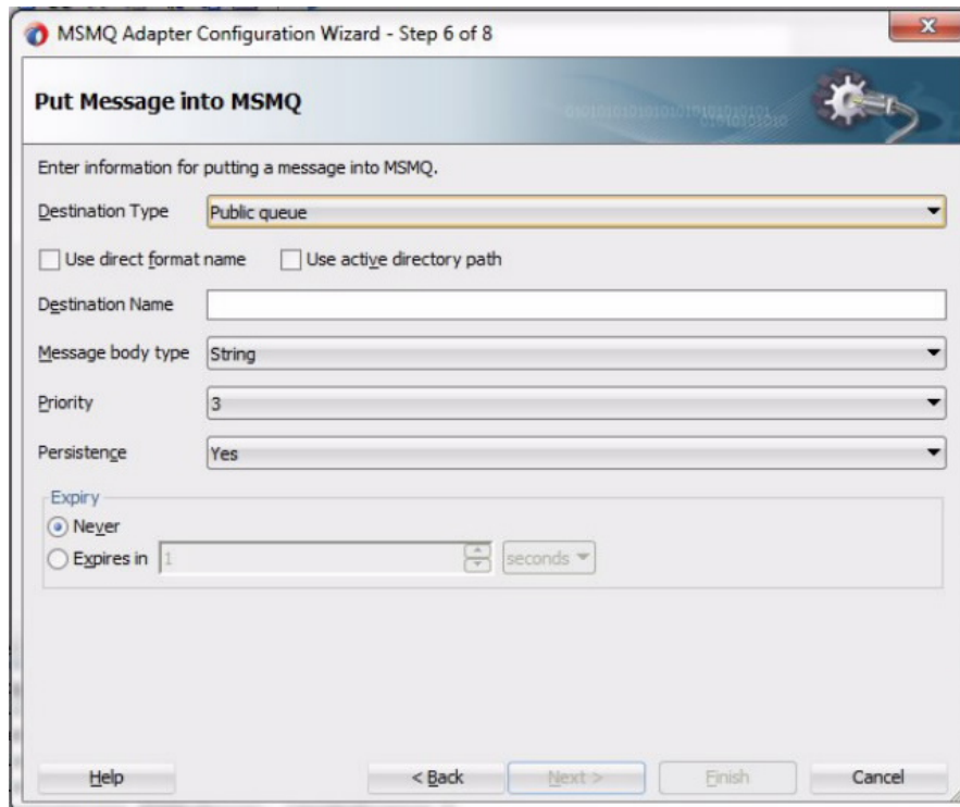
Figure 13-3 Enqueue Operation
