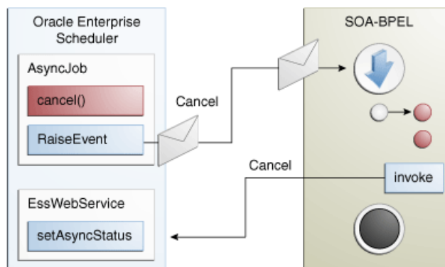
Figure 21-12 BPEL Handling Cancellation
