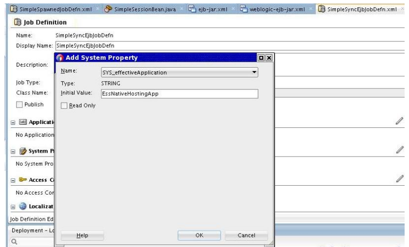
Figure 6-23 Add System Property Dialog
