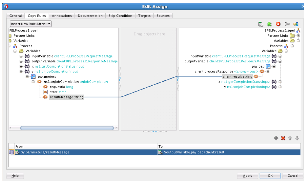
Figure 16-20 Map the onJobCompletion Component's Output Parameter resultMessage to the callbackClient Component's input Parameter result Variable
