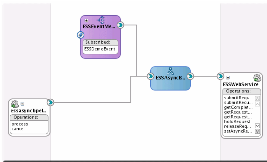
Figure 21-11 Composite with BPEL and ESSWebService
