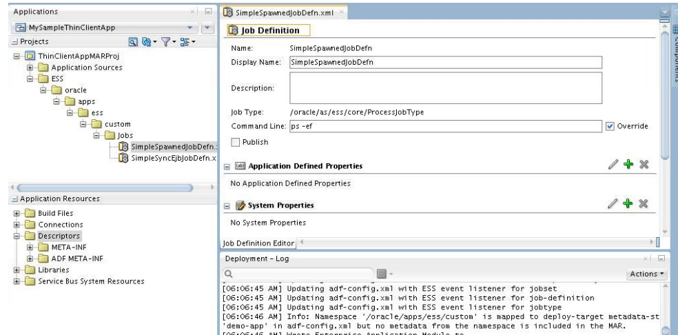
Figure 6-9 SimpleSpawnedJobDefn.xml Tab
