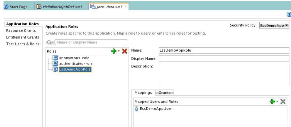
Figure 7-17 Configuring Security
