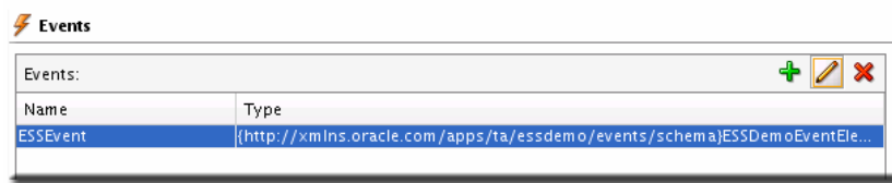
Figure 21-10 Events List
