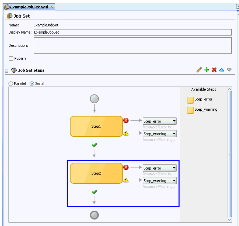
Figure 17-3 Job Set with Two Steps Added
