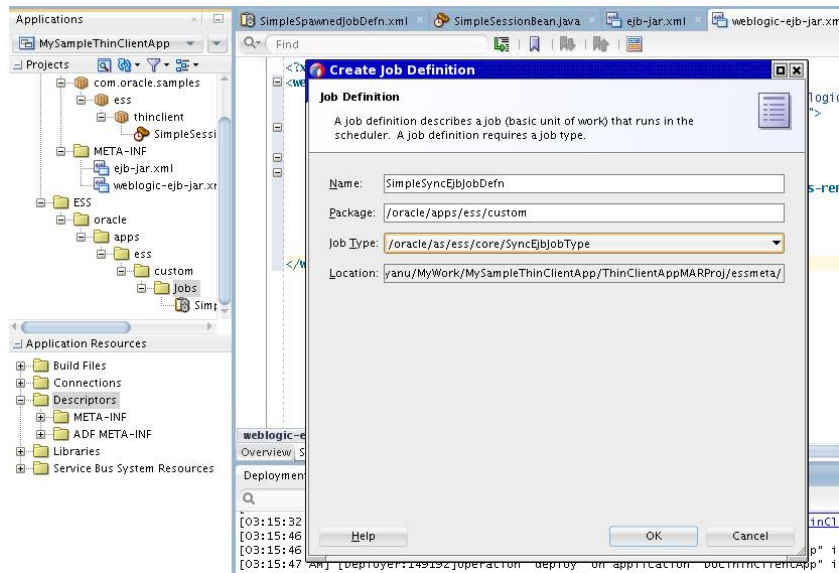
Figure 6-22 Create Job Definition Dialog
