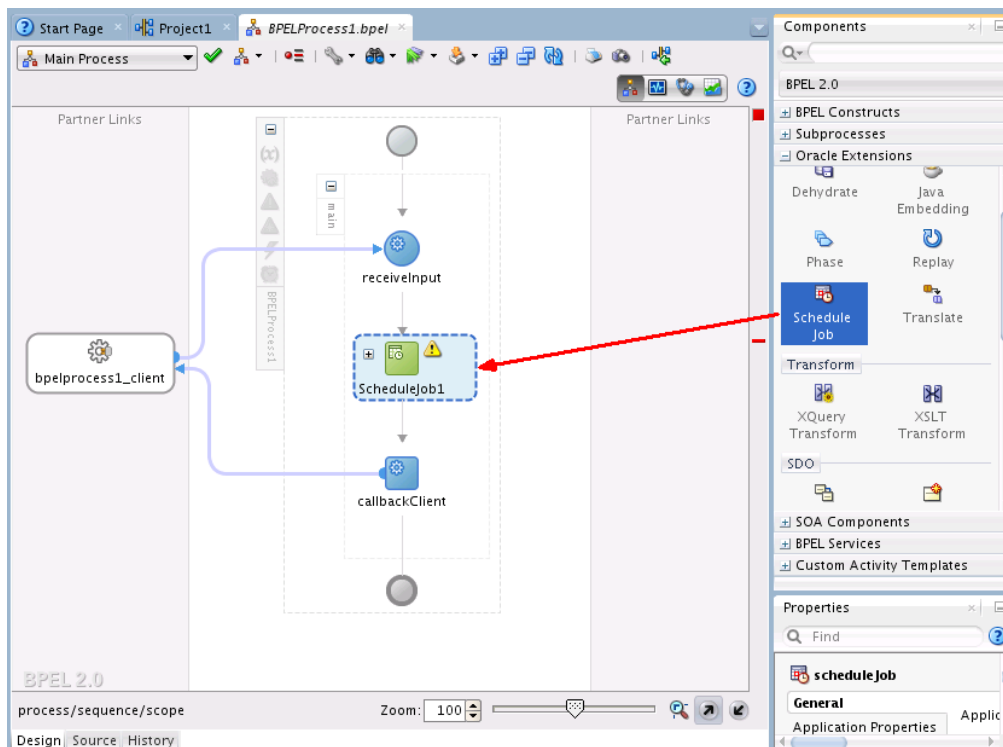
Figure 16-3 Adding the Schedule Job Component
