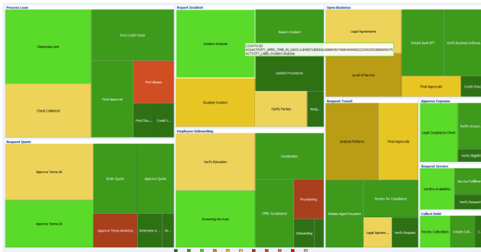
Figure 8-18 Treemap Example
