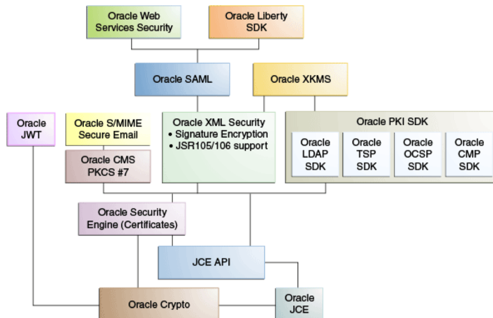
Figure 1-2 The Oracle Security Developer Tools
