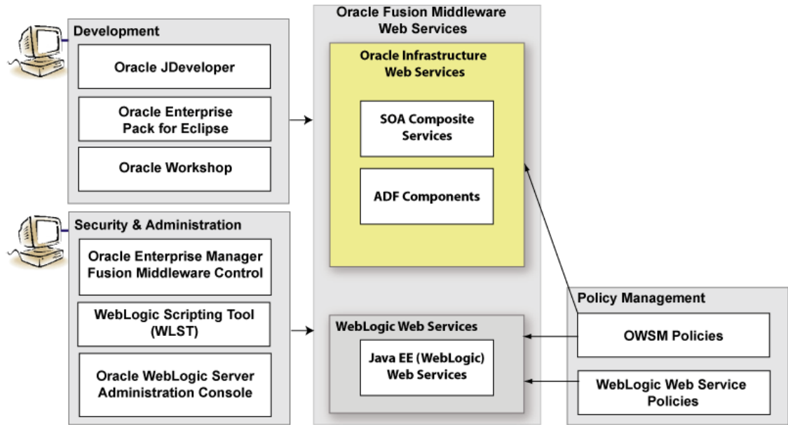
Figure 1-2 Web Services in Oracle Fusion Middleware 14c
