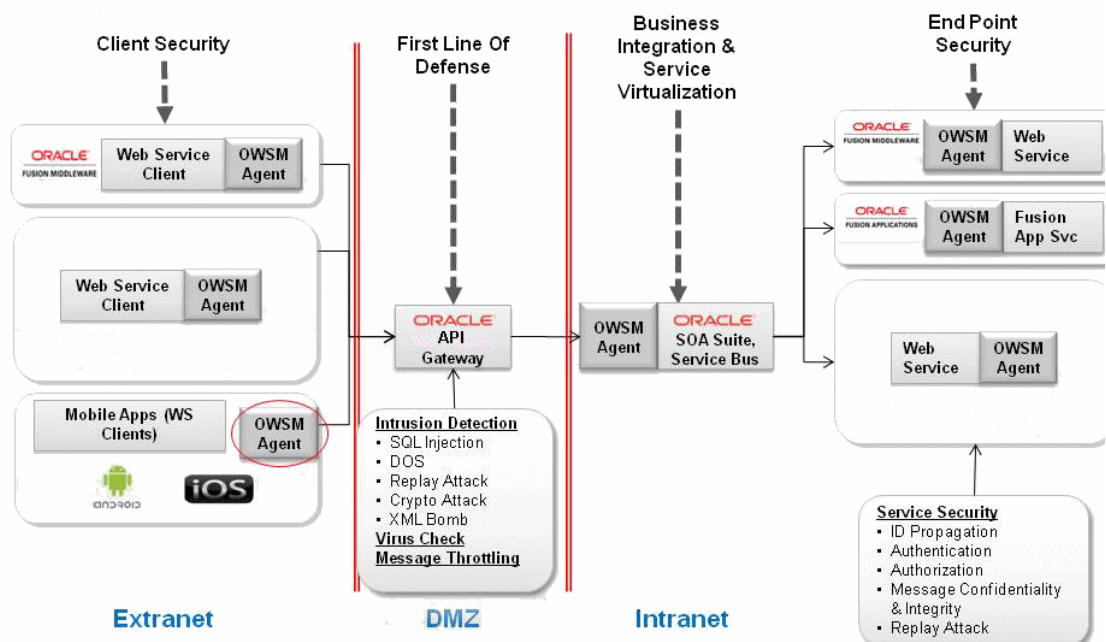
Figure 1-1 Security Provided by OWSM Agents
