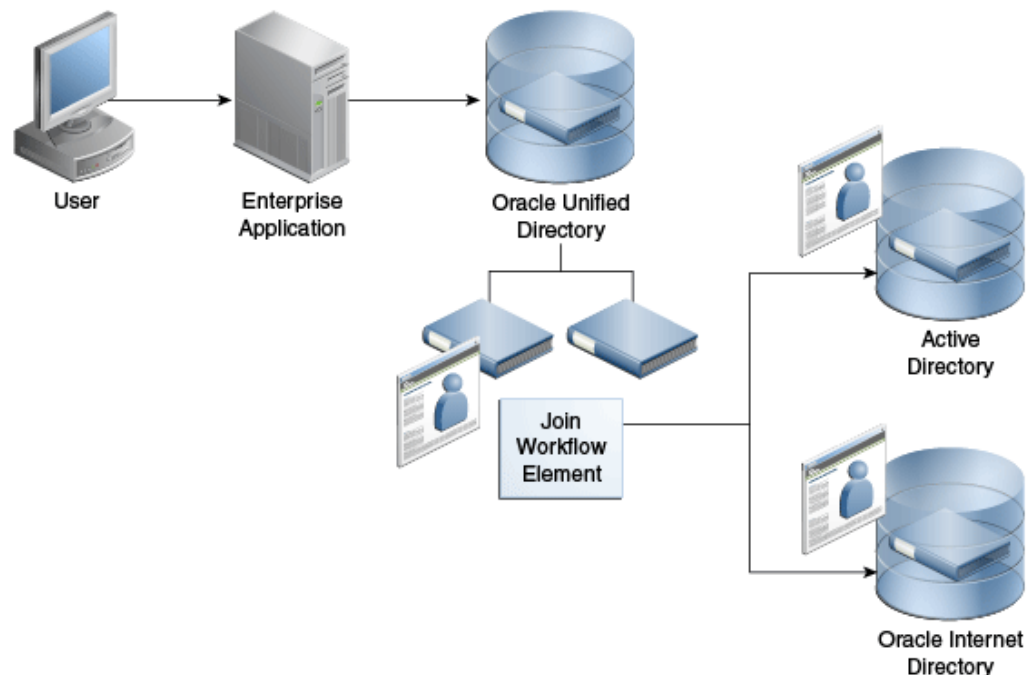
Figure 12-16 Sample One-to-One Joiner Type for Authentication
