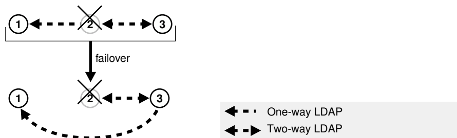
Figure 42-4 Failover Preserving Replica Type
