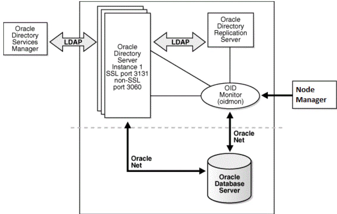
Figure 3-1 A Typical Oracle Internet Directory Node
