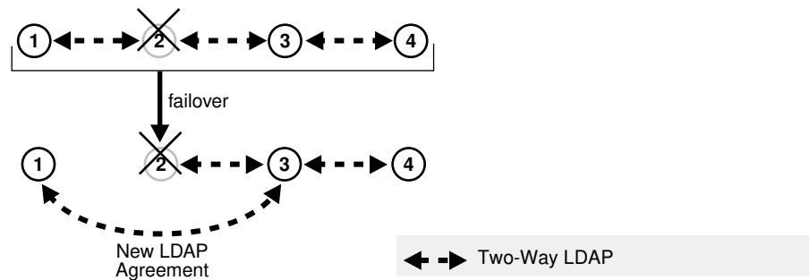
Figure 42-5 Compare and Reconcile All Connected Replicas
