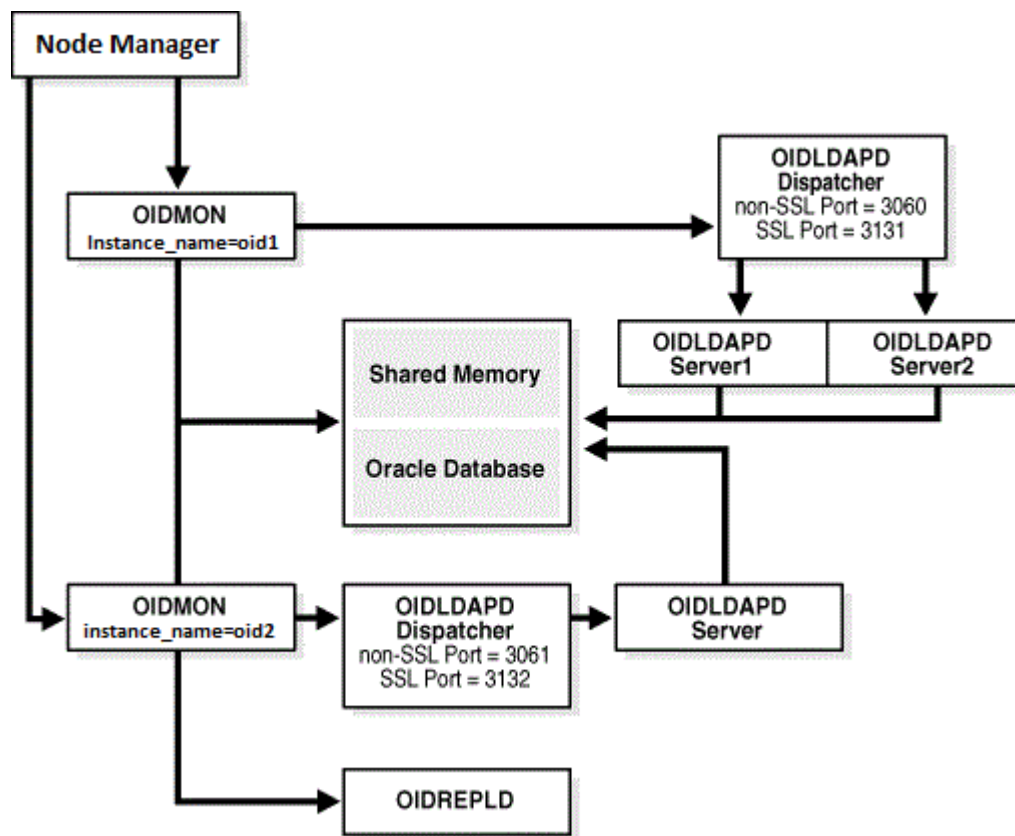
Figure 4-1 Oracle Internet Directory Process Control Architecture
