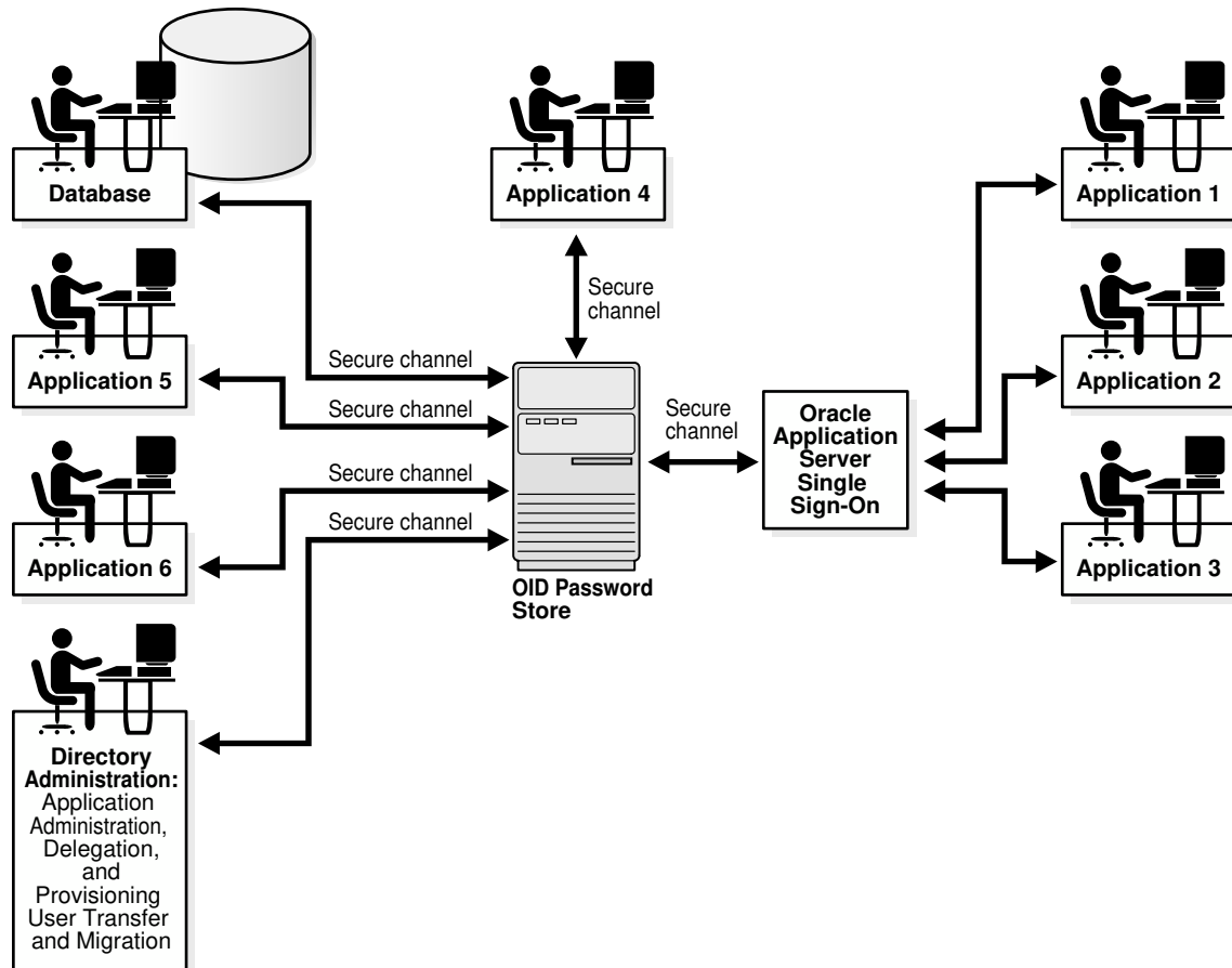
Figure 32-2 Authentication Model
