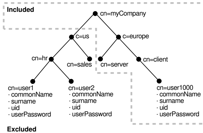
Figure 41-5 Naming Context Object #3
