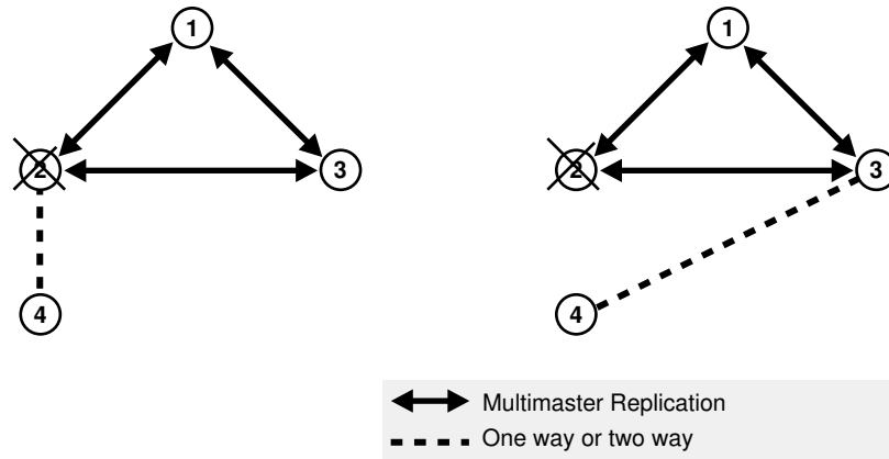
Figure 42-3 Old and New Suppliers in the Same Directory Replication Group
