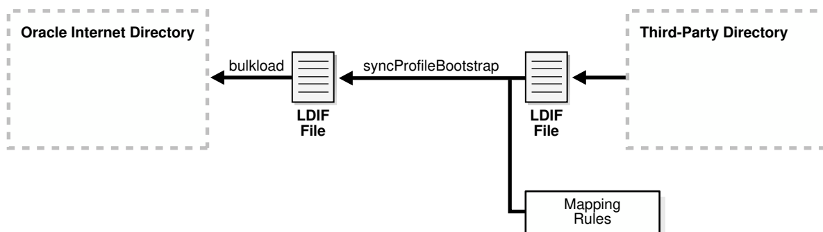
Figure 38-4 Using syncProfileBootstrap, bulkload, and LDIF Files
