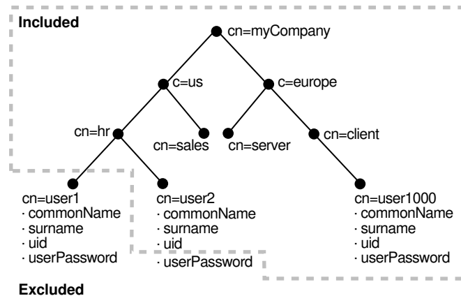
Figure 41-4 Result of Combining Naming Context Objects #1 and #2
