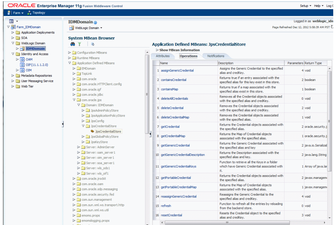
Figure A-4 getPortableCredential Operation
