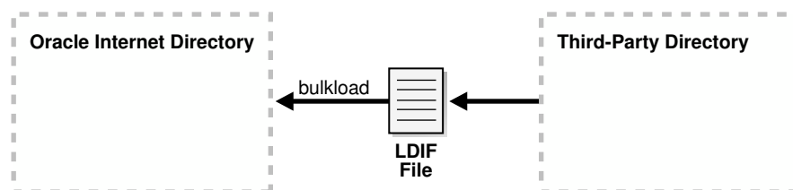
Figure 38-1 Using an LDIF File and Bulk Loader
