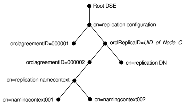
Figure 43-2 Example: Replication Configuration Entries for Node C
