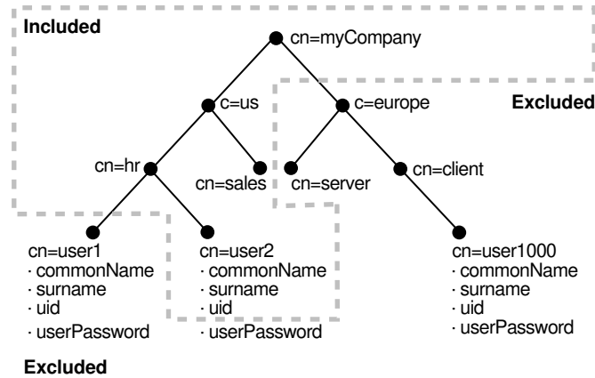
Figure 41-10 Naming Context Object #7
