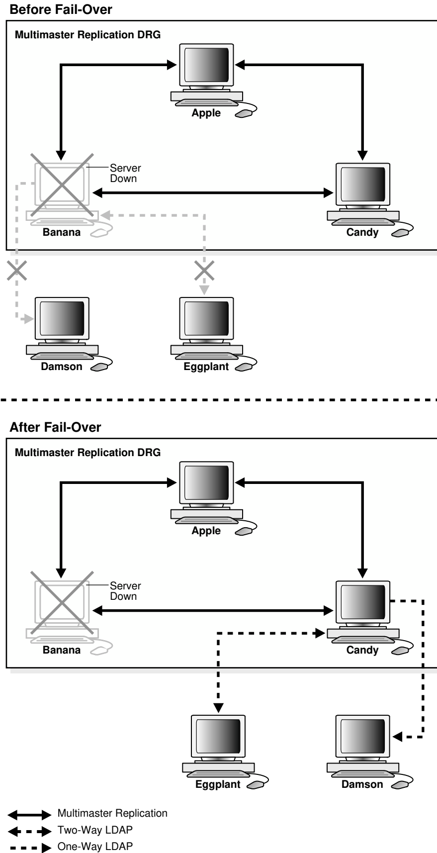
Figure 42-1 Replication Failover Scenario
