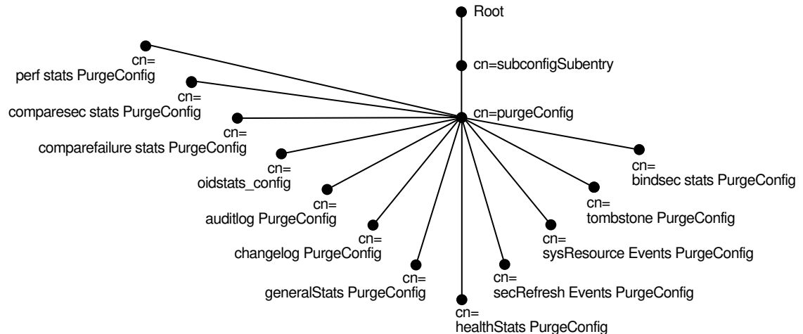
Figure 37-2 Garbage Collection Entries in the DIT
