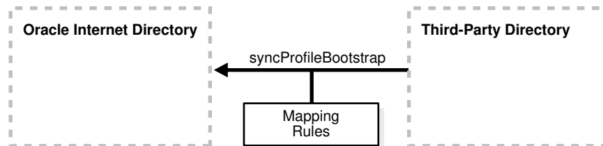
Figure 38-2 Using syncProfileBootstrap Directly
