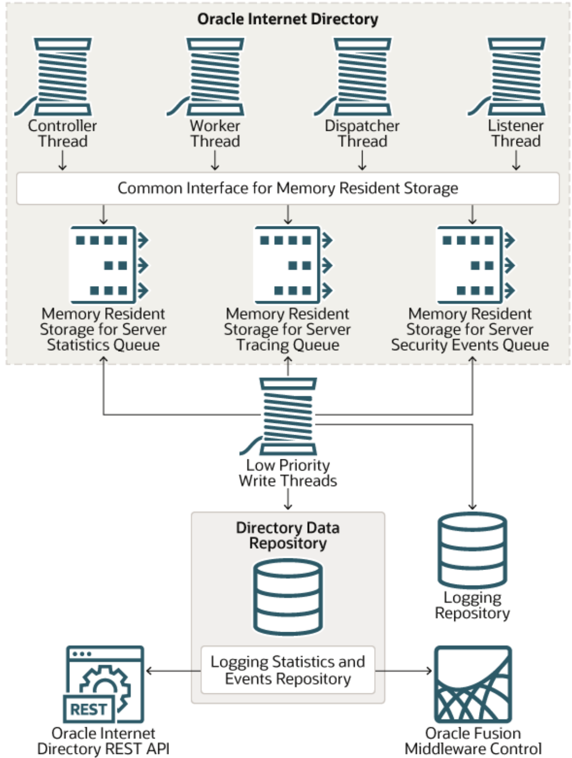
Figure 25-1 Architecture of Oracle Internet Directory Server Manageability
