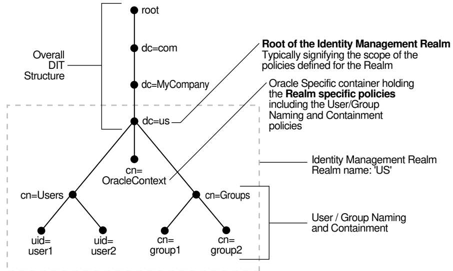
Figure 35-1 Example of an Identity Management Realm
