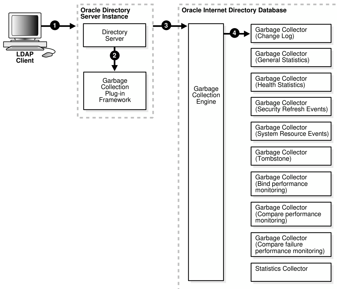
Figure 37-1 Example: Garbage Collection of Change Log Entries
