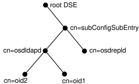
Figure 8-1 DIT Showing Two Instance-Specific Configuration Entries
