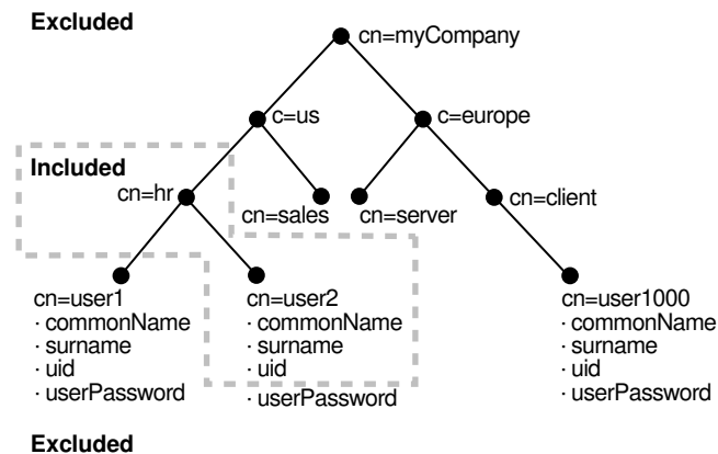
Figure 41-9 Naming Context Object #6
