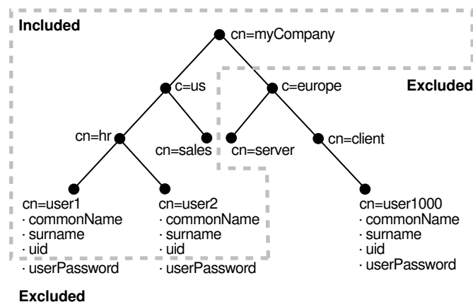
Figure 41-8 Naming Context Object #5
