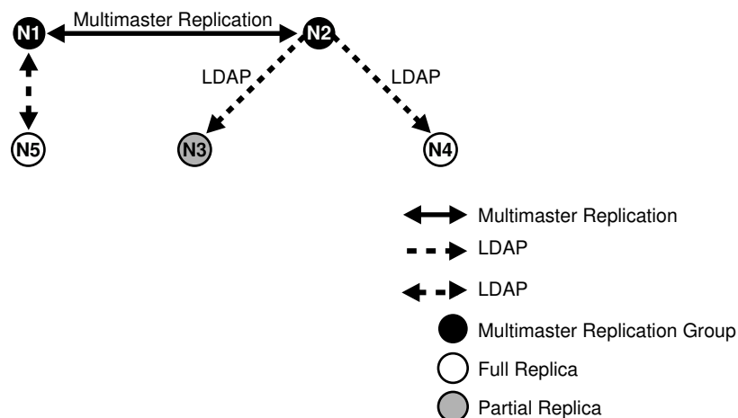
Figure 41-11 Example of Fan-Out Replication
