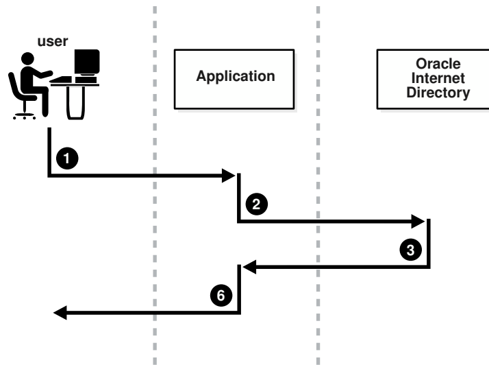
Figure 32-3 How Password Verification Works
