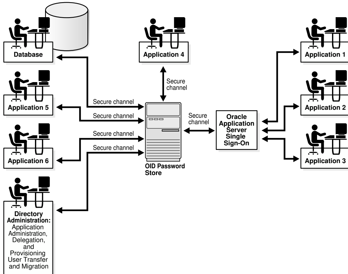
Figure 32-2 Authentication Model
