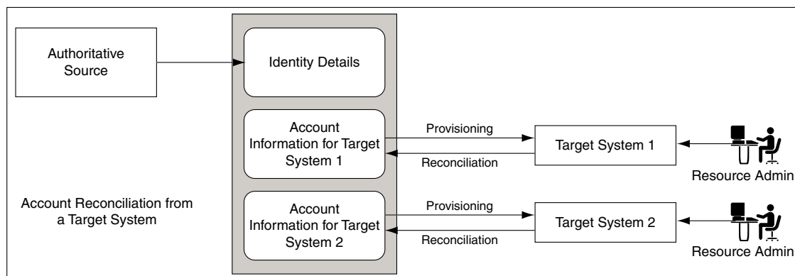
Figure 11-3 Account Reconciliation From a Target System
