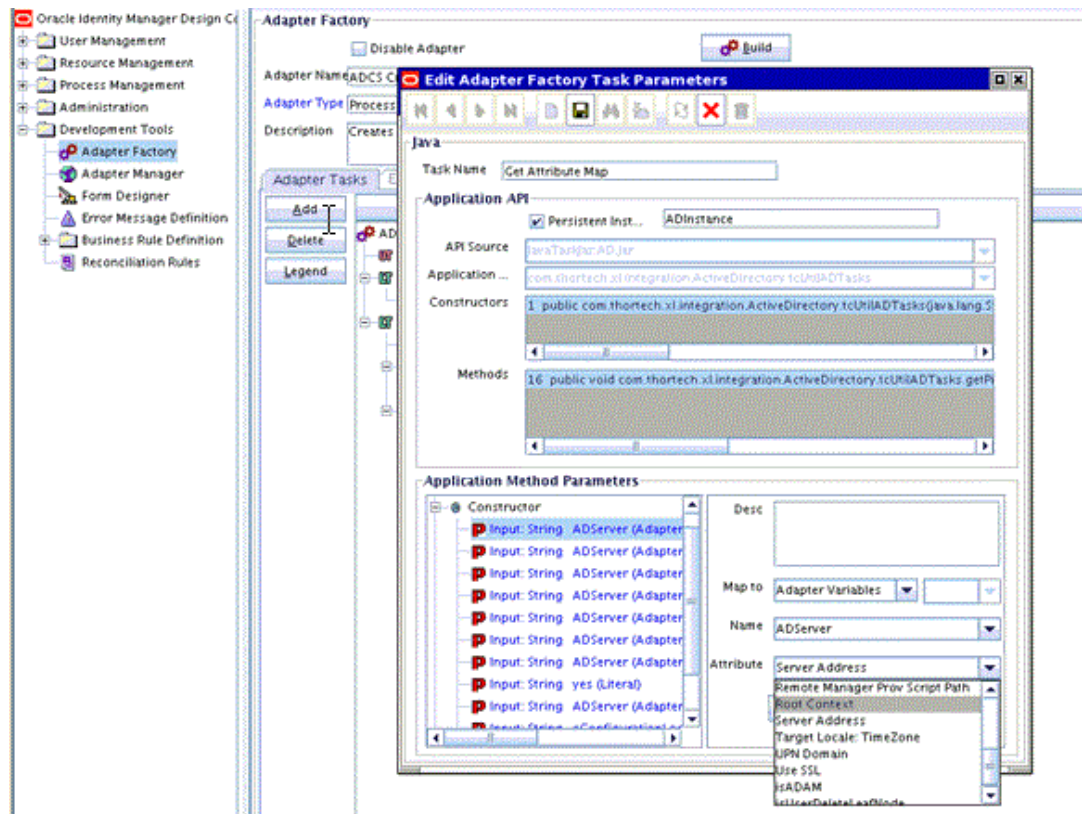
Figure 10-4 The Edit Adapter Factory Task Parameters Dialog Box
