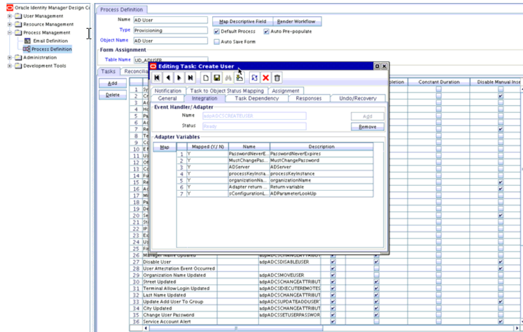
Figure 10-5 The Integration Tab of the Editing Task Dialog Box
