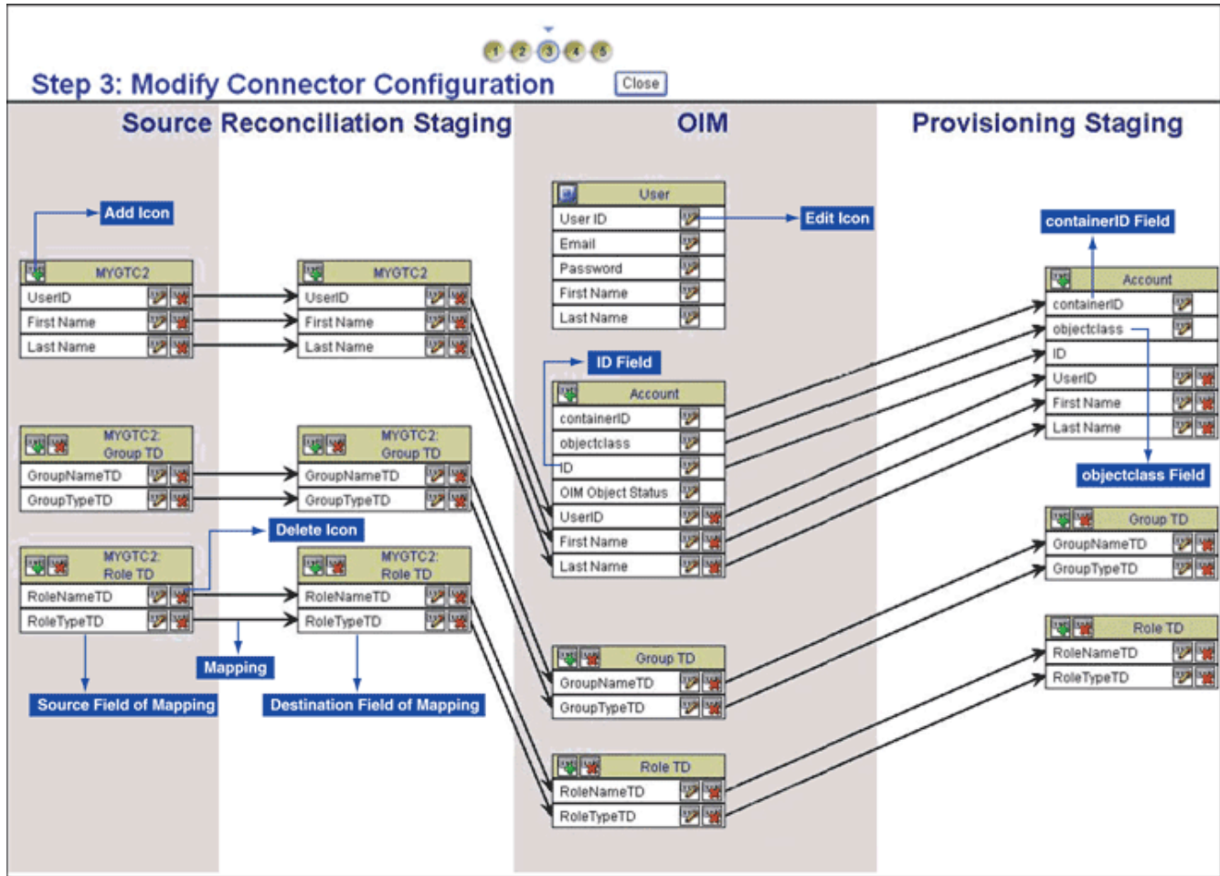
Figure 8-1 Step 3: Modify Connector Configuration Page
