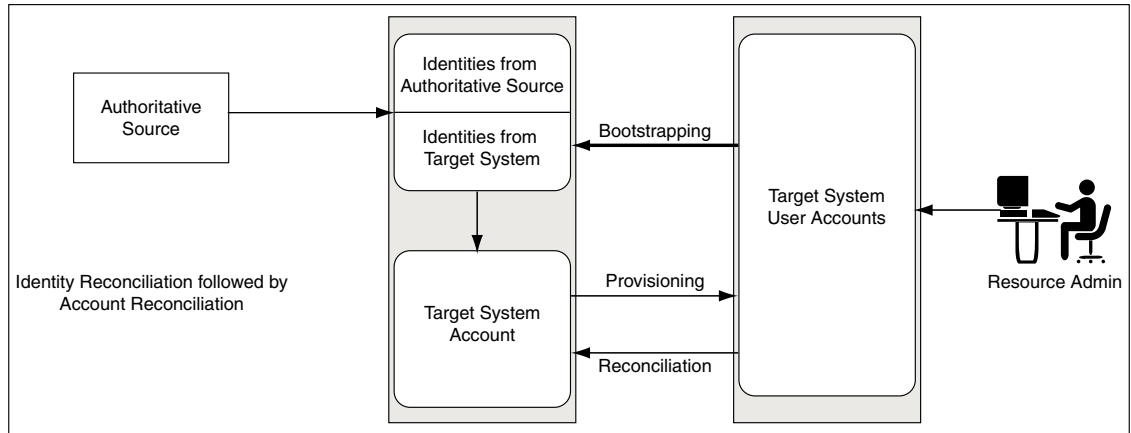
Figure 11-4 Identity and Account Reconciliation
