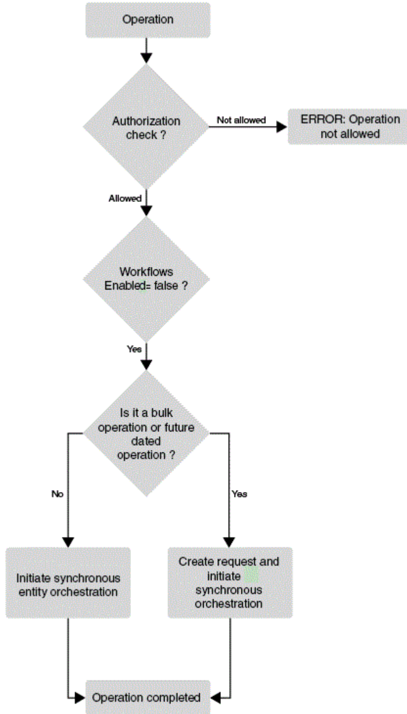
Figure 4-7 Disabled Workflows
