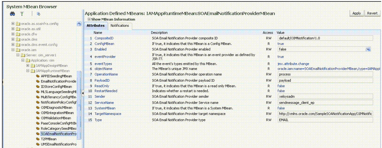
Figure 18-4 SOAEmailNotificationProviderMBean Properties
