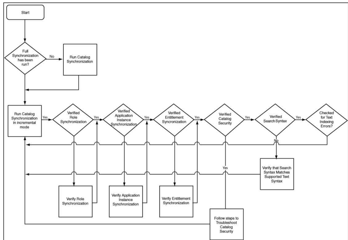
Figure 12-7 Catalog Search
