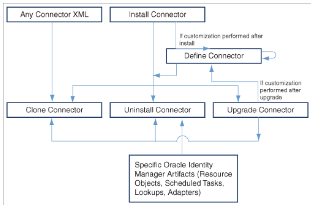
Figure 10-1 Connector Lifecycle
