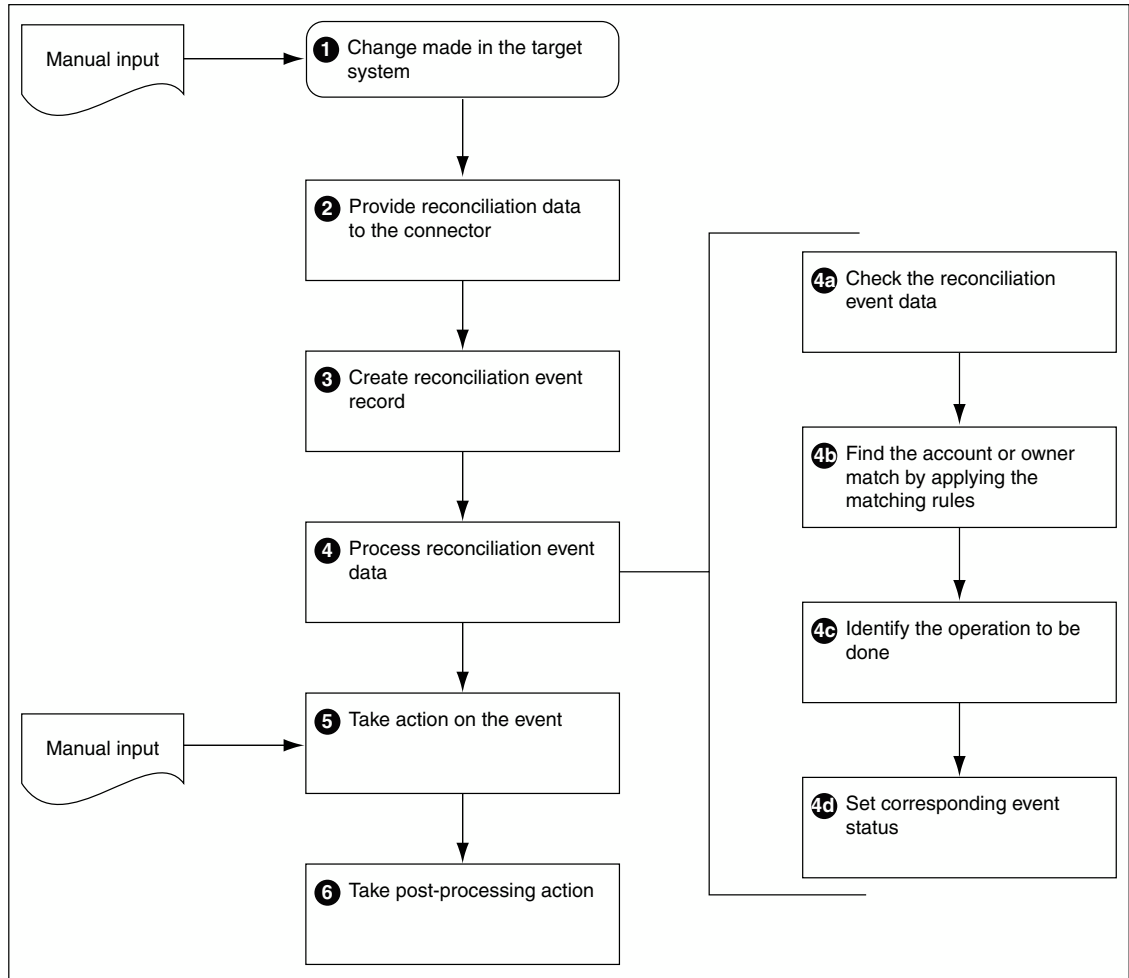
Figure 11-5 Reconciliation Process Flow
