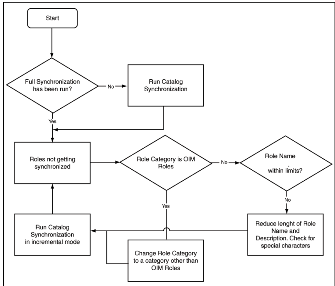
Figure 12-3 Catalog Synchronization Diagnostic Flowchart
