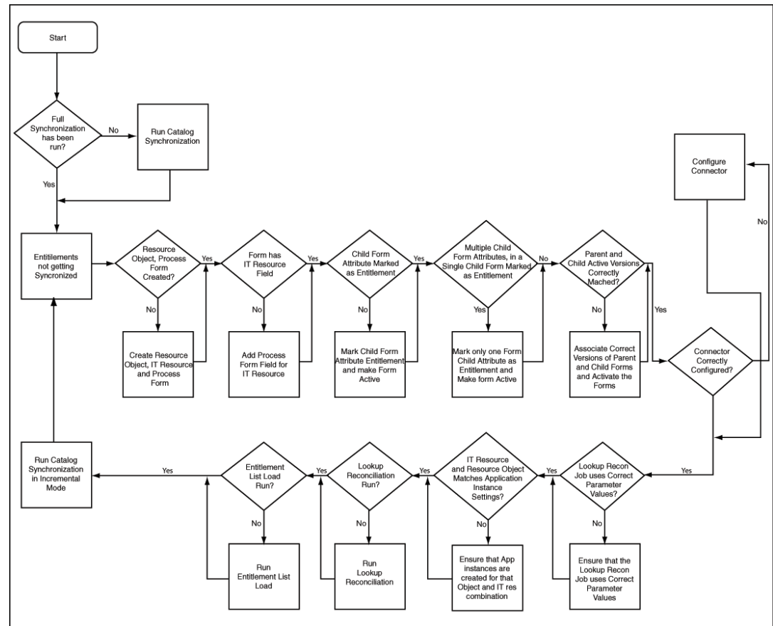
Figure 12-5 Troubleshooting Synchronizing Entitlements Flowchart
