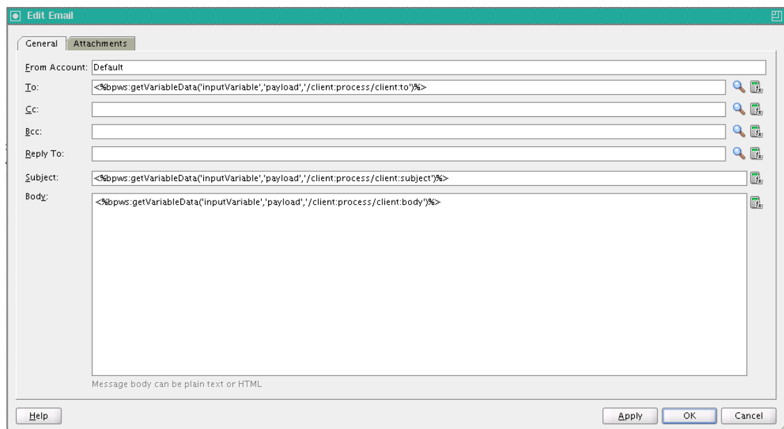
Figure 18-3 Sample Mapping of Composite Payload
