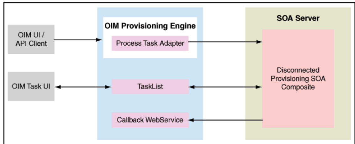
Figure 9-2 Disconnected Resource Architecture
