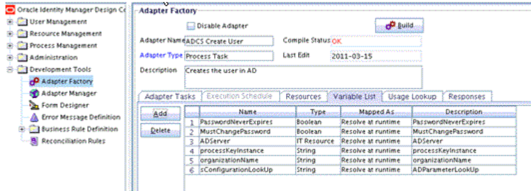
Figure 10-3 The Variable List Tab of the Adapter Factory Form
