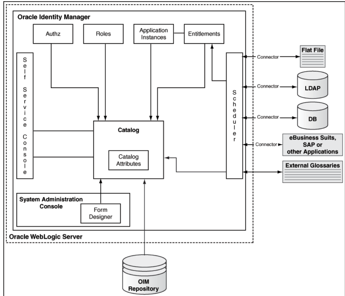
Figure 12-1 High-Level Catalog Architecture
