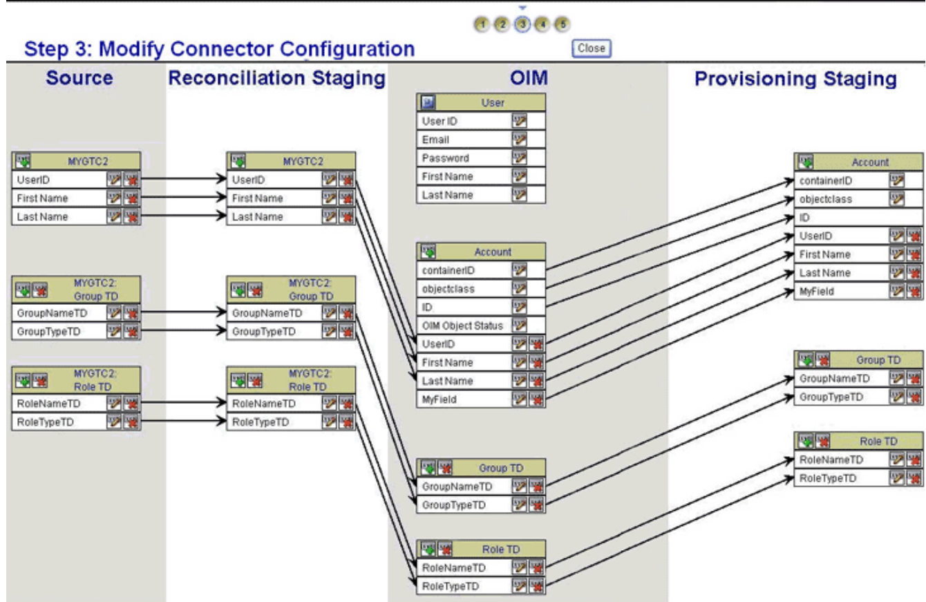
Figure 8-2 Step 3: Modify Connector Configuration Page After Addition of a Field
