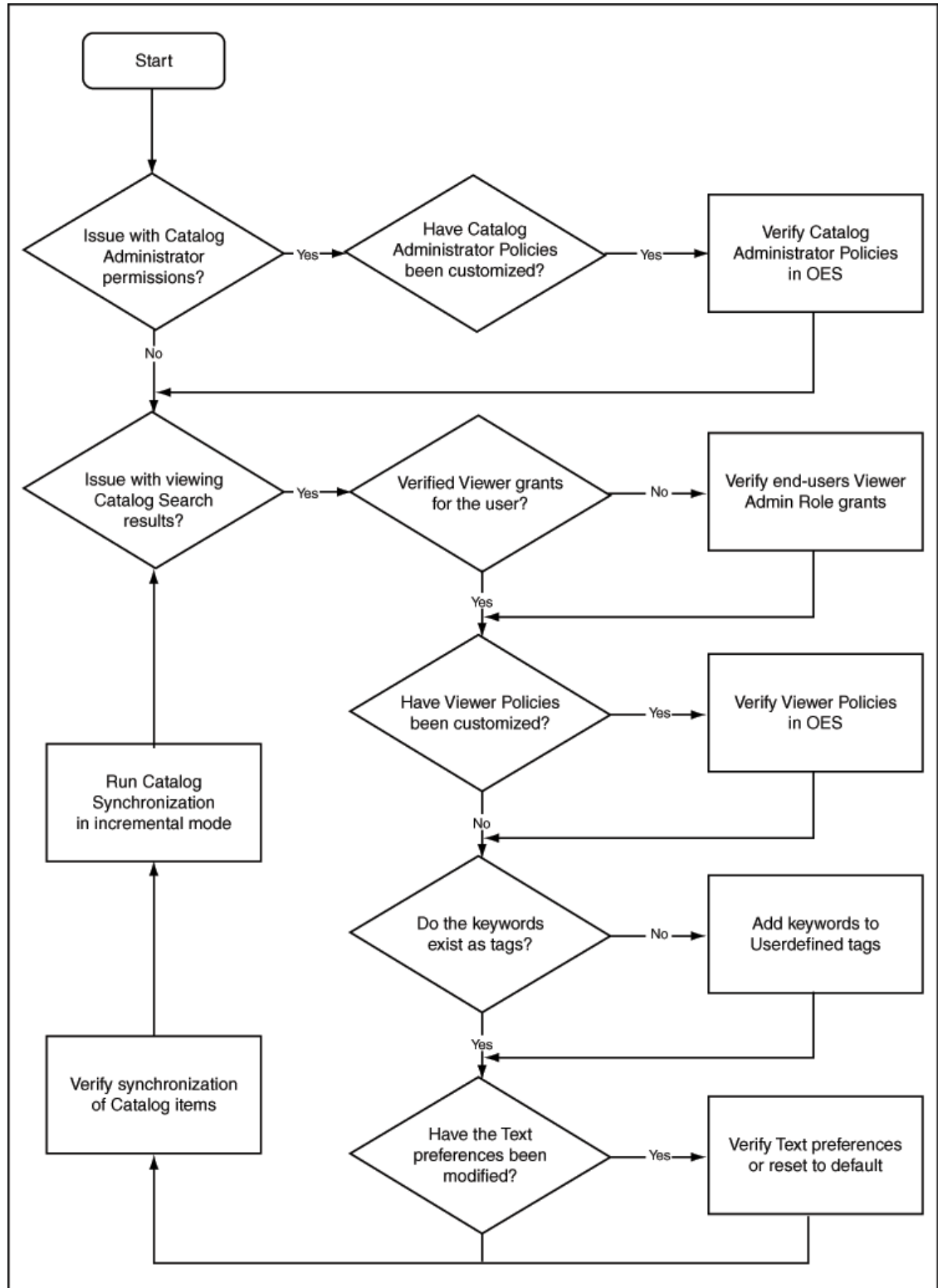
Figure 12-6 Diagnostic Flowchart With Security Issues
