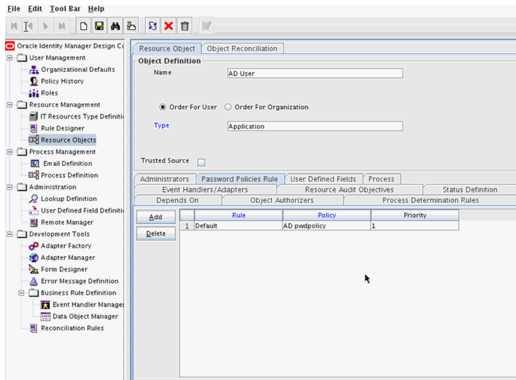
Figure 9-1 Attach Password Policy to Application Instance
