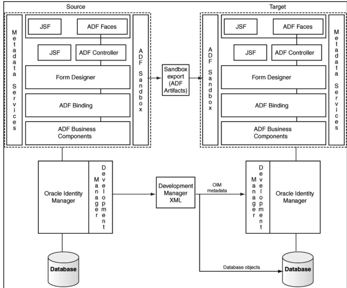
Figure 12-2 Test to Production Process for Catalog
