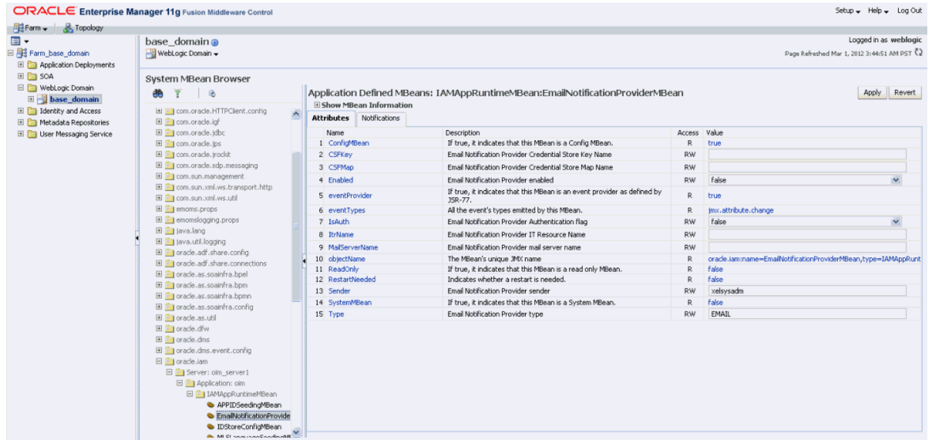
Figure 18-2 EmailNotificationProviderMBean Properties
