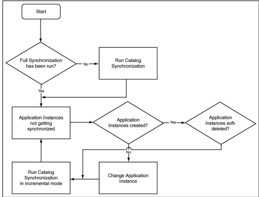
Figure 12-4 Trouble Shooting Synchronization Application Instances Flowchart
