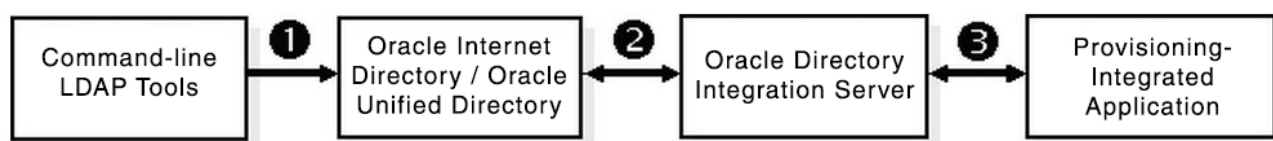
Figure 15-2 Asynchronous Provisioning using Command-Line LDAP Tools
