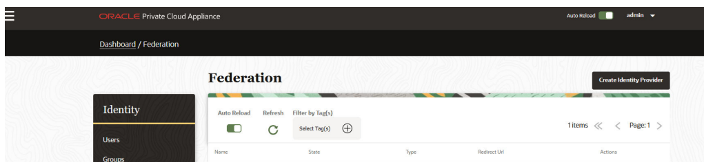
Figure 54-3 Create IDP
