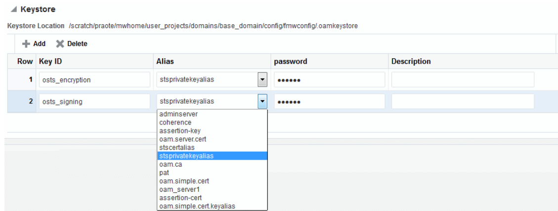
Figure 32-2 Keystore Settings
