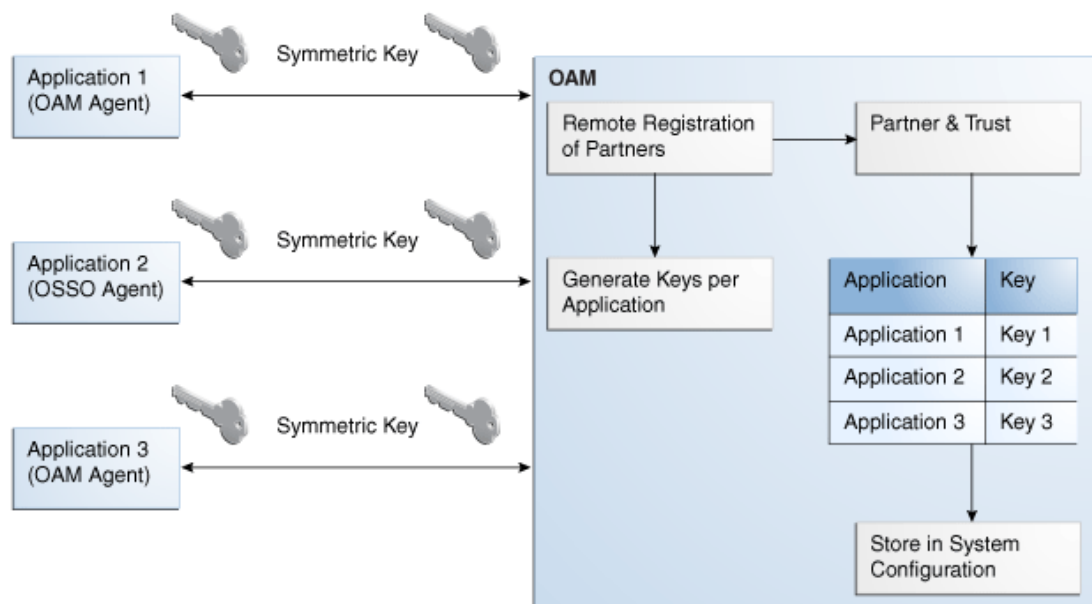
Figure 15-5 Key Generation
