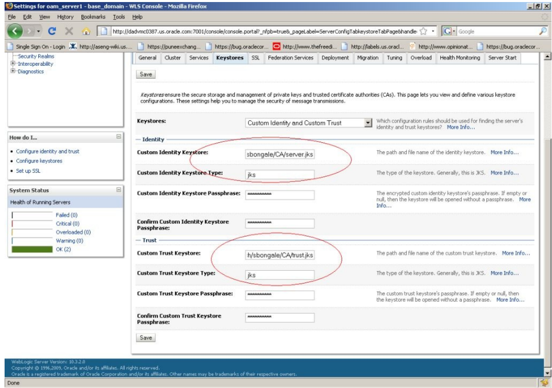
Figure 23-6 Keystore Configuration
