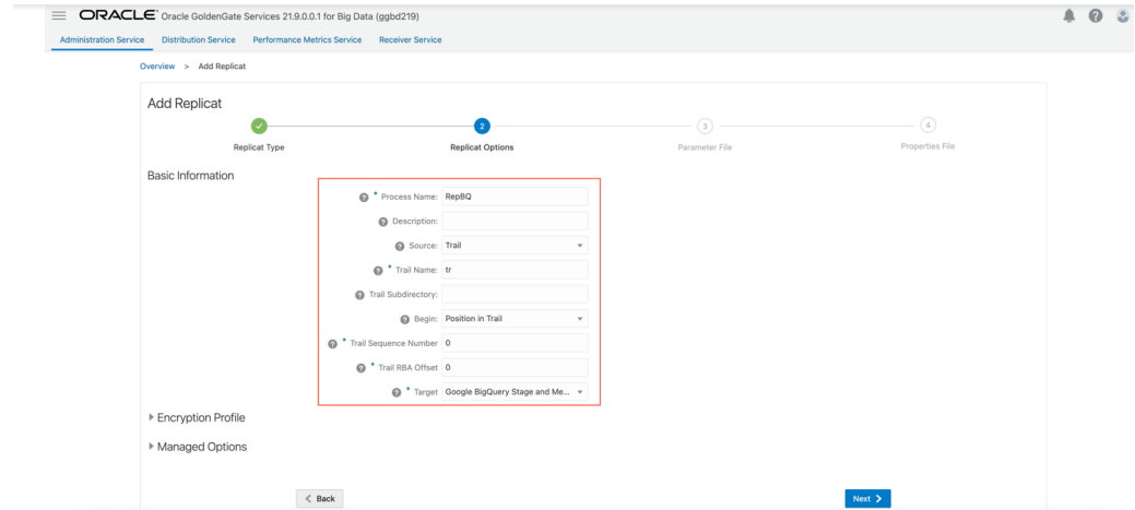
Figure 7-4 Process Name, Trail Name, and Target Names
