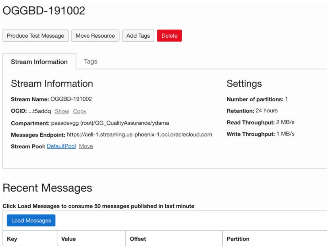
Figure 8-2 Example OSS Panel showing DefaultPool
