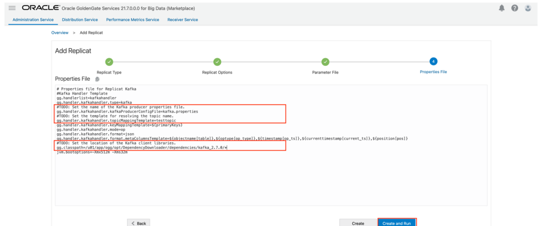
Figure 7-24 Properties file updates.
