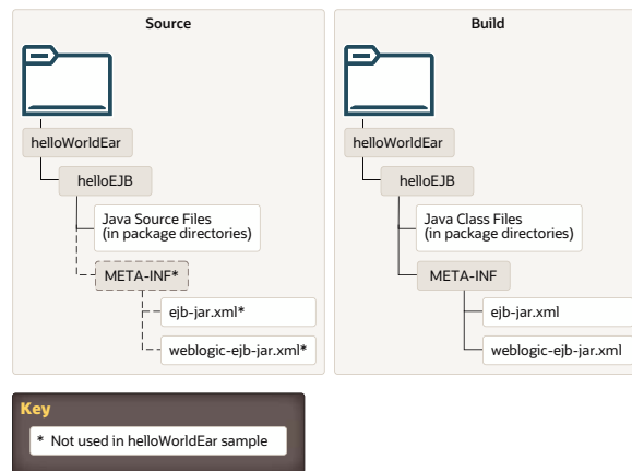
Figure 4-4 Enterprise Application Source Directory
