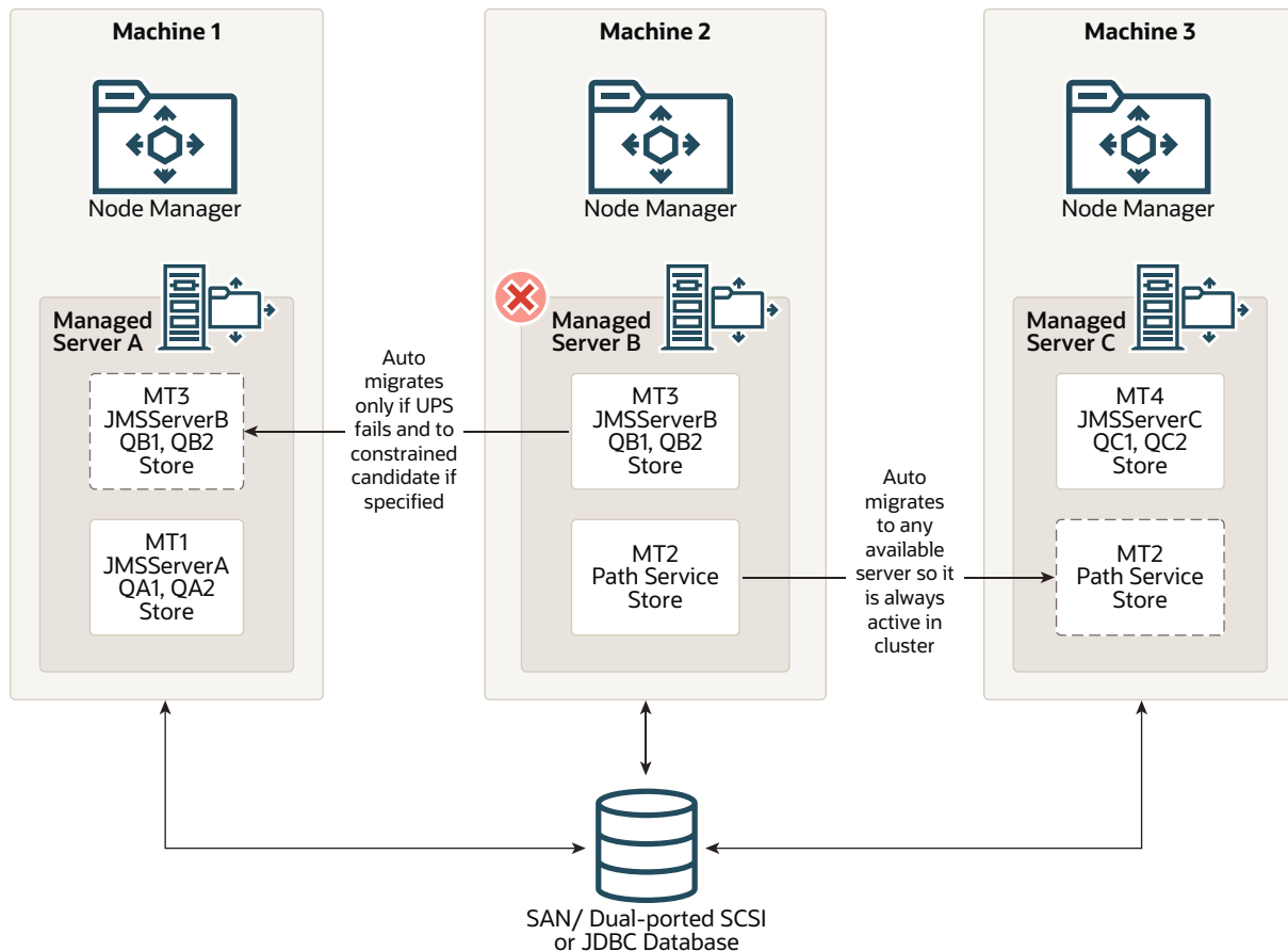
Figure 7-1 Migratable Targets In a Cluster
