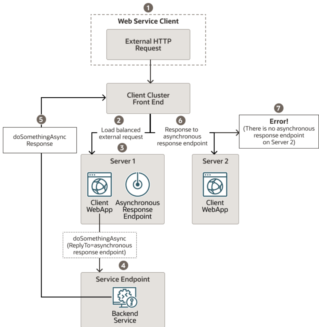
Figure 12-3 Clustering Scenario Resulting in an Error
