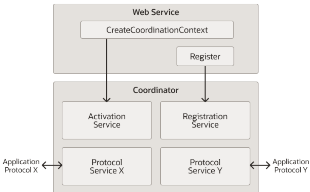
Figure 15-1 Web Services Atomic Transactions Framework
