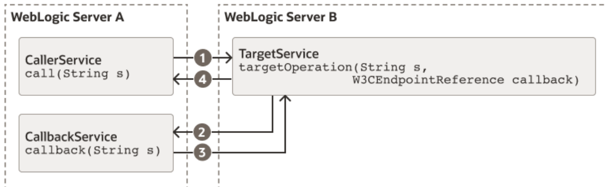
Figure 26-1 Example Callback Implementation
