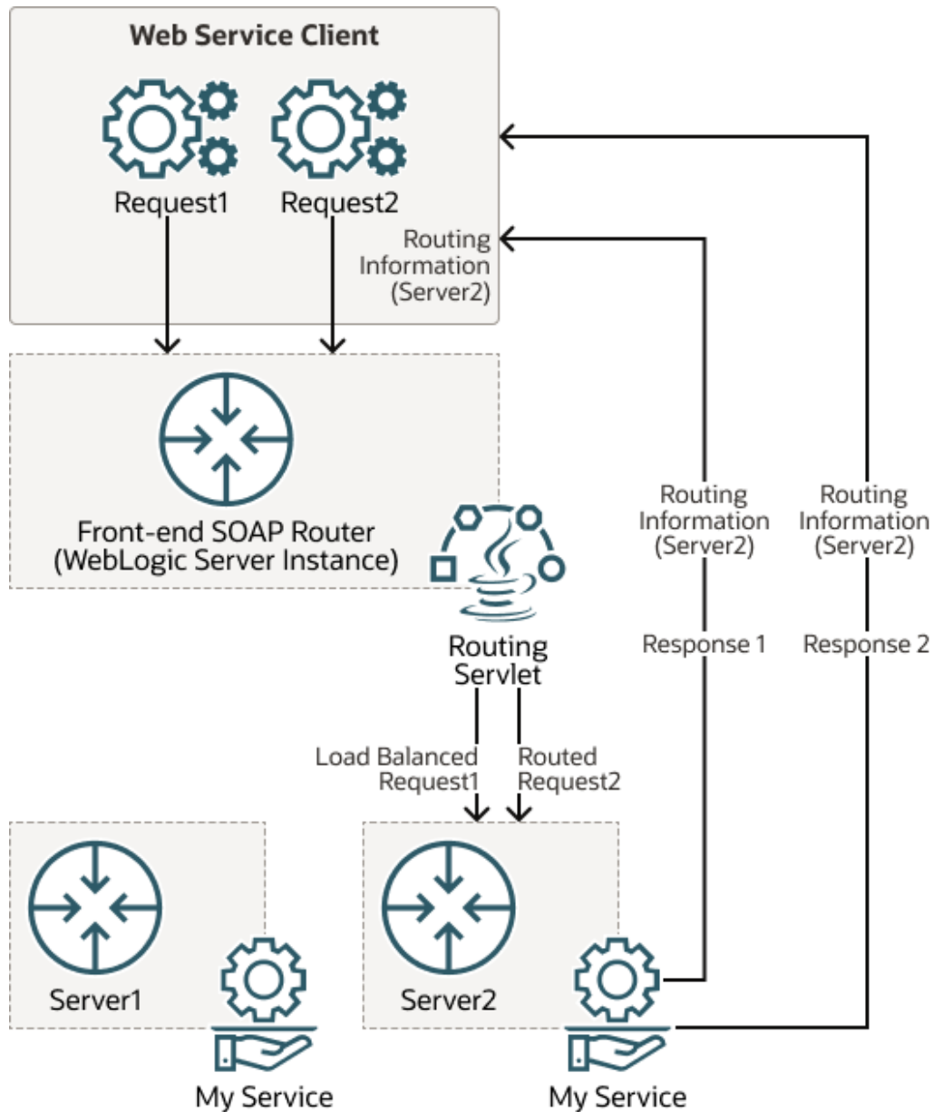
Figure 23-2 Routing Web Service Requests to a Single Server
