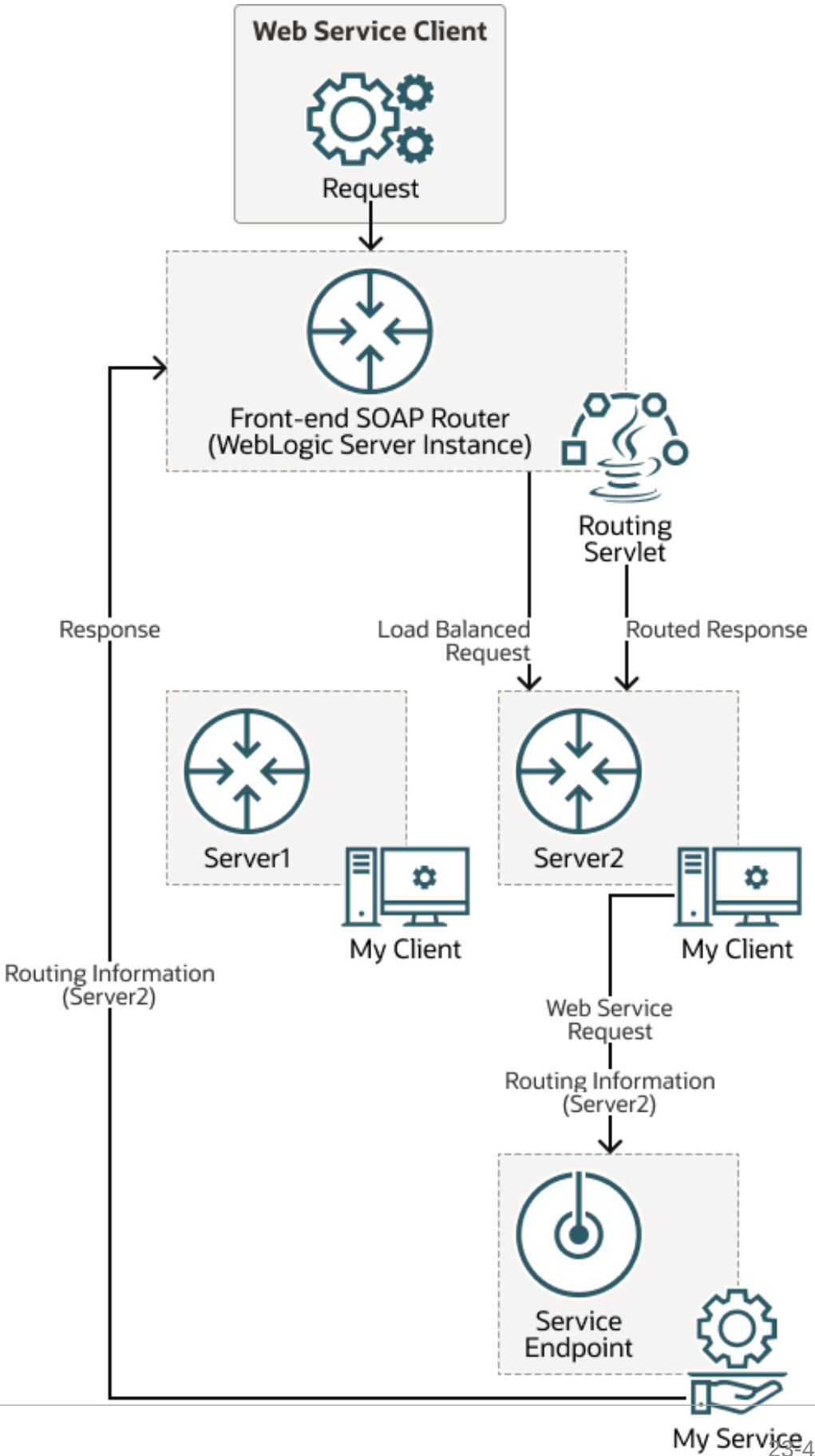
Figure 23-1 Routing a Web Service Response to a Single Server
