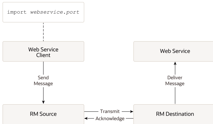
Figure 14-1 Web Service Reliable Message Exchange
