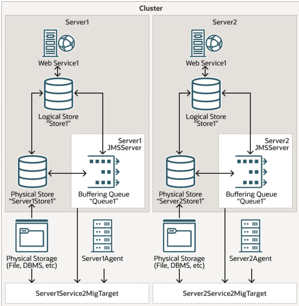
Figure 21-2 Example of a Two-Node Cluster Configuration (Before Migration)
