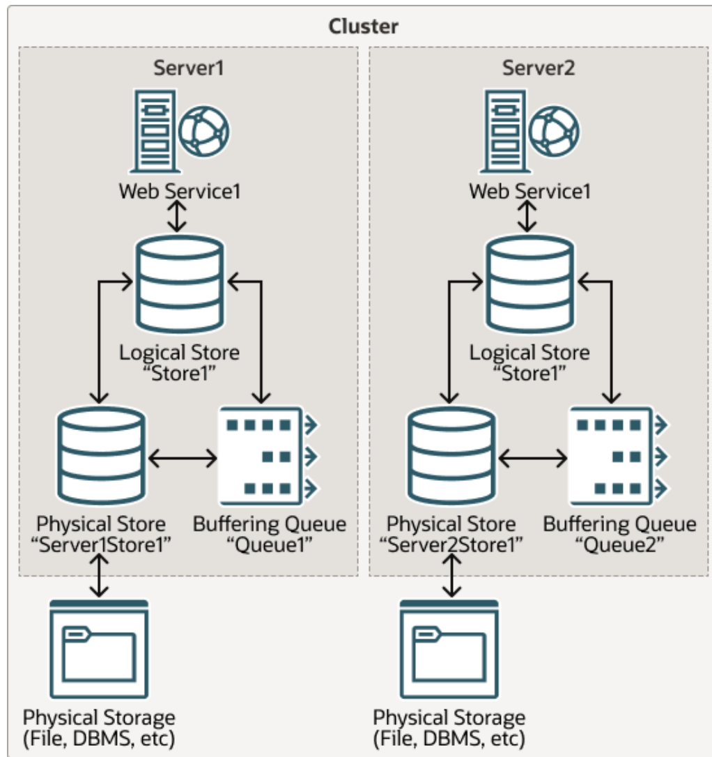
Figure 21-1 Example Web Service Persistence Configuration
