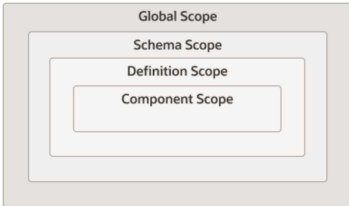
Figure 5-2 Scopes for Custom Binding Declarations
