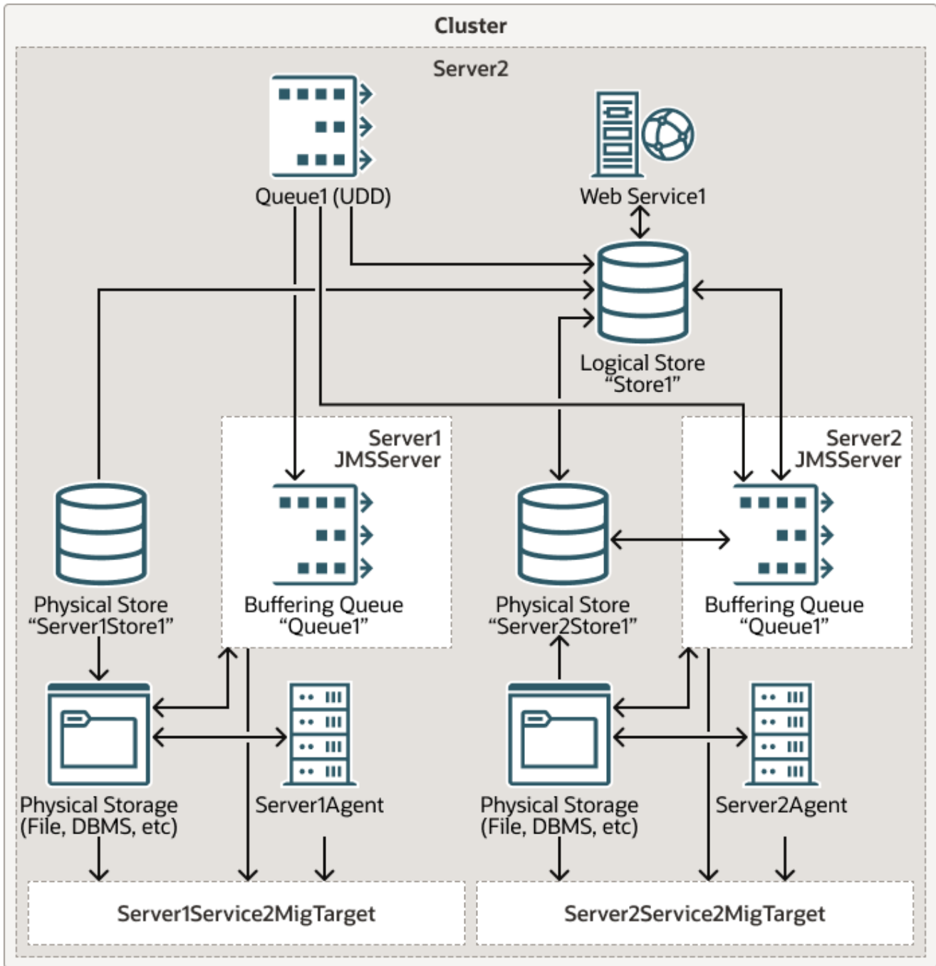
Figure 21-3 Example of a Two-Node Cluster Configuration (After Migration)
