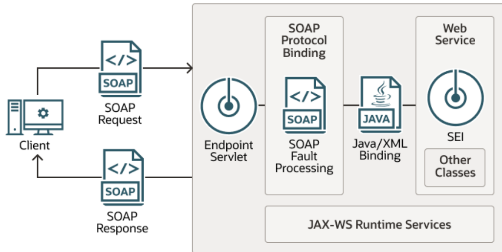
Figure 19-1 How SOAP Faults Are Processed
