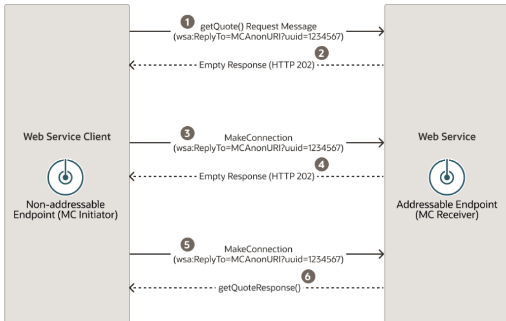
Figure 12-2 Make Connection Message Flow
