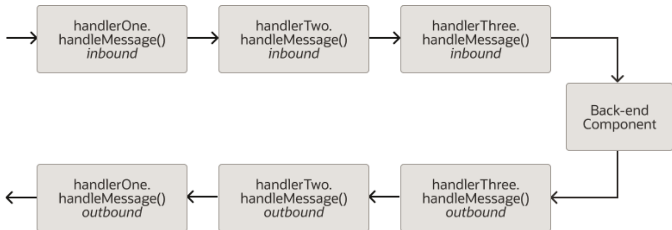
Figure 18-1 Order of Execution of Handler Methods
