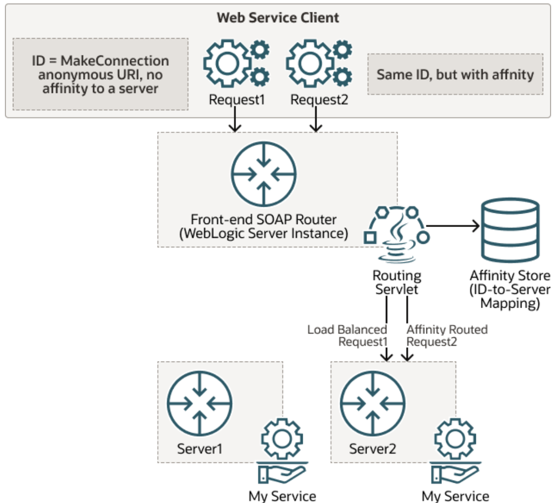
Figure 23-3 Routing Web Service Requests to a Single Server Using an ID
