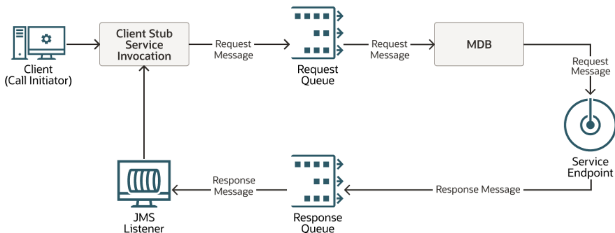
Figure 17-1 Web Service Invocation Using SOAP Over JMS Transport
