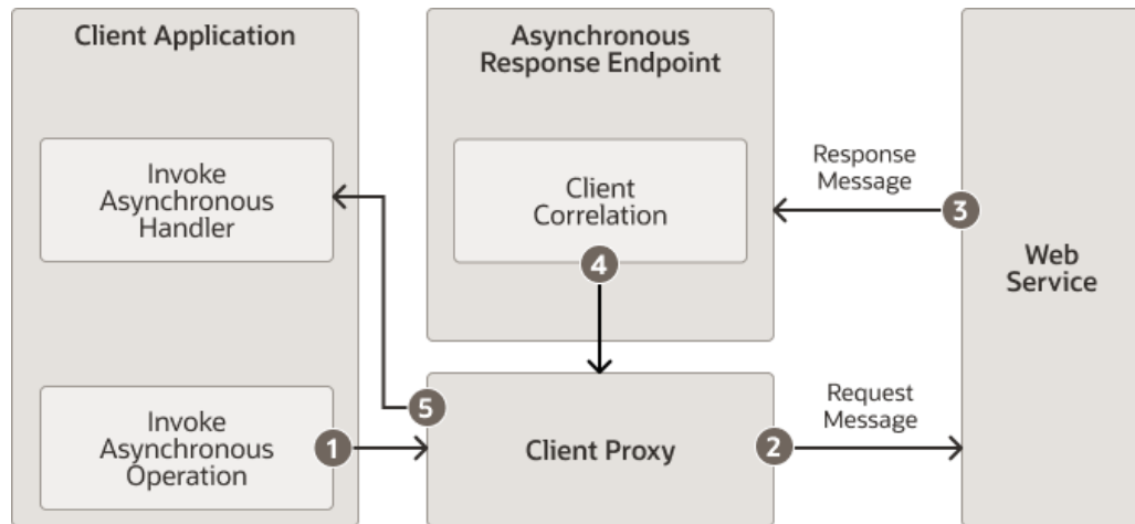
Figure 12-1 Asynchronous Client Transport Feature
