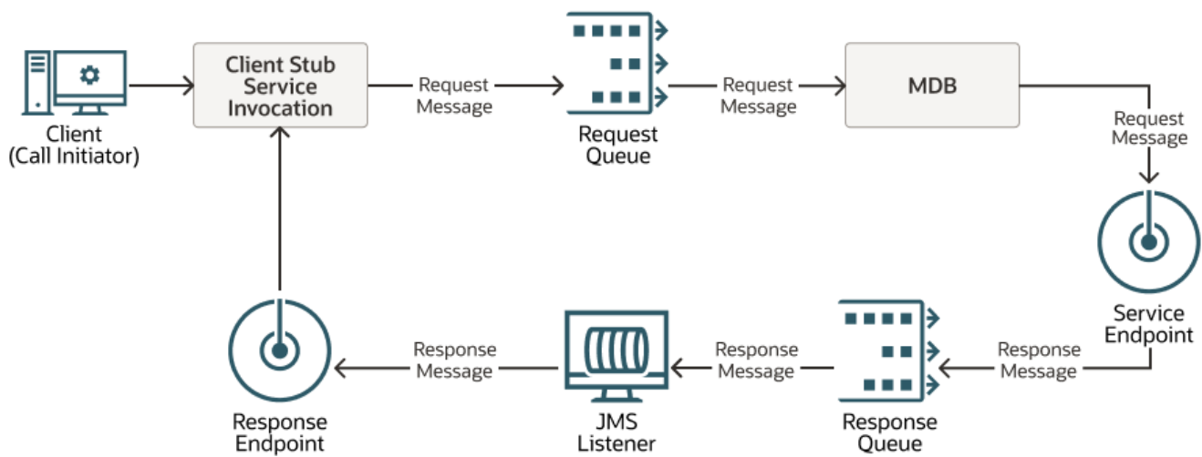
Figure 17-2 Asynchronous Web Service Invocation Using SOAP Over JMS Transport
