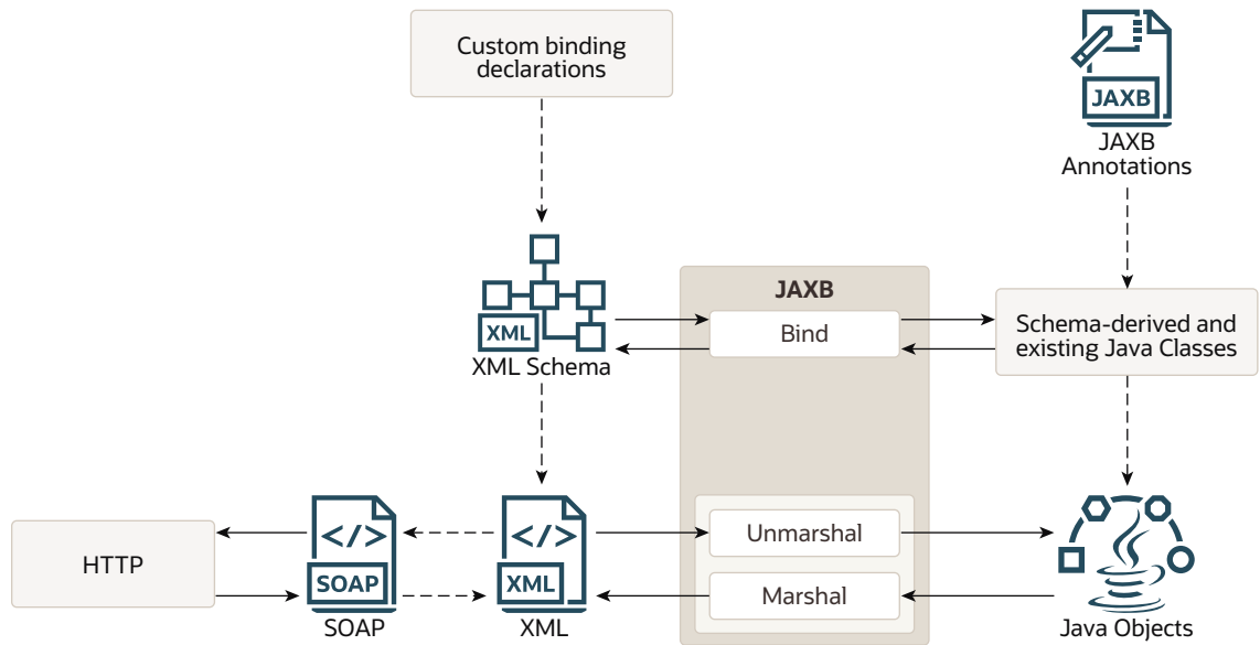
Figure 5-1 Data Binding With JAXB
