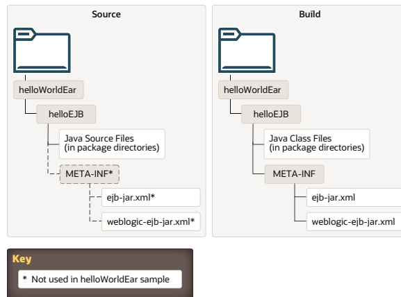
Figure 4-4 Enterprise Application Source Directory
