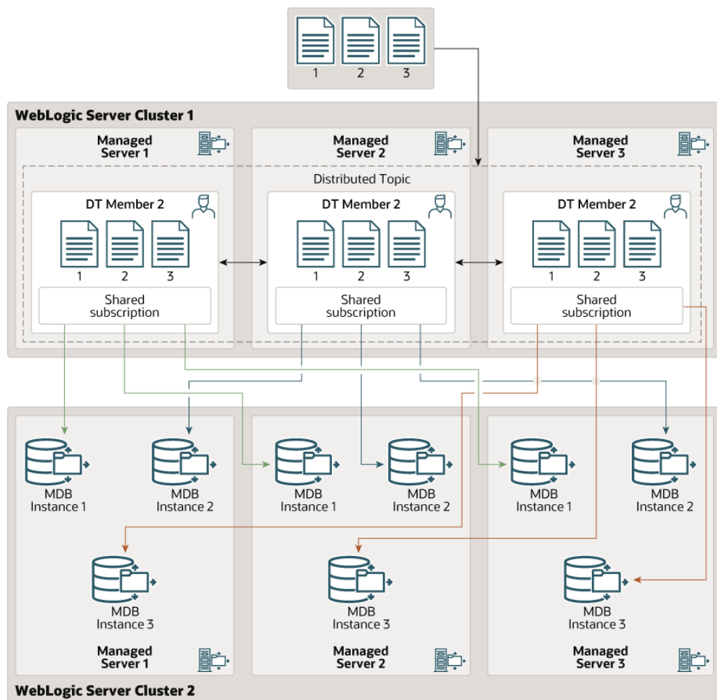
Figure A-6 Scenario 6: Replicated DT, One Copy Per Application, Remote Deployment
