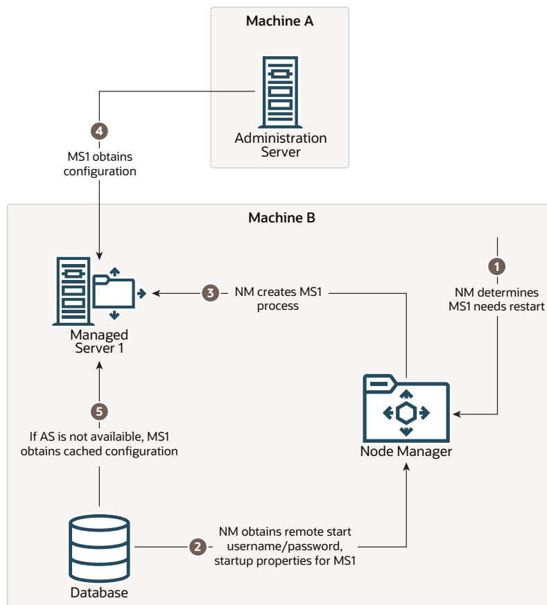
Figure 2-5 Restarting a Managed Server
