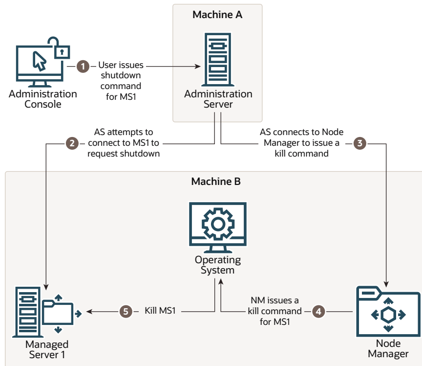
Figure 2-6 Shutting Down a Server Instance Under Node Manager Control
