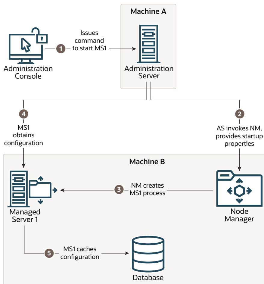
Figure 2-3 Starting a Managed Server
