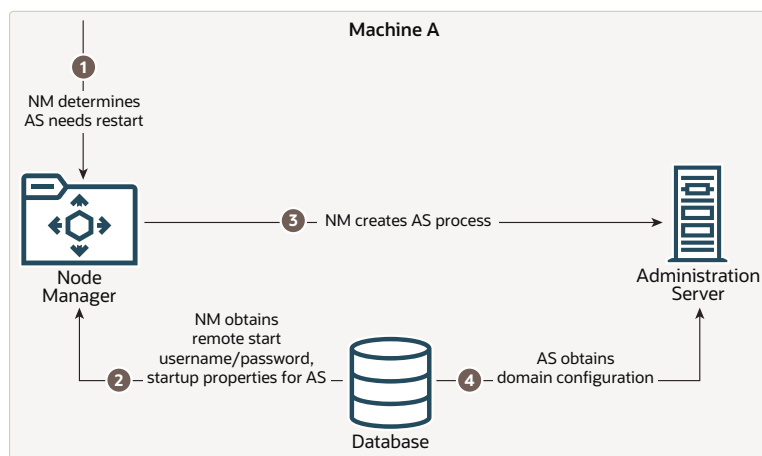
Figure 2-4 Restarting an Administration Server
