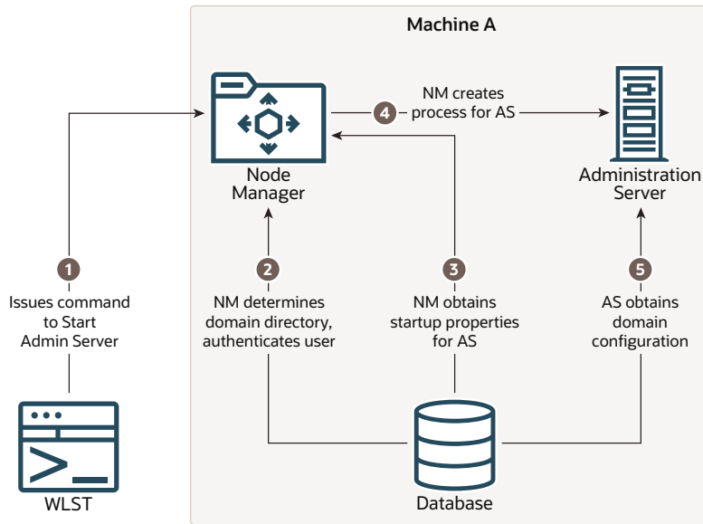
Figure 2-2 Starting an Administration Server
