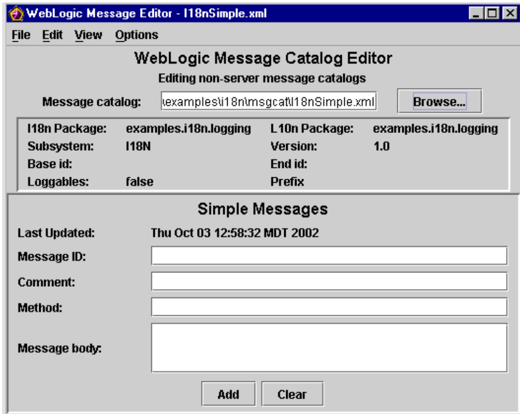
Figure 5-4 WebLogic Message Editor for Simple Messages
