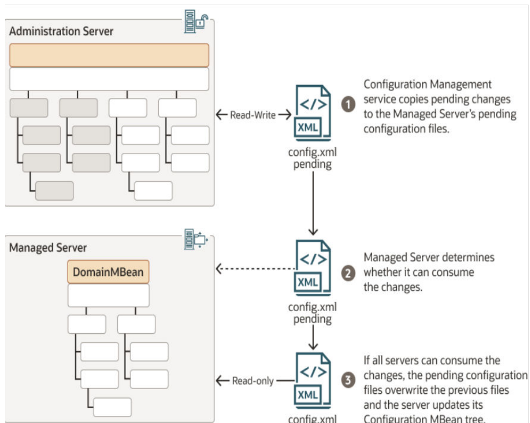
Figure 4-3 Activating Changes in Managed Servers
