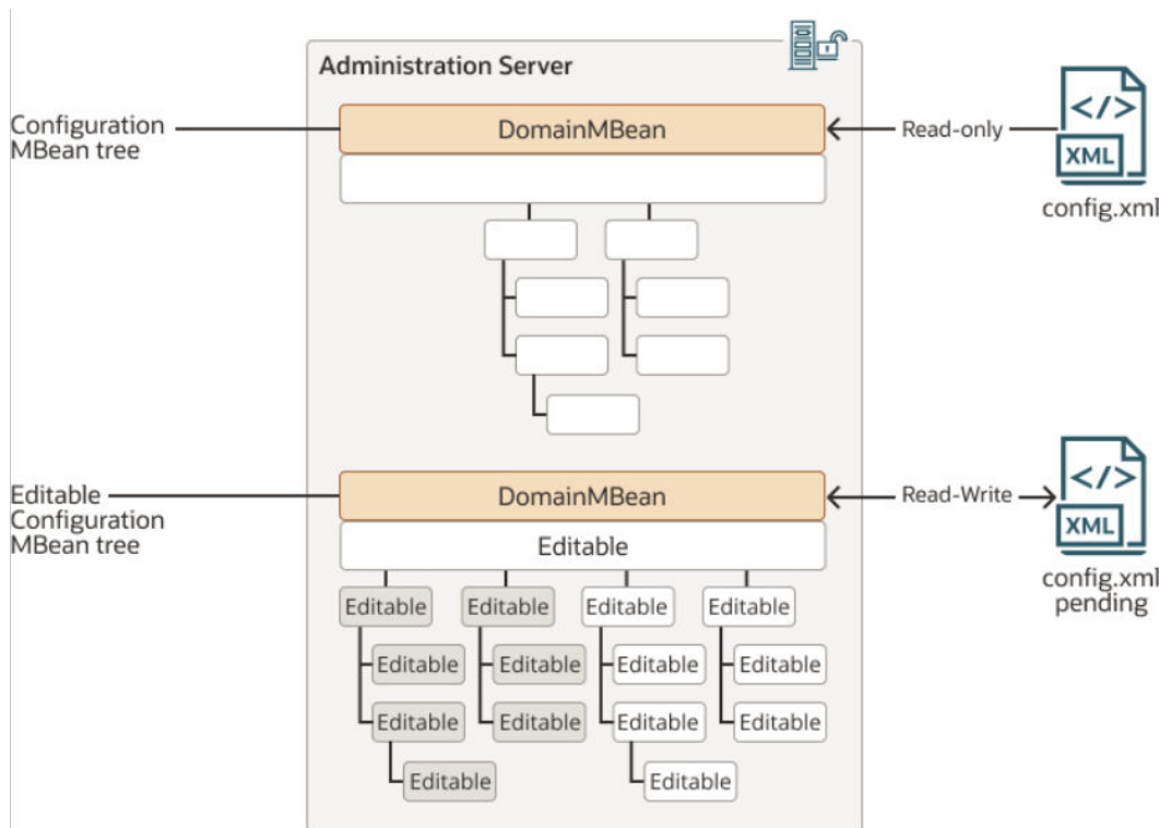
Figure 4-2 The Administration Server's Pending config.xml File
