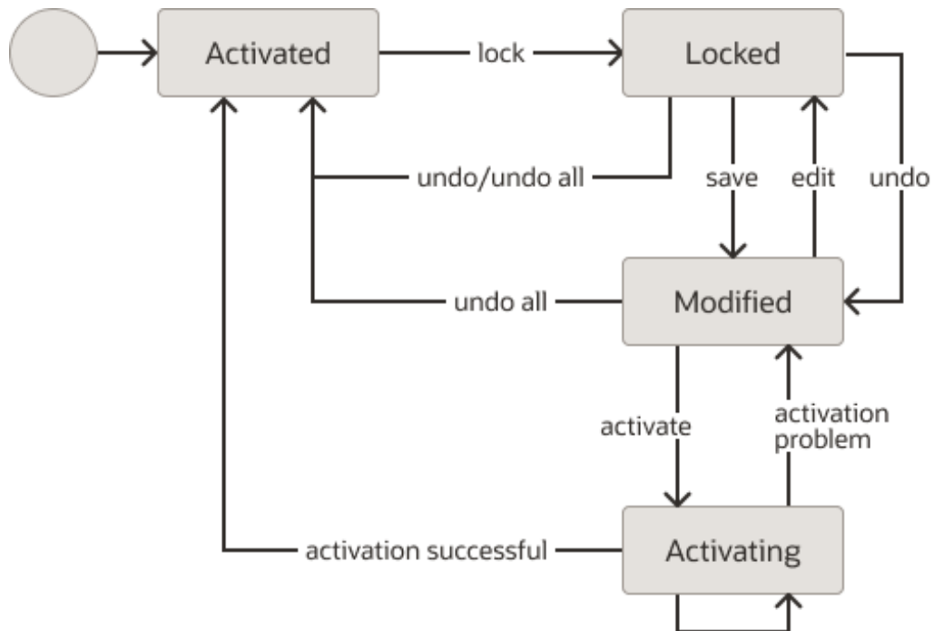
Figure 4-4 Configuration Management State Diagram
