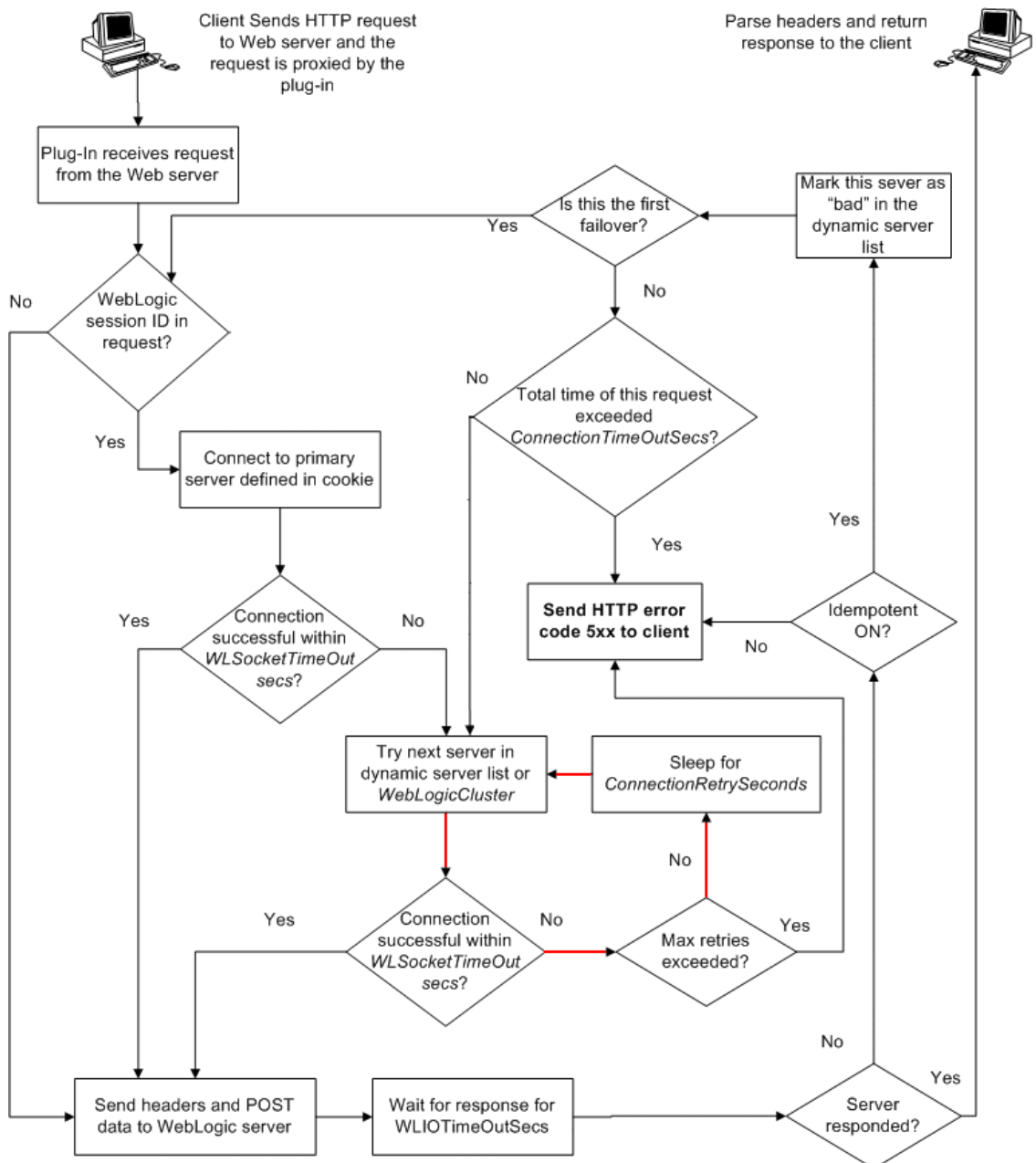
Figure 6-1 Connection Failover
