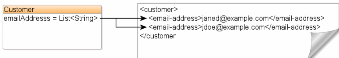
Figure 4-10 XML Direct Collection Mapping to Text Nodes
