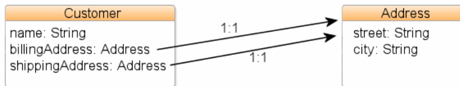
Figure 3-1 Sample Mapped Classes
