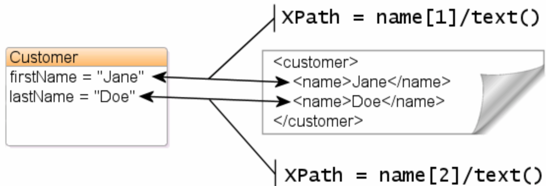
Figure 4-4 XML Direct Mapping to a Text Node
