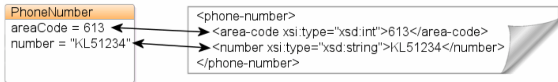
Figure 4-9 XML Direct Mapping with Simple Type Translator
