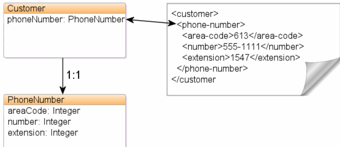
Figure 6-1 One-to-one Relationship
