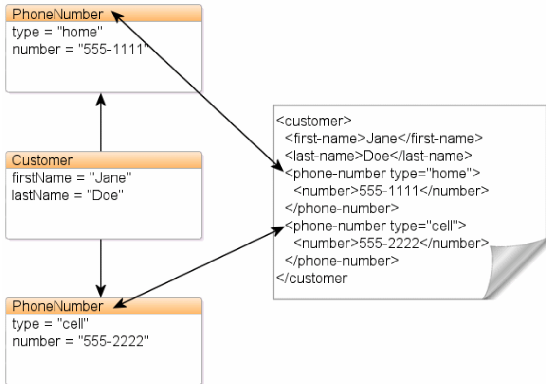
Figure 6-2 One-to-many Relationship
