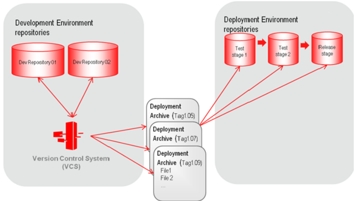
Figure 5-1 Repositories in Development and Deployment Environments
