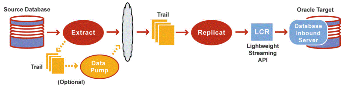
Figure 28-3 Integrated Replicat Configuration
