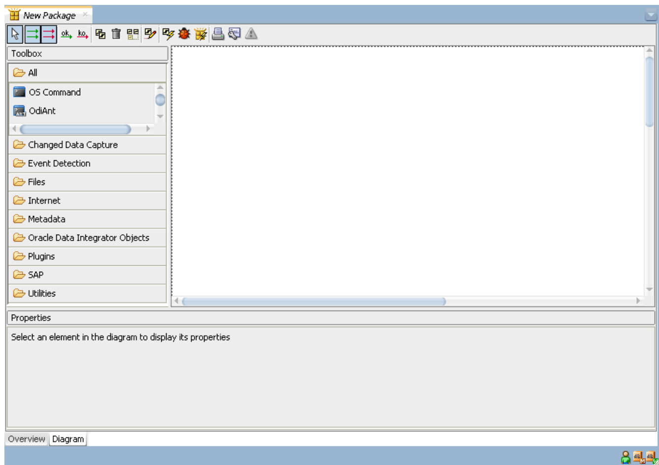
Figure 7-2 Package editor
