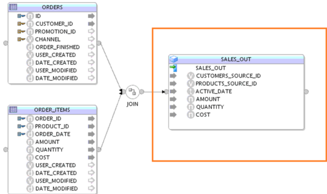
Figure 9-8 Cube Component
