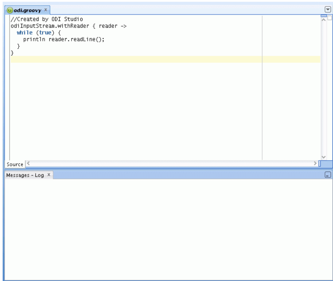
Figure 16-1 Groovy Editor
