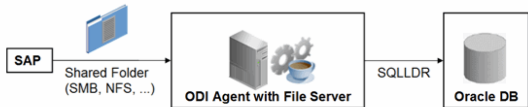
Figure 7-1 Configuration 1
