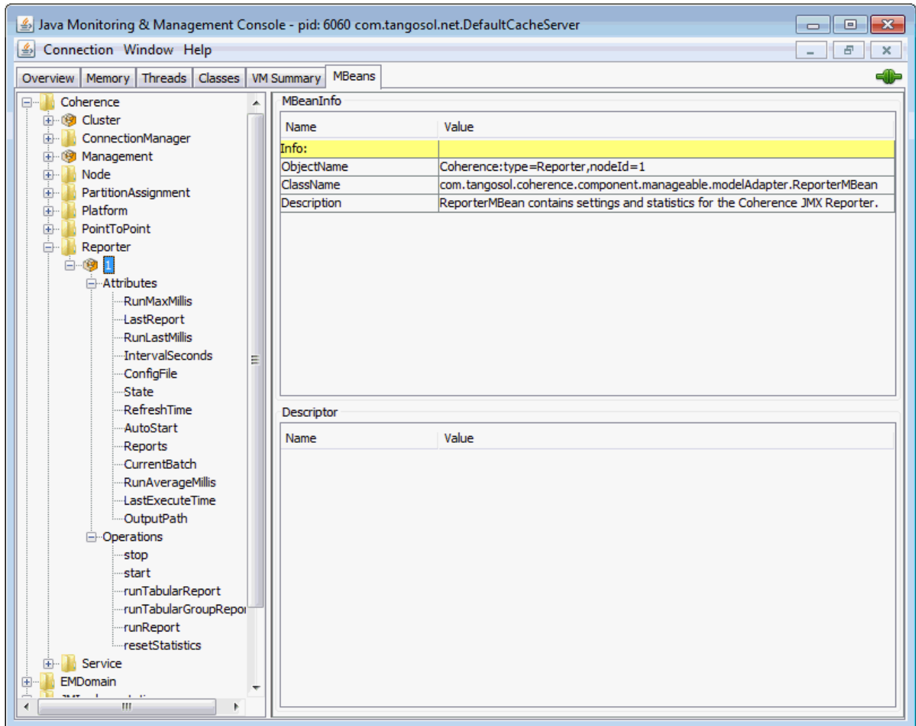
Figure 5-1 ReporterMBean MBean in JConsole
