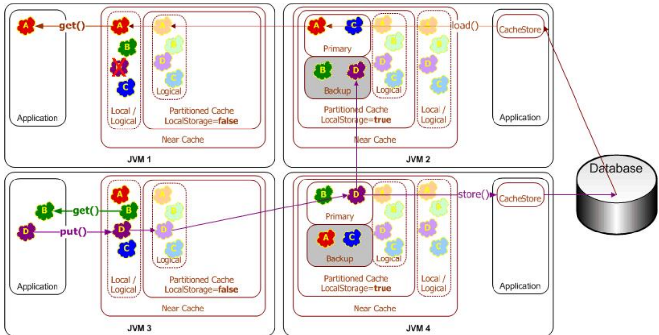
Figure 14-2 Write-Through Caching
