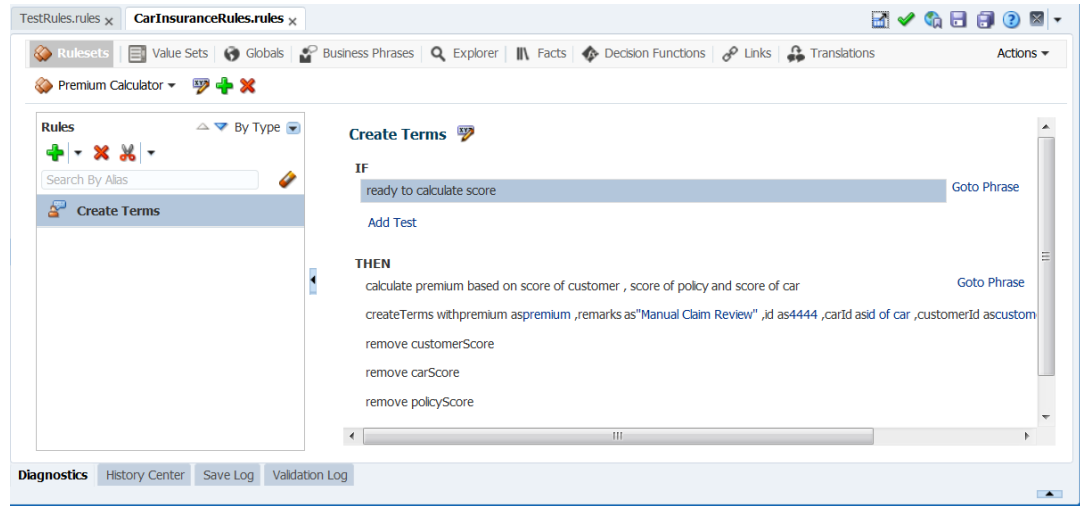
Figure 12-8 Rules Tabs
