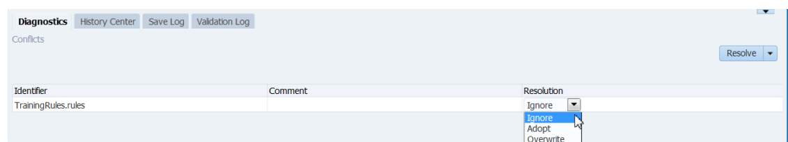
Figure 12-59 Diagnostics Tab
