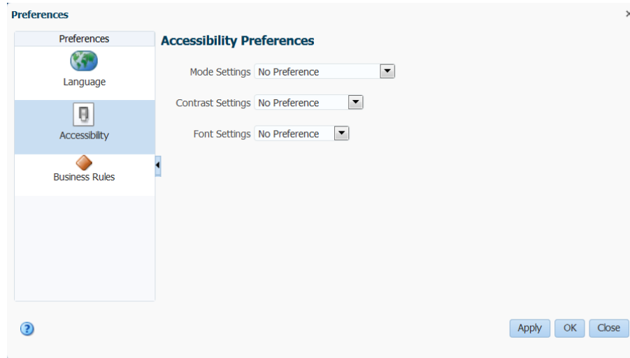
Figure 12-7 Preferences Dialog
