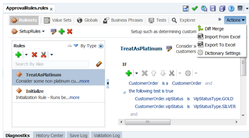
Figure 12-52 Actions Toolbar
