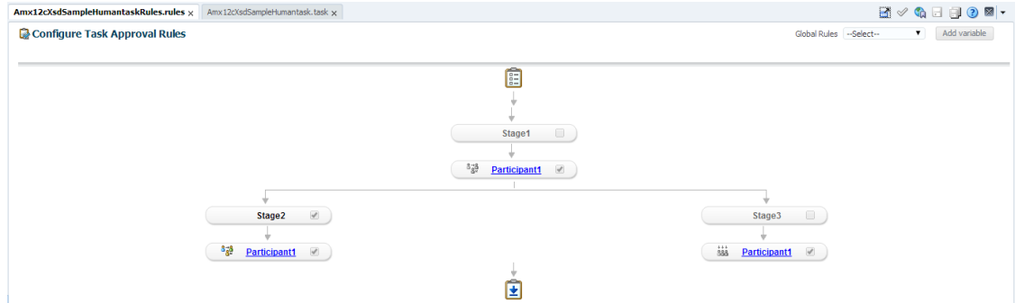
Figure 12-61 Configuring Tasks
