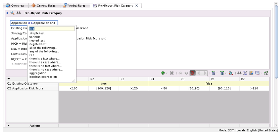
Figure 5-10 Options List
