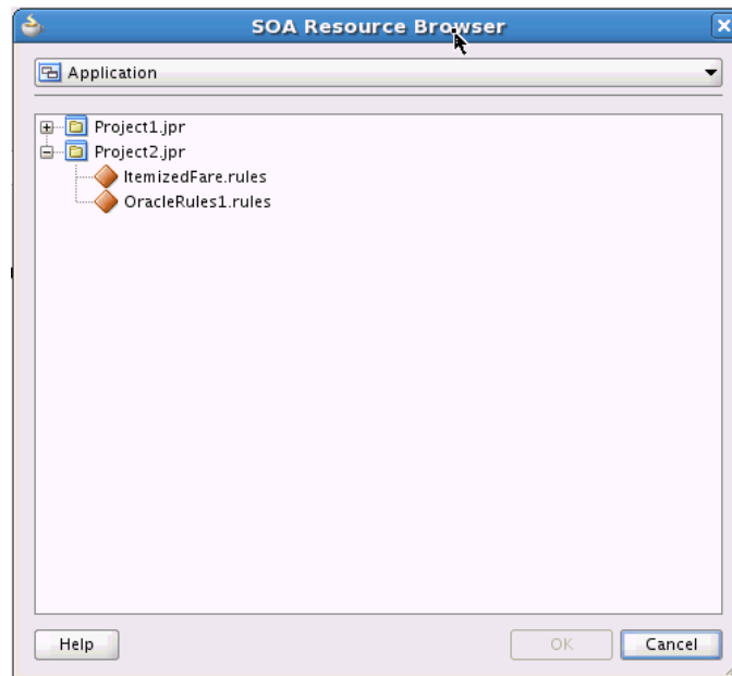
Figure 2-8 Resource Picker
