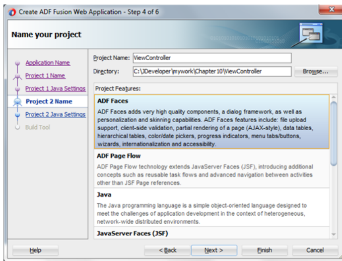
Figure 10-4 Step 4 of 6
