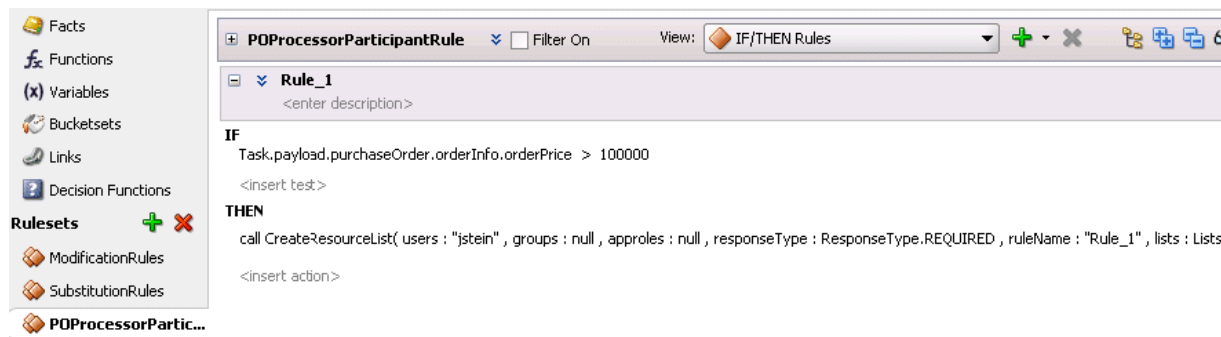
Figure 29-30 Business Rules
