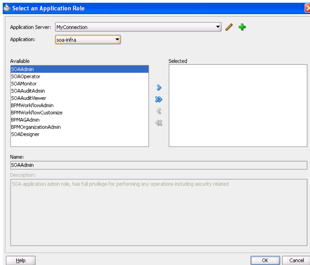
Figure 29-10 Application Role
