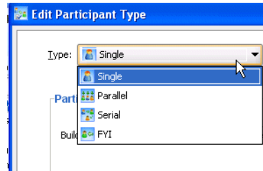
Figure 29-20 Type List
