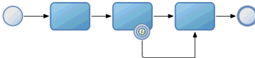
Figure 17-3 Activity Deadline
