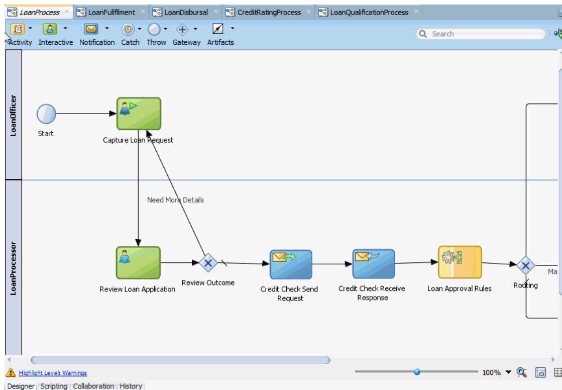
Figure 1-4 Process Editor
