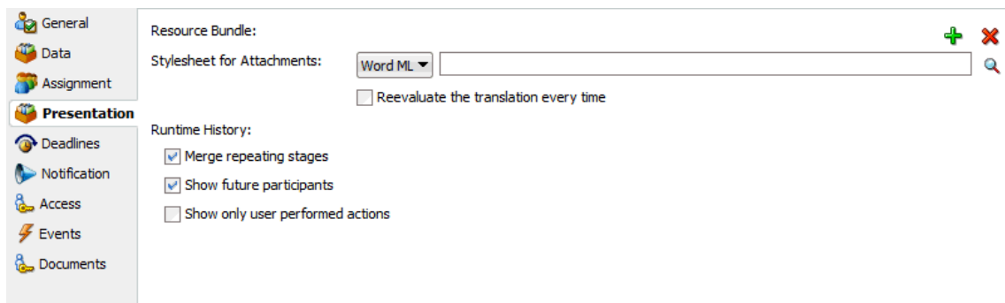
Figure 29-51 Presentation Section
