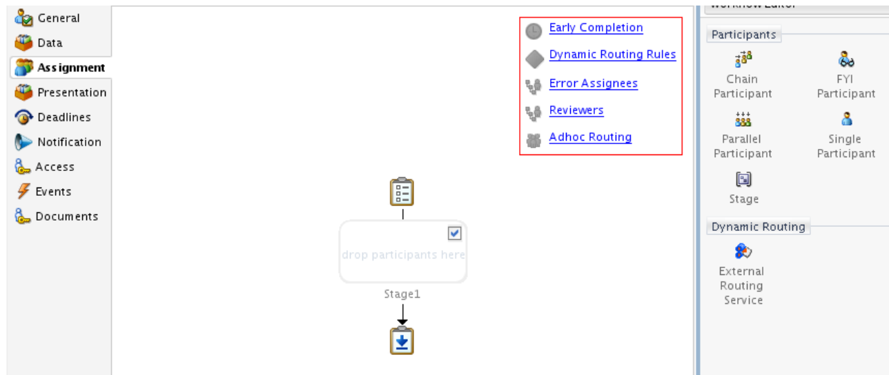
Figure 32-13 Create Stage
