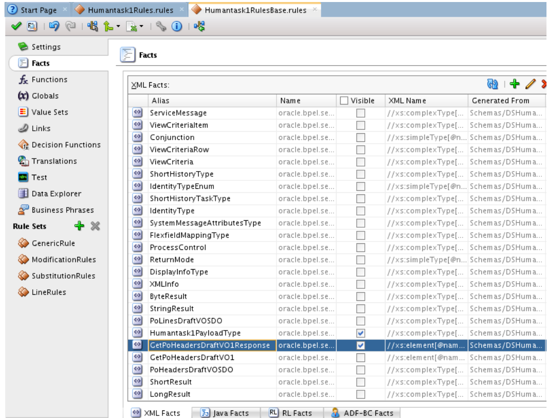
Figure 32-33 Facts List
