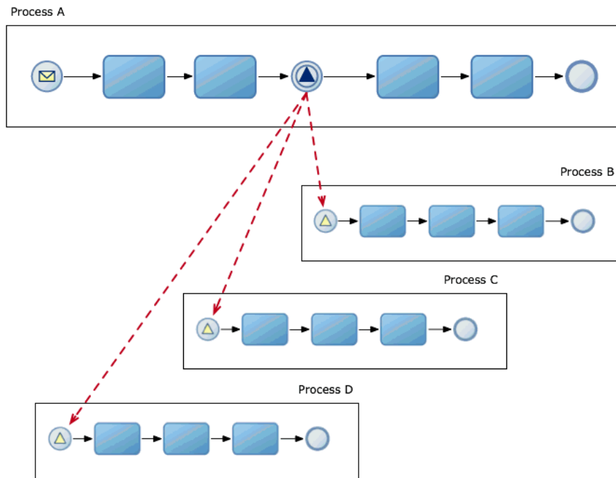
Figure 20-4 Signal Broadcast
