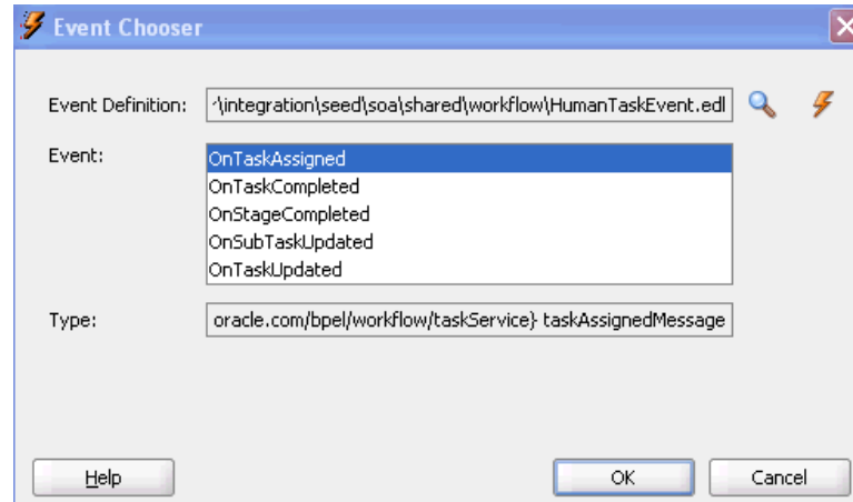
Figure 29-65 Event Callbacks
