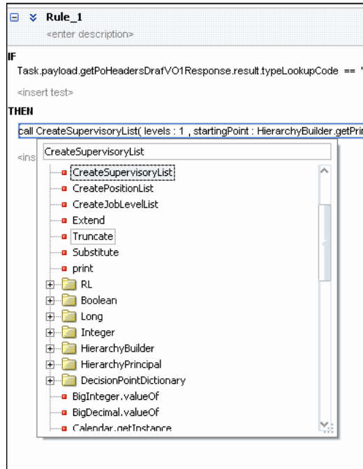
Figure 32-31 Rule Functions
