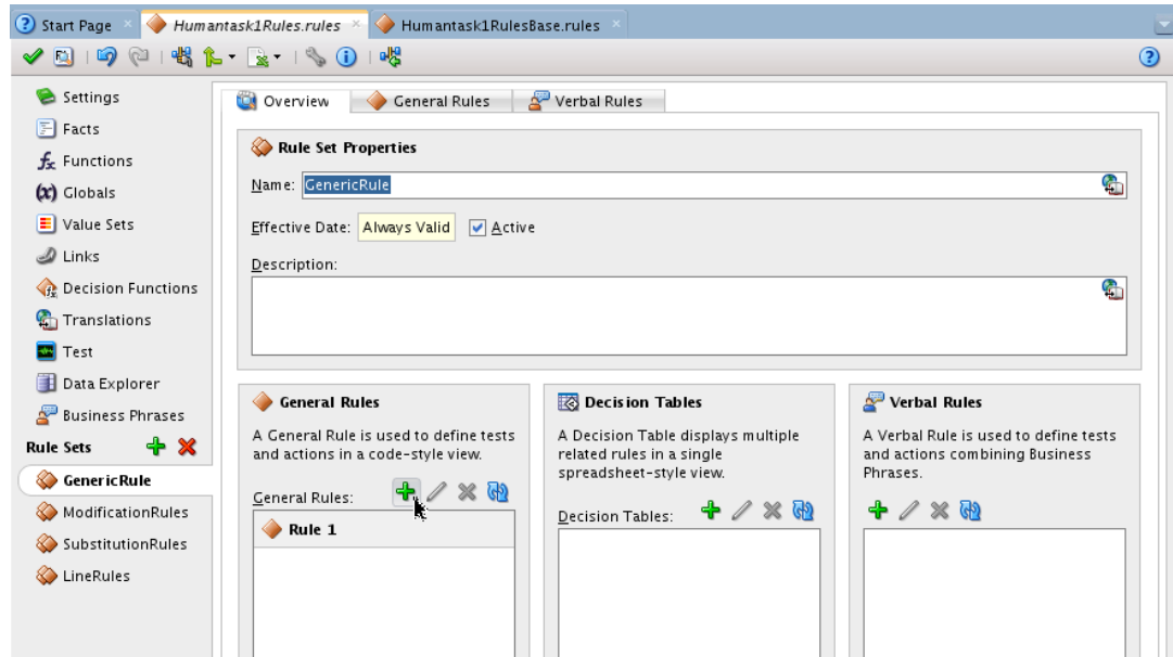
Figure 32-35 Rule-Definition Section
