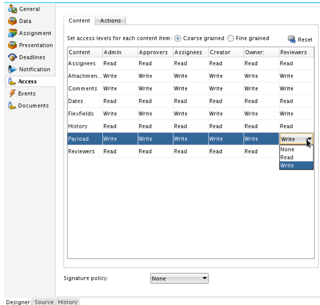
Figure 32-40 Configure Task Content Access Dialog (1)
