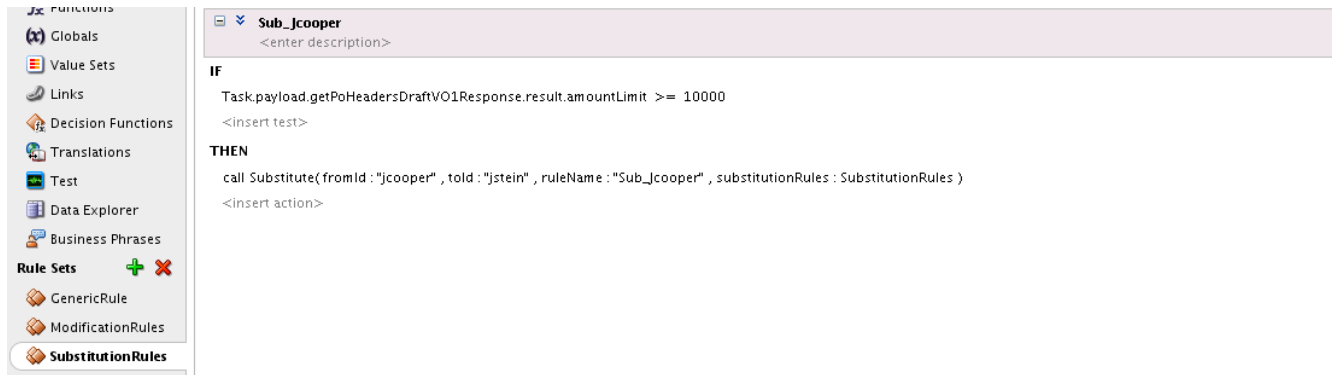
Figure 32-30 Sample Approver-Substitution Action
