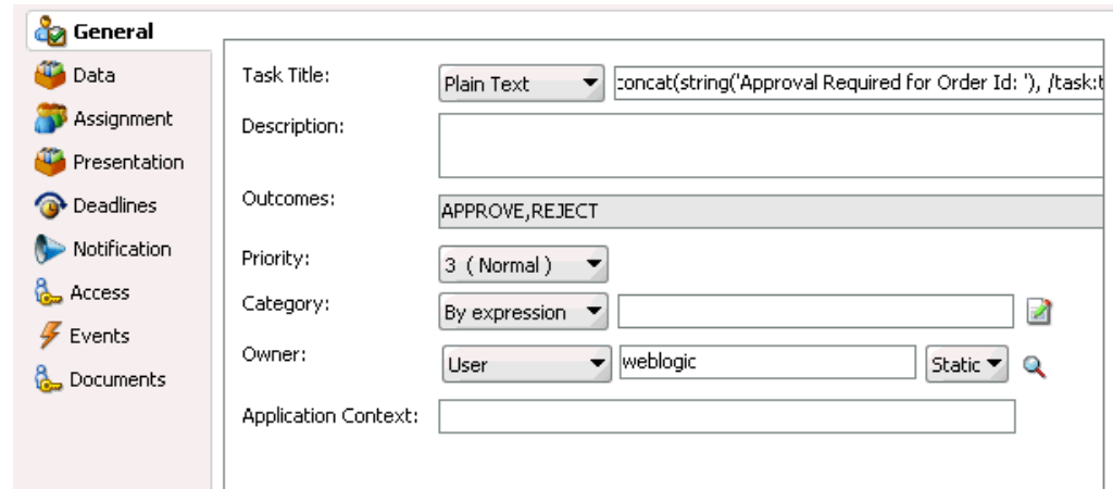
Figure 29-1 Human Task Editor
