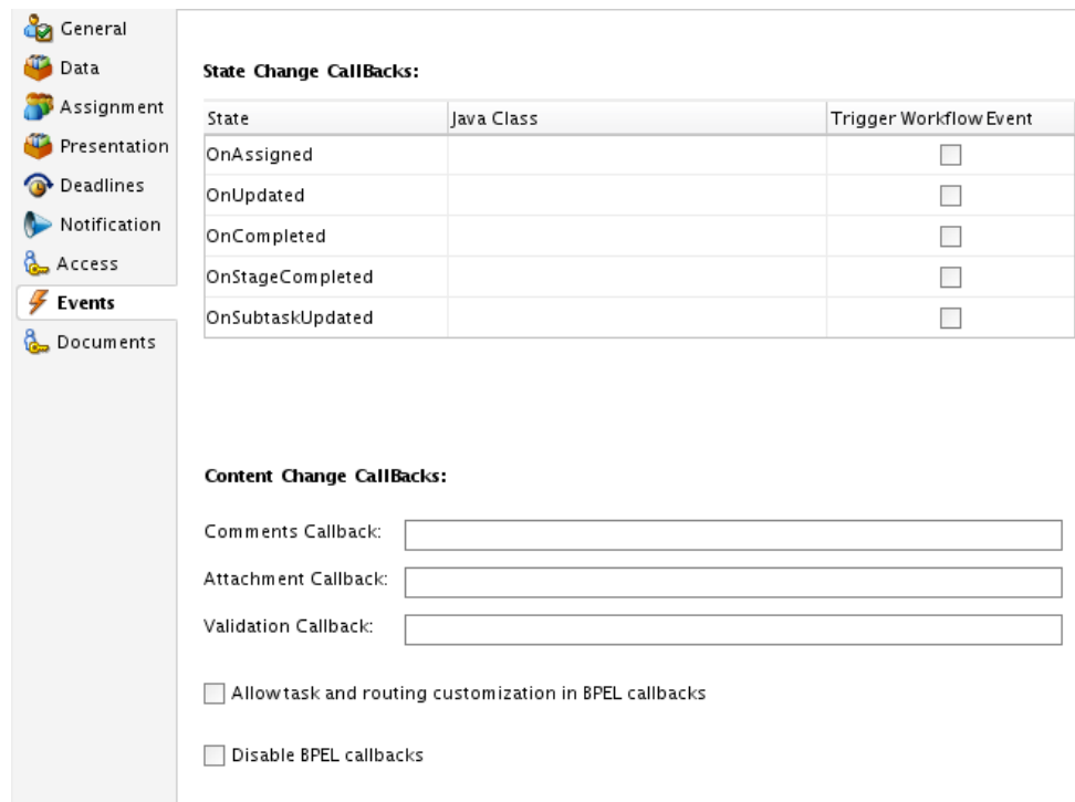
Figure 32-39 Callback Details Dialog
