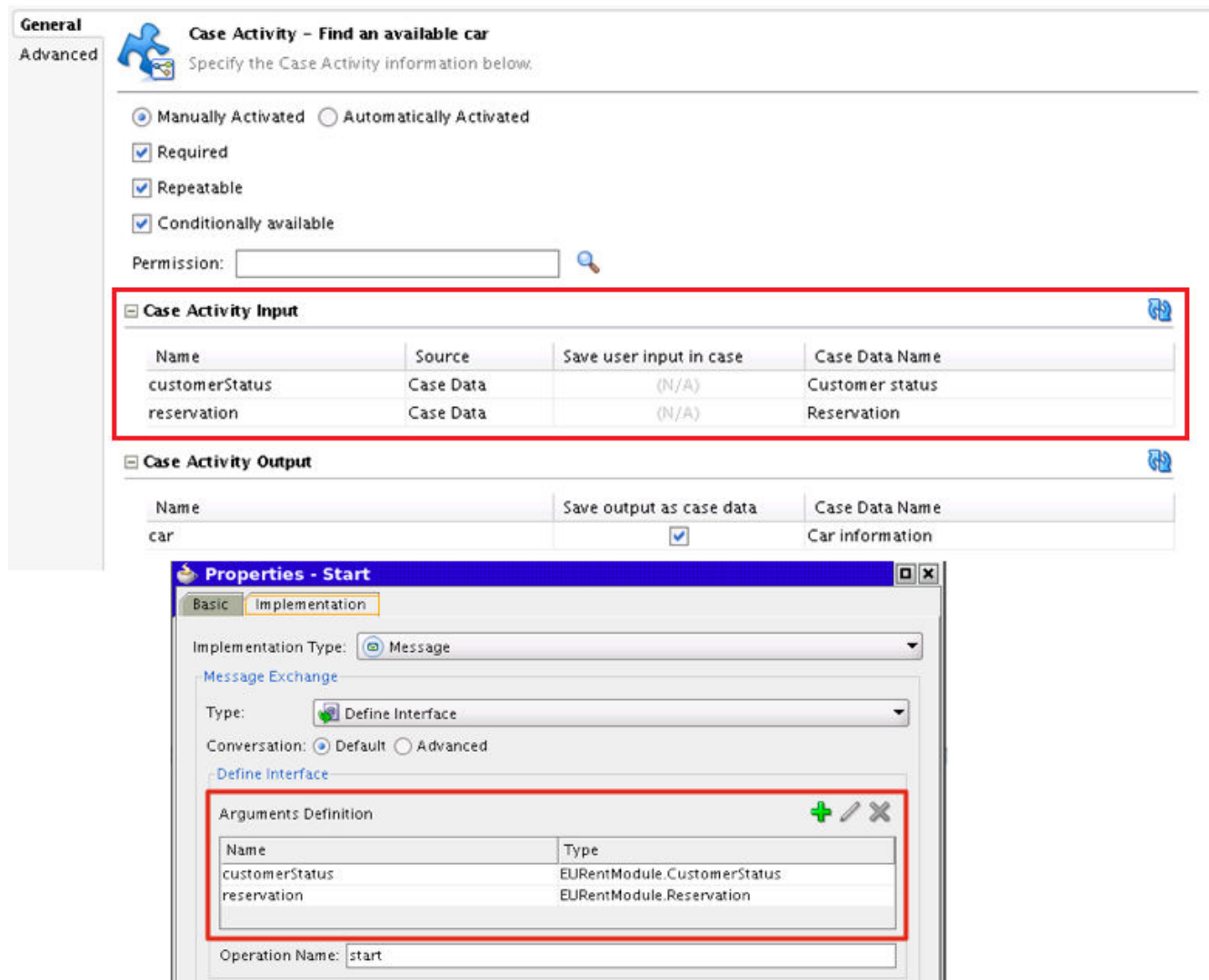
Figure 33-8 BPMN Process Based Case Activity Input Parameters
