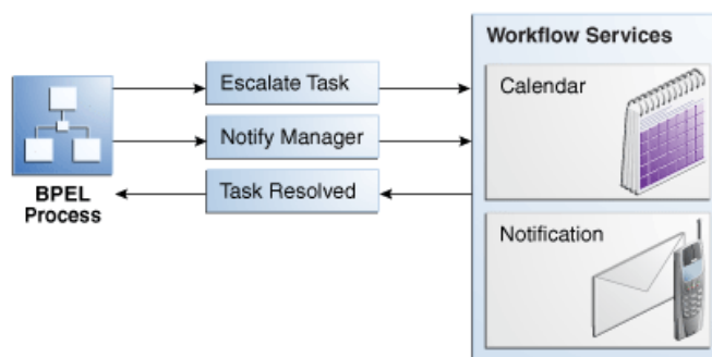
Figure 27-5 Escalation and Notification
