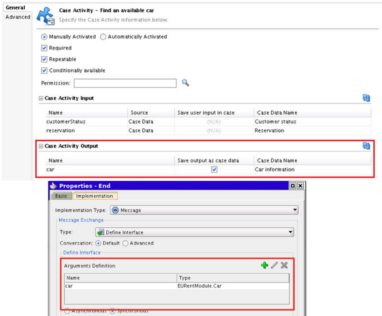
Figure 33-9 BPMN Process Based Case Activity Output Parameters
