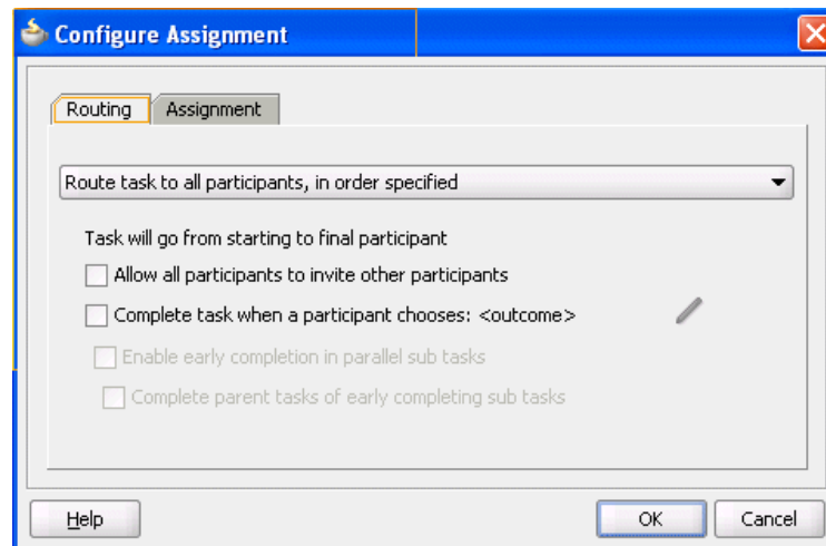
Figure 29-40 Configure Assignment
