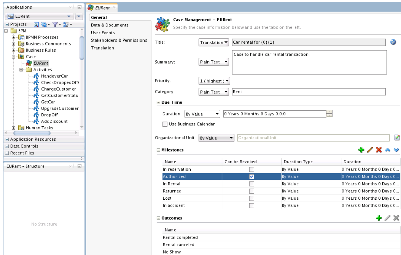
Figure 33-2 Case Management Editor
