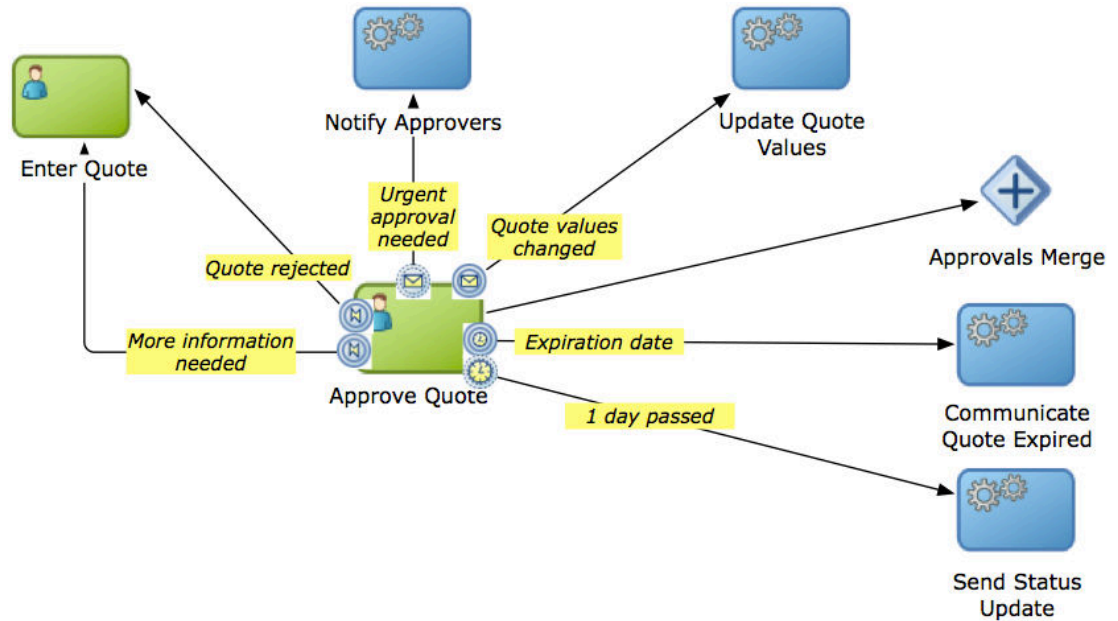
Figure 6-1 The Approve Quote user task with multiple boundary events
