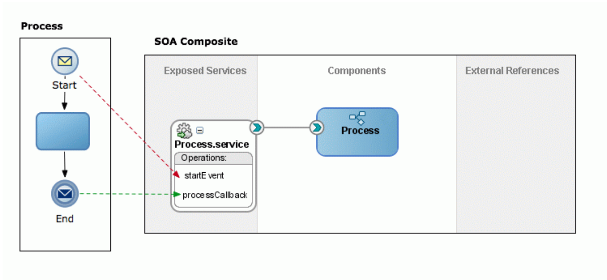
Figure 21-3 Asynchronous BPMN process that exposes a start operation an its corresponding callback
