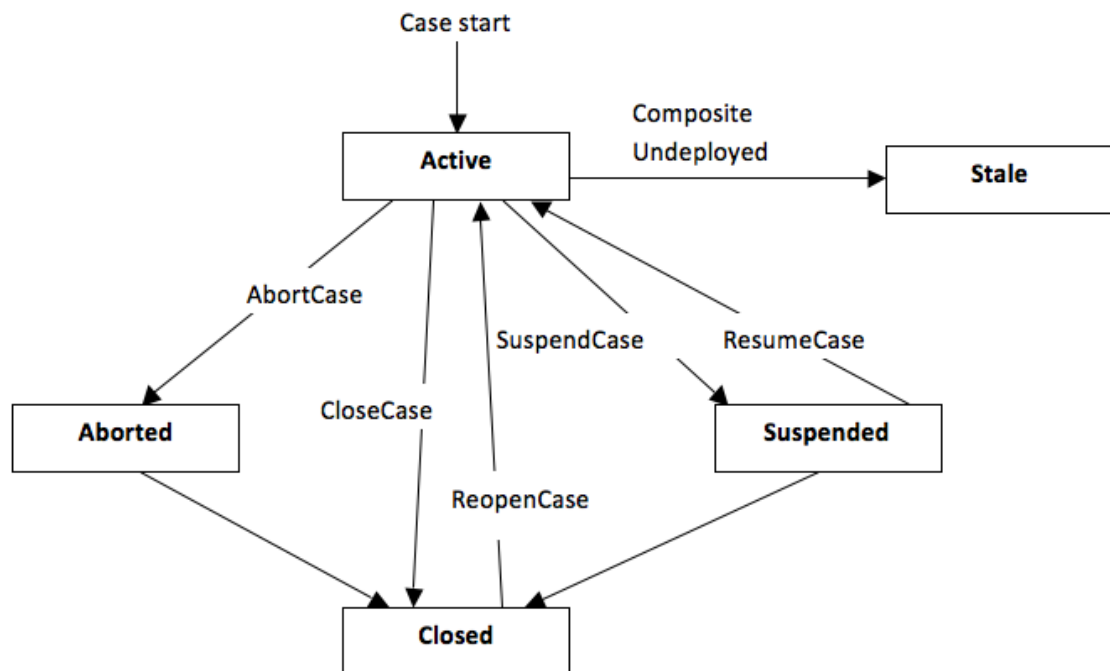
Figure 33-1 Case State Model
