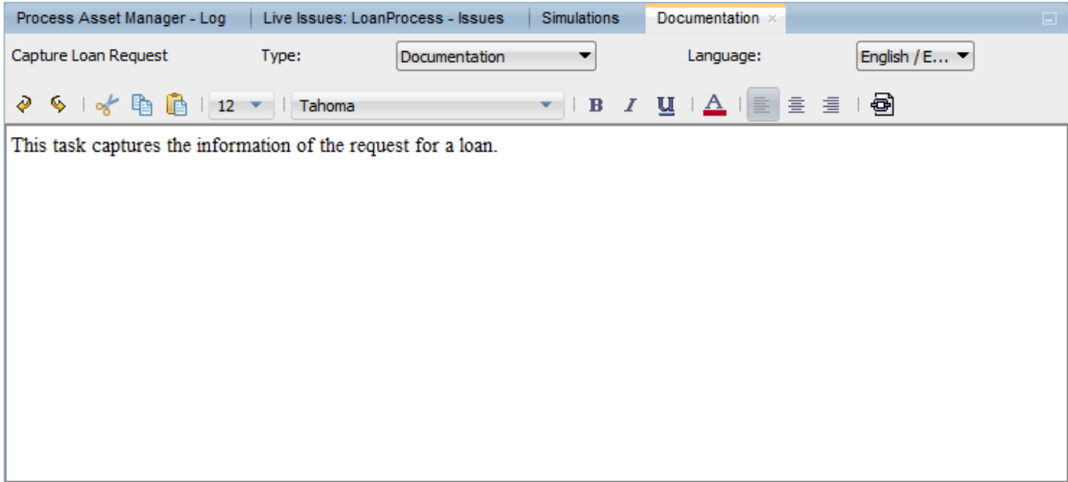
Figure 1-10 Documentation Window
