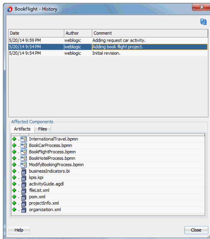
Figure 9-2 History Dialog
