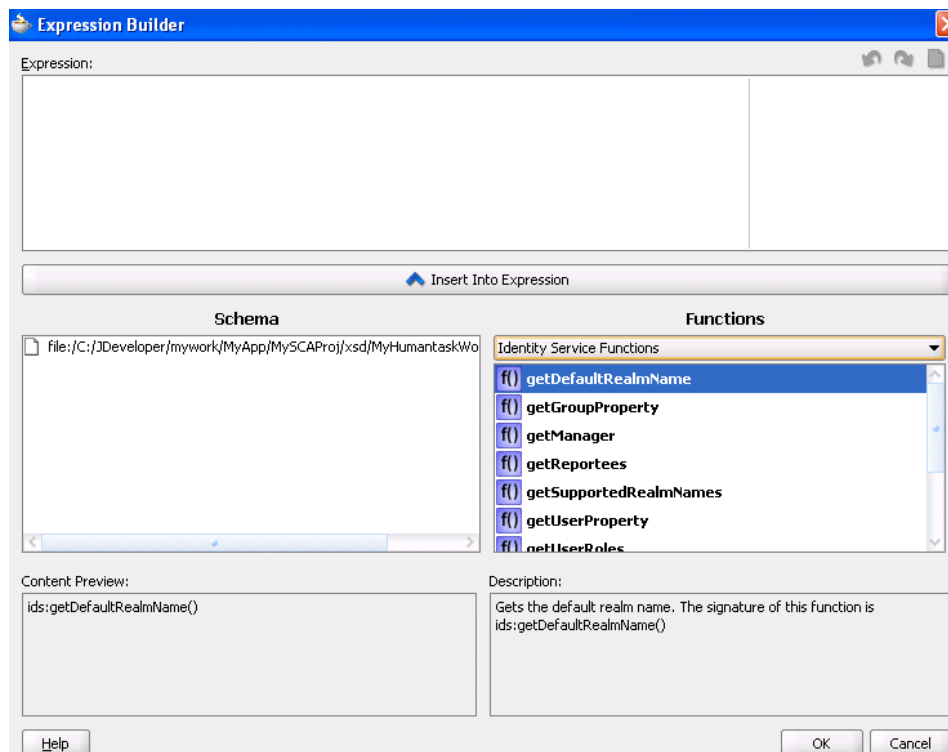
Figure 29-12 Expression Builder
