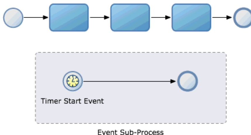
Figure 17-4 Process Deadline
