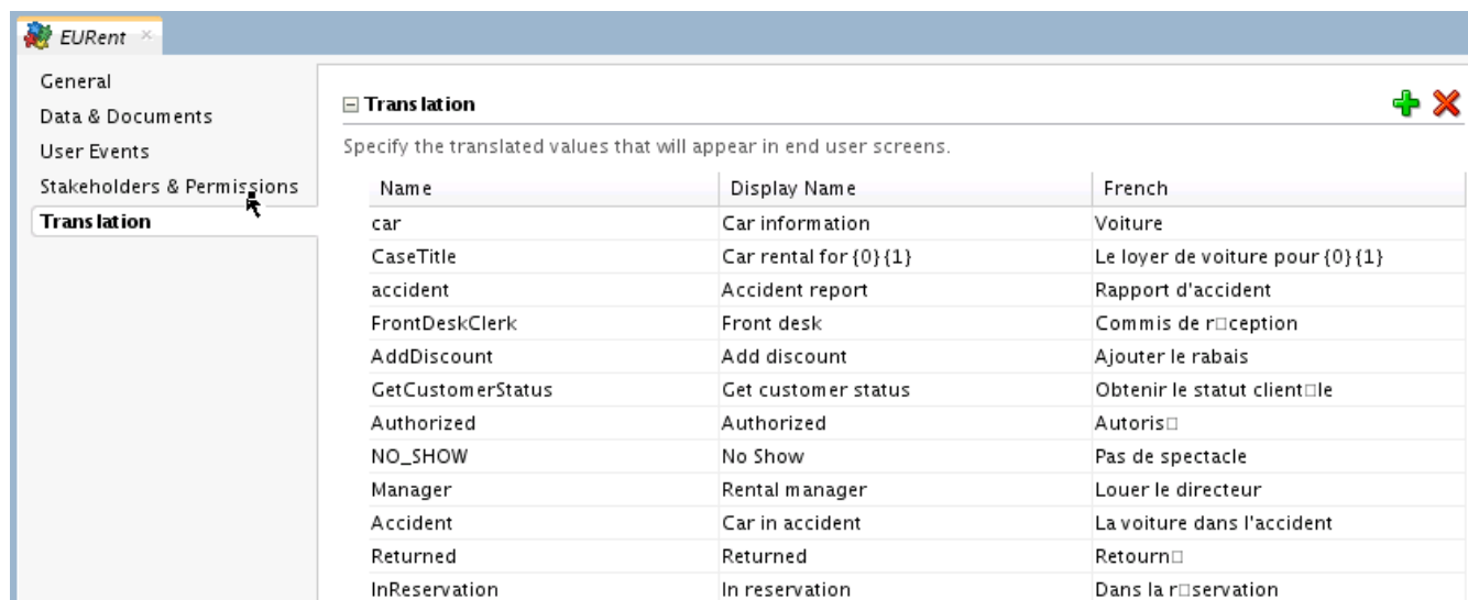
Figure 33-6 Translation Editor
