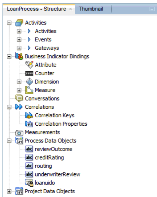
Figure 1-7 Structure View
