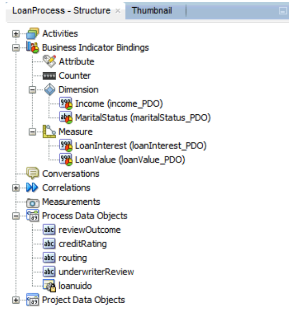
Figure 5-1 Structure Window
