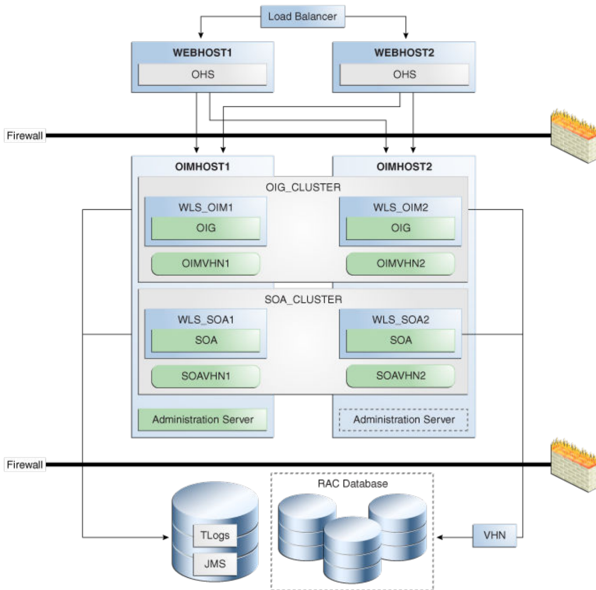
Figure 6-2 Oracle Identity Governance High Availability Architecture
