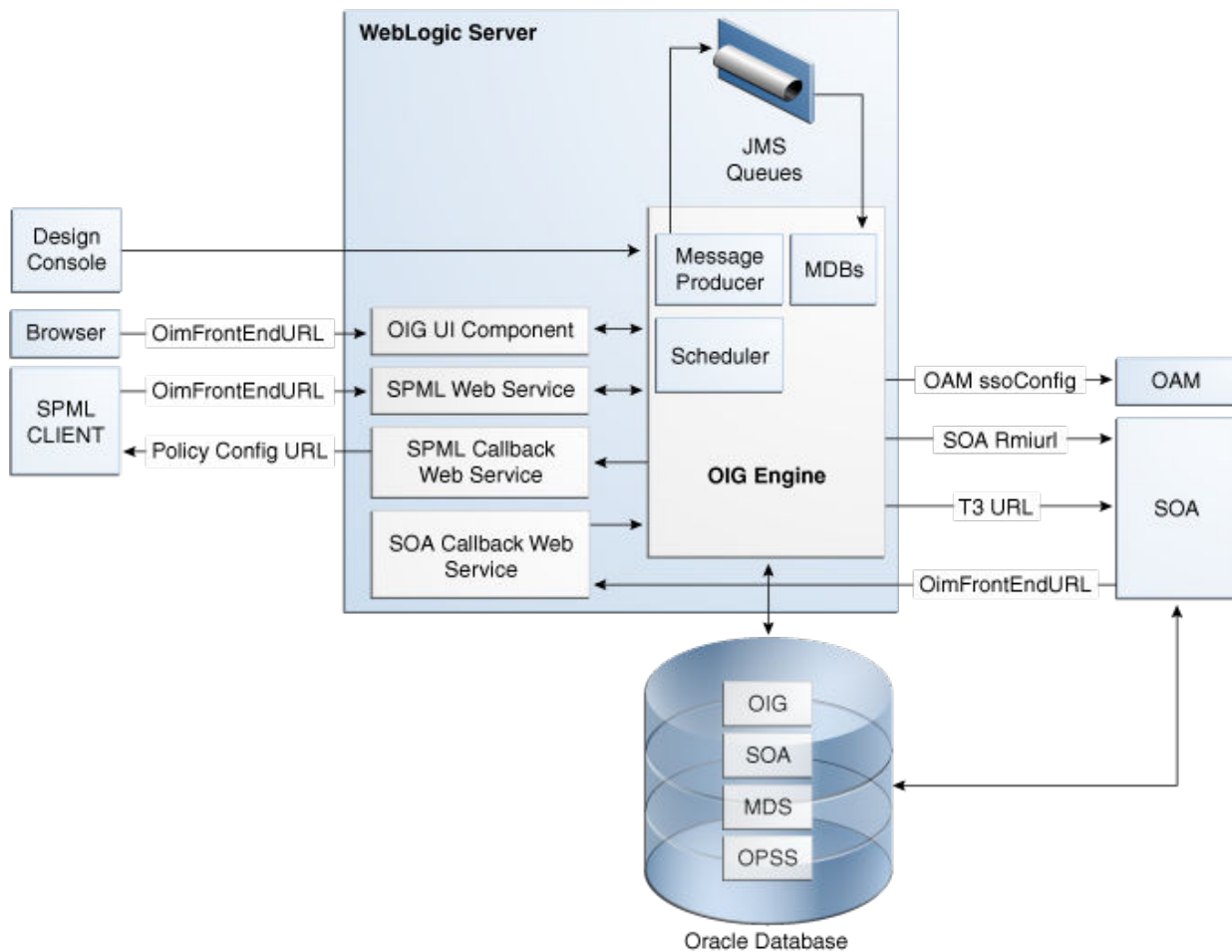
Figure 6-1 Oracle Identity Governance Component Architecture
