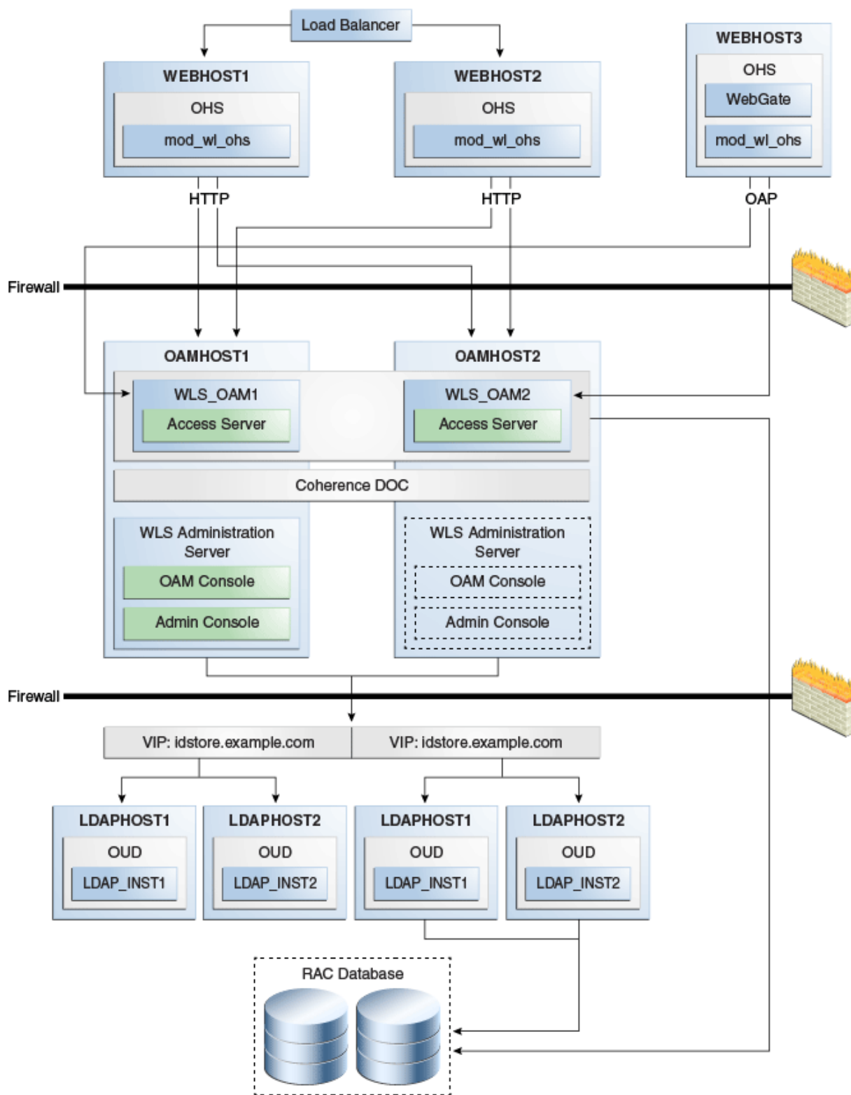
Figure 7-2 Access Manager High Availability Architecture
