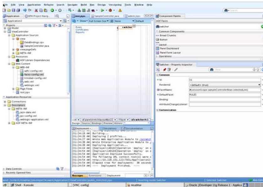
Figure A-23 Adding and Specifying a Switcher
