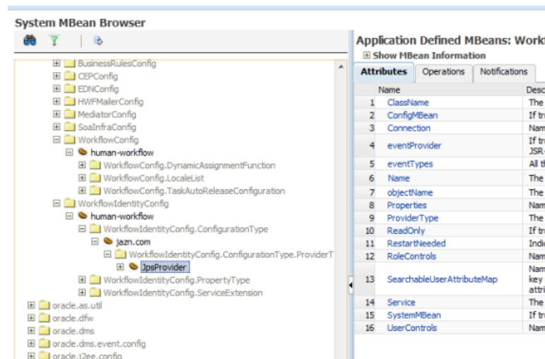
Figure 10-8 Viewing Attributes Tab for JpsProvider
