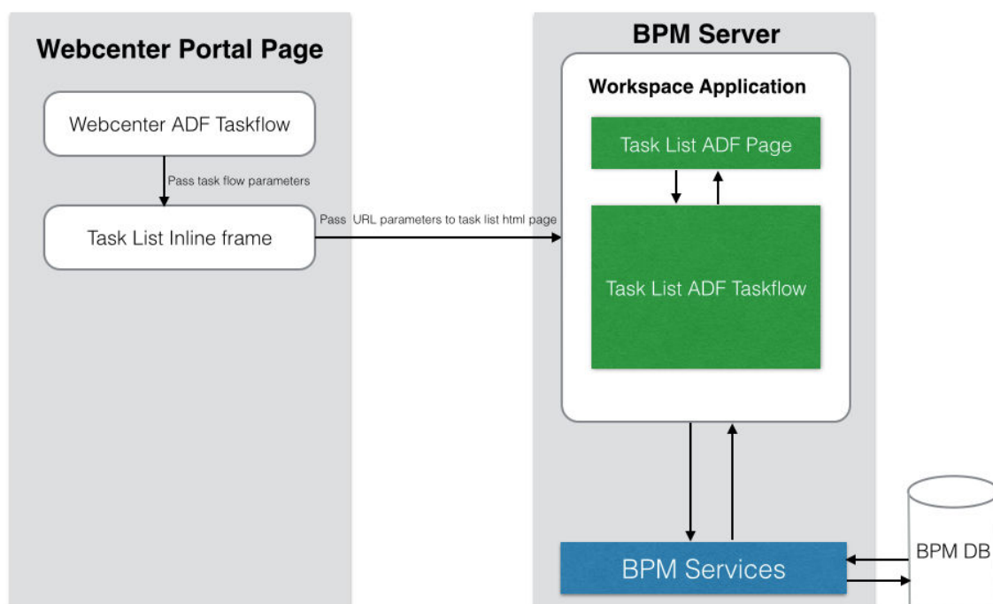
Figure 9-33 WebCenter Portal BPM Integration Architecture
