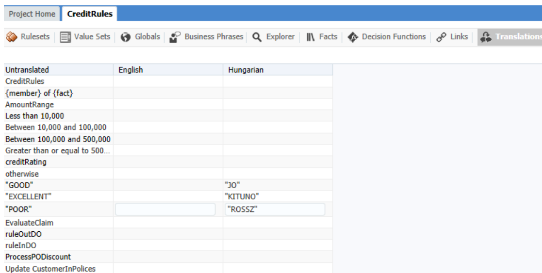
Figure 17-17 Business Rules Editor - Translations
