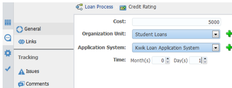
Figure 6-19 Business Properties - General
