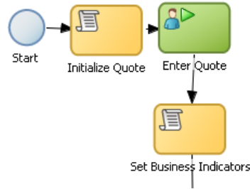
Figure A-50 The Script Task within the Sales Quote Example
