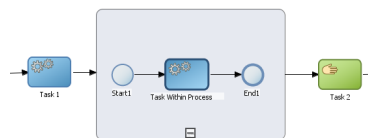
Figure A-47 Example of an Expanded Embedded Subprocess
