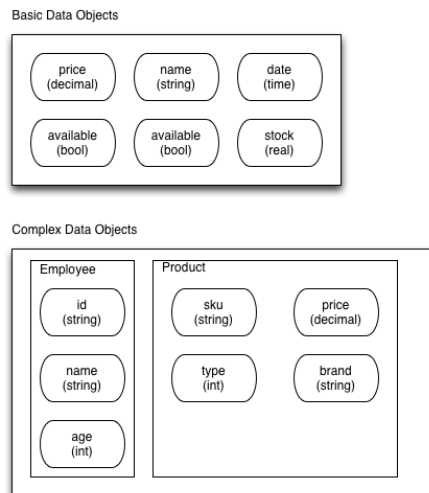
Figure 13-1 Relationship Between Basic and Complex Data Objects
