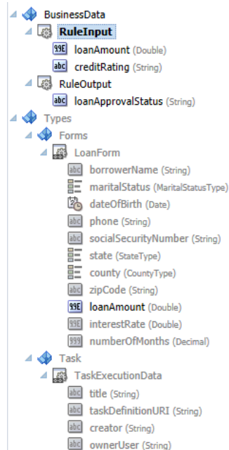
Figure 14-1 Complex Data Types Defined in the Example Project
