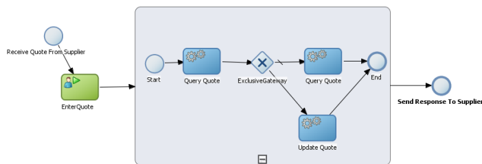
Figure A-48 Example of an Embedded Subprocess
