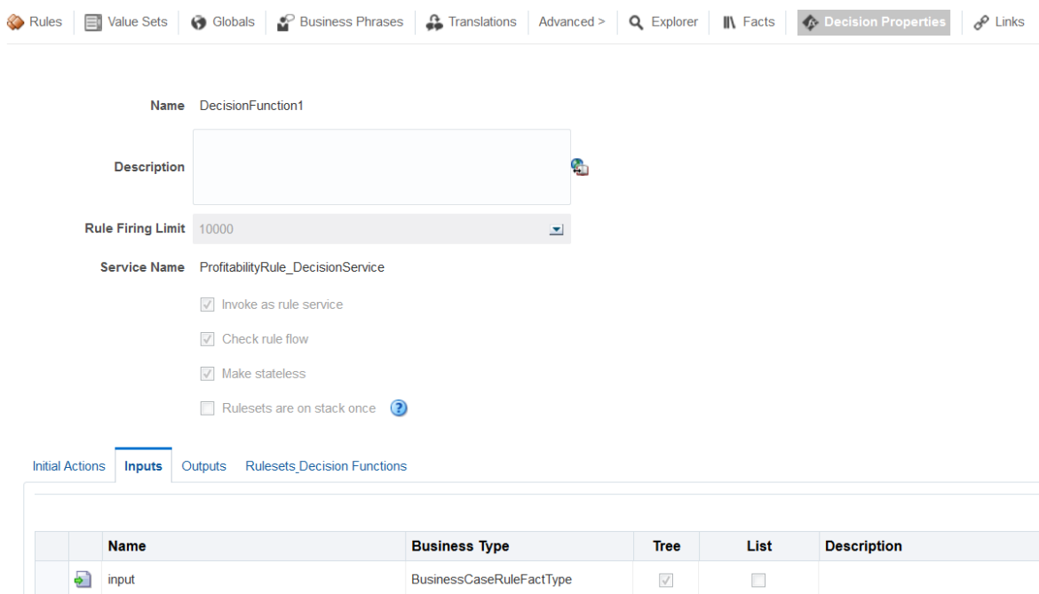
Figure 17-15 Business Rules Editor - Decision Functions
