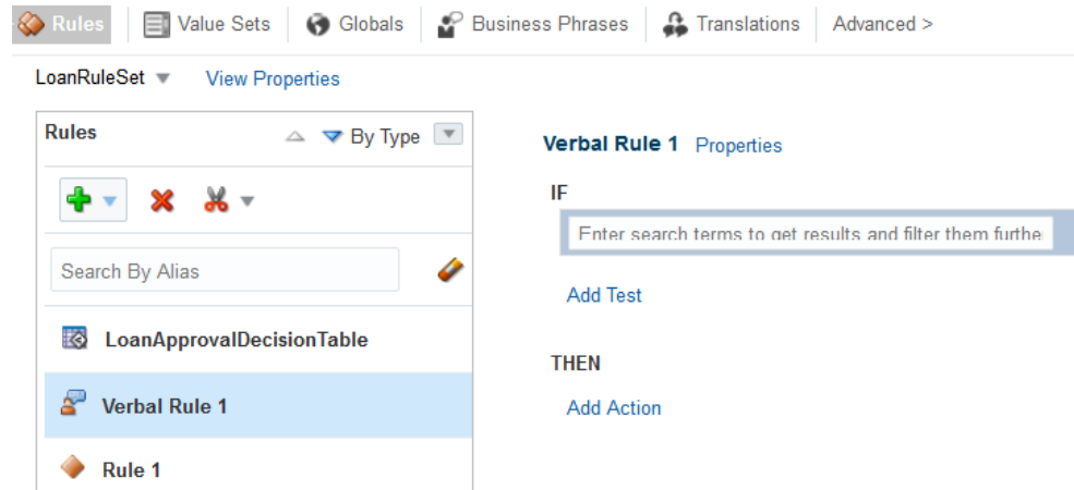
Figure 17-7 Business Rules Editor: Rulesets - New Verbal Rule
