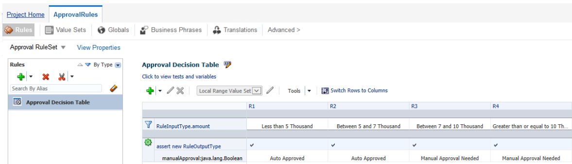
Figure 17-1 Business Rules Editor - Rulesets
