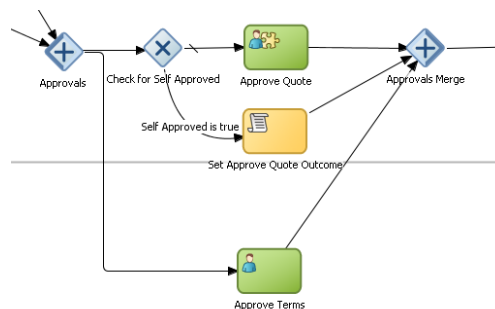
Figure A-40 Example of a Parallel Gateway
