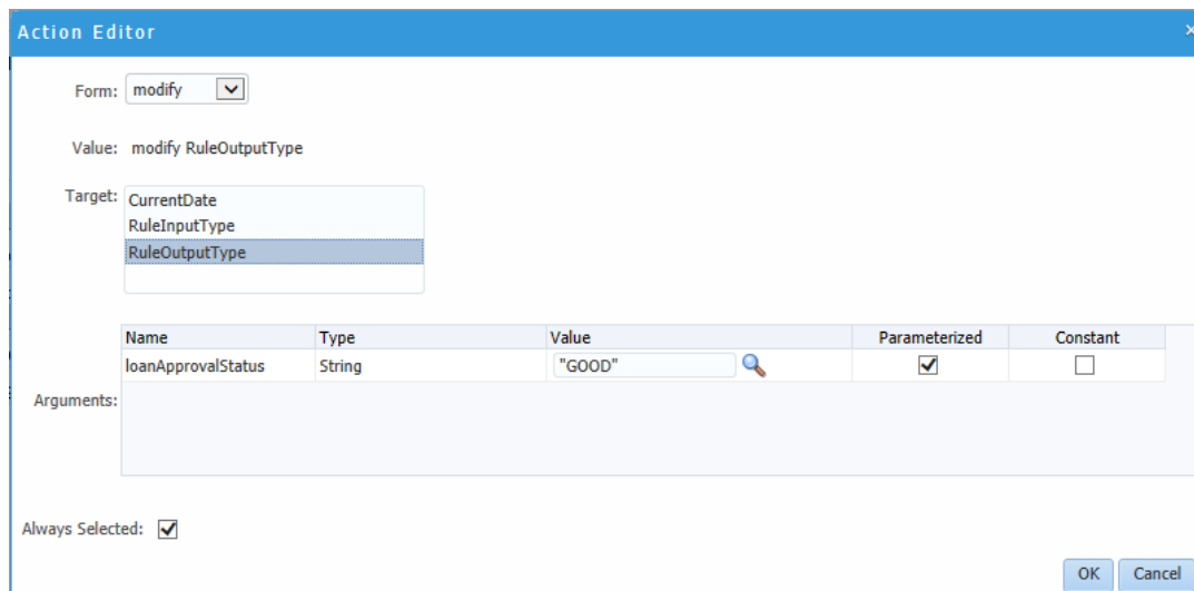
Figure 17-9 Action Editor Showing Paramaterized Action with Default Value
