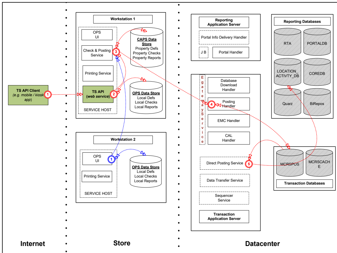
Figure 1-1 - Symphony Architecture
