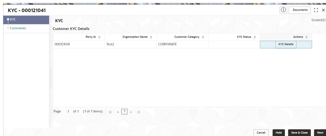
Figure 1-6 KYC Details
