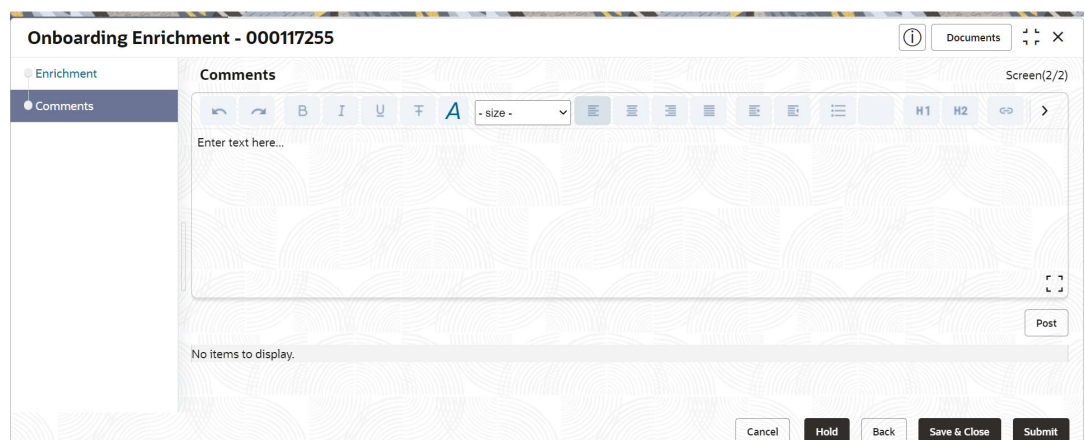
Figure 1-14 Enrichment – Comments
