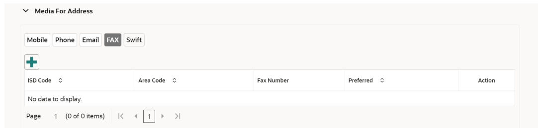
Figure 1-22 FAX
