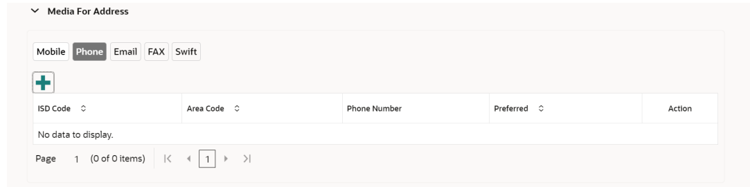
Figure 1-20 Phone
