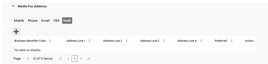
Figure 1-23 SWIFT
