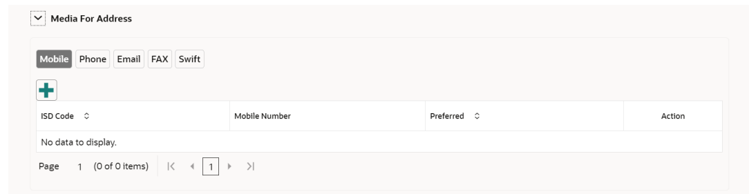
Figure 1-19 Mobile
