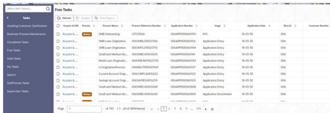
Figure 1-5 Free Tasks
