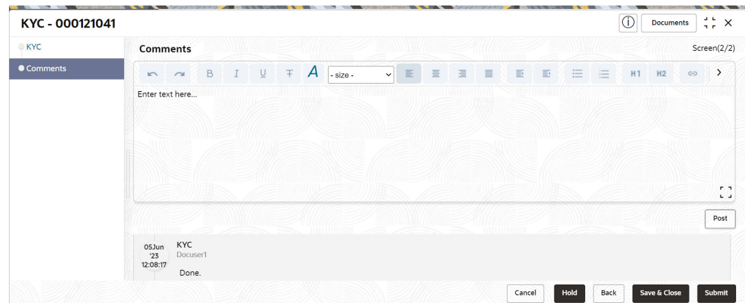
Figure 1-7 KYC – Comments
