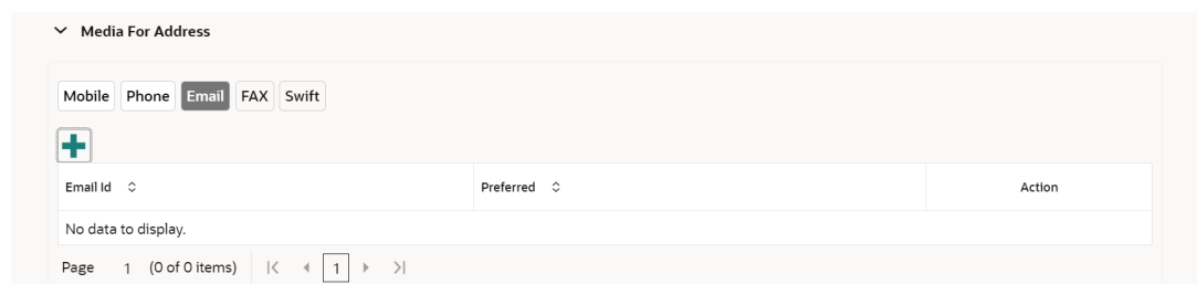
Figure 1-21 Email
