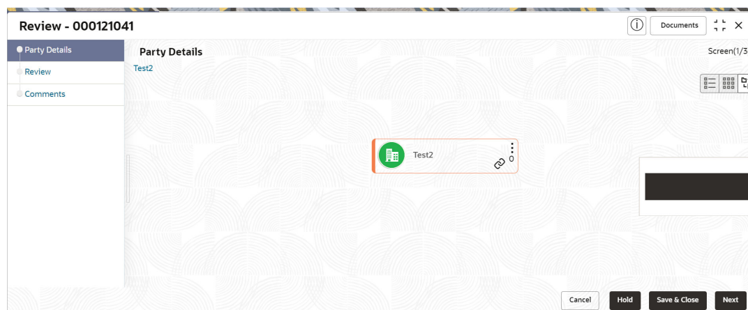
Figure 1-34 Corporate Customer–Review
