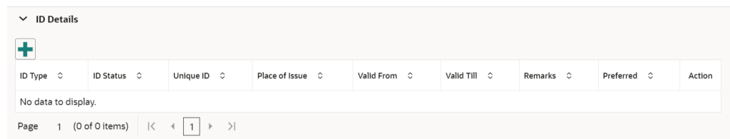
Figure 1-13 ID Details
