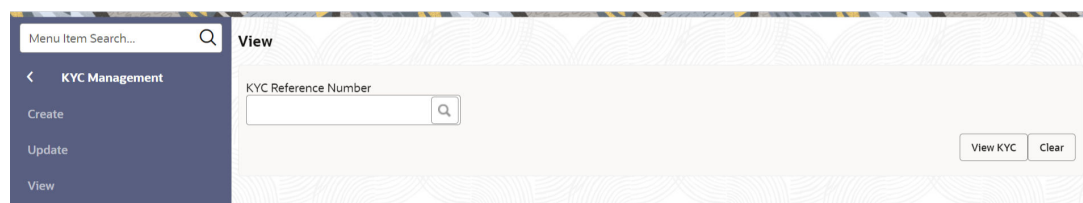
Figure 3-4 View KYC
