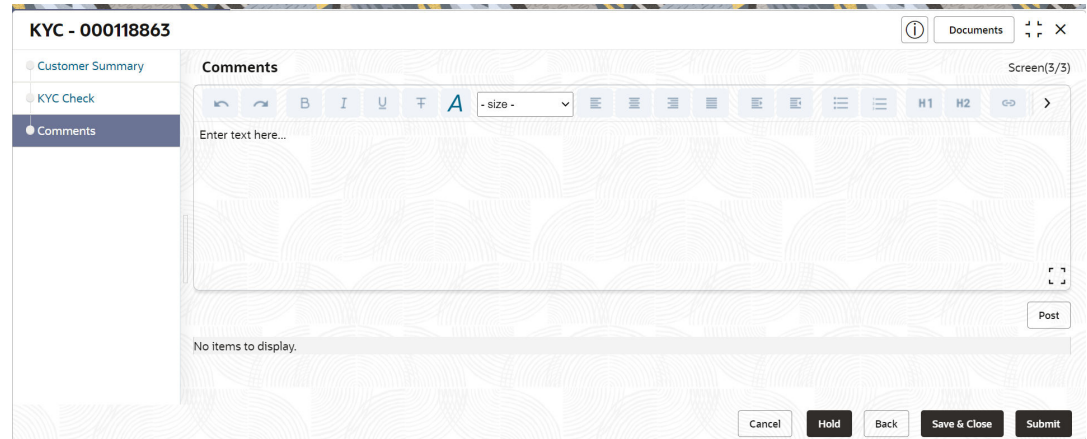
Figure 1-43 KYC – Comments
