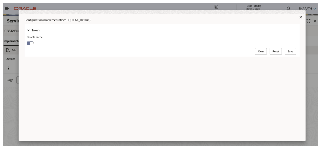
Figure 4-11 Configuration
