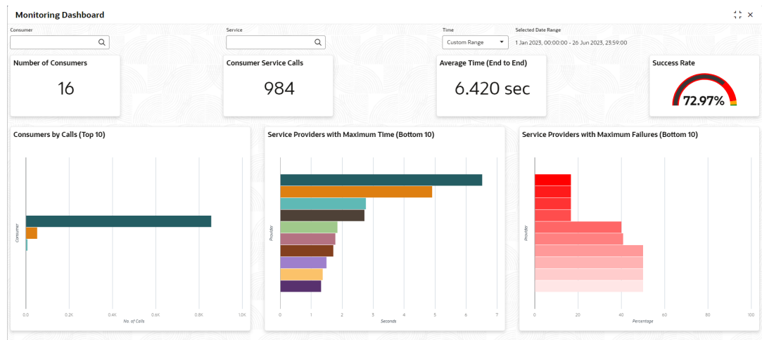
Figure 15-1 Monitoring Dashboard
