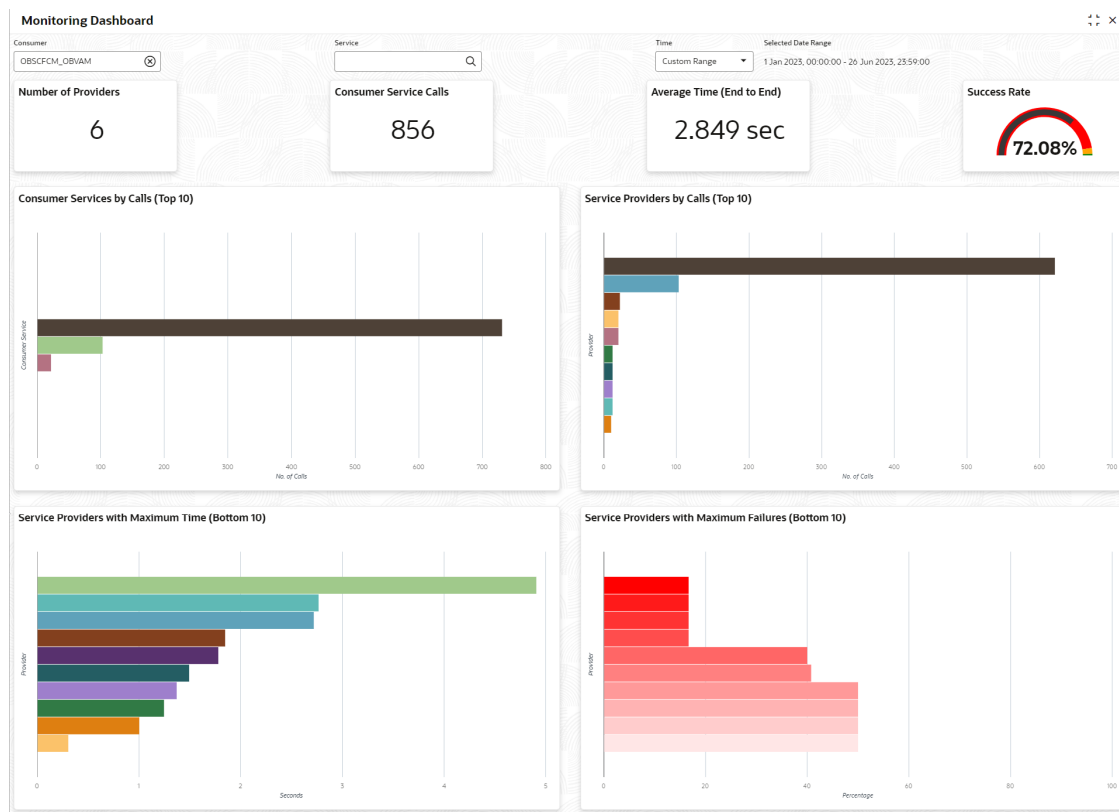
Figure 15-2 Consumer Page
