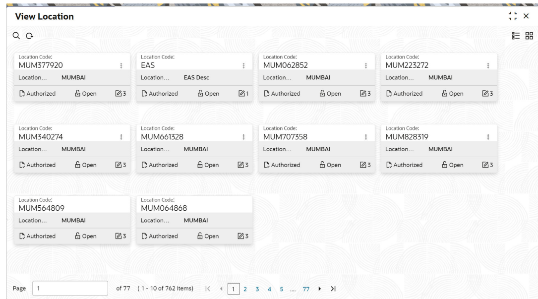
Figure 1-11 View Location
