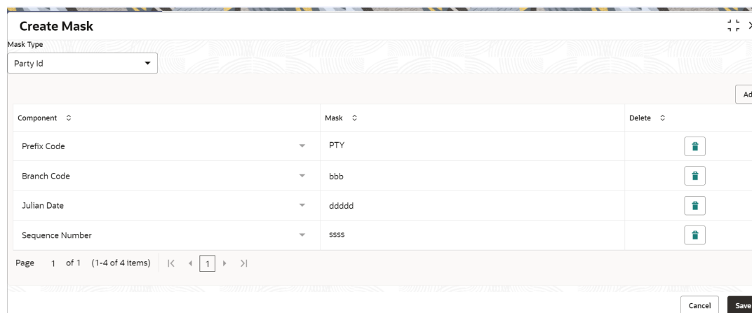
Figure 1-12 Create Mask
