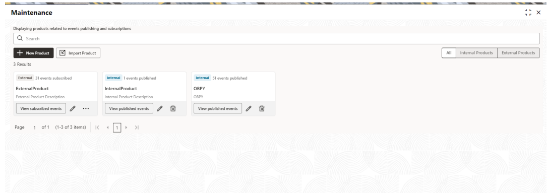
Figure 1-35 Event Maintenance
