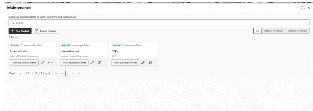
Figure 1-31 Event Maintenance
