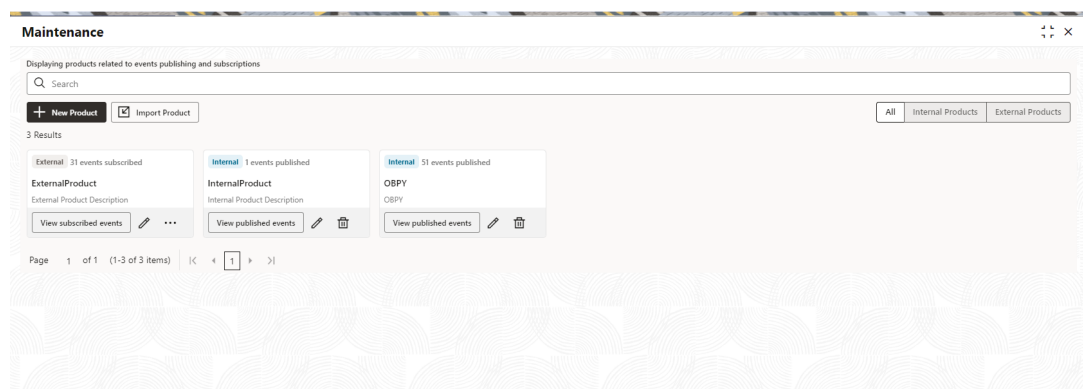
Figure 1-33 Event Maintenance
