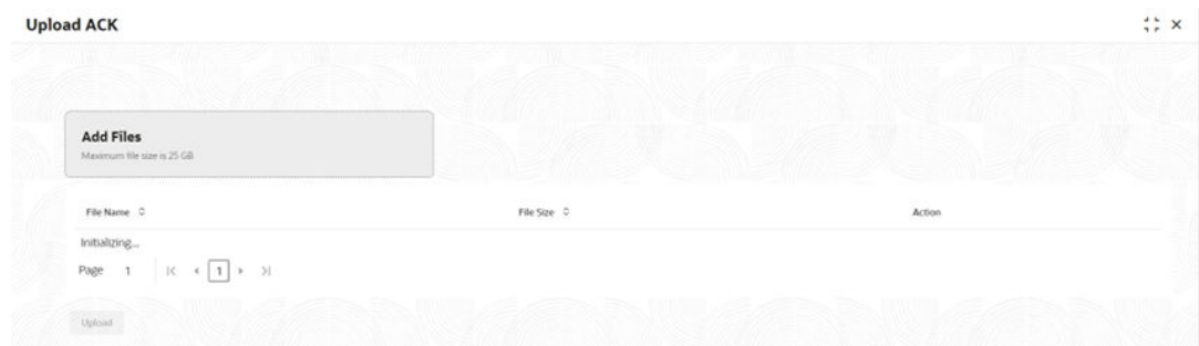
Figure 1-53 Upload ACK
