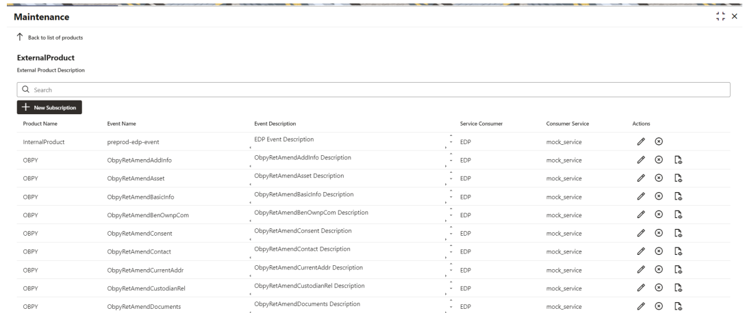
Figure 1-36 Published Events
