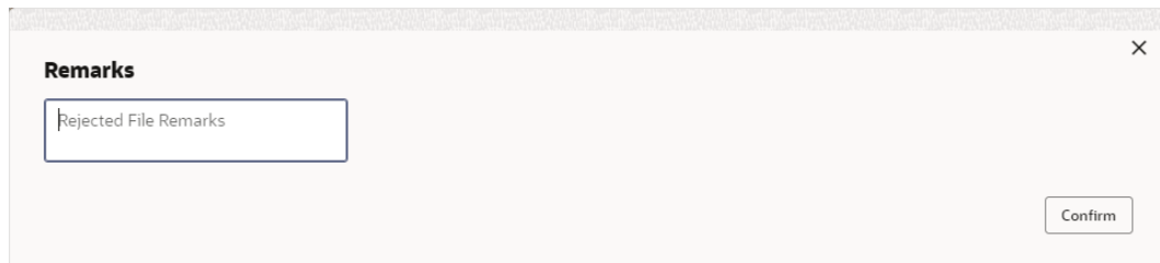
Figure 4-7 Remarks - Reject
