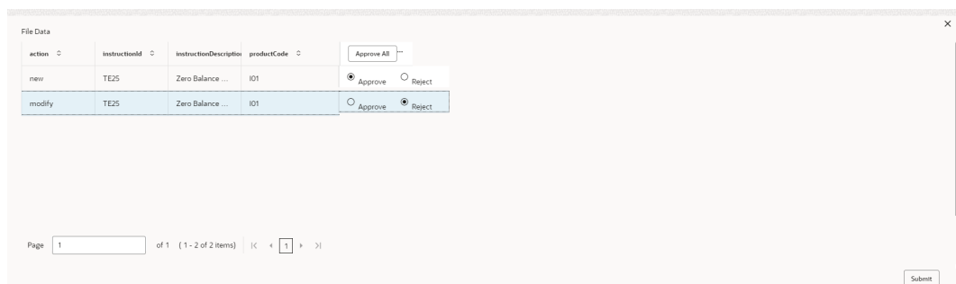
Figure 4-8 File Data
