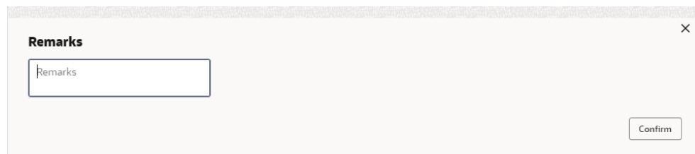
Figure 4-6 Remarks - Approve
