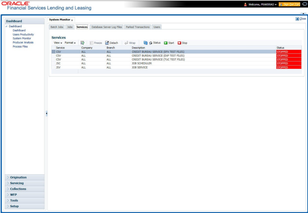
Figure 3-4 Services
