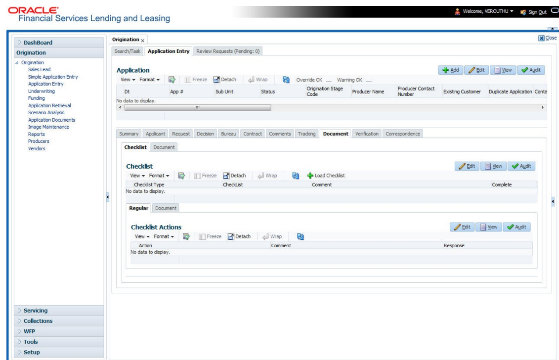
Figure 6-14 Document
