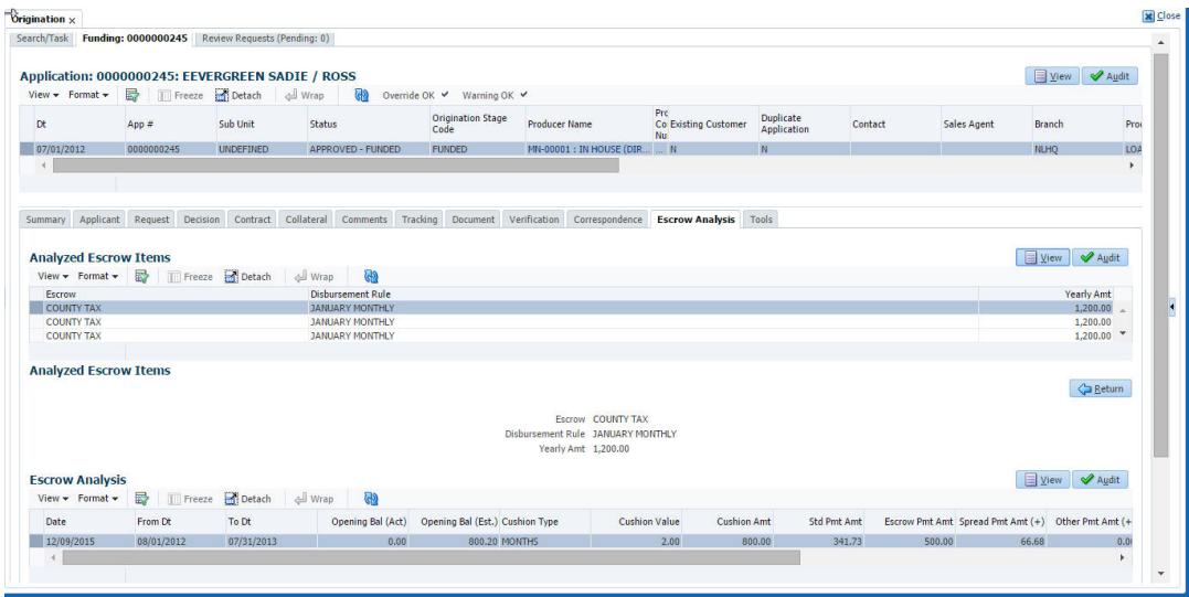
Figure 8-20 Escrow Analysis
