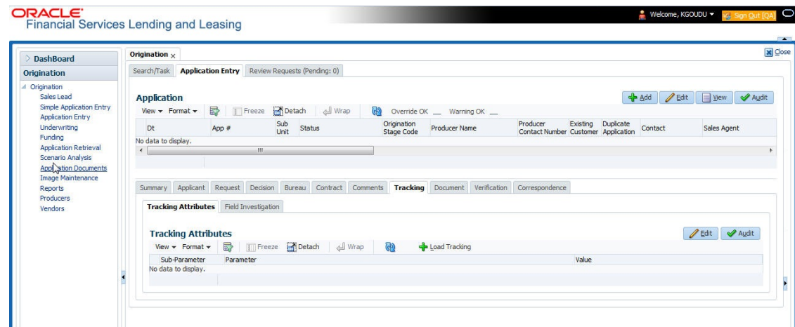
Figure 6-13 Tracking
