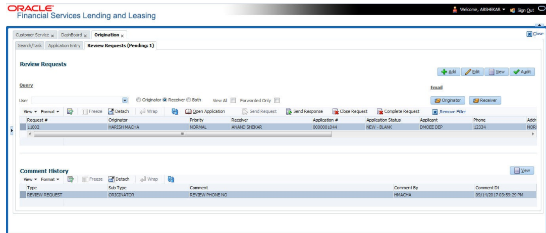
Figure 7-21 Review Requests
