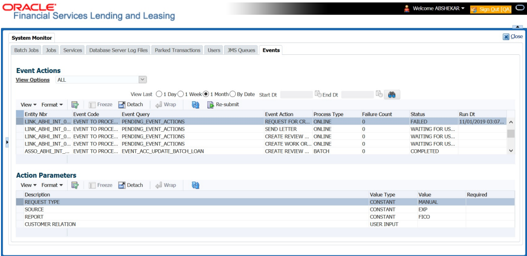
Figure 3-9 Events
