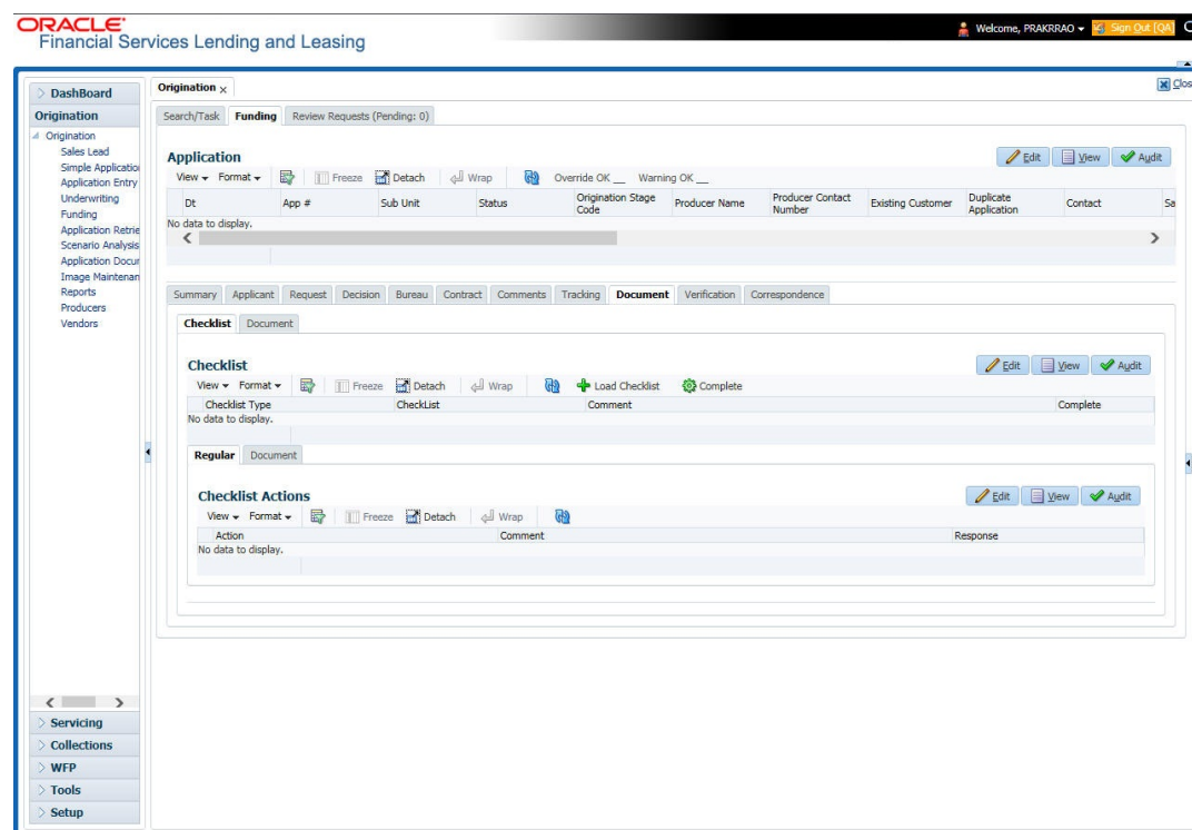
Figure 8-17 Document
