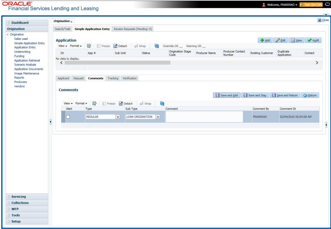
Figure 5-10 Comments
