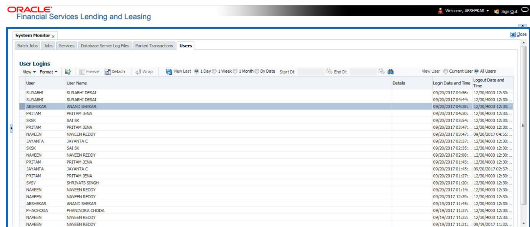
Figure 3-6 Users
