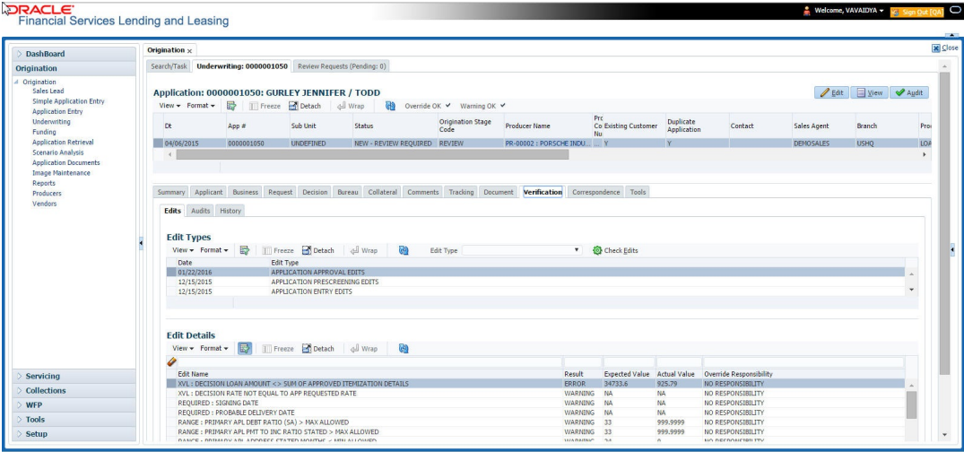
Figure 7-17 Verification
