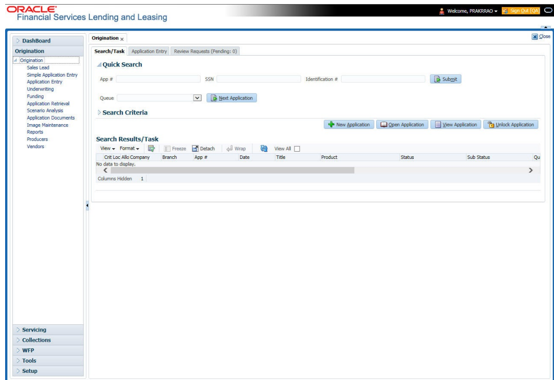
Figure 2-4 Search/Task tab
