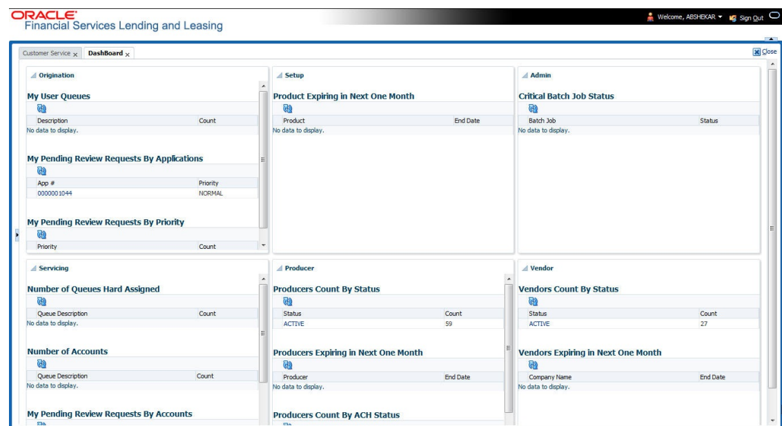
Figure 7-20 Review Request-DashBoard
