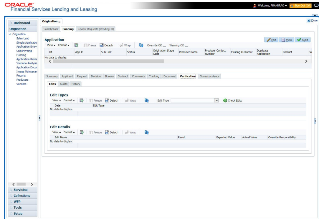
Figure 8-18 Verification
