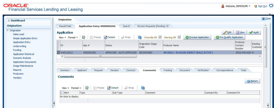
Figure 6-12 Comments
