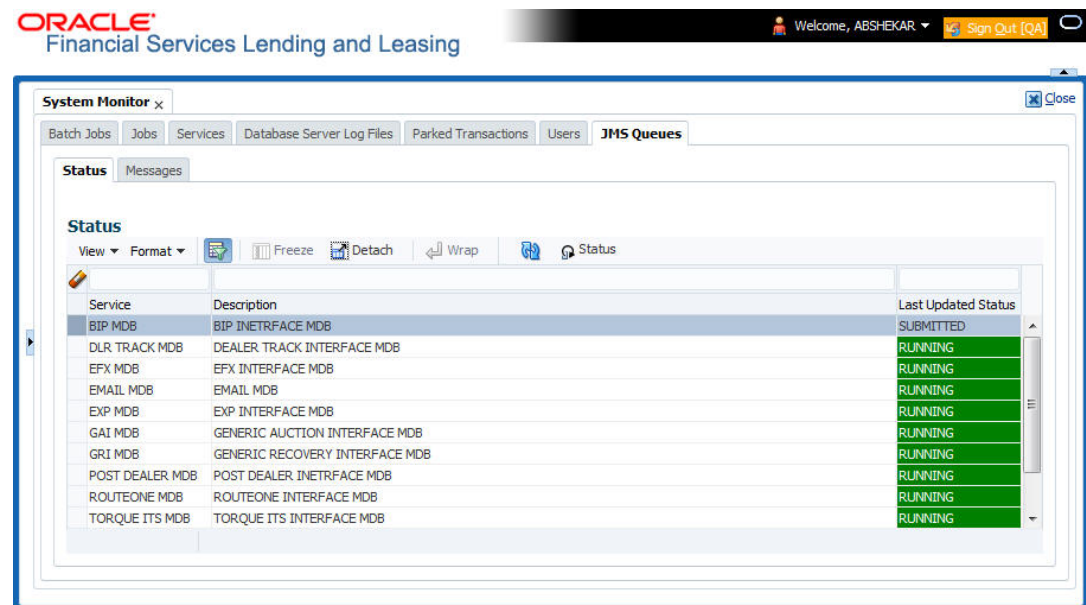
Figure 3-7 JMS Queues
