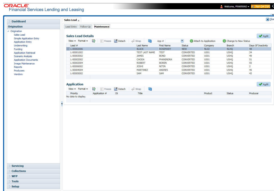
Figure 4-5 Maintenance
