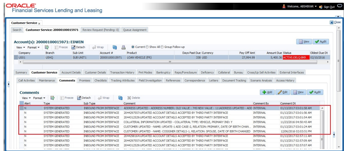
Figure C-3 Update Case
