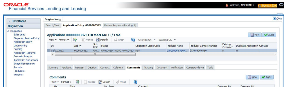
Figure 6-11 Collateral-Other
