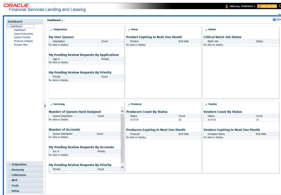
Figure 3-1 Dashboard
