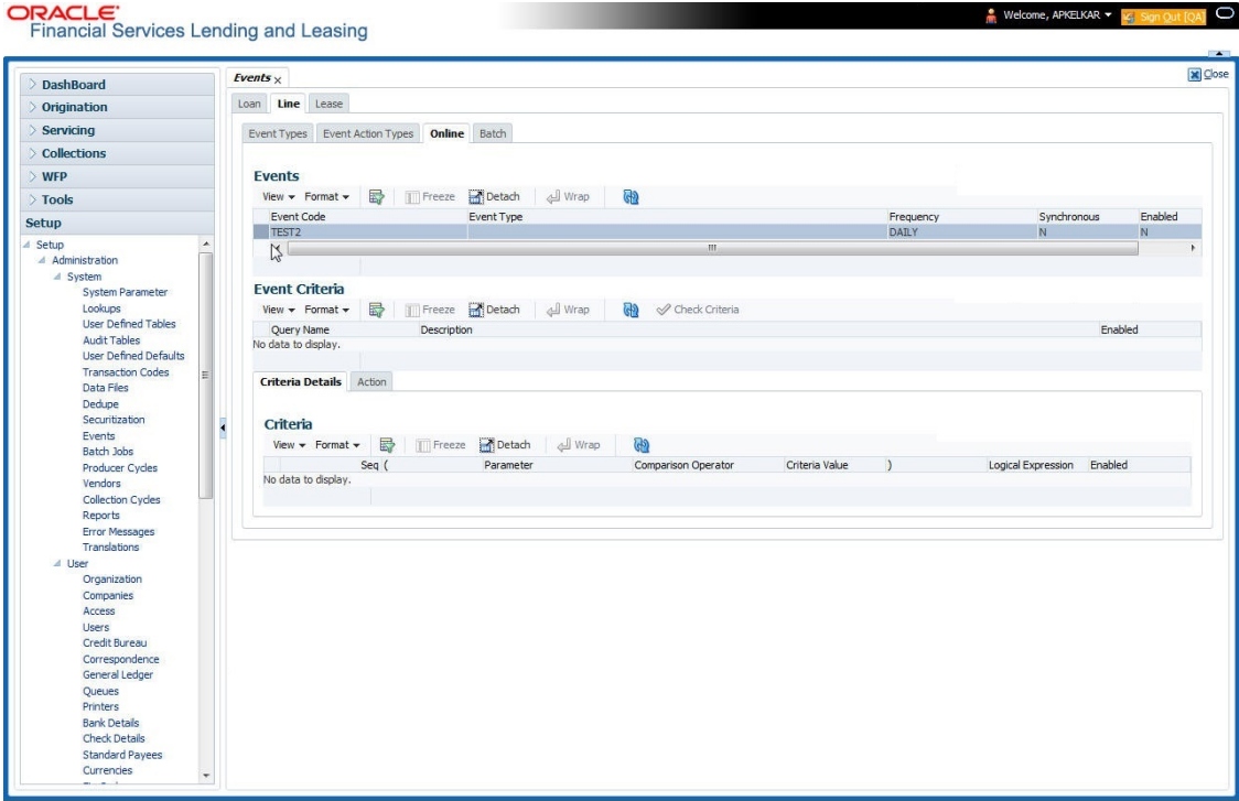
Figure 2-15 Online Setup
