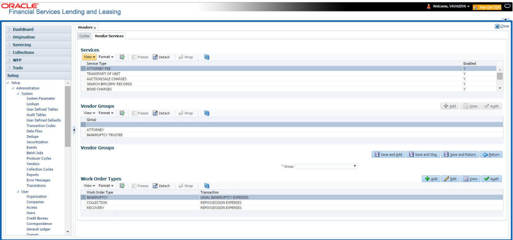
Figure 2-29 Vendor Services
