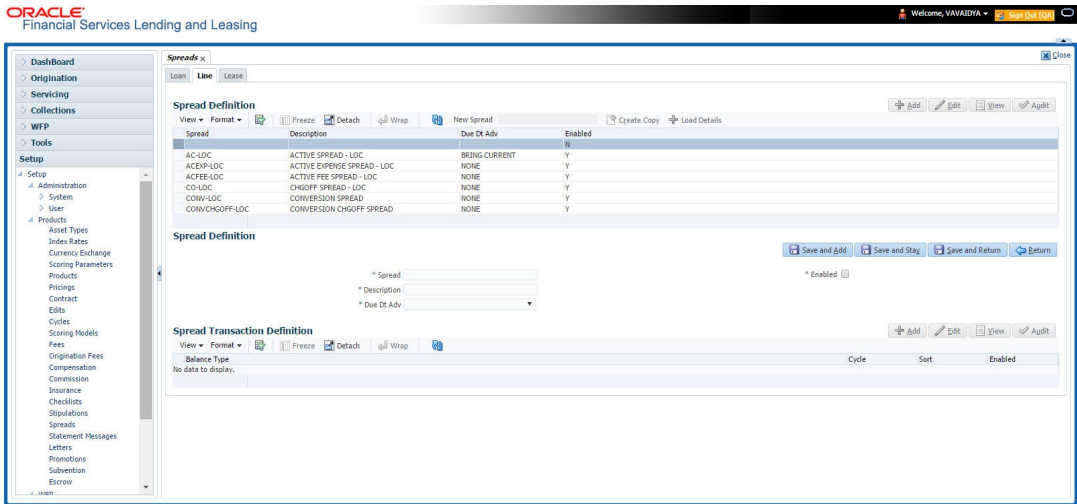
Figure 4-12 Spreads
