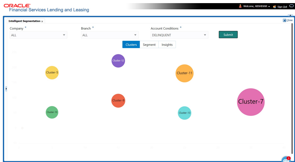
Figure 3-48 Cluster view
