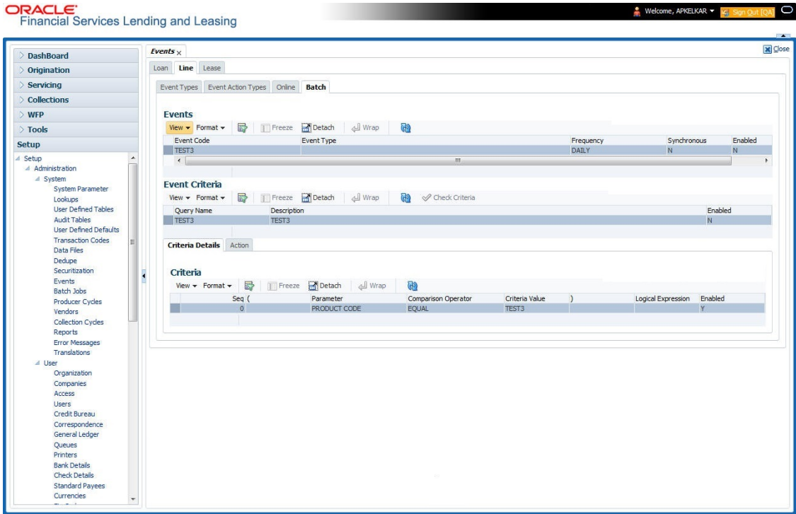
Figure 2-16 Batch Setup
