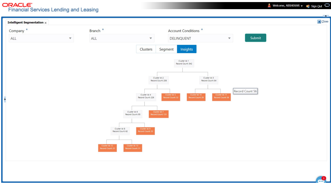
Figure 3-50 Insights View
