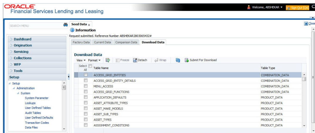
Figure 2-39 Seed Data_Download
