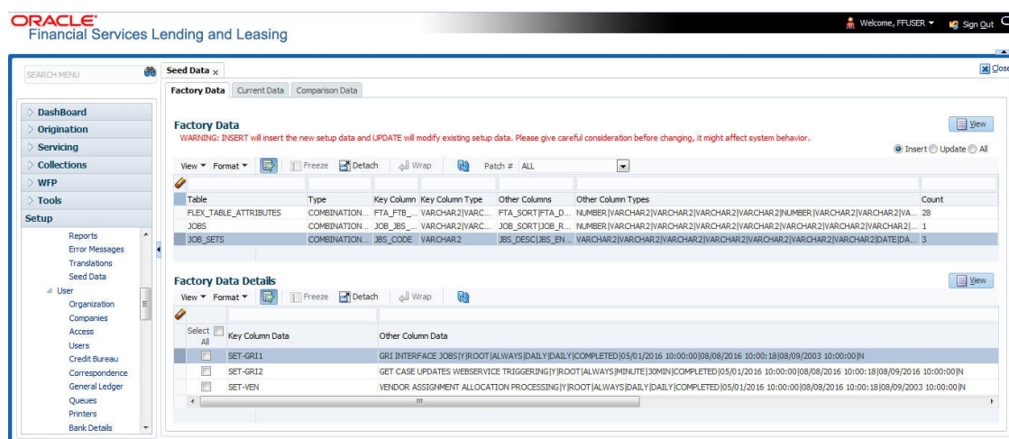
Figure 2-36 Seed Data_Factory
