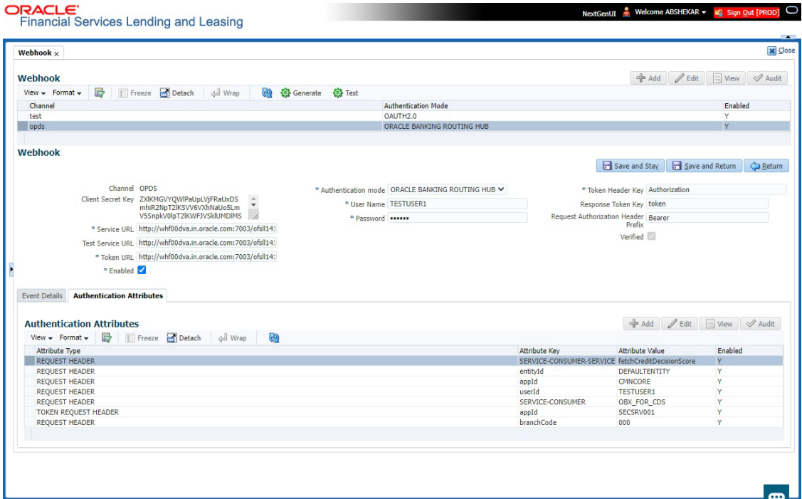
Figure 2-42 Webhook
