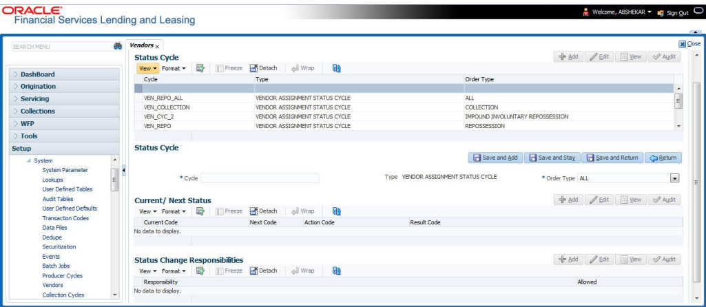
Figure 2-28 Vendor cycles
