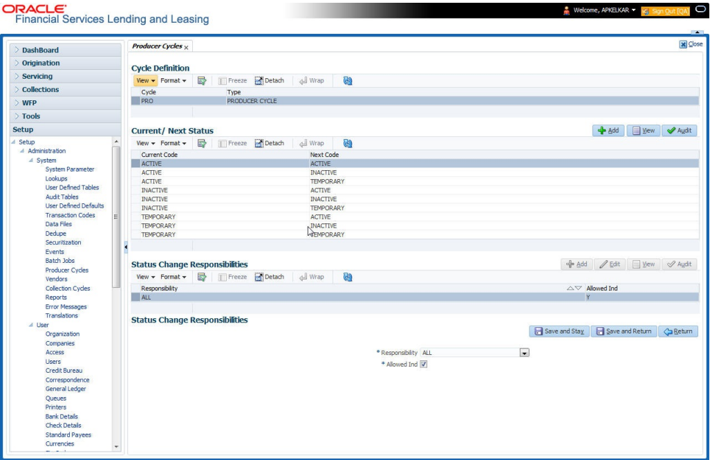
Figure 2-23 Producer Cycles
