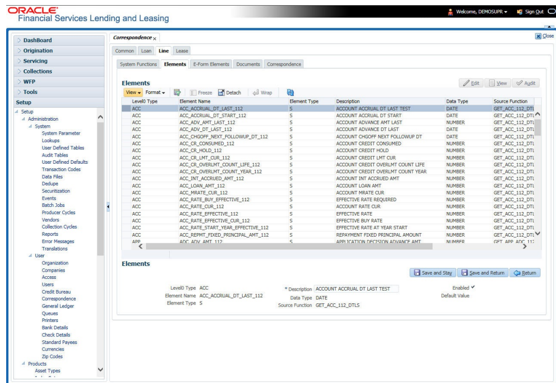
Figure 3-29 Correspondence_Line_Elements
