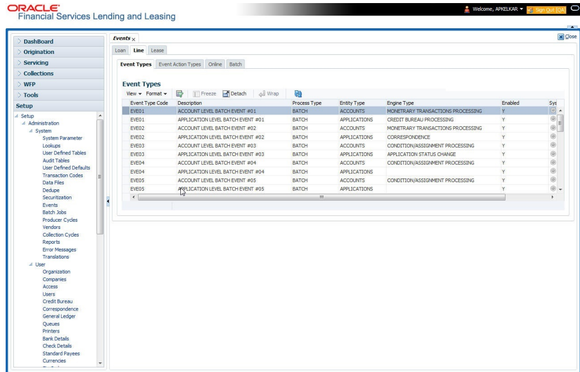
Figure 2-13 Events Setup
