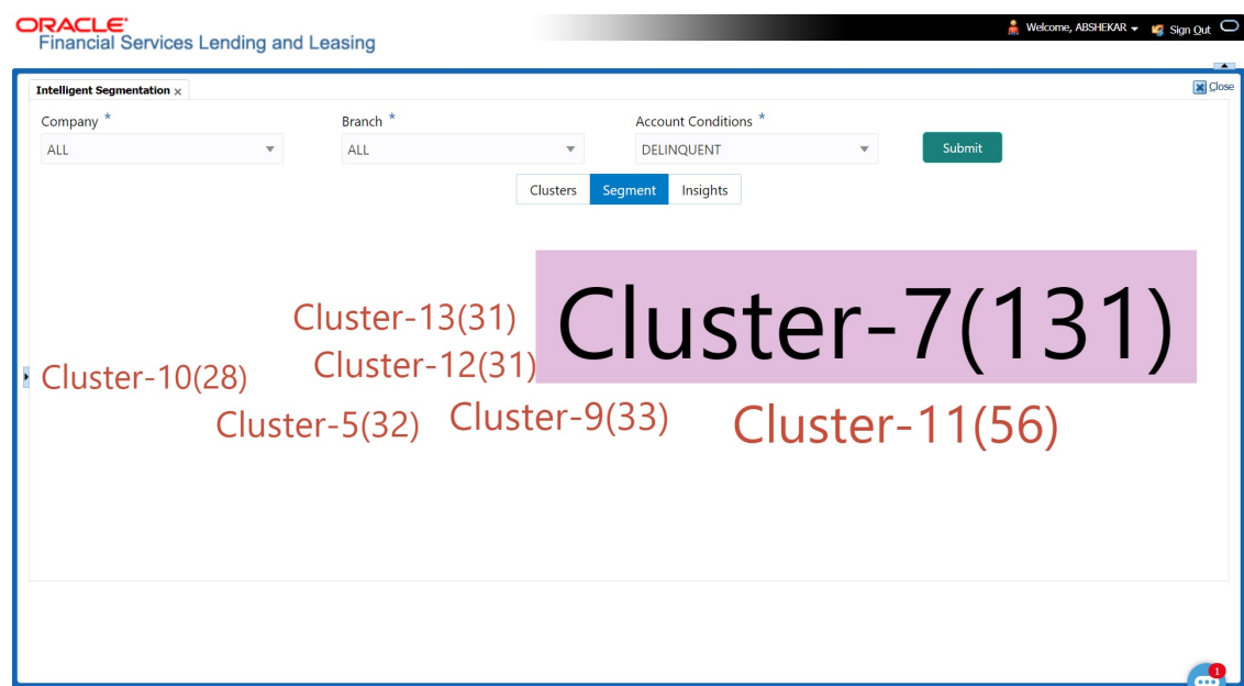
Figure 3-49 Segment View
