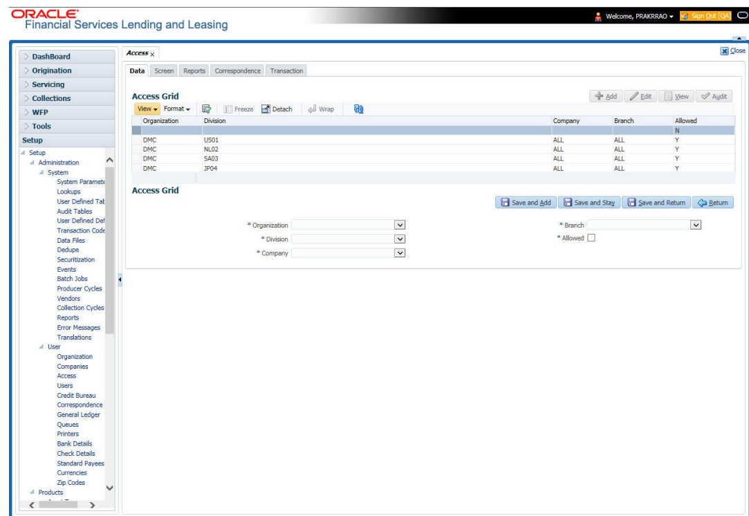
Figure 3-8 Access Grid
