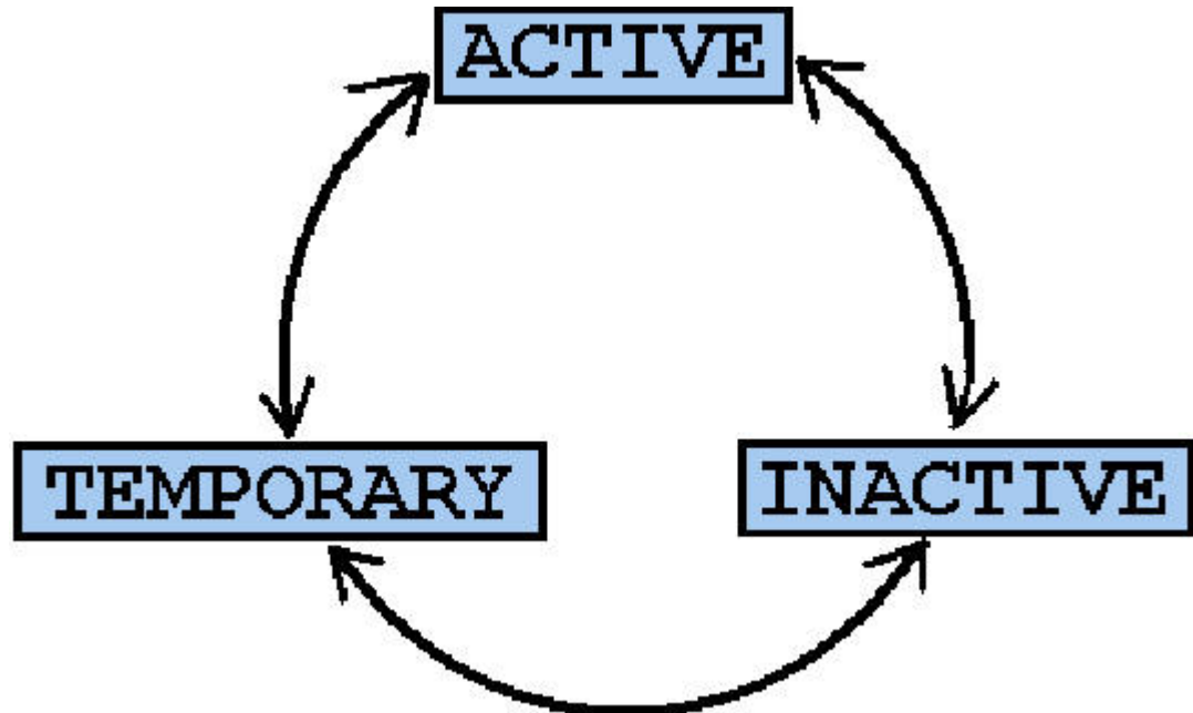
Figure 2-22 Producer Cycle
