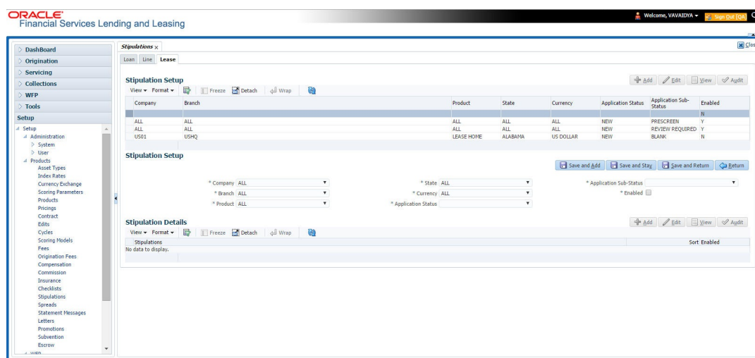
Figure 4-20 Stipulations
