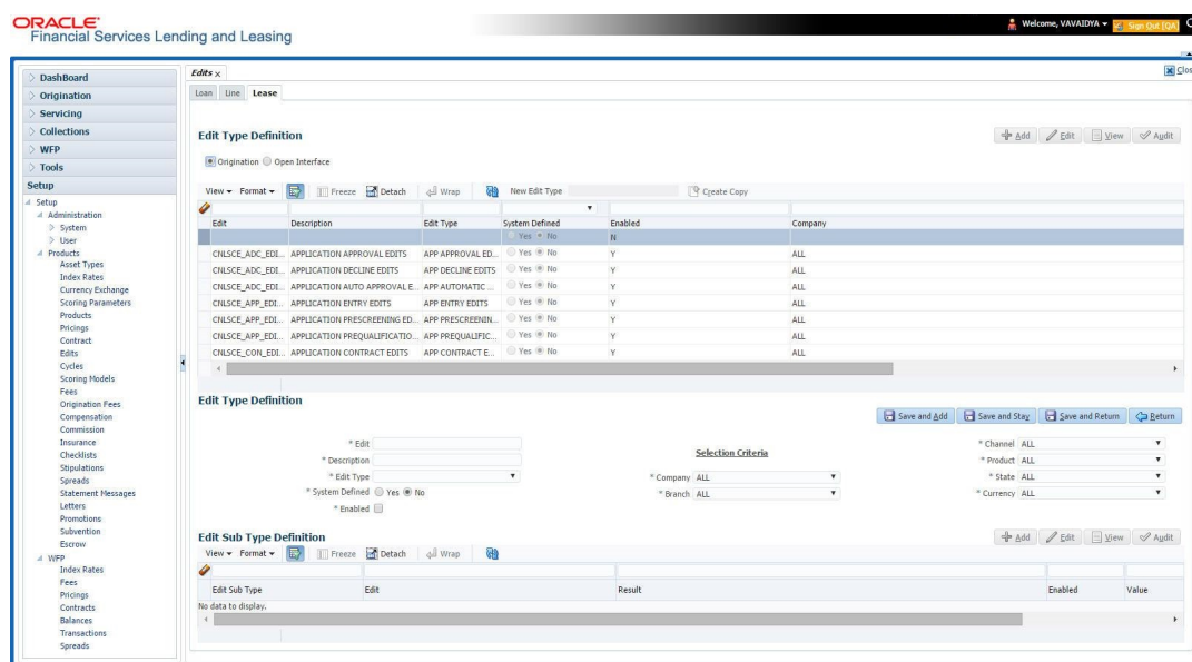
Figure 4-8 Edits
