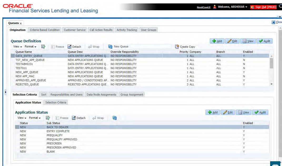
Figure 3-37 Origination Definition
