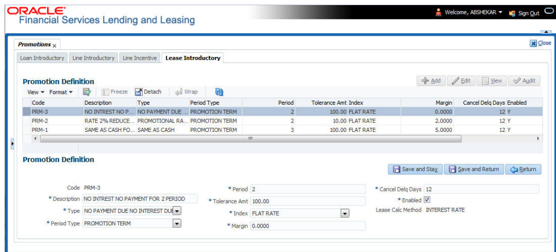
Figure 4-22 Promotions-Lease Introductory
