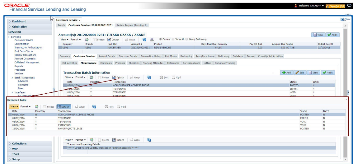
Figure 1-17 Detached Table
