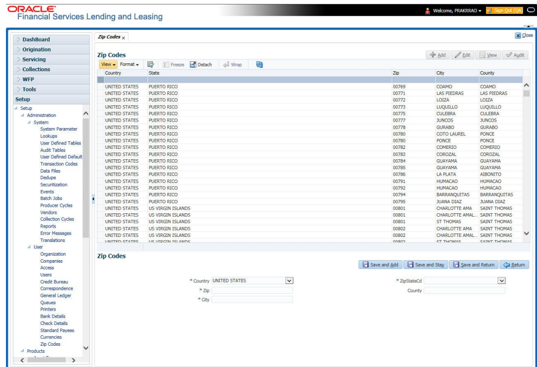
Figure 3-51 Zip Codes
