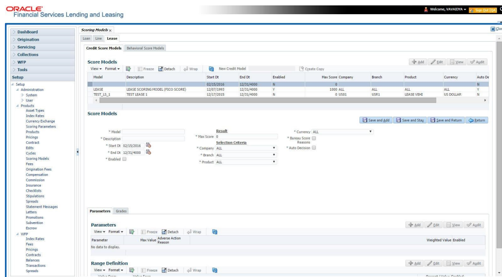
Figure 4-12 Score Models
