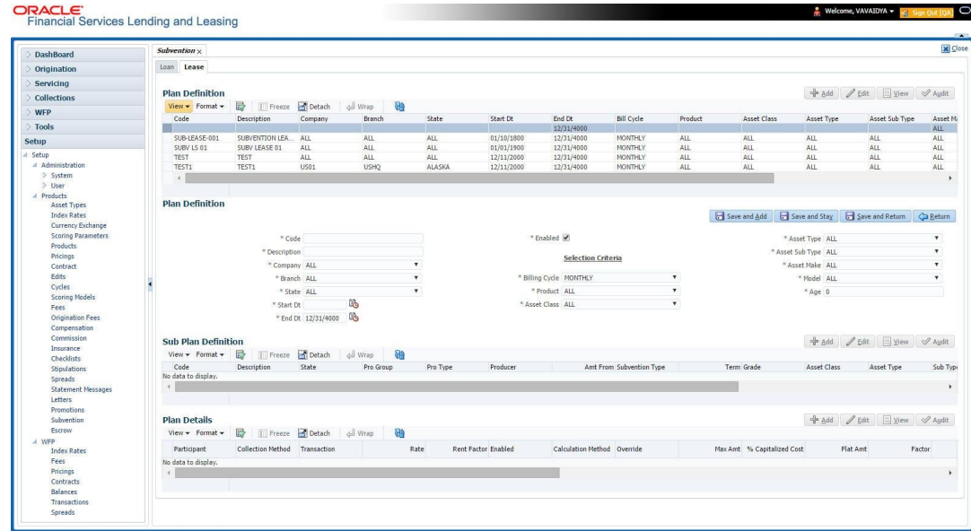
Figure 4-23 Subvention
