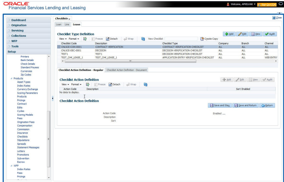
Figure 4-19 Checklists
