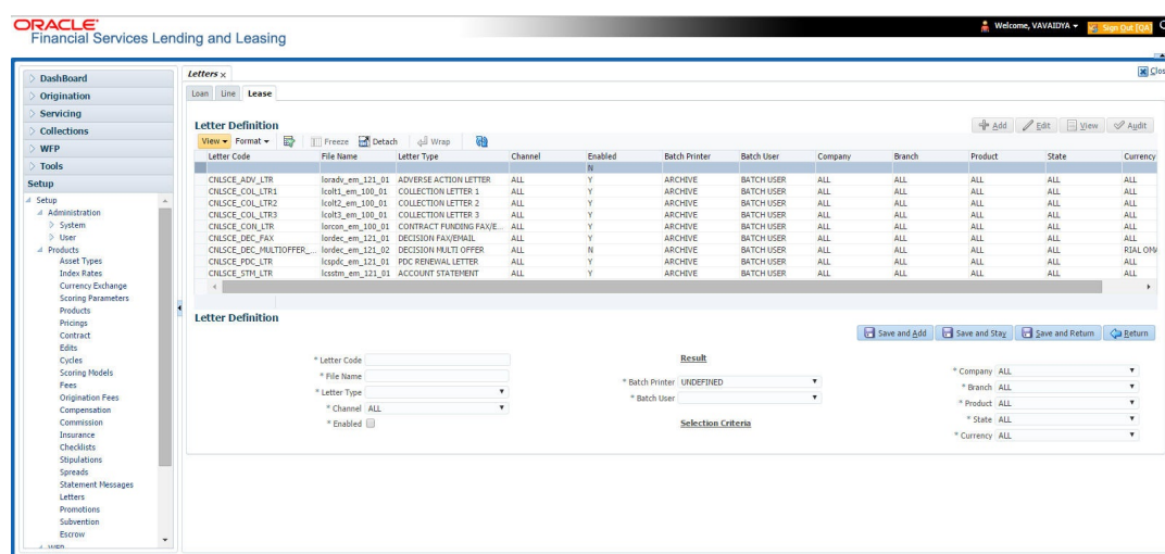
Figure 4-21 Letters
