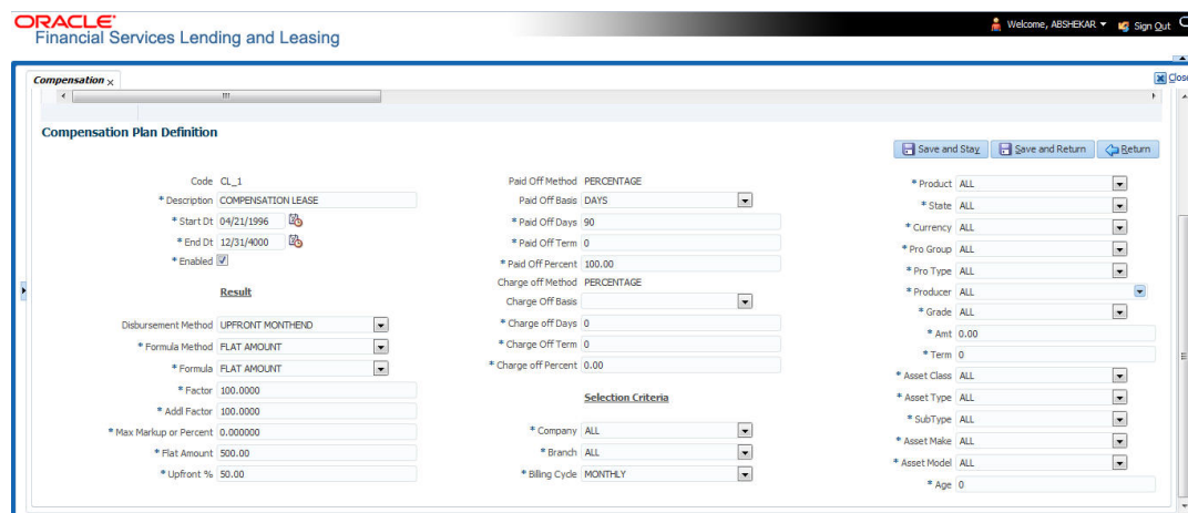
Figure 4-16 Compensation
