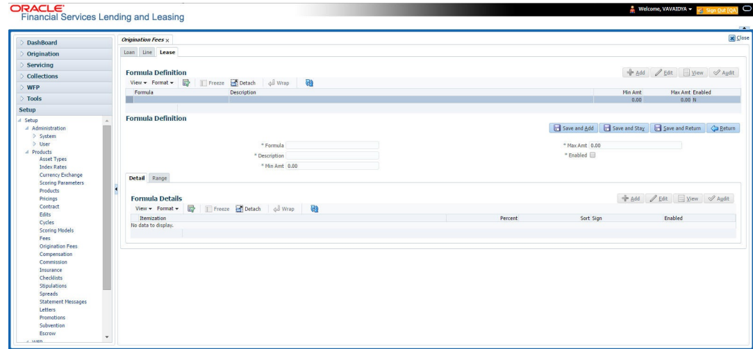
Figure 4-15 Origination Fees
