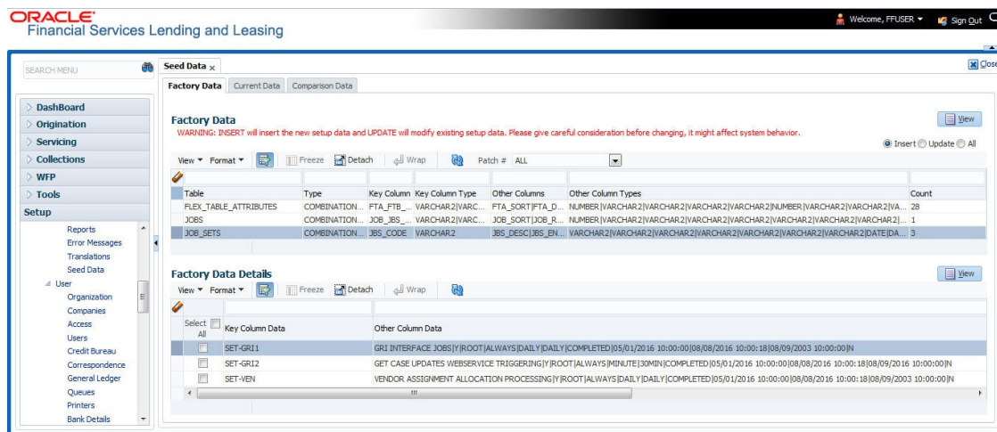
Figure 2-37 Seed Data_Factory
