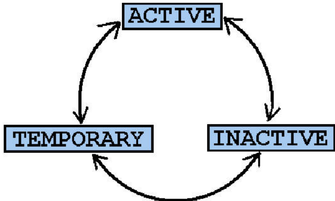
Figure 2-23 Producer Cycle
