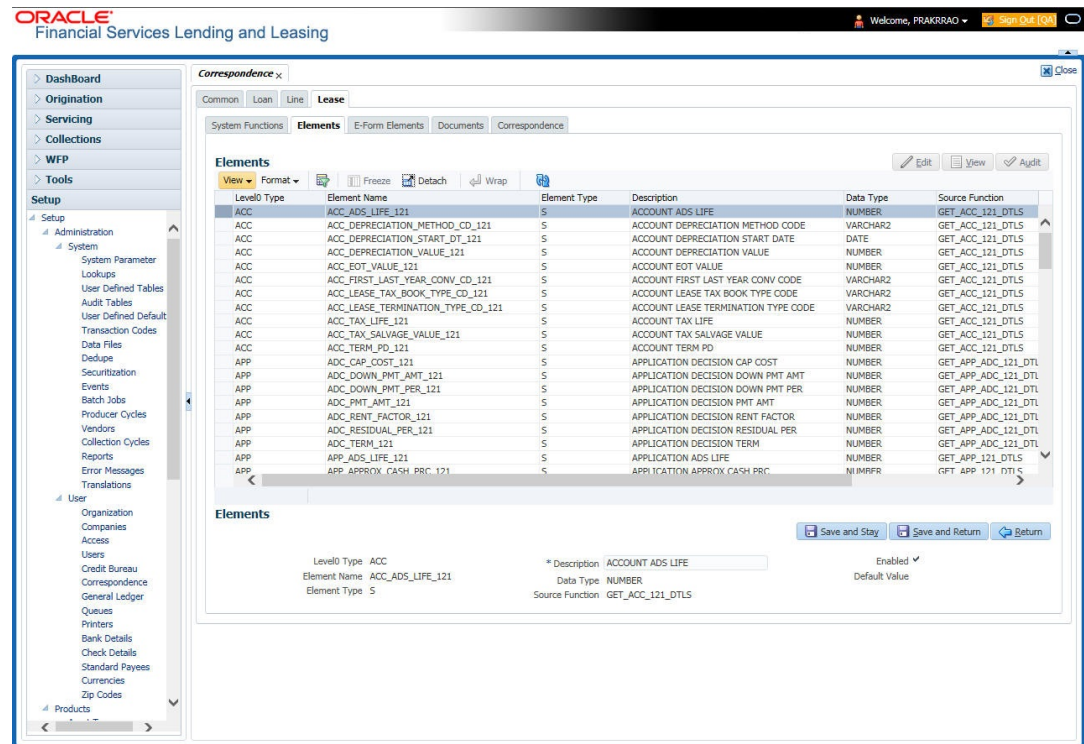
Figure 3-28 Correspondence_Lease_Elements
