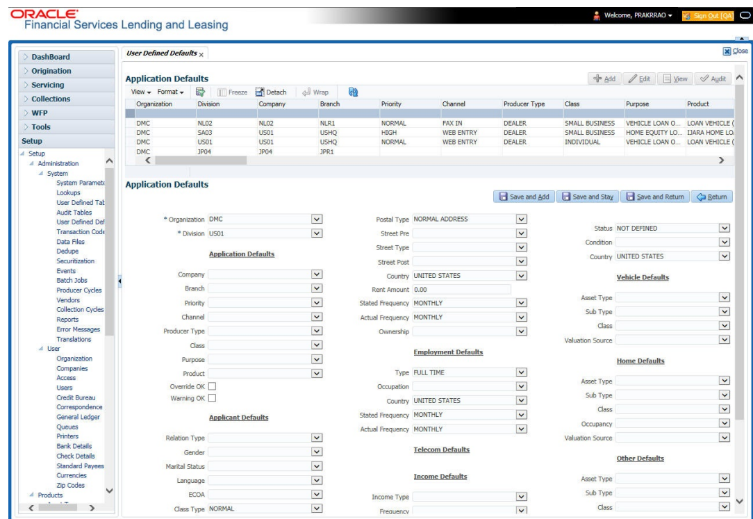
Figure 2-8 Application Defaults
