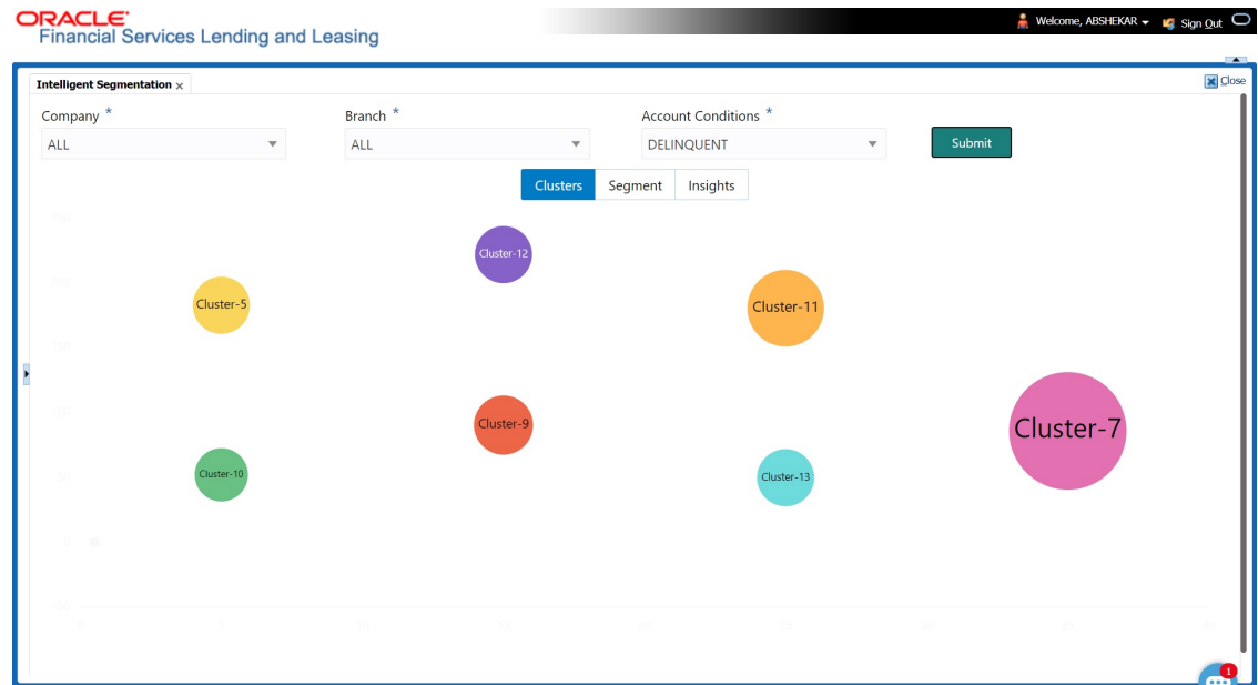
Figure 3-41 Cluster view
