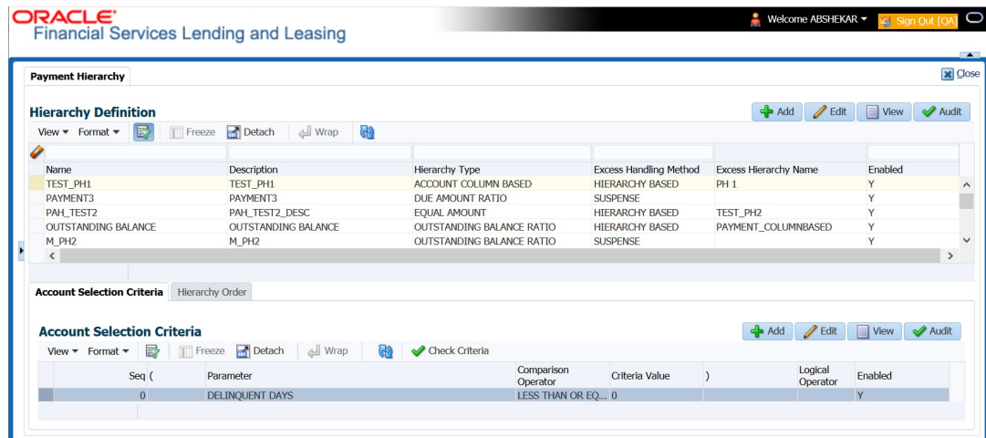
Figure 3-53 Hierarchy Definition
