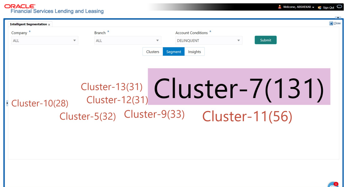
Figure 3-42 Segment View
