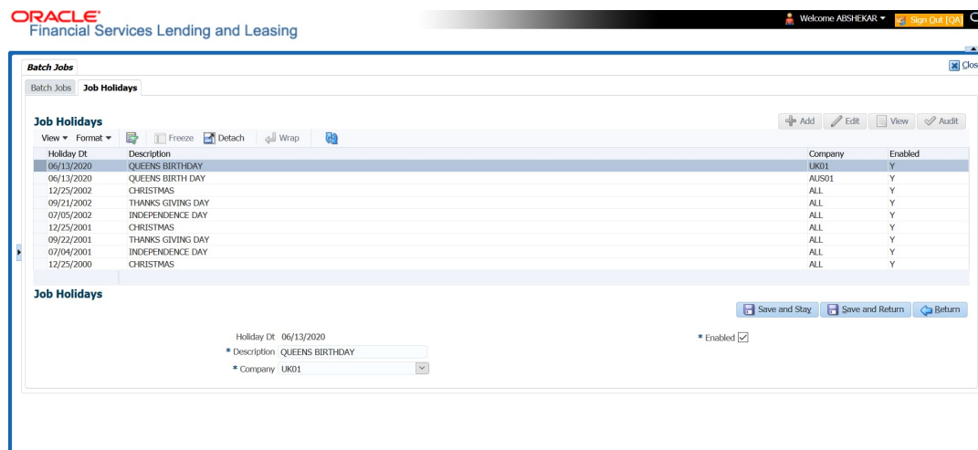
Figure 2-22 Job Holidays
