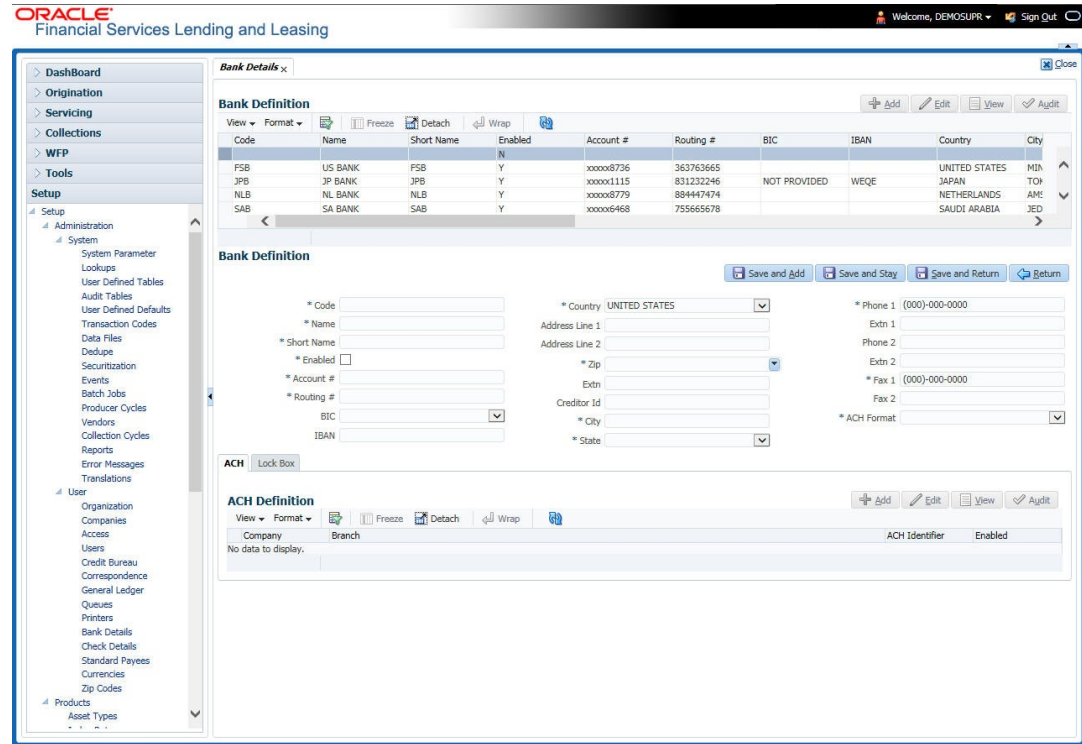
Figure 3-46 Banks Definition
