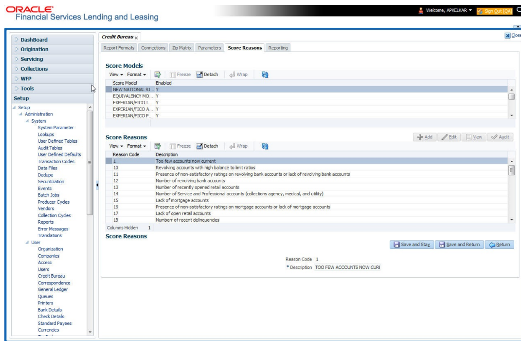
Figure 3-20 Score Models
