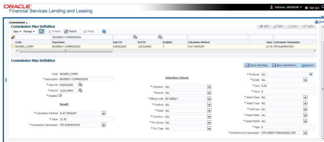
Figure 4-17 Commission
