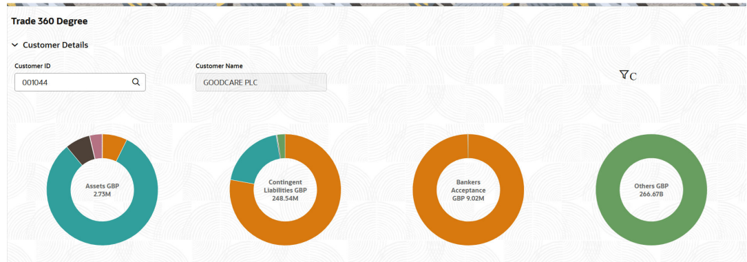
Figure 1-2 Customer 360 Degree
