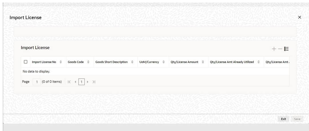
Figure 5-20 Import License
