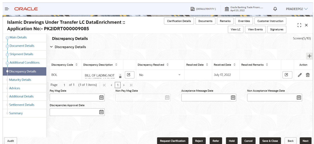
Figure 2-24 Discrepancy Details
