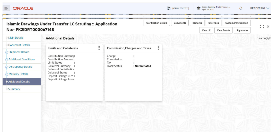
Figure 2-14 Additional Details
