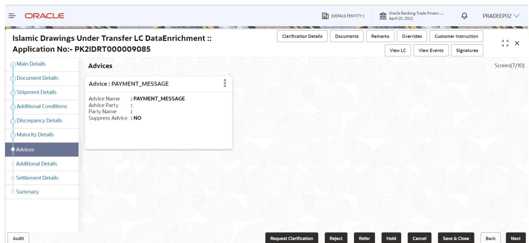
Figure 2-26 Advices
