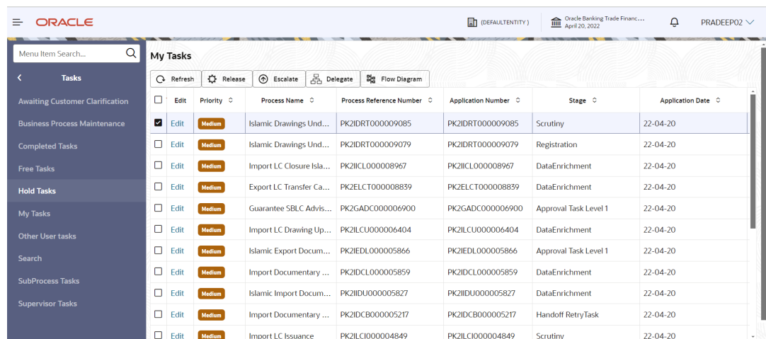
Figure 2-18 My Task
