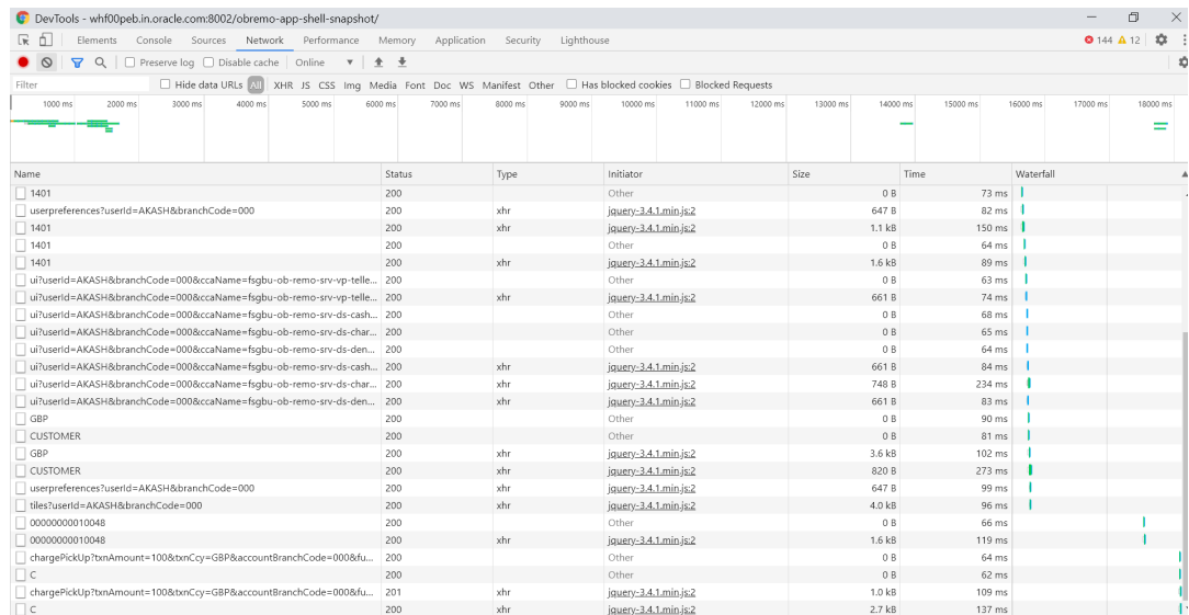
Figure 1-2 Call Responses
