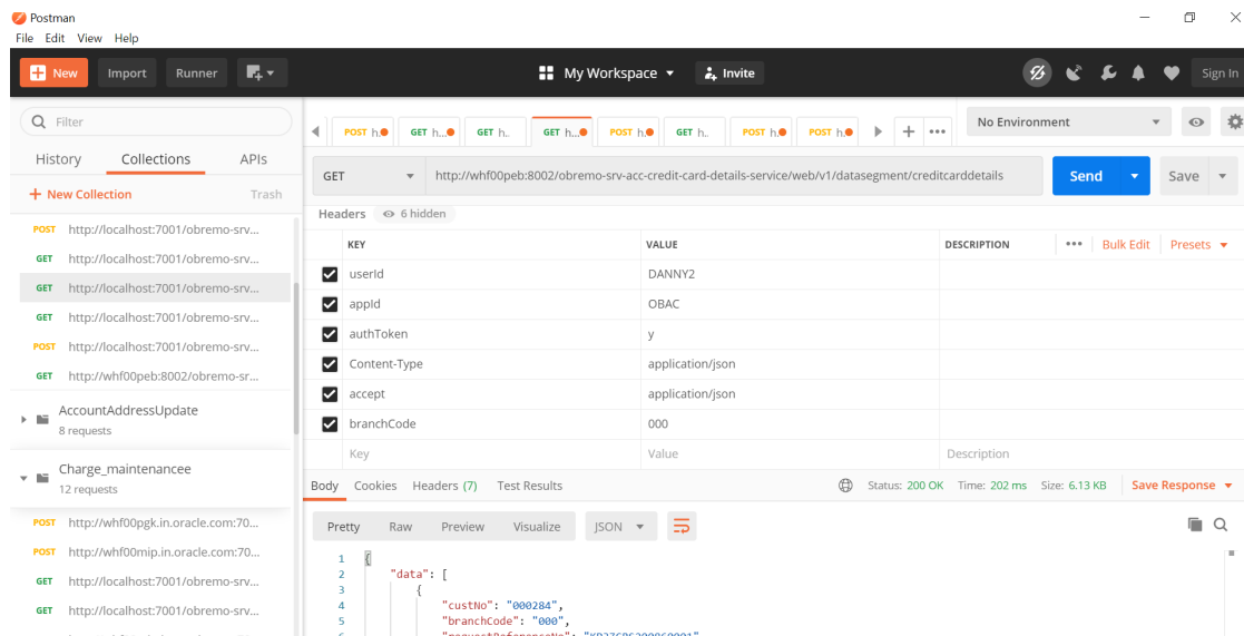
Figure 4-6 Postman
