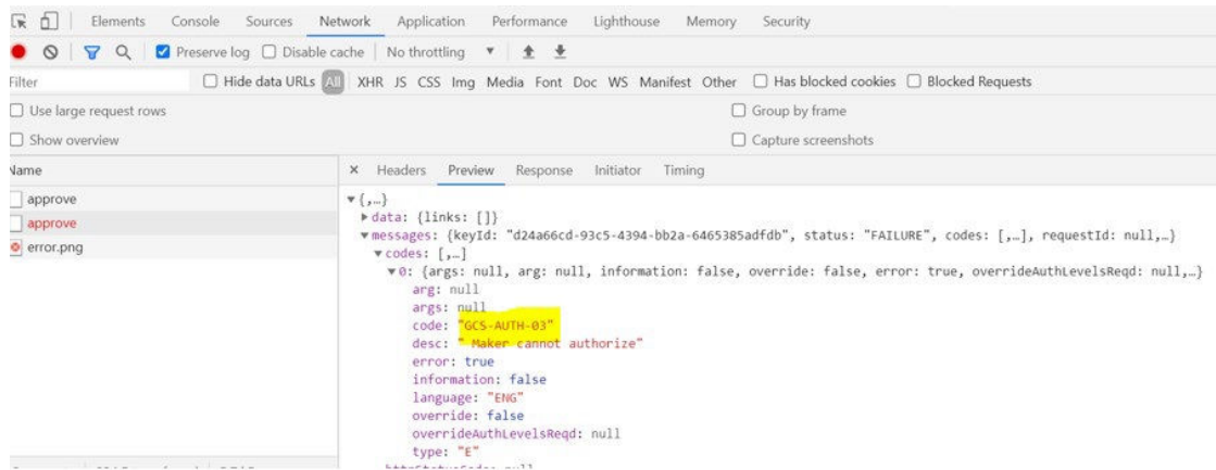
Figure 4-2 Error Code
