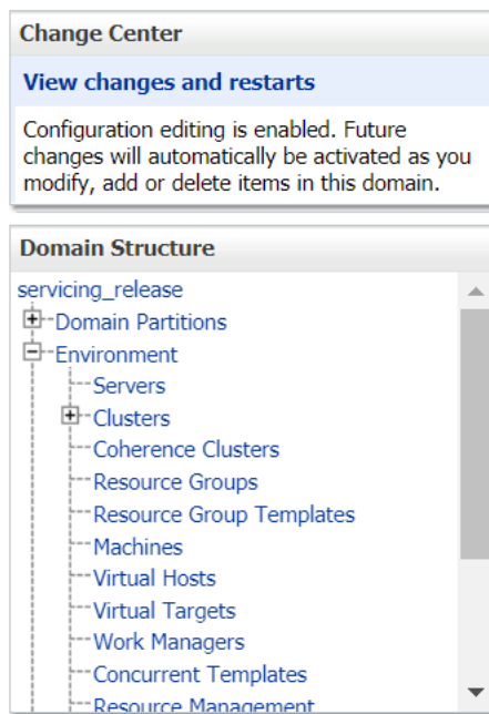
Figure 7-1 Domain Structure
