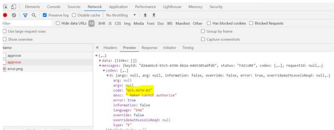
Figure 4-2 Error Code
