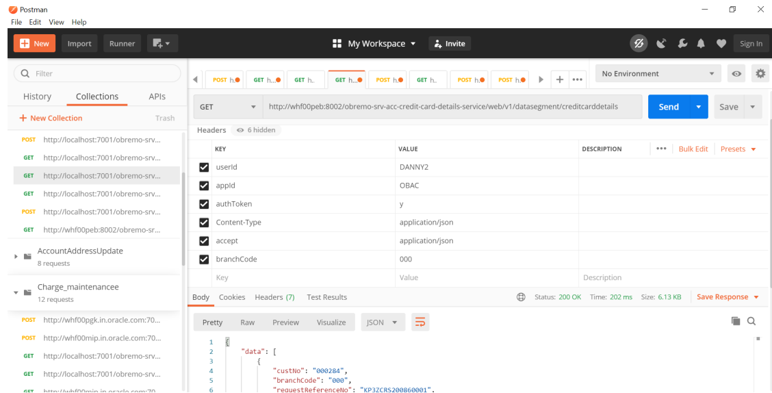
Figure 4-6 Postman
